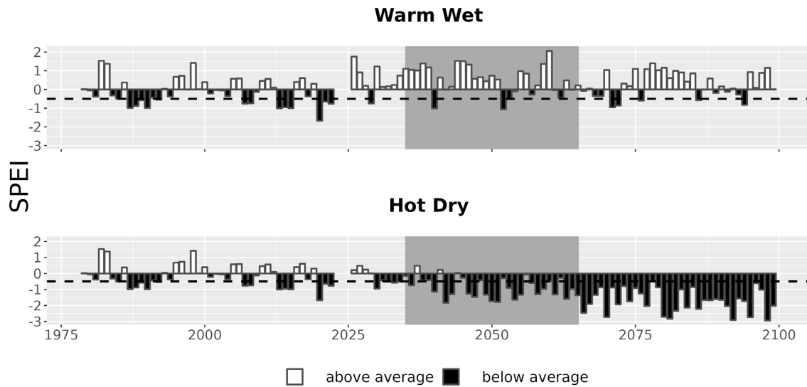
Figure 7. Drought metrics for RORI. Drought index (SPEI; units = standard deviations from historical) timeseries for each climate future. Below-average SPEI (black bars) indicates dry conditions. The dotted line (SPEI = -0.5) indicates drought conditions.
