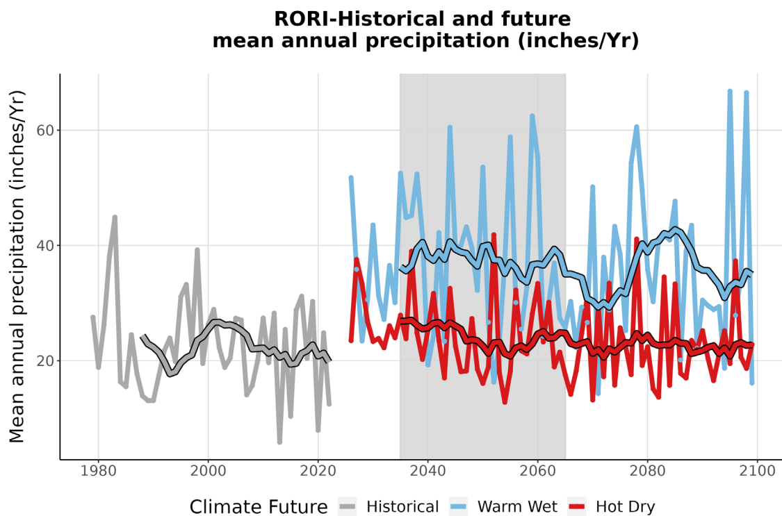
Figure 4. This graph compares observed average annual precipitation at RORI (inches/year) (1979-2022) with projected average annual precipitation for the two climate futures over the period 2023-2099. The historically observed data is shown in gray, the Warm Wet climate future in blue, and the Hot Dry climate future in red. The smooth line running through each projection is the 10-year running average for historical observations and future projections. The gray-shaded area represents the time period that was averaged (2035-2065) to summarize future projections for the year 2050 (Appendix 1).
