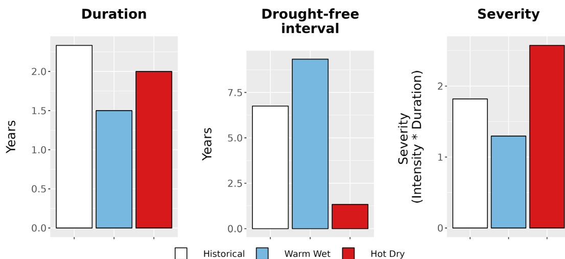
Figure 8. Drought metrics for RORI. (Left) Average drought duration (years) historically (1979-2012) and under each climate future. (Middle) Average drought return interval (years), indicating the expected amount of time between periods of drought, historically and under each climate future. (Right) Average drought severity, a measure of drought intensity multiplied by duration, historically and under each climate future.
