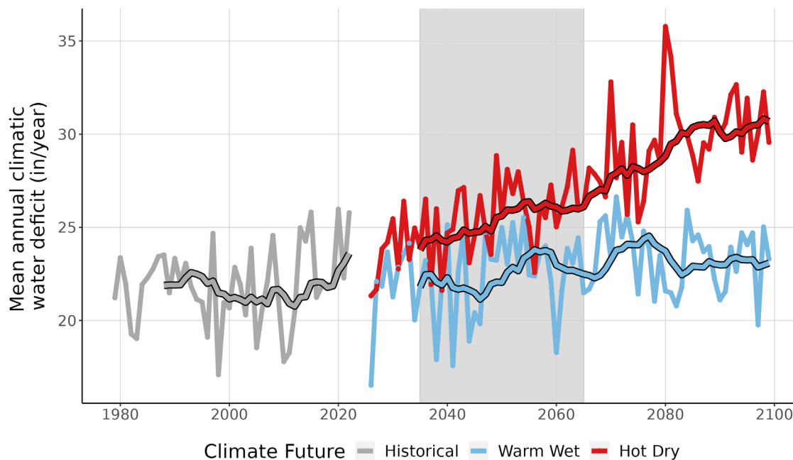
Figure 9. This line graph compares observed climatic water deficit at RORI (inches/year) (1979-2022) with projected climatic water deficit for the two climate futures over the period 2023-2099. The historical observation data is shown in gray, the Warm Wet climate future in blue, and the Hot Dry climate future in red. The smooth line running through each projection is the 10-year running average for historical observations and future projections. Gray-shaded area represents the time period that was averaged (2035-2065) to summarize future projections for the year 2050.
