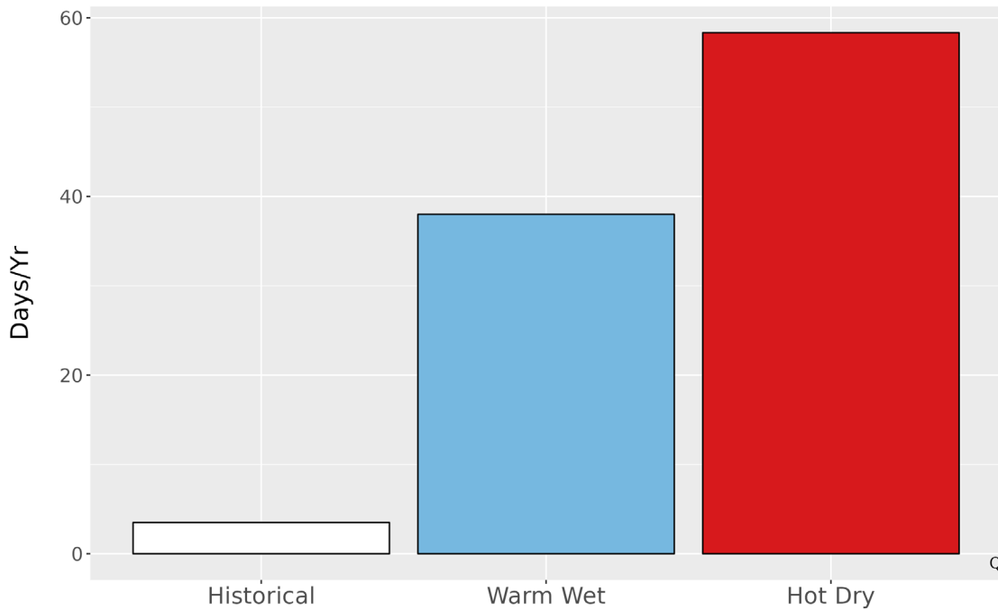
Figure 5. Metrics of extreme temperature at RORI. The bar graph represents the average number of days annually with temperatures greater than the historical 99th percentile (85.4 °F) historically (1979-2012) and for the two climate futures (2050).
