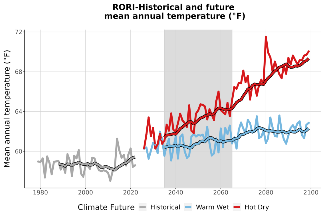
Figure 3. This graph compares observed average annual temperature at RORI (°F) (1979-2022) with projected average annual temperature for the two climate futures over the period 2023-2099. The historically observed data is shown in gray, the Warm Wet climate future in blue, and the Hot Dry climate future in red. The smooth line
