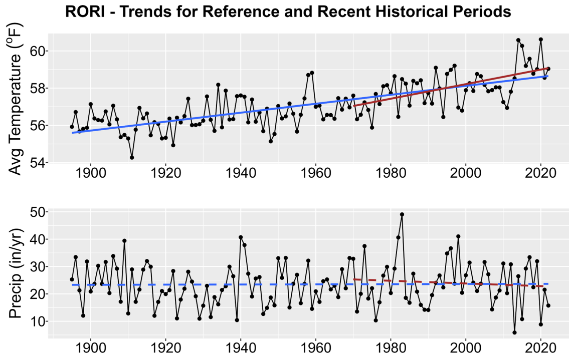
Figure 1. Historical trends in annual average temperature (upper plot) and annual total precipitation (lower plot) for RORI from 1895-2022. Black points show yearly values while blue lines are linear regressions for the entire period record and red lines for 1970-2022 trends. Solid lines are significant trends (i.e., p < 0.05 ); dashed lines are not statistically significant.
