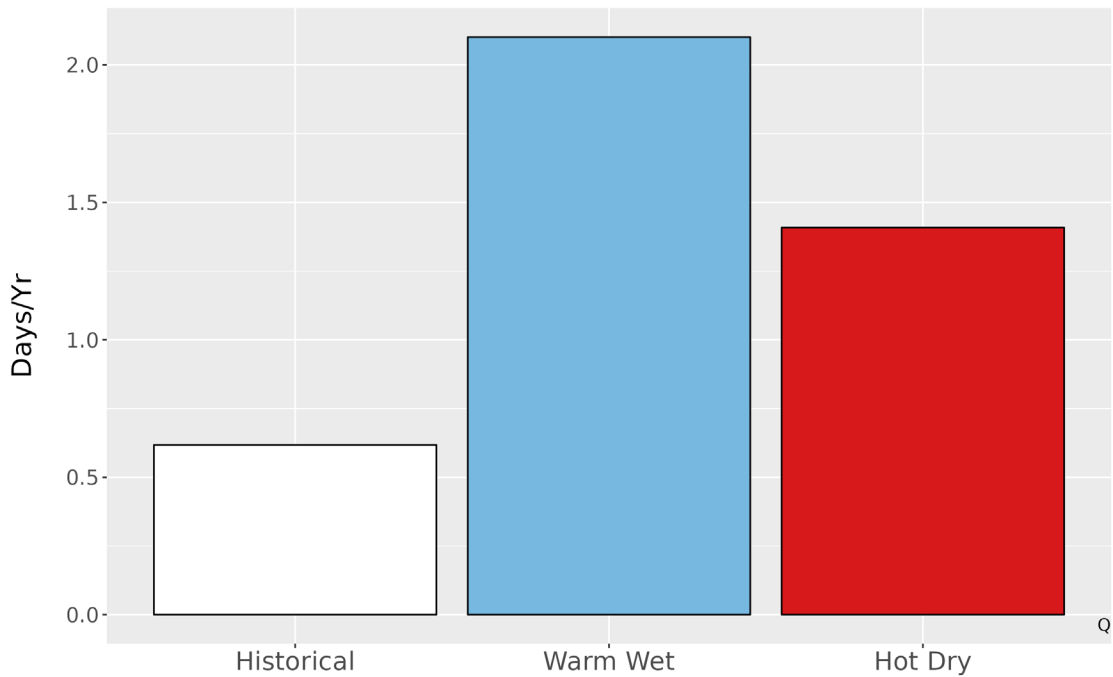
Figure 6. Average number of days annually with precipitation exceeding the 99th percentile (1.8 in.) of precipitation from the historical period 1979-2012 and for each climate future.
