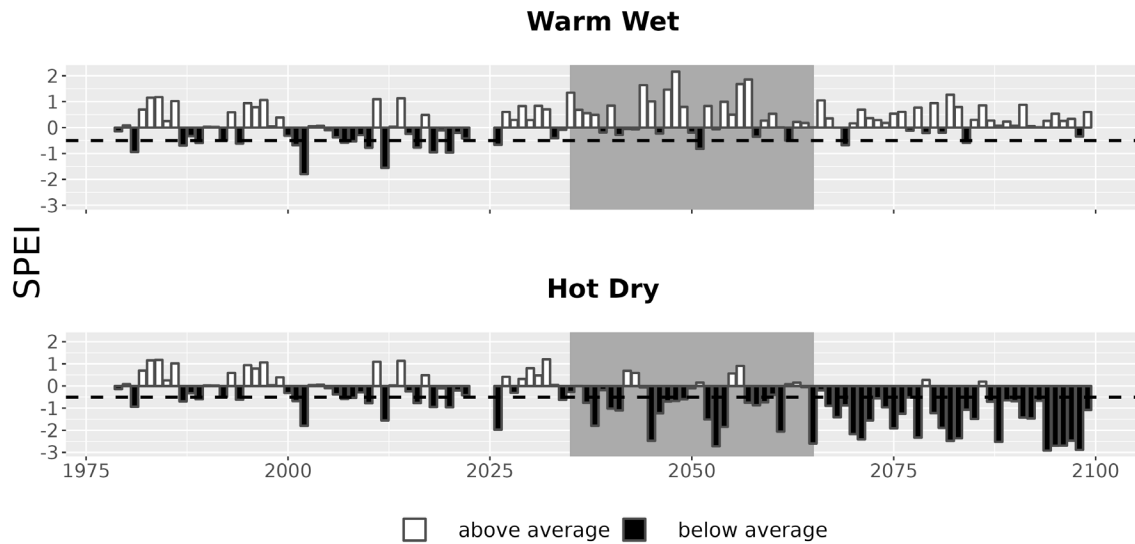
Figure 7. Drought metrics for ROMO. Drought index (SPEI; units = standard deviations from historical) timeseries for each climate future. Below-average SPEI (black bars) indicates dry conditions. The dotted line (SPEI = -0.5) indicates drought conditions.
