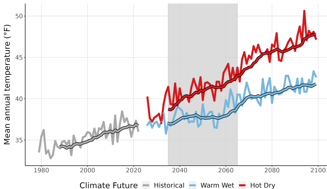
Figure 3. This graph compares observed average annual temperature at ROMO (°F) (1979-2022) with projected average annual temperature for the two climate futures over the period 2023-2099. The historically observed data is shown in gray, the Warm Wet climate future in blue, and the Hot Dry climate future in red. The smooth line running through each projection is the 10-year running average for historical observations and future projections. Gray-shaded area represents the time period that was averaged (2035-2065) to summarize future projections for the year 2050 (Appendix 1).
