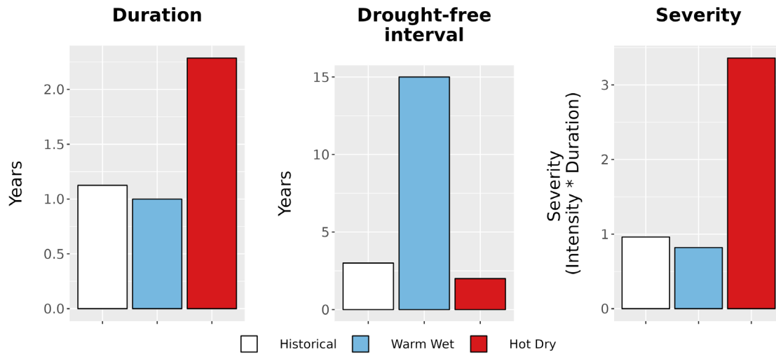
Figure 8. Drought metrics for ROMO. (Left) Average drought duration (years) historically (1979-2012) and under each climate future. (Middle) Average drought return interval (years), indicating the expected amount of time between periods of drought, historically and under each climate future. (Right) Average drought severity, a measure of drought intensity multiplied by duration, historically and under each climate future.
