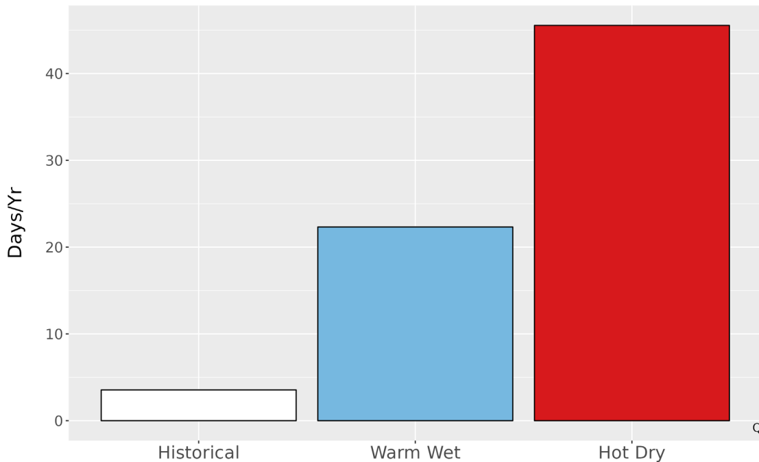
Figure 5. Metrics of extreme temperature at ROMO. The bar graph represents the average number of days annually with temperatures greater than the historical 99th percentile (74.9 °F) historically (1979-2012) and for the two climate futures (2050).
