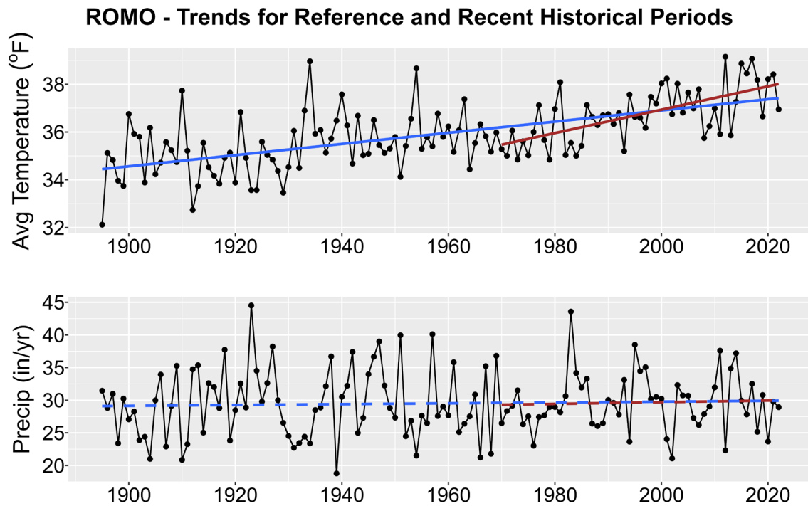
Figure 1. Historical trends in annual average temperature (upper plot) and annual total precipitation (lower plot) for ROMO from 1895-2022. Black points show yearly values while blue lines are linear regressions for the entire period record and red lines for 1970-2022 trends. Solid lines are significant trends (i.e., p < 0.05 ); dashed lines are not statistically significant.
