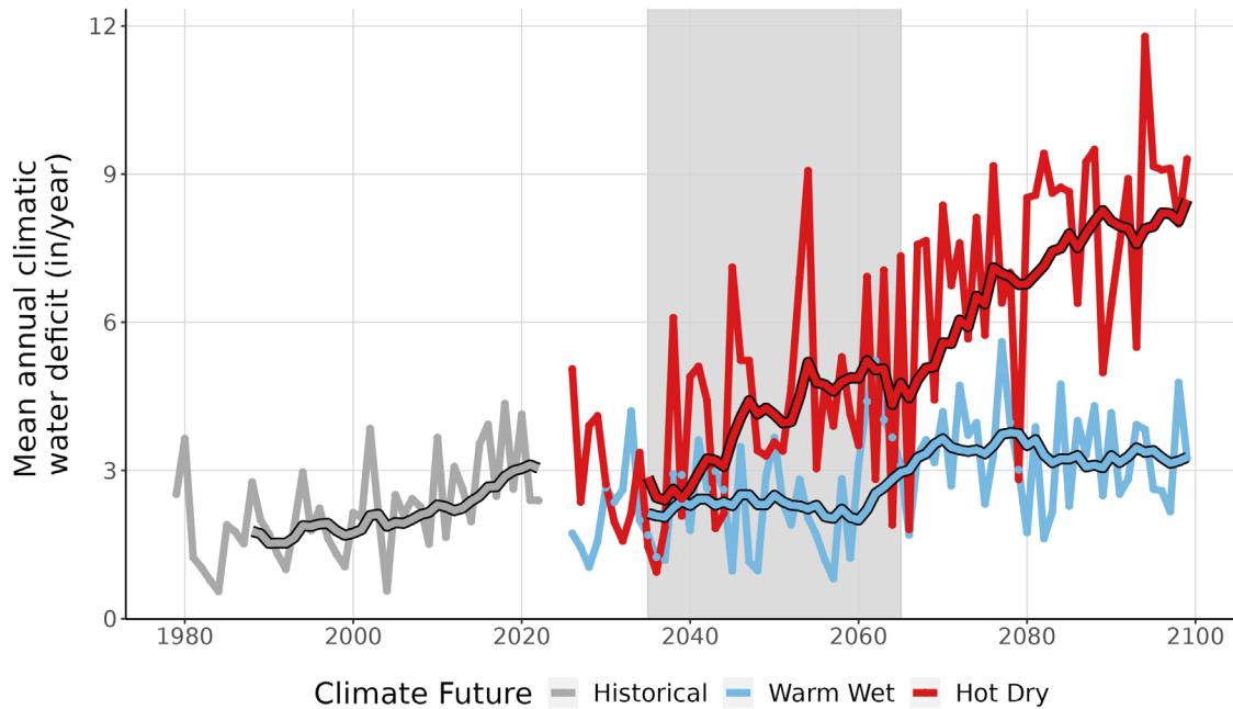
Figure 9. This line graph compares observed climatic water deficit at ROMO (inches/year) (1979-2022) with projected climatic water deficit for the two climate futures over the period 2023-2099. The historical observation data is shown in gray, the Warm Wet climate future in blue, and the Hot Dry climate future in red. The smooth line running through each projection is the 10-year running average for historical observations and future projections. Gray-shaded area represents the time period that was averaged (2035-2065) to summarize future projections for the year 2050.
