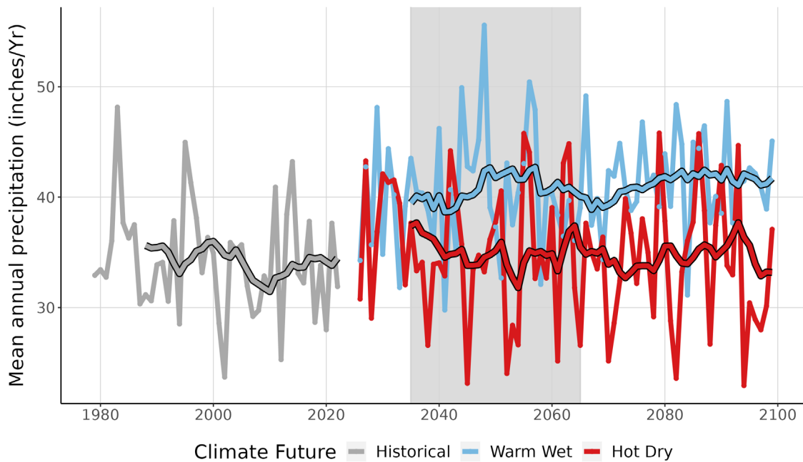
Figure 4. This graph compares observed average annual precipitation at ROMO (inches/year) (1979-2022) with projected average annual precipitation for the two climate futures over the period 2023-2099. The historically observed data is shown in gray, the Warm Wet climate future in blue, and the Hot Dry climate future in red. The smooth line running through each projection is the 10-year running average for historical observations and future projections. The gray-shaded area represents the time period that was averaged (2035-2065) to summarize future projections for the year 2050 (Appendix 1).
