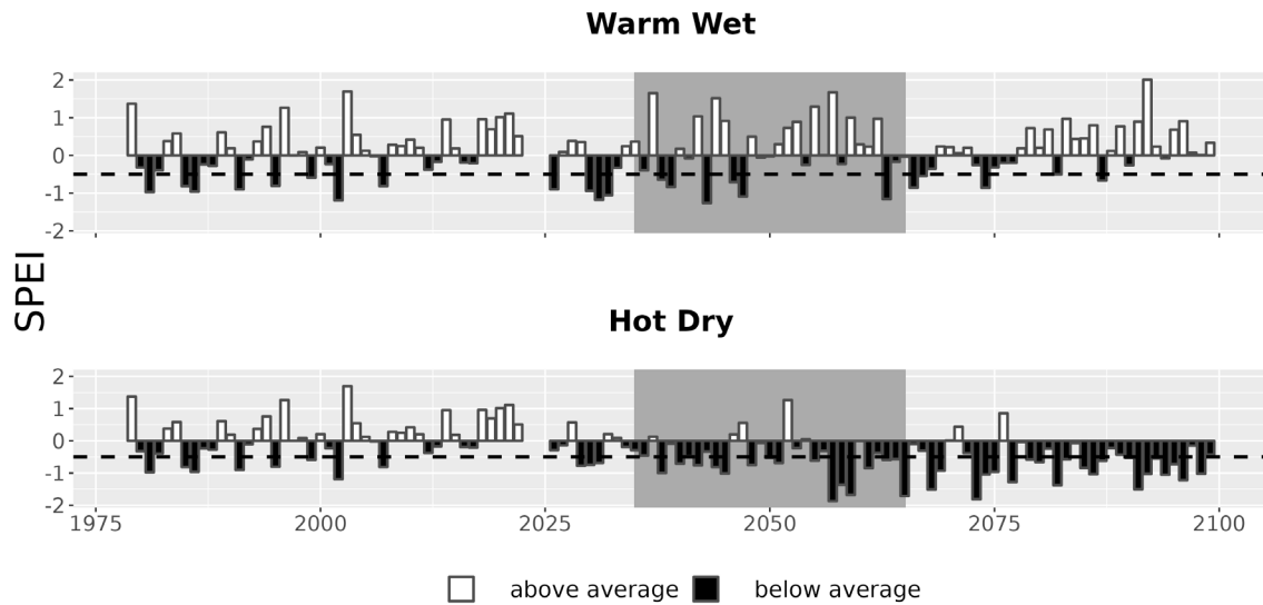
Figure 7. Drought metrics for ROCR. Drought index (SPEI; units = standard deviations from historical) timeseries for each climate future. Below-average SPEI (black bars) indicates dry conditions. The dotted line (SPEI = -0.5) indicates drought conditions.
