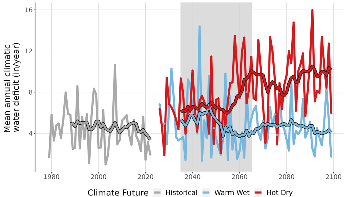
Figure 9. This line graph compares observed climatic water deficit at ROCR (inches/year) (1979-2022) with projected climatic water deficit for the two climate futures over the period 2023-2099. The historical observation data is shown in gray, the Warm Wet climate future in blue, and the Hot Dry climate future in red. The smooth line running through each projection is the 10-year running average for historical observations and future projections. Gray-shaded area represents the time period that was averaged (2035-2065) to summarize future projections for the year 2050.
