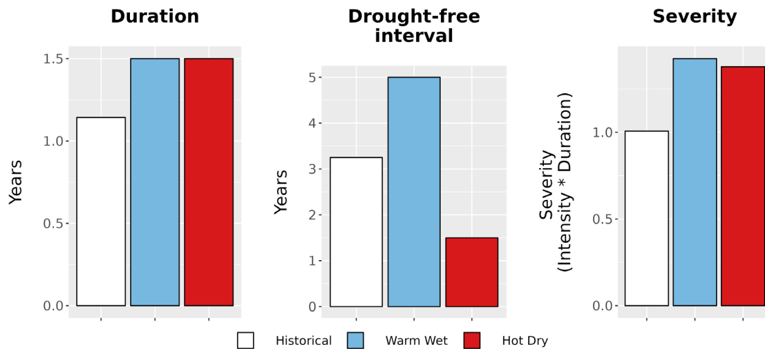
Figure 8. Drought metrics for ROCR. (Left) Average drought duration (years) historically (1979-2012) and under each climate future. (Middle) Average drought return interval (years), indicating the expected amount of time between periods of drought, historically and under each climate future. (Right) Average drought severity, a measure of drought intensity multiplied by duration, historically and under each climate future.
