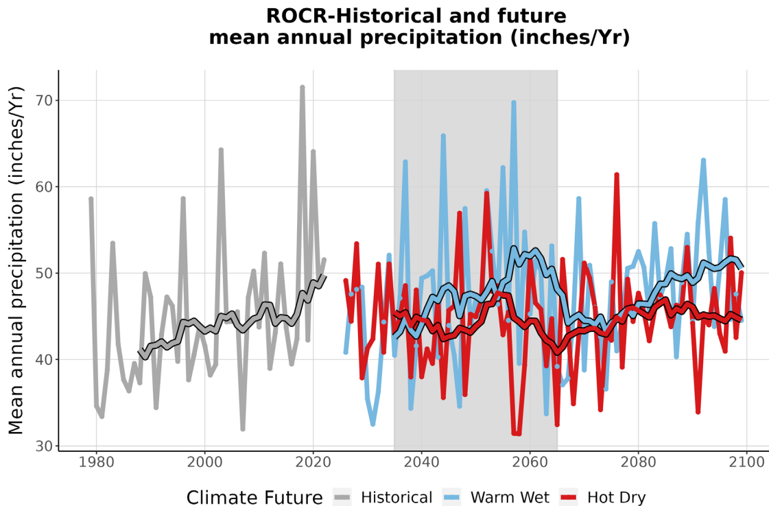
Figure 4. This graph compares observed average annual precipitation at ROCR (inches/year) (1979-2022) with projected average annual precipitation for the two climate futures over the period 2023-2099. The historically observed data is shown in gray, the Warm Wet climate future in blue, and the Hot Dry climate future in red. The smooth line running through each projection is the 10-year running average for historical observations and future projections. The gray-shaded area represents the time period that was averaged (2035-2065) to summarize future projections for the year 2050 (Appendix 1).
