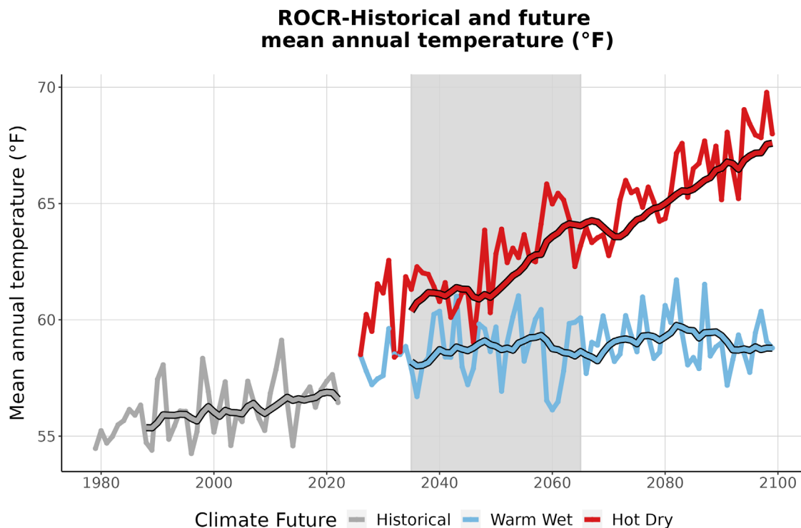
Figure 3. This graph compares observed average annual temperature at ROCR (°F) (1979-2022) with projected average annual temperature for the two climate futures over the period 2023-2099. The historically observed data
