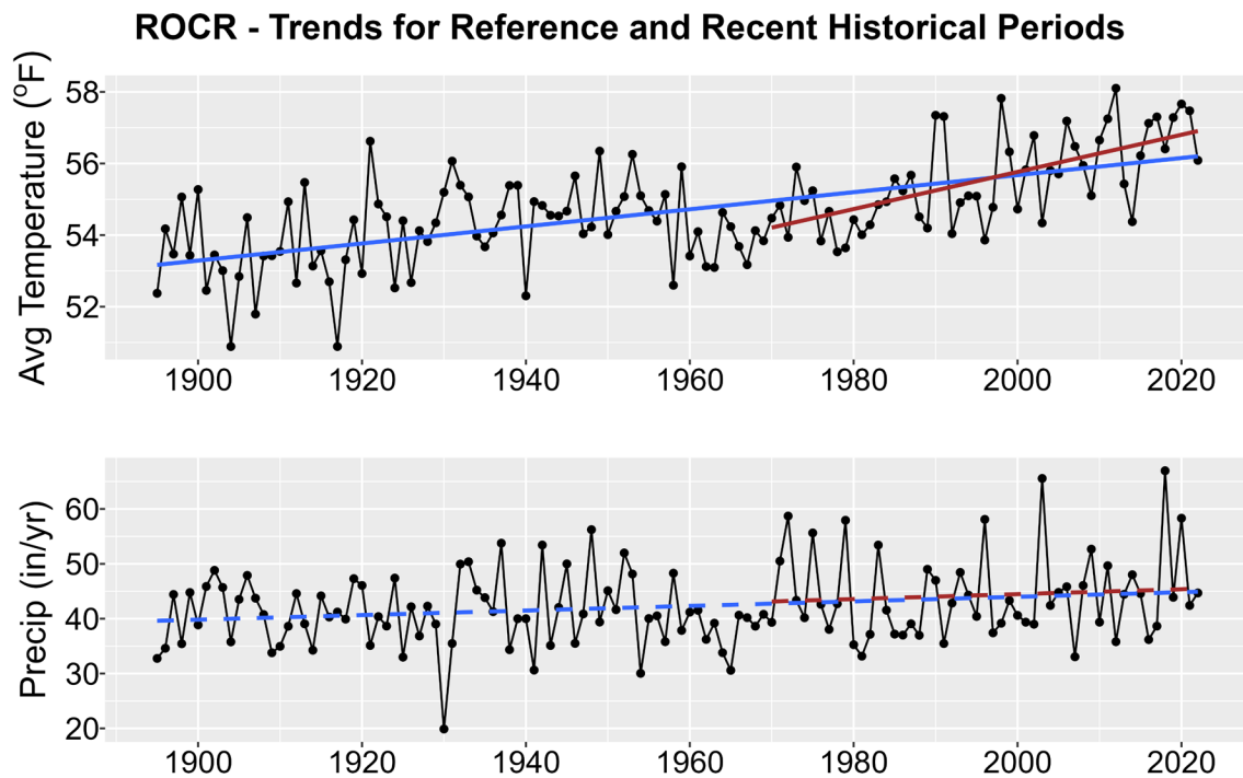
Figure 1. Historical trends in annual average temperature (upper plot) and annual total precipitation (lower plot) for ROCR from 1895-2022. Black points show yearly values while blue lines are linear regressions for the entire period record and red lines for 1970-2022 trends. Solid lines are significant trends (i.e., p < 0.05 ); dashed lines are not statistically significant.
