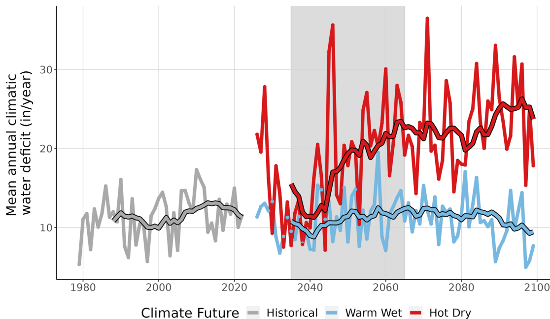
Figure 9. This line graph compares observed climatic water deficit at REER (inches/year) (1979-2022) with projected climatic water deficit for the two climate futures over the period 2023-2099. The historical observation data is shown in gray, the Warm Wet climate future in blue, and the Hot Dry climate future in red. The smooth line running through each projection is the 10-year running average for historical observations and future projections. Gray-shaded area represents the time period that was averaged (2035-2065) to summarize future projections for the year 2050.
