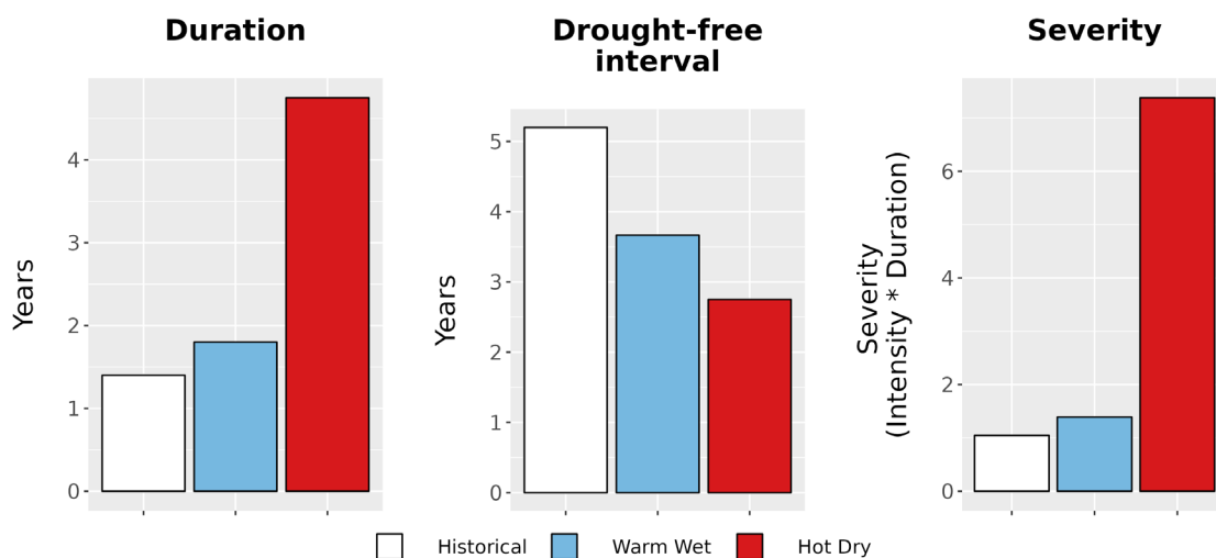
Figure 8. Drought metrics for REER. (Left) Average drought duration (years) historically (1979-2012) and under each climate future. (Middle) Average drought return interval (years), indicating the expected amount of time between periods of drought, historically and under each climate future. (Right) Average drought severity, a measure of drought intensity multiplied by duration, historically and under each climate future.
