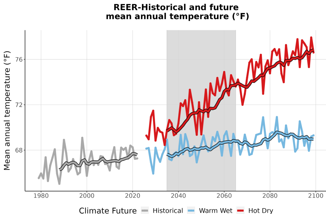
Figure 3. This graph compares observed average annual temperature at REER (°F) (1979-2022) with projected average annual temperature for the two climate futures over the period 2023-2099. The historically observed data
