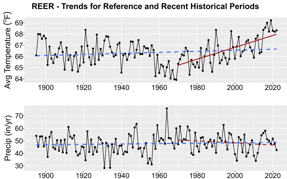
Figure 1. Historical trends in annual average temperature (upper plot) and annual total precipitation (lower plot) for REER from 1895-2022. Black points show yearly values while blue lines are linear regressions for the entire period record and red lines for 1970-2022 trends. Solid lines are significant trends (i.e., p < 0.05 ); dashed lines are not statistically significant.
