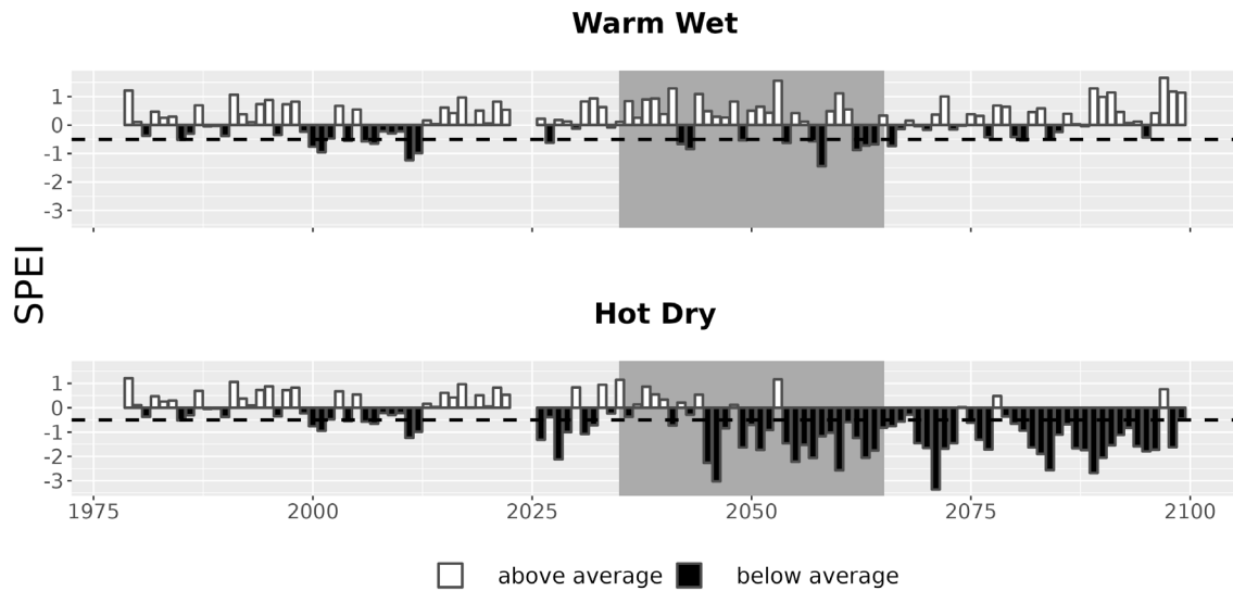
Figure 7. Drought metrics for REER. Drought index (SPEI; units = standard deviations from historical) timeseries for each climate future. Below-average SPEI (black bars) indicates dry conditions. The dotted line (SPEI = -0.5) indicates drought conditions.
