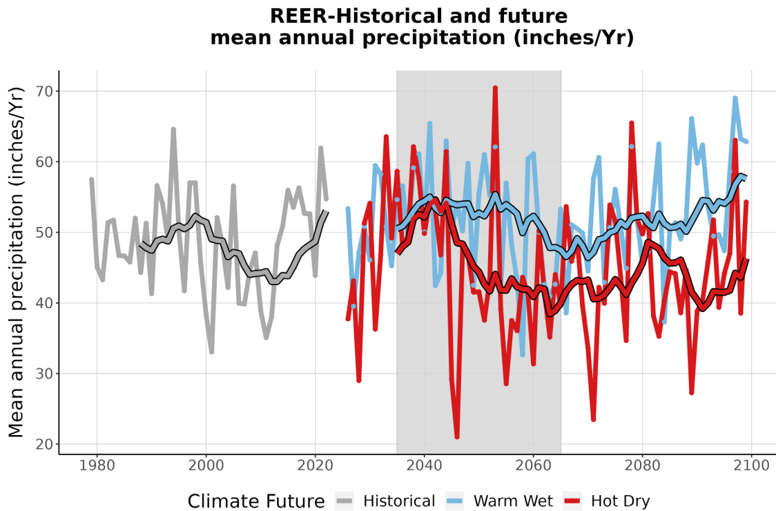
Figure 4. This graph compares observed average annual precipitation at REER (inches/year) (1979-2022) with projected average annual precipitation for the two climate futures over the period 2023-2099. The historically observed data is shown in gray, the Warm Wet climate future in blue, and the Hot Dry climate future in red. The smooth line running through each projection is the 10-year running average for historical observations and future projections. The gray-shaded area represents the time period that was averaged (2035-2065) to summarize future projections for the year 2050 (Appendix 1).
