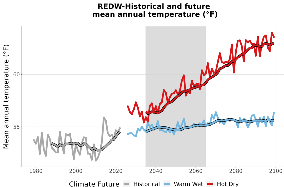
Figure 3. This graph compares observed average annual temperature at REDW (°F) (1979-2022) with projected average annual temperature for the two climate futures over the period 2023-2099. The historically observed data
