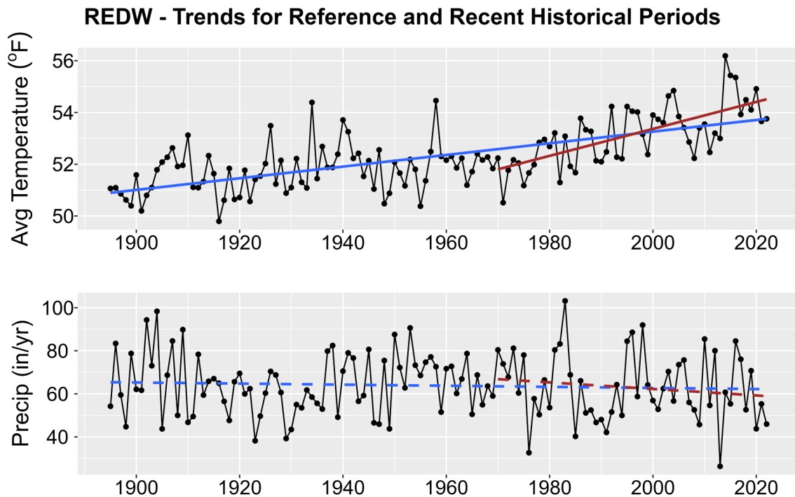
Figure 1. Historical trends in annual average temperature (upper plot) and annual total precipitation (lower plot) for REDW from 1895-2022. Black points show yearly values while blue lines are linear regressions for the entire period record and red lines for 1970-2022 trends. Solid lines are significant trends (i.e., p < 0.05 ); dashed lines are not statistically significant.
