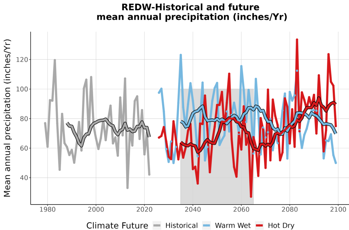
Figure 4. This graph compares observed average annual precipitation at REDW (inches/year) (1979-2022) with projected average annual precipitation for the two climate futures over the period 2023-2099. The historically observed data is shown in gray, the Warm Wet climate future in blue, and the Hot Dry climate future in red. The smooth line running through each projection is the 10-year running average for historical observations and future projections. The gray-shaded area represents the time period that was averaged (2035-2065) to summarize future projections for the year 2050 (Appendix 1).
