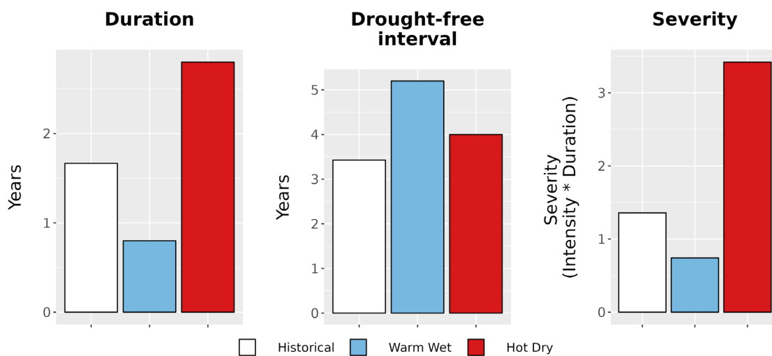
Figure 8. Drought metrics for REDW. (Left) Average drought duration (years) historically (1979-2012) and under each climate future. (Middle) Average drought return interval (years), indicating the expected amount of time between periods of drought, historically and under each climate future. (Right) Average drought severity, a measure of drought intensity multiplied by duration, historically and under each climate future.
