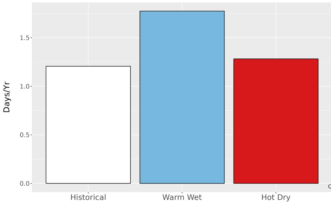
Figure 6. Average number of days annually with precipitation exceeding the 99th percentile (3 in.) of precipitation from the historical period 1979-2012 and for each climate future.
