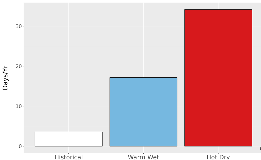
Figure 5. Metrics of extreme temperature at REDW. The bar graph represents the average number of days annually with temperatures greater than the historical 99th percentile (78.7 °F) historically (1979-2012) and for the two climate futures (2050).
