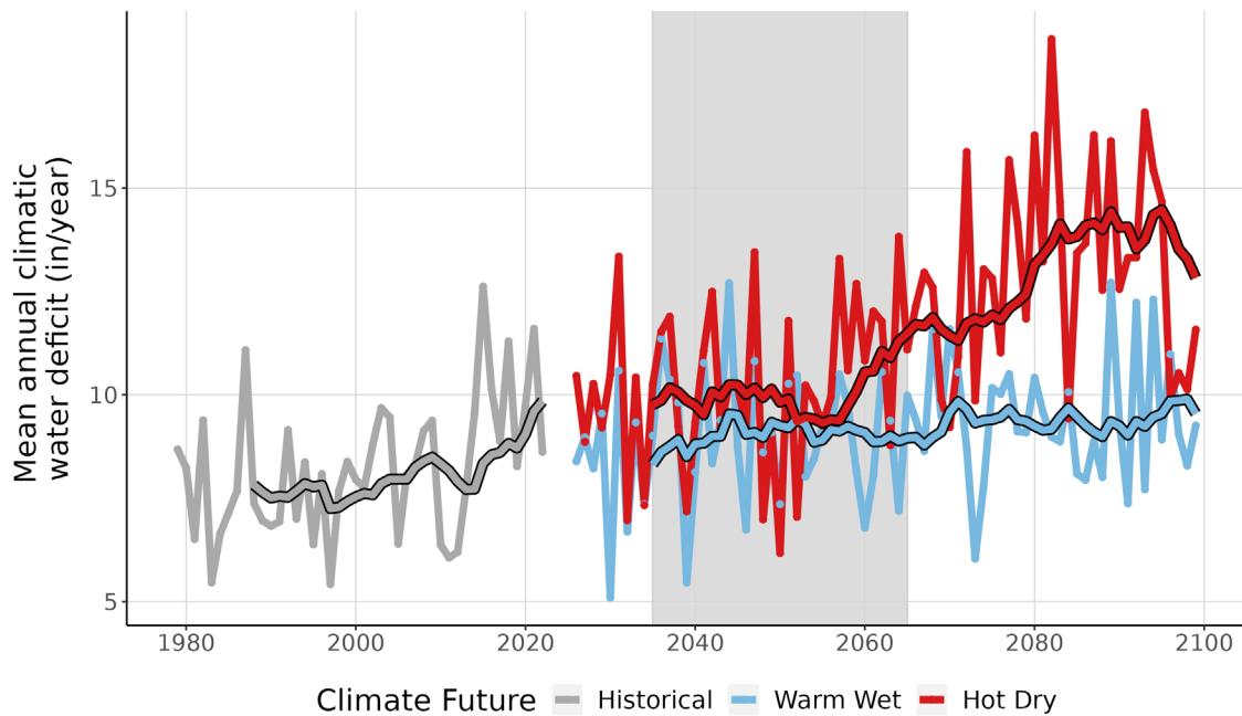
Figure 9. This line graph compares observed climatic water deficit at REDW (inches/year) (1979-2022) with projected climatic water deficit for the two climate futures over the period 2023-2099. The historical observation data is shown in gray, the Warm Wet climate future in blue, and the Hot Dry climate future in red. The smooth line running through each projection is the 10-year running average for historical observations and future projections. Gray-shaded area represents the time period that was averaged (2035-2065) to summarize future projections for the year 2050.
