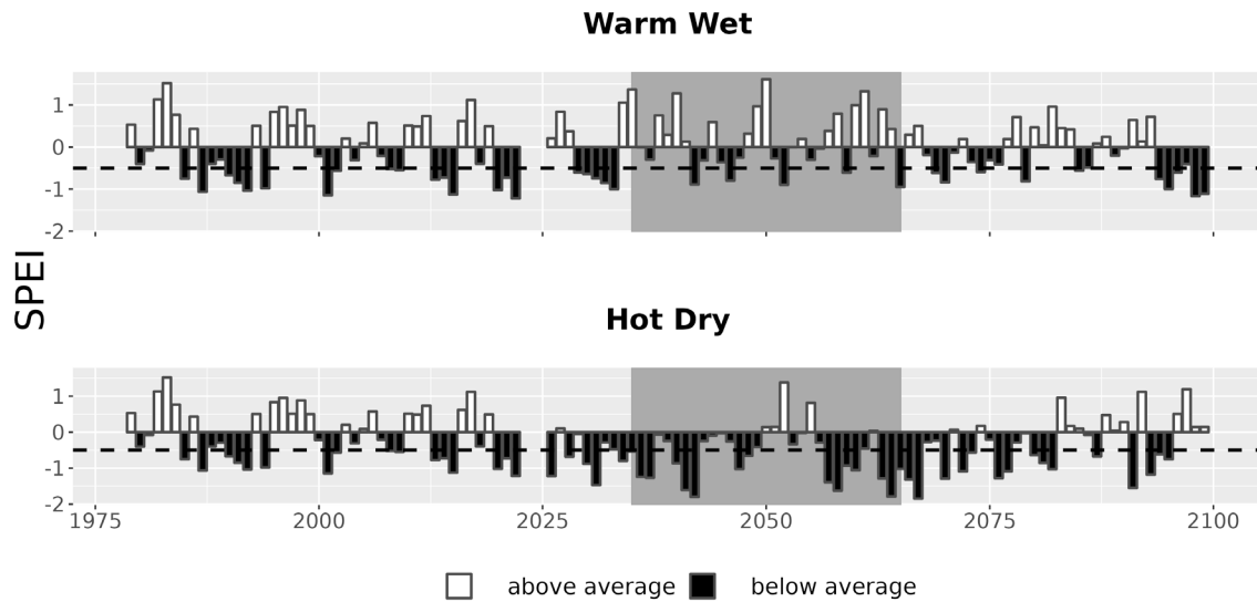
Figure 7. Drought metrics for REDW. Drought index (SPEI; units = standard deviations from historical) timeseries for each climate future. Below-average SPEI (black bars) indicates dry conditions. The dotted line (SPEI = -0.5) indicates drought conditions.
