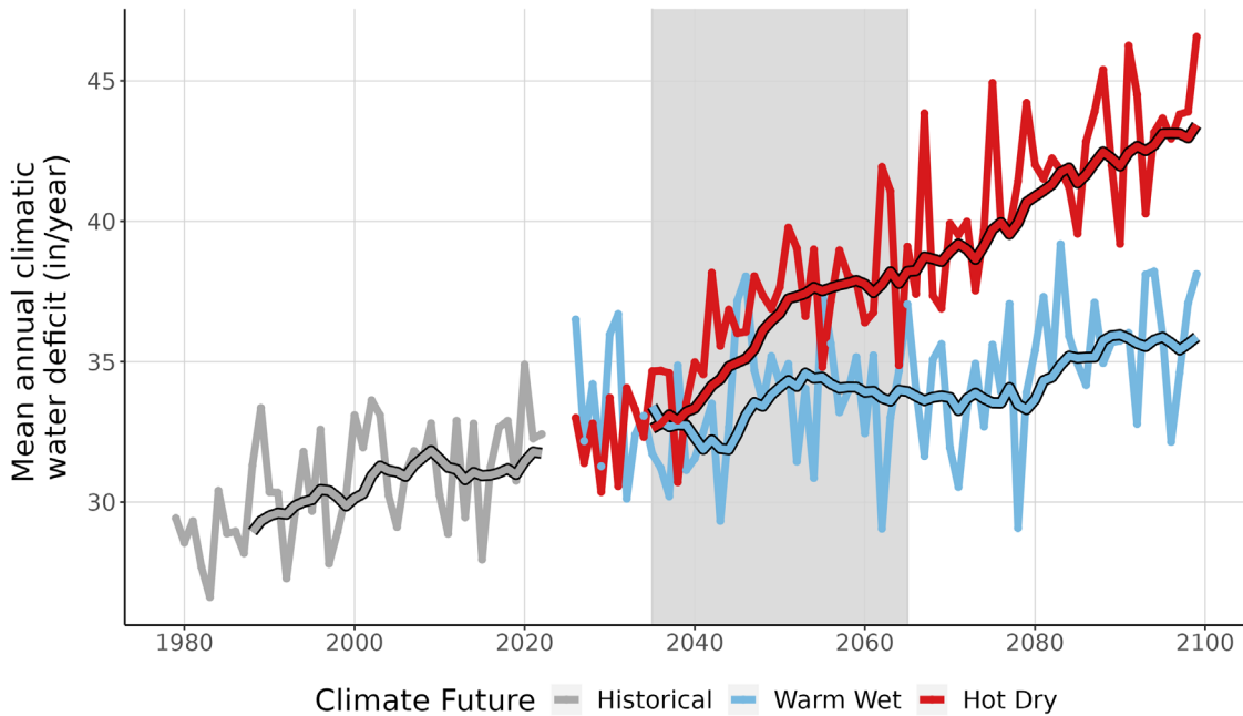
Figure 9. This line graph compares observed climatic water deficit at RABR (inches/year) (1979-2022) with projected climatic water deficit for the two climate futures over the period 2023-2099. The historical observation data is shown in gray, the Warm Wet climate future in blue, and the Hot Dry climate future in red. The smooth line running through each projection is the 10-year running average for historical observations and future projections. Gray-shaded area represents the time period that was averaged (2035-2065) to summarize future projections for the year 2050.
