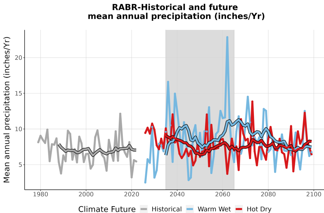
Figure 4. This graph compares observed average annual precipitation at RABR (inches/year) (1979-2022) with projected average annual precipitation for the two climate futures over the period 2023-2099. The historically observed data is shown in gray, the Warm Wet climate future in blue, and the Hot Dry climate future in red. The smooth line running through each projection is the 10-year running average for historical observations and future projections. The gray-shaded area represents the time period that was averaged (2035-2065) to summarize future projections for the year 2050 (Appendix 1).
