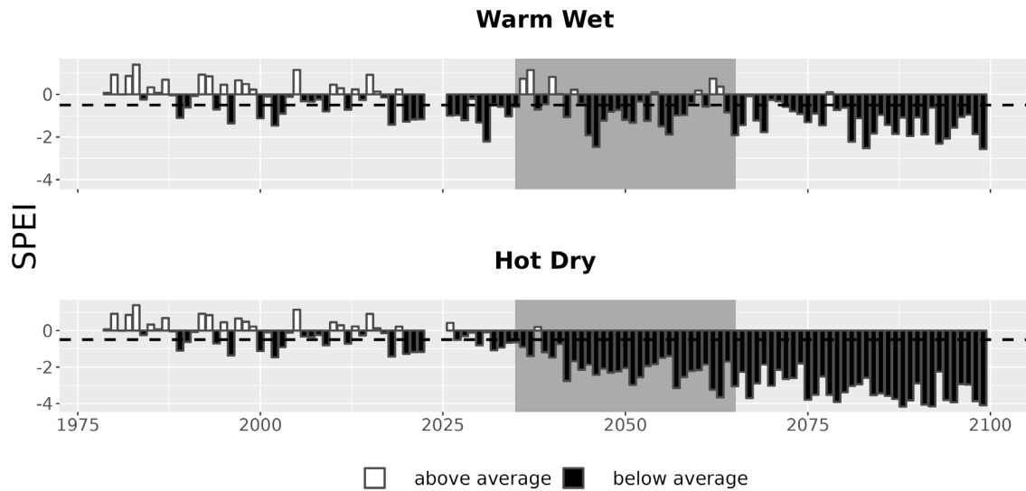
Figure 7. Drought metrics for RABR. Drought index (SPEI; units = standard deviations from historical) timeseries for each climate future. Below-average SPEI (black bars) indicates dry conditions. The dotted line (SPEI = -0.5) indicates drought conditions.
