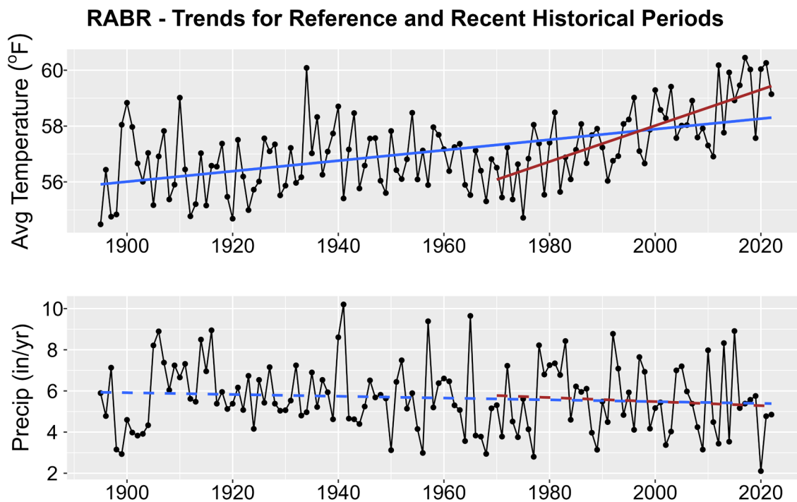
Figure 1. Historical trends in annual average temperature (upper plot) and annual total precipitation (lower plot) for RABR from 1895-2022. Black points show yearly values while blue lines are linear regressions for the entire period record and red lines for 1970-2022 trends. Solid lines are significant trends (i.e., p < 0.05 ); dashed lines are not statistically significant.
