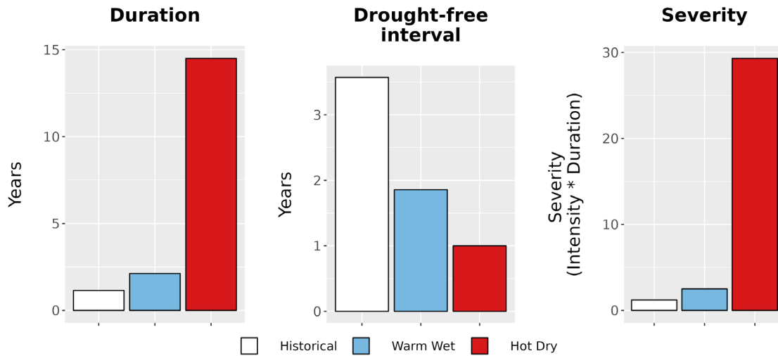
Figure 8. Drought metrics for RABR. (Left) Average drought duration (years) historically (1979-2012) and under each climate future. (Middle) Average drought return interval (years), indicating the expected amount of time between periods of drought, historically and under each climate future. (Right) Average drought severity, a measure of drought intensity multiplied by duration, historically and under each climate future.
