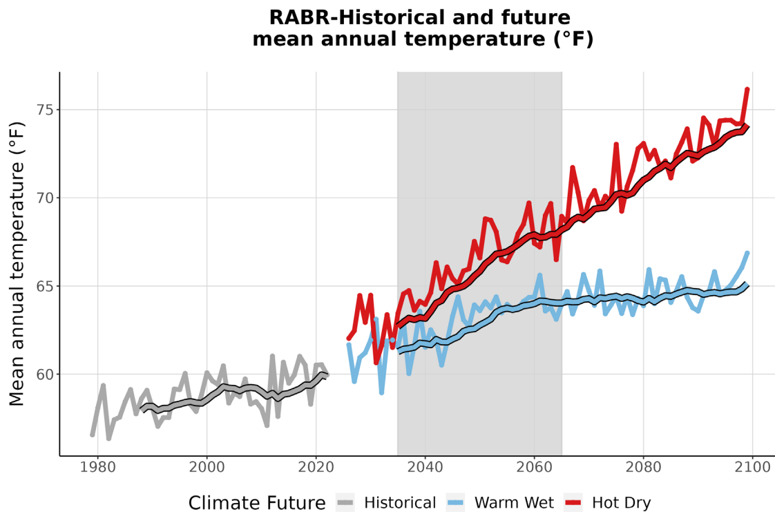
Figure 3. This graph compares observed average annual temperature at RABR (°F) (1979-2022) with projected average annual temperature for the two climate futures over the period 2023-2099. The historically observed data is shown in gray, the Warm Wet climate future in blue, and the Hot Dry climate future in red. The smooth line
