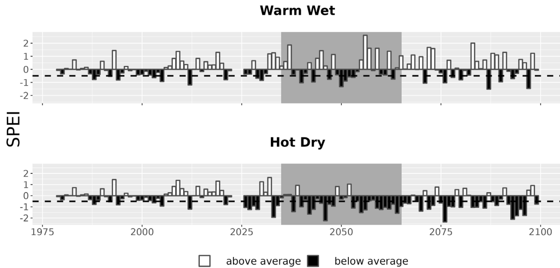
Figure 7. Drought metrics for PULL. Drought index (SPEI; units = standard deviations from historical) timeseries for each climate future. Below-average SPEI (black bars) indicates dry conditions. The dotted line (SPEI = -0.5) indicates drought conditions.
