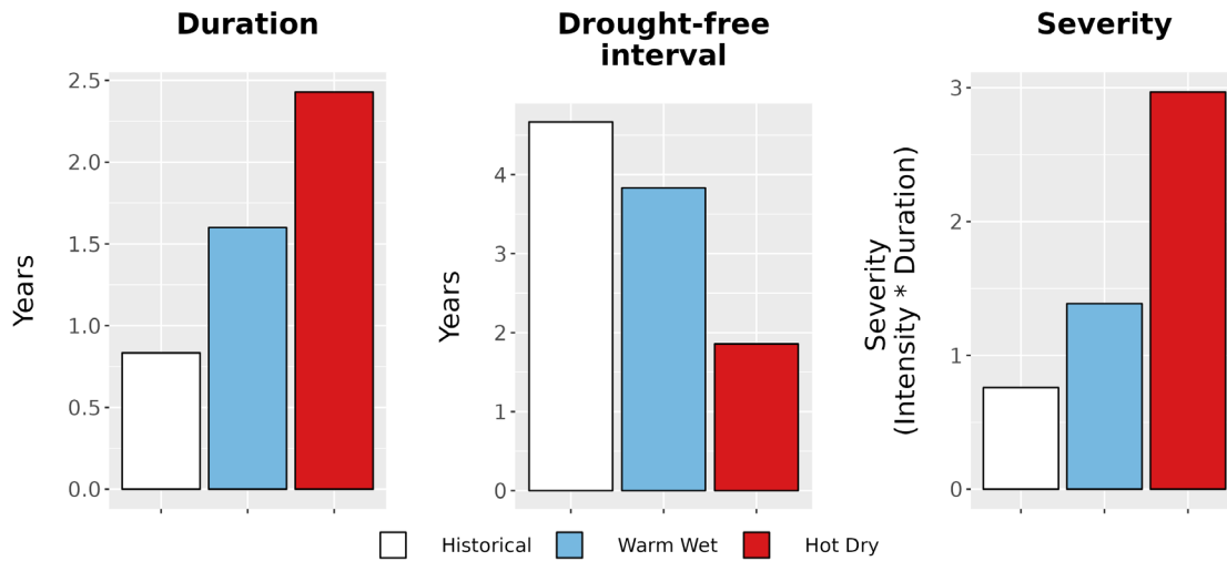
Figure 8. Drought metrics for PULL. (Left) Average drought duration (years) historically (1979-2012) and under each climate future. (Middle) Average drought return interval (years), indicating the expected amount of time between periods of drought, historically and under each climate future. (Right) Average drought severity, a measure of drought intensity multiplied by duration, historically and under each climate future.
