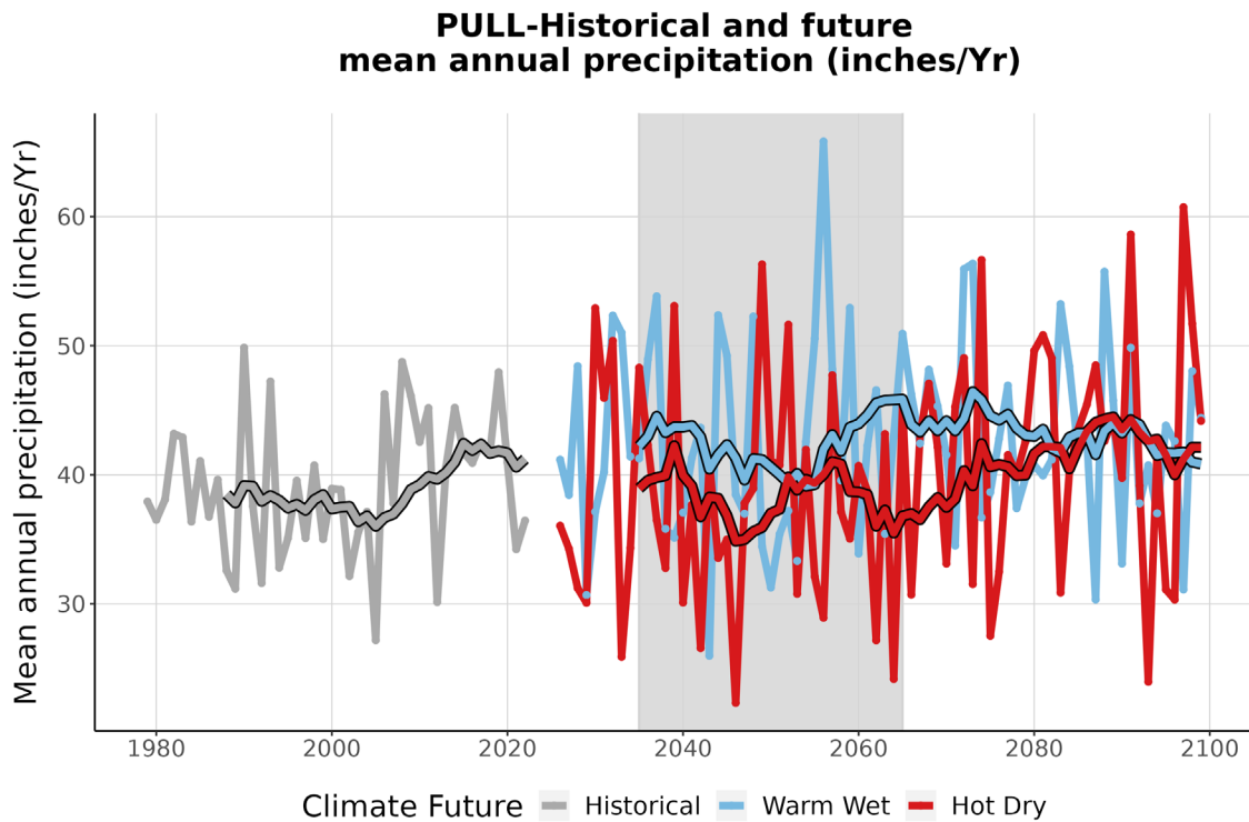
Figure 4. This graph compares observed average annual precipitation at PULL (inches/year) (1979-2022) with projected average annual precipitation for the two climate futures over the period 2023-2099. The historically observed data is shown in gray, the Warm Wet climate future in blue, and the Hot Dry climate future in red. The smooth line running through each projection is the 10-year running average for historical observations and future projections. The gray-shaded area represents the time period that was averaged (2035-2065) to summarize future projections for the year 2050 (Appendix 1).
