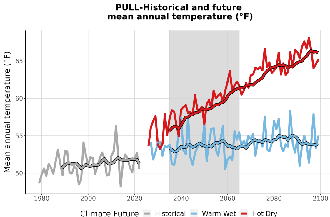
Figure 3. This graph compares observed average annual temperature at PULL (°F) (1979-2022) with projected average annual temperature for the two climate futures over the period 2023-2099. The historically observed data
