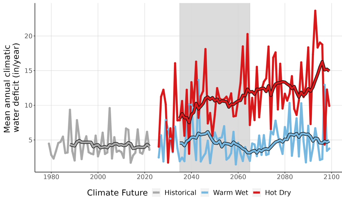
Figure 9. This line graph compares observed climatic water deficit at PULL (inches/year) (1979-2022) with projected climatic water deficit for the two climate futures over the period 2023-2099. The historical observation data is shown in gray, the Warm Wet climate future in blue, and the Hot Dry climate future in red. The smooth line running through each projection is the 10-year running average for historical observations and future projections. Gray-shaded area represents the time period that was averaged (2035-2065) to summarize future projections for the year 2050.
