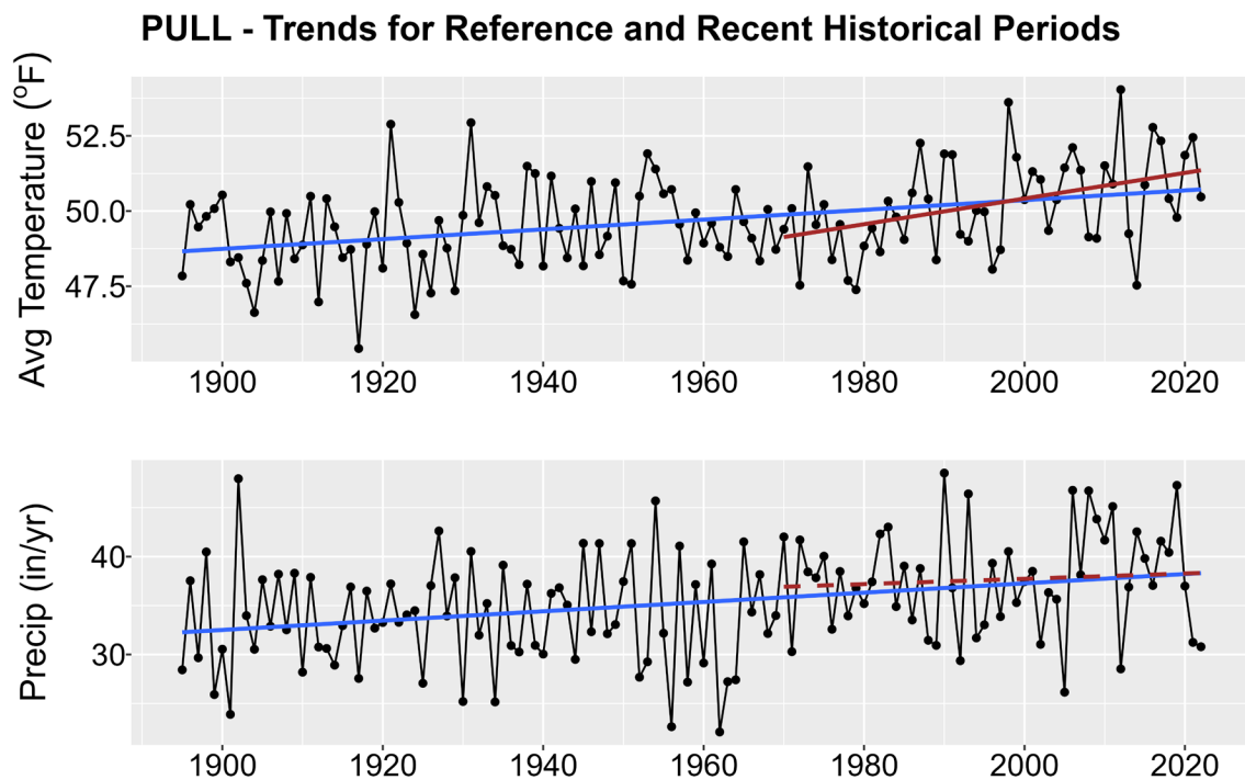
Figure 1. Historical trends in annual average temperature (upper plot) and annual total precipitation (lower plot) for PULL from 1895-2022. Black points show yearly values while blue lines are linear regressions for the entire period record and red lines for 1970-2022 trends. Solid lines are significant trends (i.e., p < 0.05 ); dashed lines are not statistically significant.
