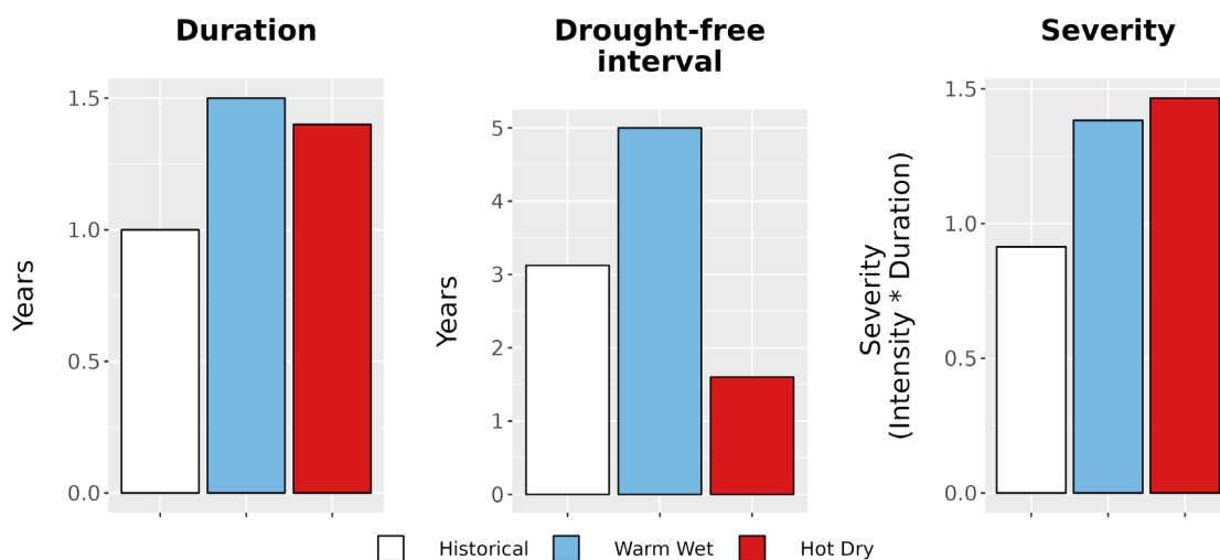
Figure 8. Drought metrics for PRWI. (Left) Average drought duration (years) historically (1979-2012) and under each climate future. (Middle) Average drought return interval (years), indicating the expected amount of time between periods of drought, historically and under each climate future. (Right) Average drought severity, a measure of drought intensity multiplied by duration, historically and under each climate future.
