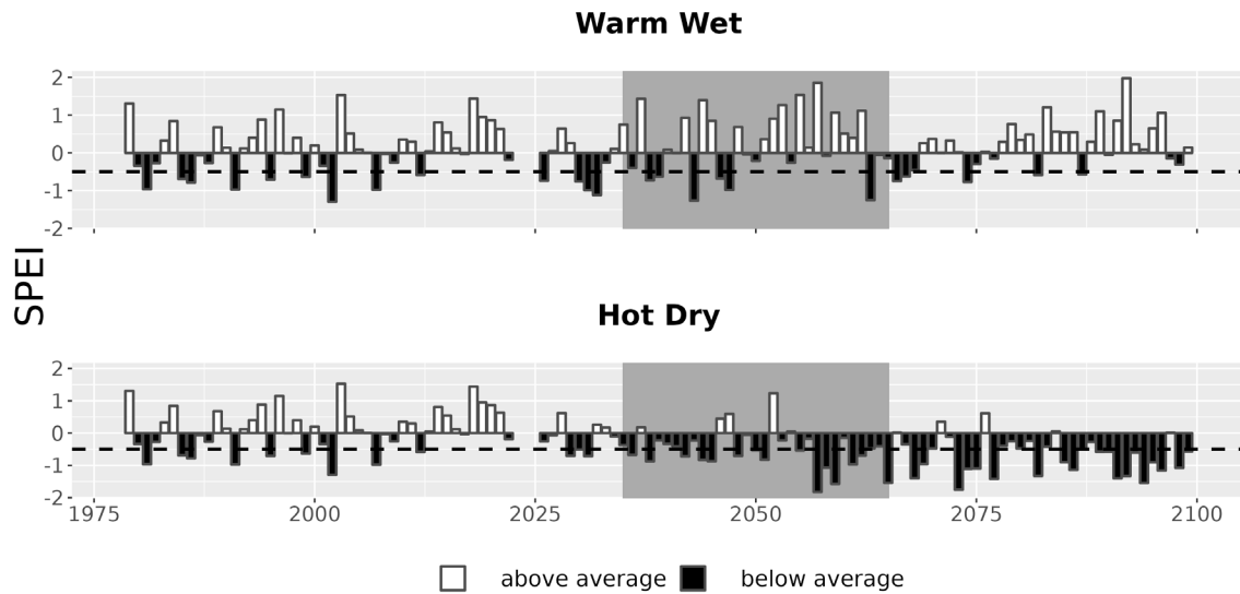
Figure 7. Drought metrics for PRWI. Drought index (SPEI; units = standard deviations from historical) timeseries for each climate future. Below-average SPEI (black bars) indicates dry conditions. The dotted line (SPEI = -0.5) indicates drought conditions.
