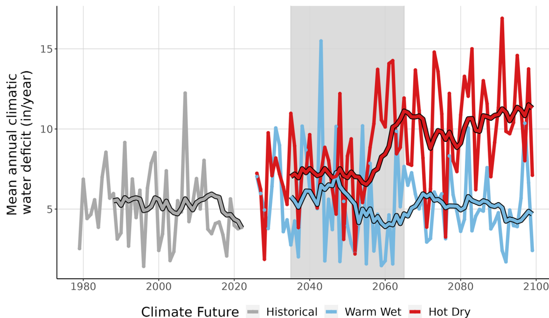
Figure 9. This line graph compares observed climatic water deficit at PRWI (inches/year) (1979-2022) with projected climatic water deficit for the two climate futures over the period 2023-2099. The historical observation data is shown in gray, the Warm Wet climate future in blue, and the Hot Dry climate future in red. The smooth line running through each projection is the 10-year running average for historical observations and future projections. Gray-shaded area represents the time period that was averaged (2035-2065) to summarize future projections for the year 2050.
