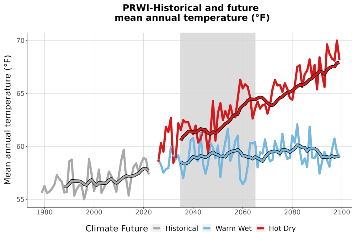
Figure 3. This graph compares observed average annual temperature at PRWI (°F) (1979-2022) with projected average annual temperature for the two climate futures over the period 2023-2099. The historically observed data
