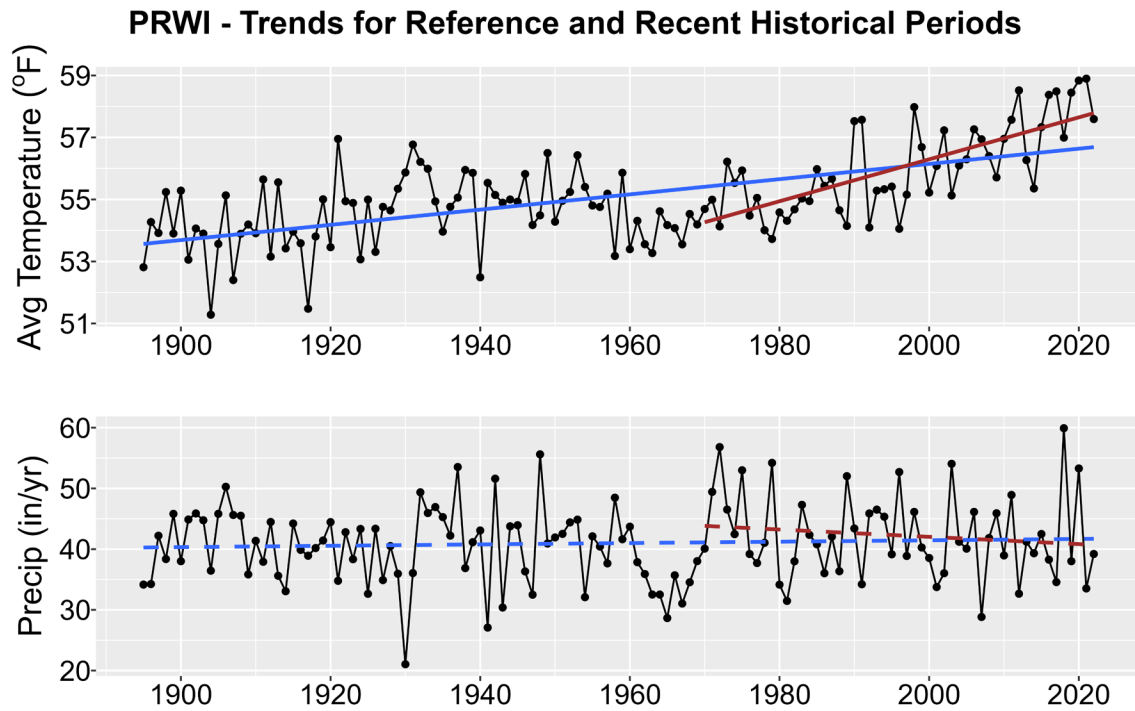
Figure 1. Historical trends in annual average temperature (upper plot) and annual total precipitation (lower plot) for PRWI from 1895-2022. Black points show yearly values while blue lines are linear regressions for the entire period record and red lines for 1970-2022 trends. Solid lines are significant trends (i.e., p < 0.05 ); dashed lines are not statistically significant.
