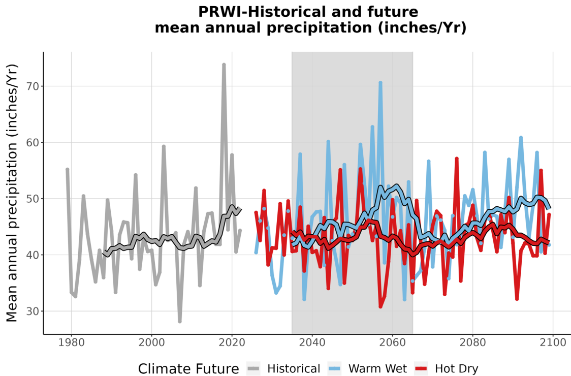
Figure 4. This graph compares observed average annual precipitation at PRWI (inches/year) (1979-2022) with projected average annual precipitation for the two climate futures over the period 2023-2099. The historically observed data is shown in gray, the Warm Wet climate future in blue, and the Hot Dry climate future in red. The smooth line running through each projection is the 10-year running average for historical observations and future projections. The gray-shaded area represents the time period that was averaged (2035-2065) to summarize future projections for the year 2050 (Appendix 1).
