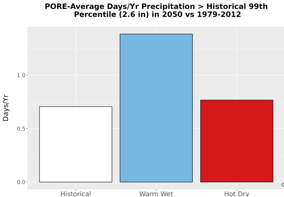
Figure 6. Average number of days annually with precipitation exceeding the 99th percentile (2.6 in.) of precipitation from the historical period 1979-2012 and for each climate future.
