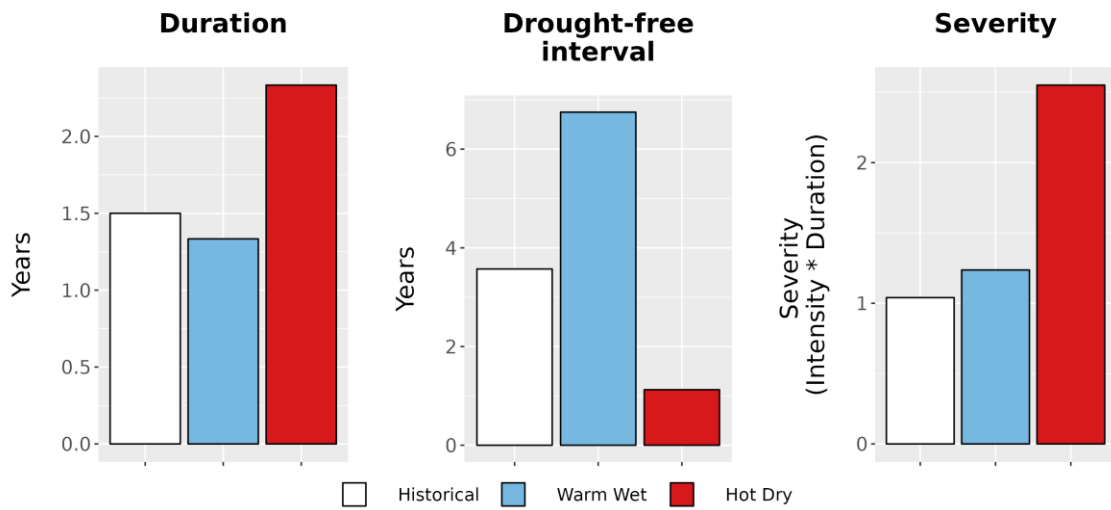
Figure 8. Drought metrics for PORE. (Left) Average drought duration (years) historically (1979-2012) and under each climate future. (Middle) Average drought return interval (years), indicating the expected amount of time between periods of drought, historically and under each climate future. (Right) Average drought severity, a measure of drought intensity multiplied by duration, historically and under each climate future.
