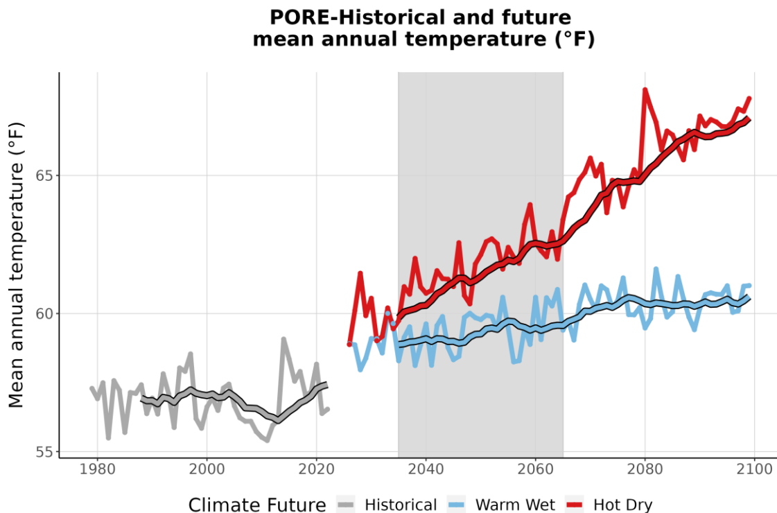
Figure 3. This graph compares observed average annual temperature at PORE (°F) (1979-2022) with projected average annual temperature for the two climate futures over the period 2023-2099. The historically observed data
