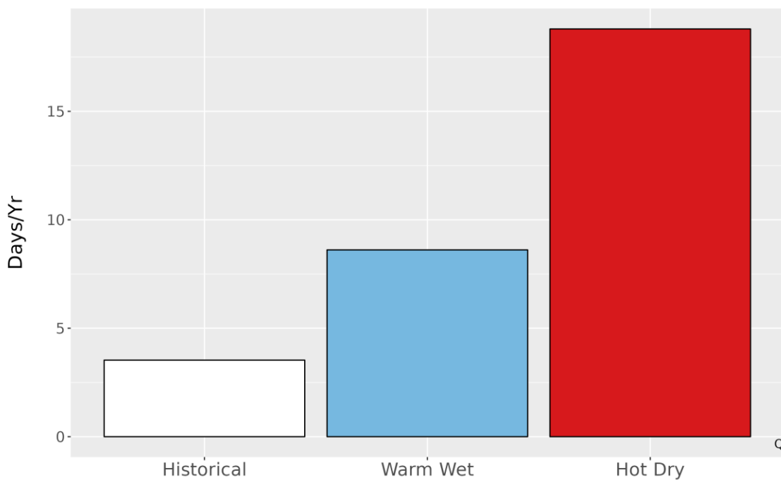
Figure 5. Metrics of extreme temperature at PORE. The bar graph represents the average number of days annually with temperatures greater than the historical 99th percentile (80.7 °F) historically (1979-2012) and for the two climate futures (2050).
