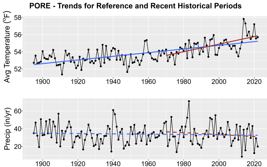
Figure 1. Historical trends in annual average temperature (upper plot) and annual total precipitation (lower plot) for PORE from 1895-2022. Black points show yearly values while blue lines are linear regressions for the entire period record and red lines for 1970-2022 trends. Solid lines are significant trends (i.e., p < 0.05 ); dashed lines are not statistically significant.
