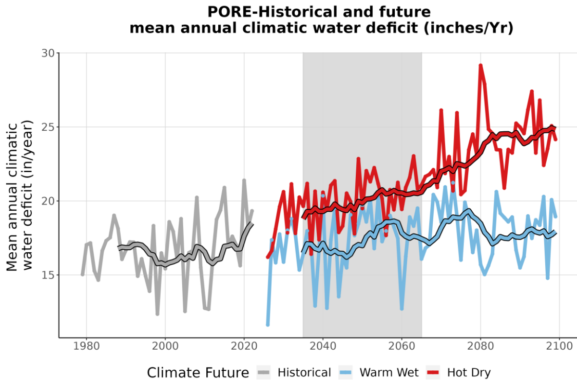
Figure 9. This line graph compares observed climatic water deficit at PORE (inches/year) (1979-2022) with projected climatic water deficit for the two climate futures over the period 2023-2099. The historical observation data is shown in gray, the Warm Wet climate future in blue, and the Hot Dry climate future in red. The smooth line running through each projection is the 10-year running average for historical observations and future projections. Gray-shaded area represents the time period that was averaged (2035-2065) to summarize future projections for the year 2050.
