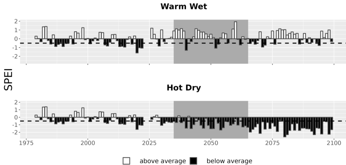
Figure 7. Drought metrics for PORE. Drought index (SPEI; units = standard deviations from historical) timeseries for each climate future. Below-average SPEI (black bars) indicates dry conditions. The dotted line (SPEI = -0.5) indicates drought conditions.
