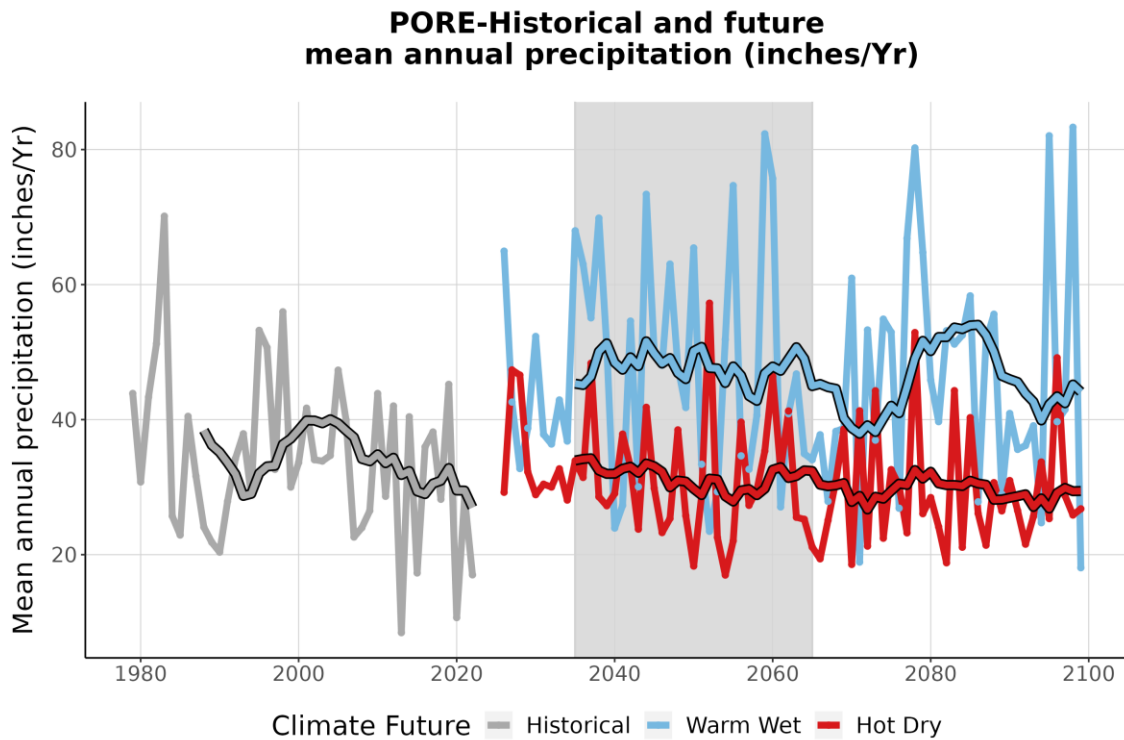
Figure 4. This graph compares observed average annual precipitation at PORE (inches/year) (1979-2022) with projected average annual precipitation for the two climate futures over the period 2023-2099. The historically observed data is shown in gray, the Warm Wet climate future in blue, and the Hot Dry climate future in red. The smooth line running through each projection is the 10-year running average for historical observations and future projections. The gray-shaded area represents the time period that was averaged (2035-2065) to summarize future projections for the year 2050 (Appendix 1).
