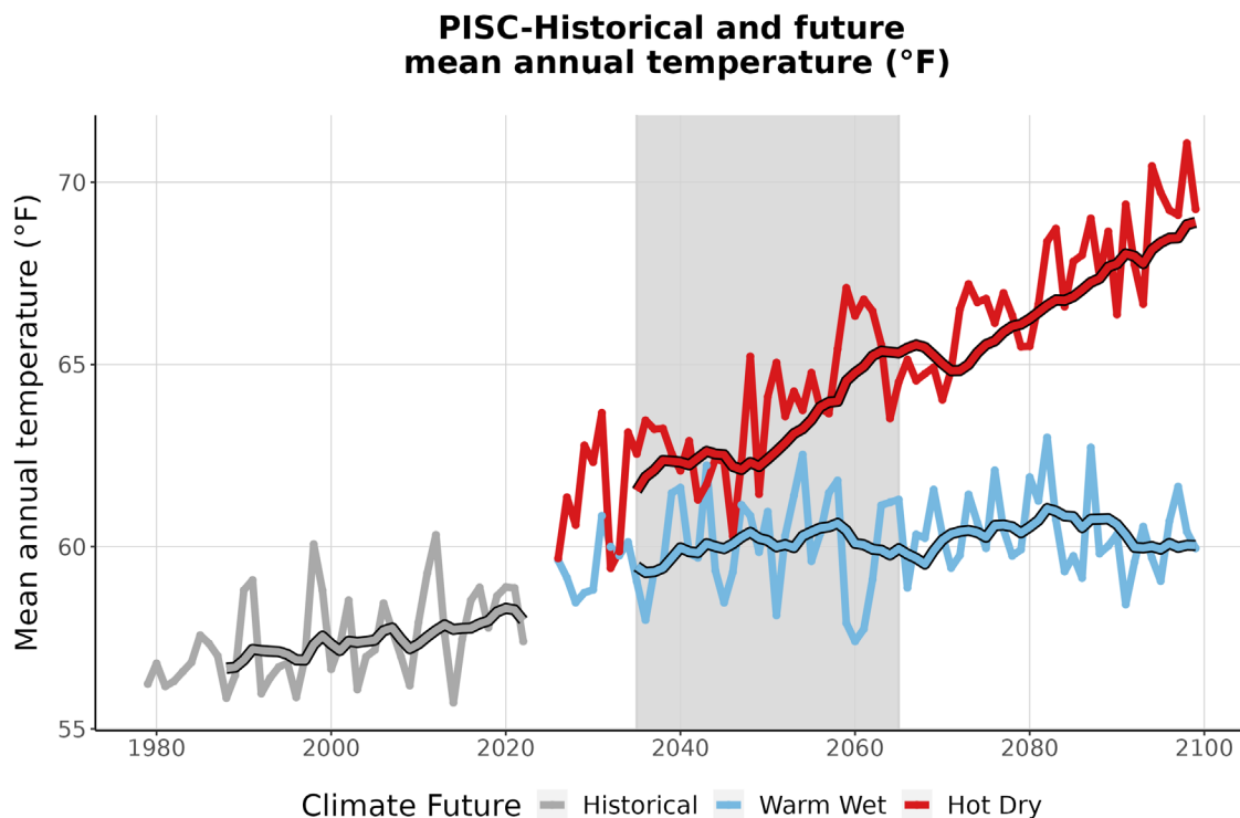
Figure 3. This graph compares observed average annual temperature at PISC (°F) (1979-2022) with projected average annual temperature for the two climate futures over the period 2023-2099. The historically observed data
