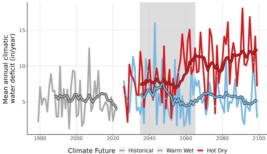
Figure 9. This line graph compares observed climatic water deficit at PISC (inches/year) (1979-2022) with projected climatic water deficit for the two climate futures over the period 2023-2099. The historical observation data is shown in gray, the Warm Wet climate future in blue, and the Hot Dry climate future in red. The smooth line running through each projection is the 10-year running average for historical observations and future projections. Gray-shaded area represents the time period that was averaged (2035-2065) to summarize future projections for the year 2050.
