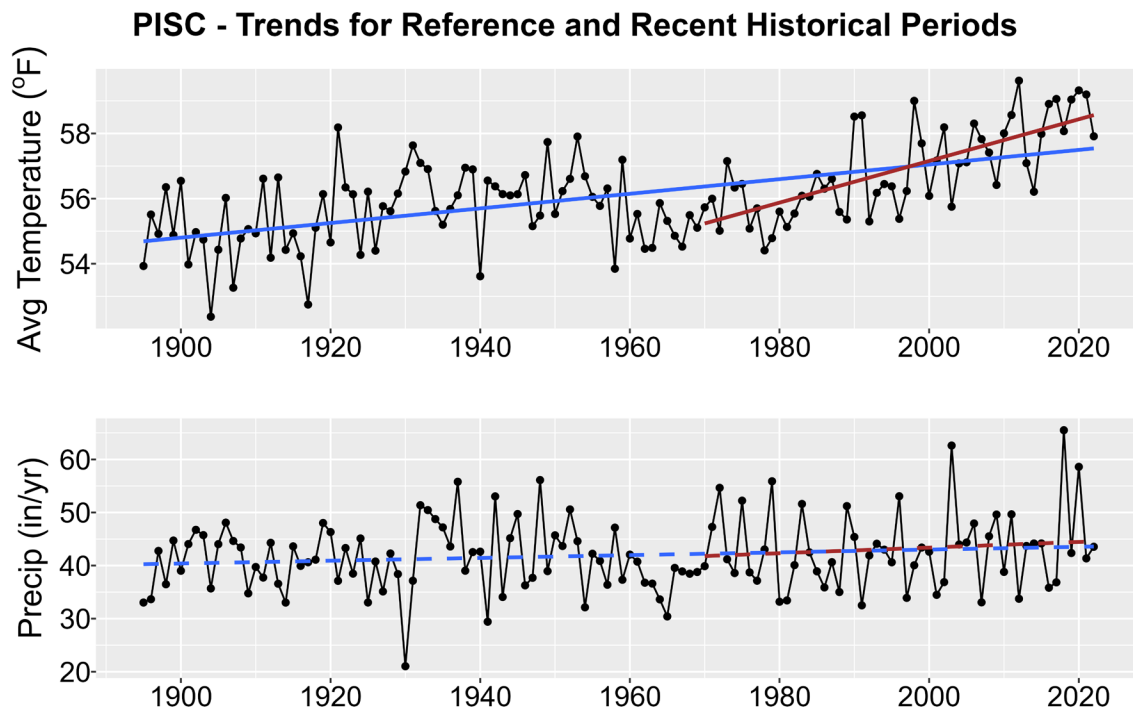
Figure 1. Historical trends in annual average temperature (upper plot) and annual total precipitation (lower plot) for PISC from 1895-2022. Black points show yearly values while blue lines are linear regressions for the entire period record and red lines for 1970-2022 trends. Solid lines are significant trends (i.e., p < 0.05 ); dashed lines are not statistically significant.
