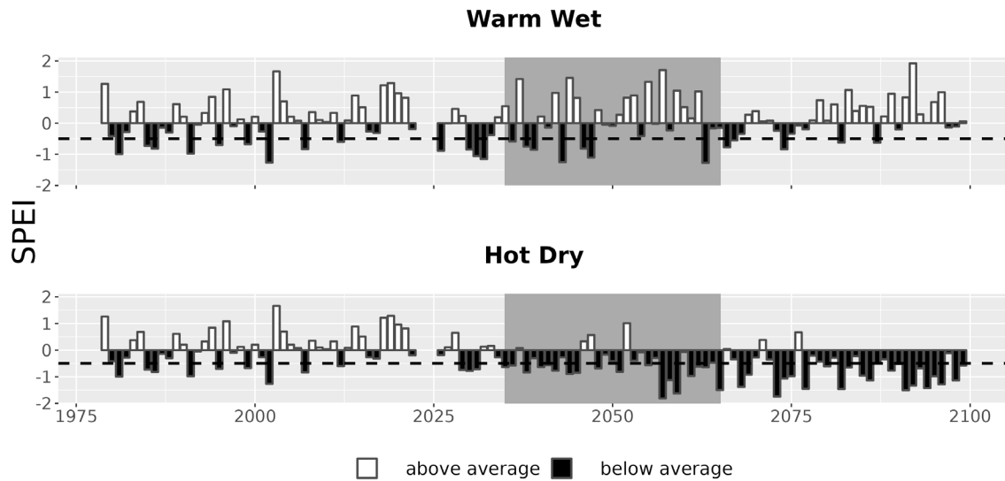
Figure 7. Drought metrics for PISC. Drought index (SPEI; units = standard deviations from historical) timeseries for each climate future. Below-average SPEI (black bars) indicates dry conditions. The dotted line (SPEI = -0.5) indicates drought conditions.
