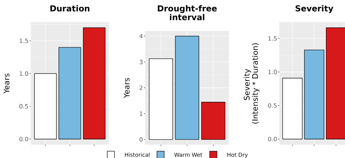
Figure 8. Drought metrics for PISC. (Left) Average drought duration (years) historically (1979-2012) and under each climate future. (Middle) Average drought return interval (years), indicating the expected amount of time between periods of drought, historically and under each climate future. (Right) Average drought severity, a measure of drought intensity multiplied by duration, historically and under each climate future.
