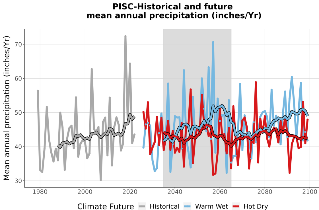
Figure 4. This graph compares observed average annual precipitation at PISC (inches/year) (1979-2022) with projected average annual precipitation for the two climate futures over the period 2023-2099. The historically observed data is shown in gray, the Warm Wet climate future in blue, and the Hot Dry climate future in red. The smooth line running through each projection is the 10-year running average for historical observations and future projections. The gray-shaded area represents the time period that was averaged (2035-2065) to summarize future projections for the year 2050 (Appendix 1).
