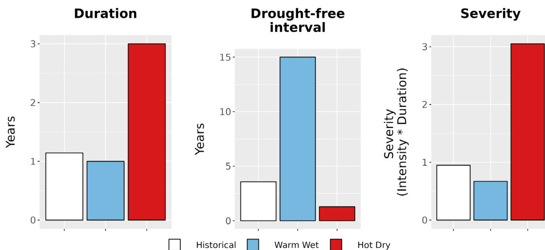
Figure 8. Drought metrics for PIRO. (Left) Average drought duration (years) historically (1979-2012) and under each climate future. (Middle) Average drought return interval (years), indicating the expected amount of time between periods of drought, historically and under each climate future. (Right) Average drought severity, a measure of drought intensity multiplied by duration, historically and under each climate future.
