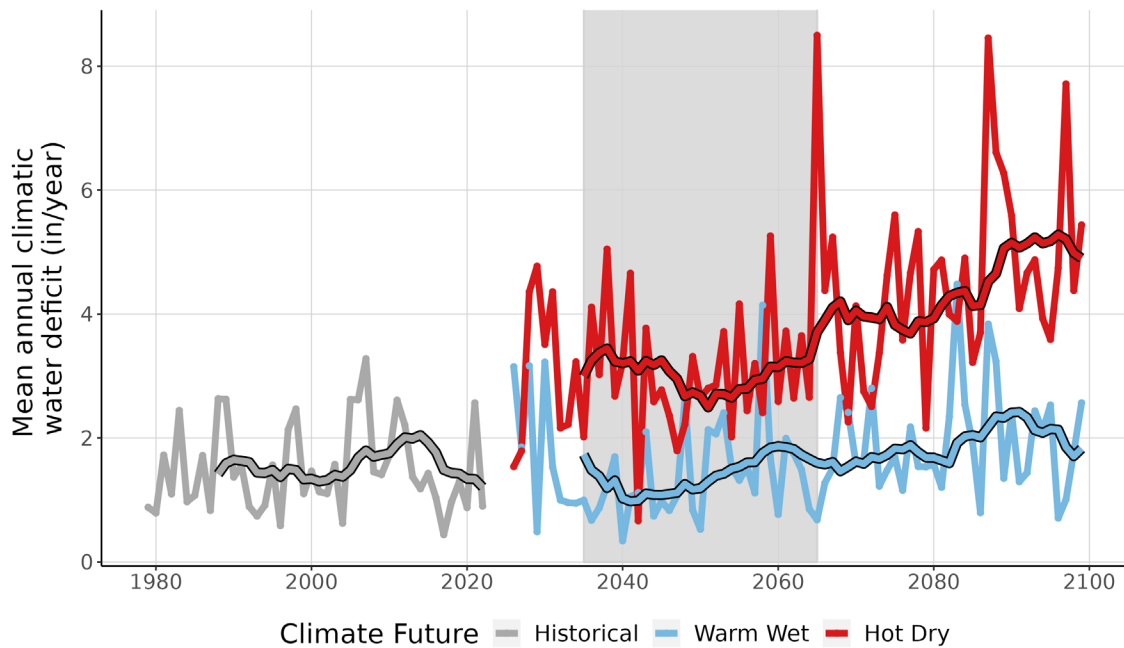
Figure 9. This line graph compares observed climatic water deficit at PIRO (inches/year) (1979-2022) with projected climatic water deficit for the two climate futures over the period 2023-2099. The historical observation data is shown in gray, the Warm Wet climate future in blue, and the Hot Dry climate future in red. The smooth line running through each projection is the 10-year running average for historical observations and future projections. Gray-shaded area represents the time period that was averaged (2035-2065) to summarize future projections for the year 2050.
