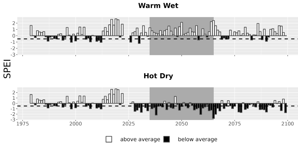
Figure 7. Drought metrics for PIRO. Drought index (SPEI; units = standard deviations from historical) timeseries for each climate future. Below-average SPEI (black bars) indicates dry conditions. The dotted line (SPEI = -0.5) indicates drought conditions.
