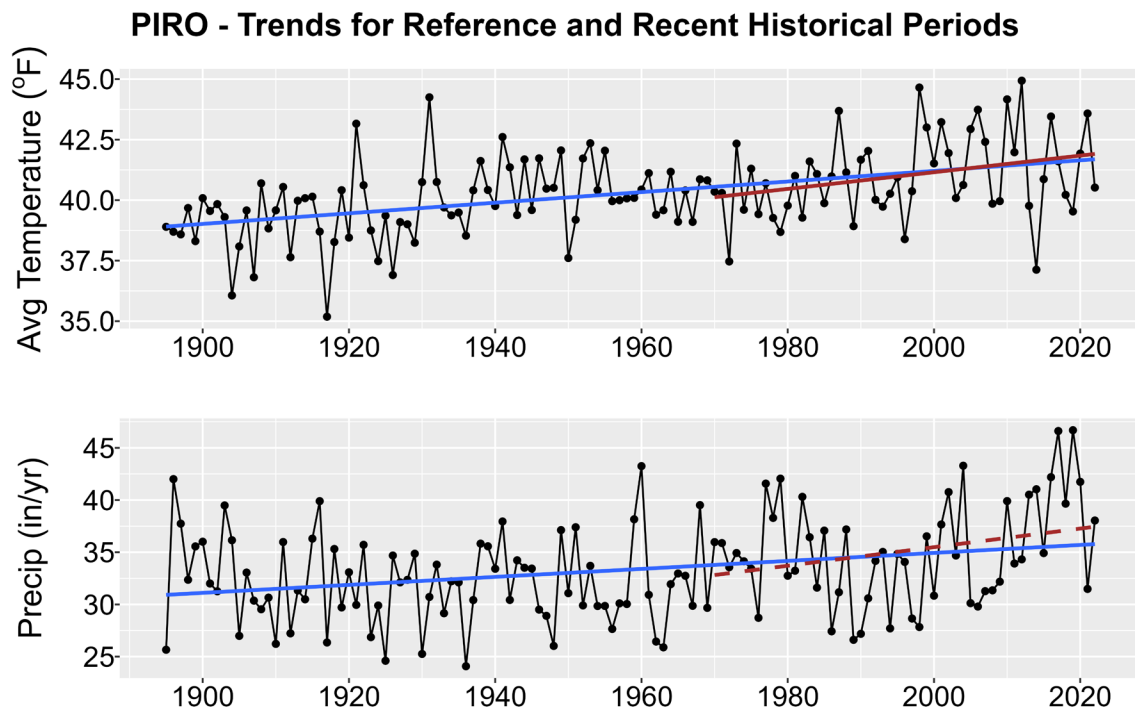
Figure 1. Historical trends in annual average temperature (upper plot) and annual total precipitation (lower plot) for PIRO from 1895-2022. Black points show yearly values while blue lines are linear regressions for the entire period record and red lines for 1970-2022 trends. Solid lines are significant trends (i.e., p < 0.05 ); dashed lines are not statistically significant.
