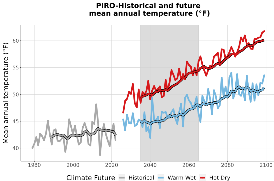
Figure 3. This graph compares observed average annual temperature at PIRO (°F) (1979-2022) with projected average annual temperature for the two climate futures over the period 2023-2099. The historically observed data is shown in gray, the Warm Wet climate future in blue, and the Hot Dry climate future in red. The smooth line
