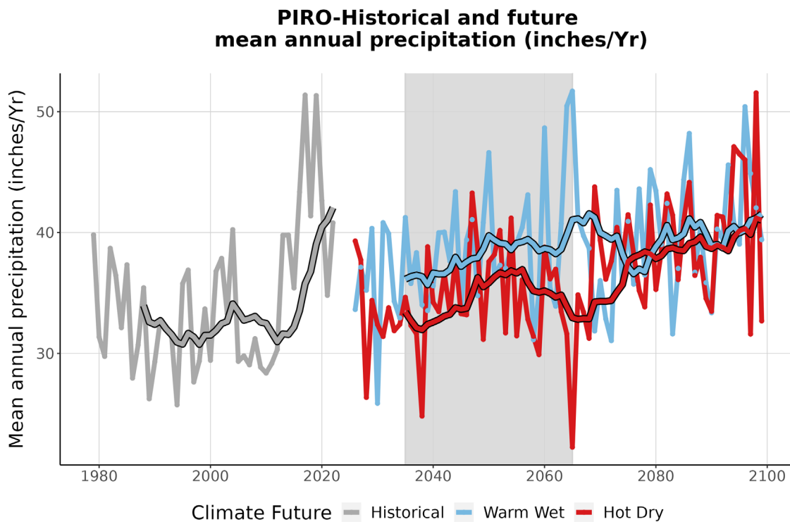
Figure 4. This graph compares observed average annual precipitation at PIRO (inches/year) (1979-2022) with projected average annual precipitation for the two climate futures over the period 2023-2099. The historically observed data is shown in gray, the Warm Wet climate future in blue, and the Hot Dry climate future in red. The smooth line running through each projection is the 10-year running average for historical observations and future projections. The gray-shaded area represents the time period that was averaged (2035-2065) to summarize future projections for the year 2050 (Appendix 1).
