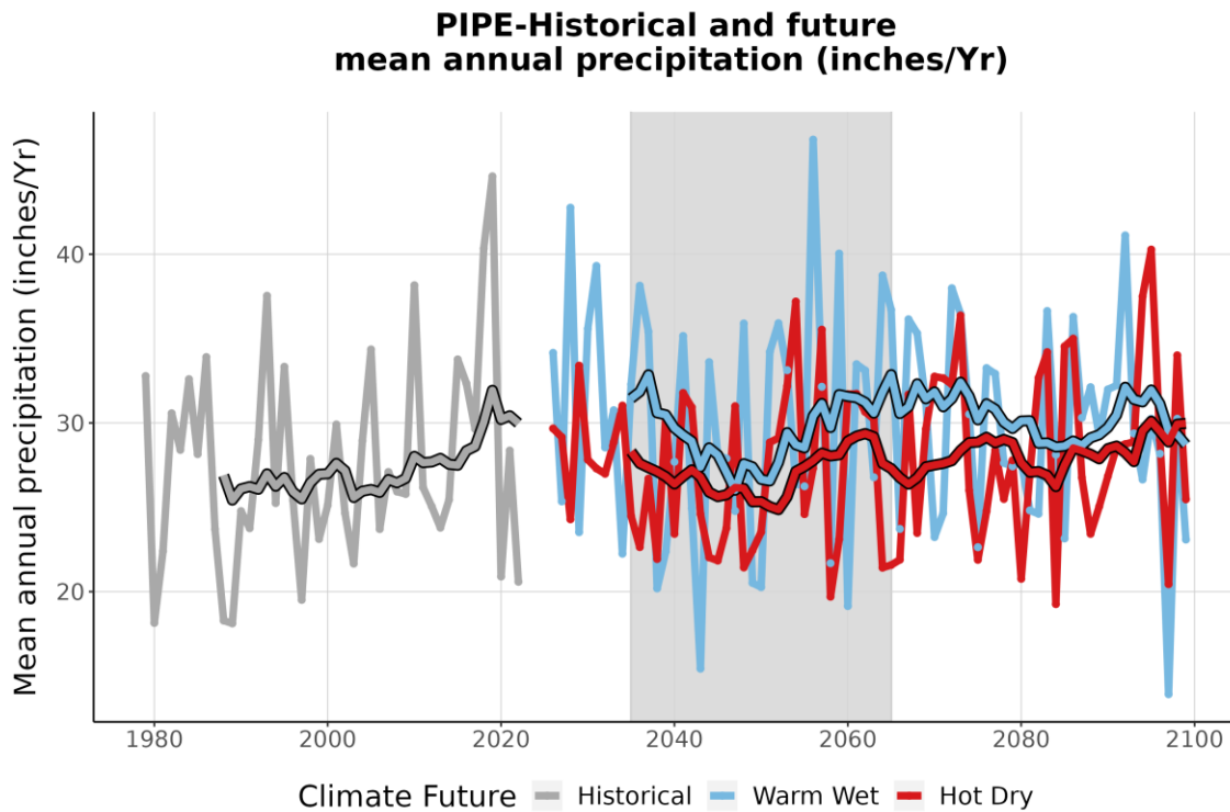
Figure 4. This graph compares observed average annual precipitation at PIPE (inches/year) (1979-2022) with projected average annual precipitation for the two climate futures over the period 2023-2099. The historically observed data is shown in gray, the Warm Wet climate future in blue, and the Hot Dry climate future in red. The smooth line running through each projection is the 10-year running average for historical observations and future projections. The gray-shaded area represents the time period that was averaged (2035-2065) to summarize future projections for the year 2050 (Appendix 1).
