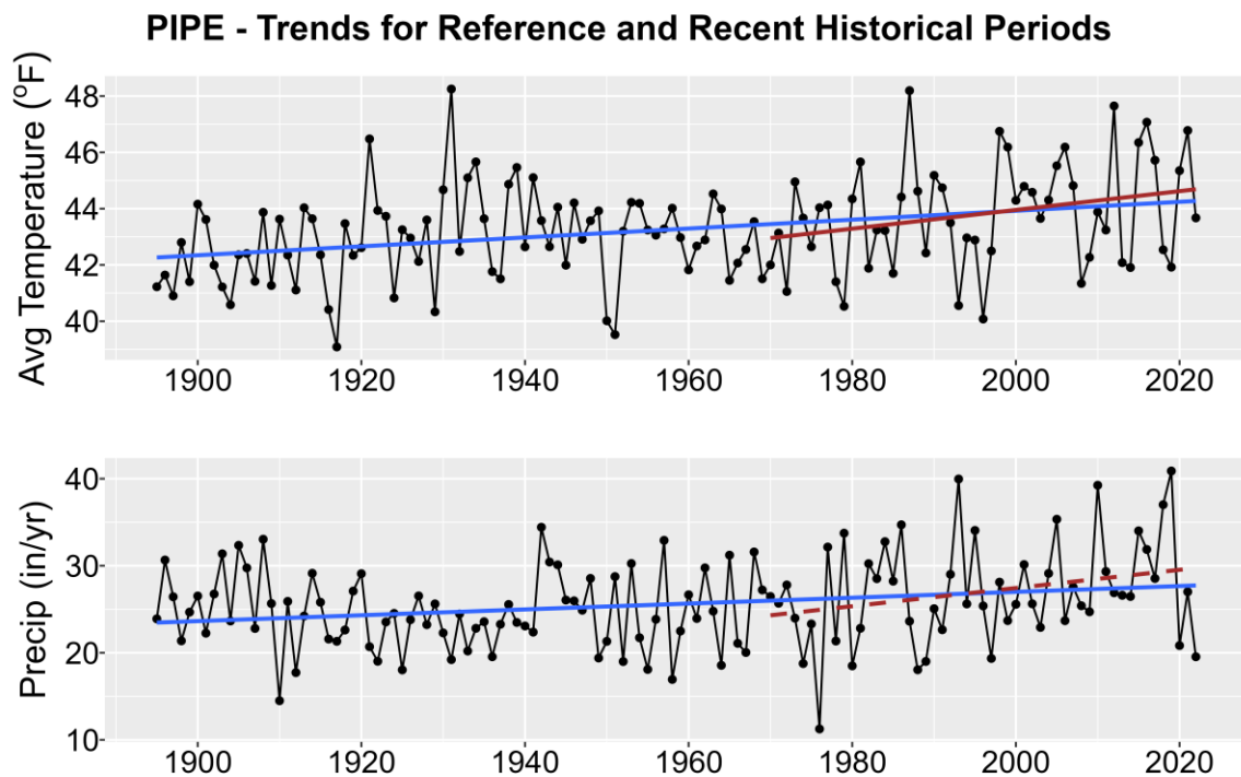
Figure 1. Historical trends in annual average temperature (upper plot) and annual total precipitation (lower plot) for PIPE from 1895-2022. Black points show yearly values while blue lines are linear regressions for the entire period record and red lines for 1970-2022 trends. Solid lines are significant trends (i.e., p < 0.05 ); dashed lines are not statistically significant.
