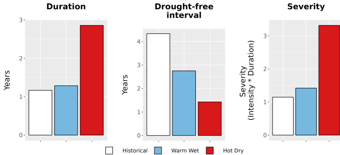
Figure 8. Drought metrics for PIPE. (Left) Average drought duration (years) historically (1979-2012) and under each climate future. (Middle) Average drought return interval (years), indicating the expected amount of time between periods of drought, historically and under each climate future. (Right) Average drought severity, a measure of drought intensity multiplied by duration, historically and under each climate future.
