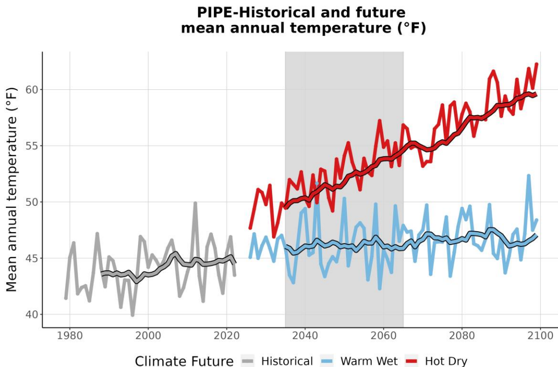
Figure 3. This graph compares observed average annual temperature at PIPE (°F) (1979-2022) with projected average annual temperature for the two climate futures over the period 2023-2099. The historically observed data
