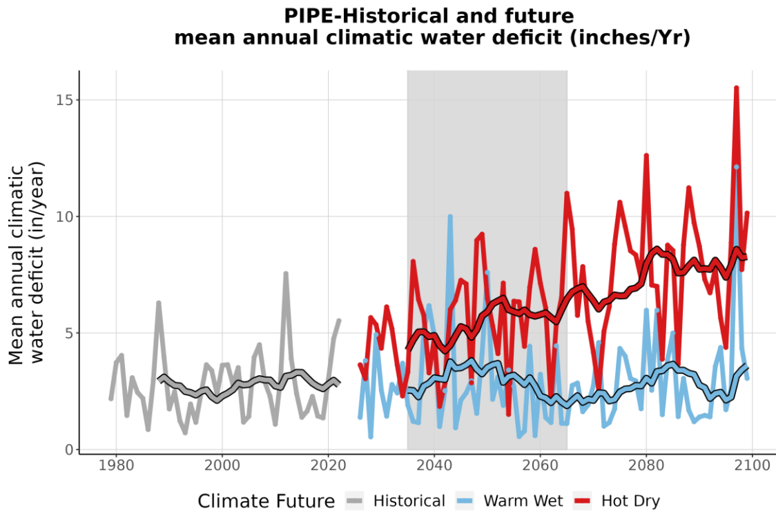
Figure 9. This line graph compares observed climatic water deficit at PIPE (inches/year) (1979-2022) with projected climatic water deficit for the two climate futures over the period 2023-2099. The historical observation data is shown in gray, the Warm Wet climate future in blue, and the Hot Dry climate future in red. The smooth line running through each projection is the 10-year running average for historical observations and future projections. Gray-shaded area represents the time period that was averaged (2035-2065) to summarize future projections for the year 2050.
