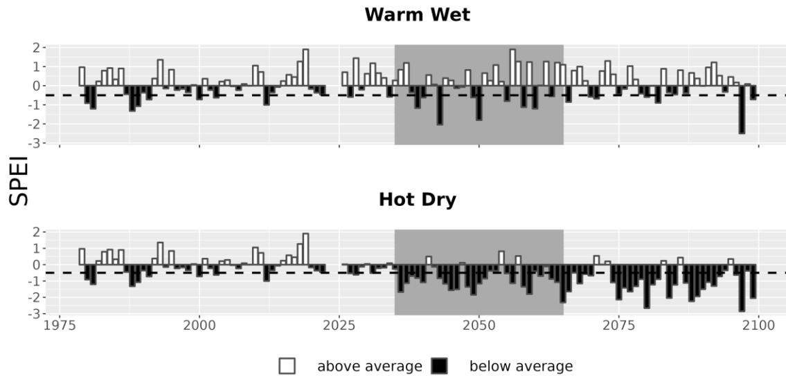
Figure 7. Drought metrics for PIPE. Drought index (SPEI; units = standard deviations from historical) timeseries for each climate future. Below-average SPEI (black bars) indicates dry conditions. The dotted line (SPEI = -0.5) indicates drought conditions.
