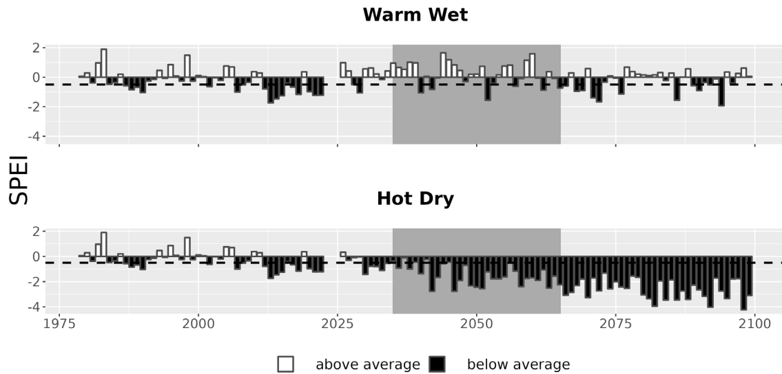
Figure 7. Drought metrics for PINN. Drought index (SPEI; units = standard deviations from historical) timeseries for each climate future. Below-average SPEI (black bars) indicates dry conditions. The dotted line (SPEI = -0.5) indicates drought conditions.
