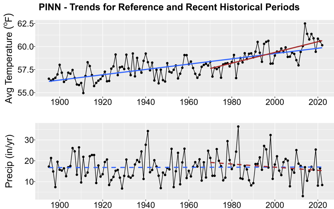
Figure 1. Historical trends in annual average temperature (upper plot) and annual total precipitation (lower plot) for PINN from 1895-2022. Black points show yearly values while blue lines are linear regressions for the entire period record and red lines for 1970-2022 trends. Solid lines are significant trends (i.e., p < 0.05 ); dashed lines are not statistically significant.
