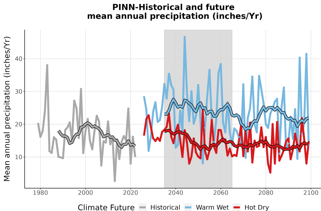
Figure 4. This graph compares observed average annual precipitation at PINN (inches/year) (1979-2022) with projected average annual precipitation for the two climate futures over the period 2023-2099. The historically observed data is shown in gray, the Warm Wet climate future in blue, and the Hot Dry climate future in red. The smooth line running through each projection is the 10-year running average for historical observations and future projections. The gray-shaded area represents the time period that was averaged (2035-2065) to summarize future projections for the year 2050 (Appendix 1).
