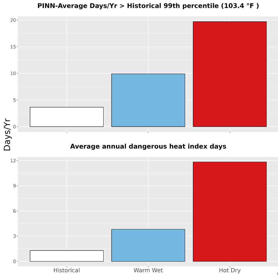
Figure 5. The upper bar graph represents the average number of days annually with temperatures greater than the historical 99th percentile (103.4 °F) historically (1979-2012) and for the two climate futures (2050). The bottom bar graph represents the average annual number of dangerous heat index days historically and for the two climate futures. Dangerous heat index days are days that exceed 105 °F.
