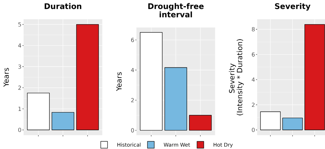
Figure 8. Drought metrics for PINN. (Left) Average drought duration (years) historically (1979-2012) and under each climate future. (Middle) Average drought return interval (years), indicating the expected amount of time between periods of drought, historically and under each climate future. (Right) Average drought severity, a measure of drought intensity multiplied by duration, historically and under each climate future.
