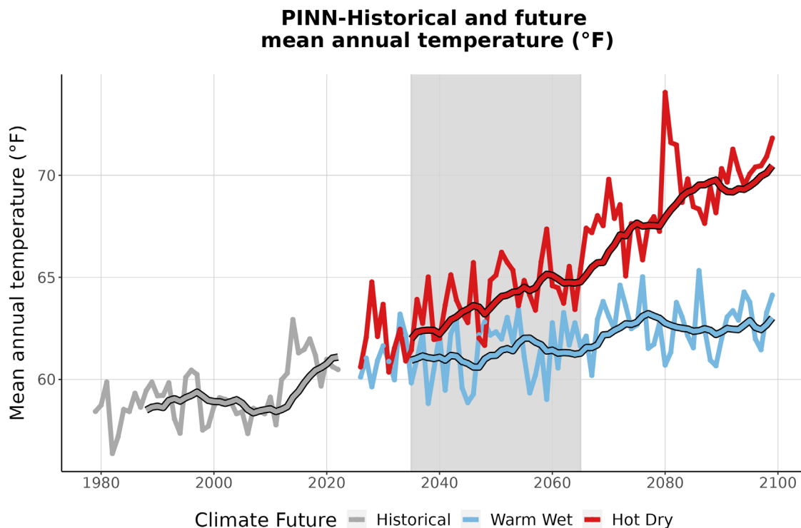
Figure 3. This graph compares observed average annual temperature at PINN (°F) (1979-2022) with projected average annual temperature for the two climate futures over the period 2023-2099. The historically observed data
