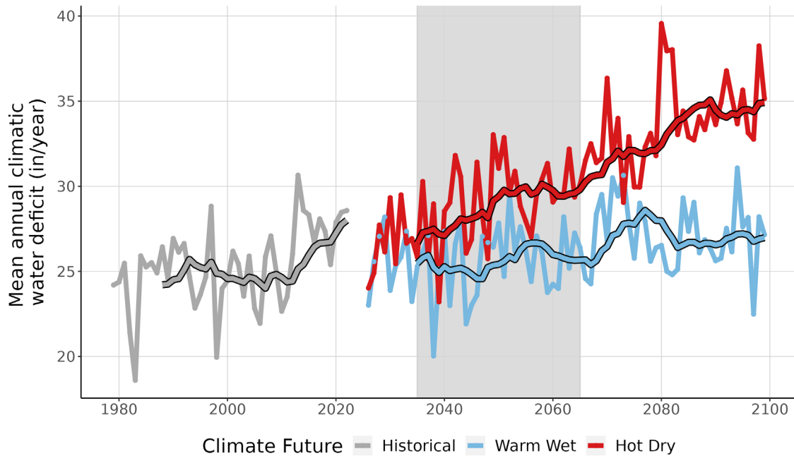
Figure 9. This line graph compares observed climatic water deficit at PINN (inches/year) (1979-2022) with projected climatic water deficit for the two climate futures over the period 2023-2099. The historical observation data is shown in gray, the Warm Wet climate future in blue, and the Hot Dry climate future in red. The smooth line running through each projection is the 10-year running average for historical observations and future projections. Gray-shaded area represents the time period that was averaged (2035-2065) to summarize future projections for the year 2050.
