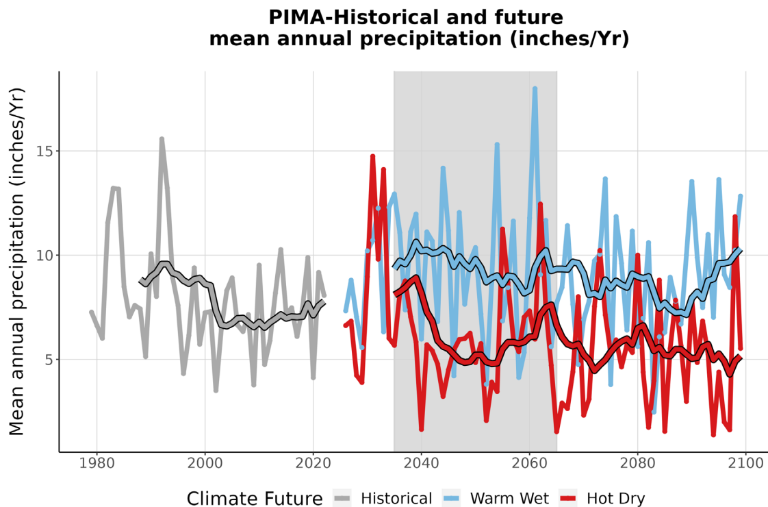
Figure 4. This graph compares observed average annual precipitation at PIMA (inches/year) (1979-2022) with projected average annual precipitation for the two climate futures over the period 2023-2099. The historically observed data is shown in gray, the Warm Wet climate future in blue, and the Hot Dry climate future in red. The smooth line running through each projection is the 10-year running average for historical observations and future projections. The gray-shaded area represents the time period that was averaged (2035-2065) to summarize future projections for the year 2050 (Appendix 1).
