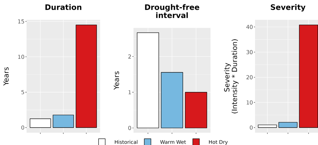
Figure 8. Drought metrics for PIMA. (Left) Average drought duration (years) historically (1979-2012) and under each climate future. (Middle) Average drought return interval (years), indicating the expected amount of time between periods of drought, historically and under each climate future. (Right) Average drought severity, a measure of drought intensity multiplied by duration, historically and under each climate future.
