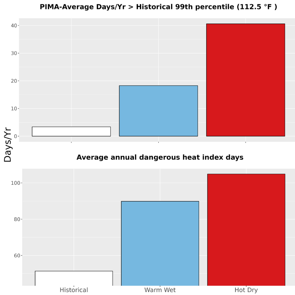
Figure 5. The upper bar graph represents the average number of days annually with temperatures greater than the historical 99th percentile (112.5 °F) historically (1979-2012) and for the two climate futures (2050). The bottom bar graph represents the average annual number of dangerous heat index days historically and for the two climate futures. Dangerous heat index days are days that exceed 105 °F.
