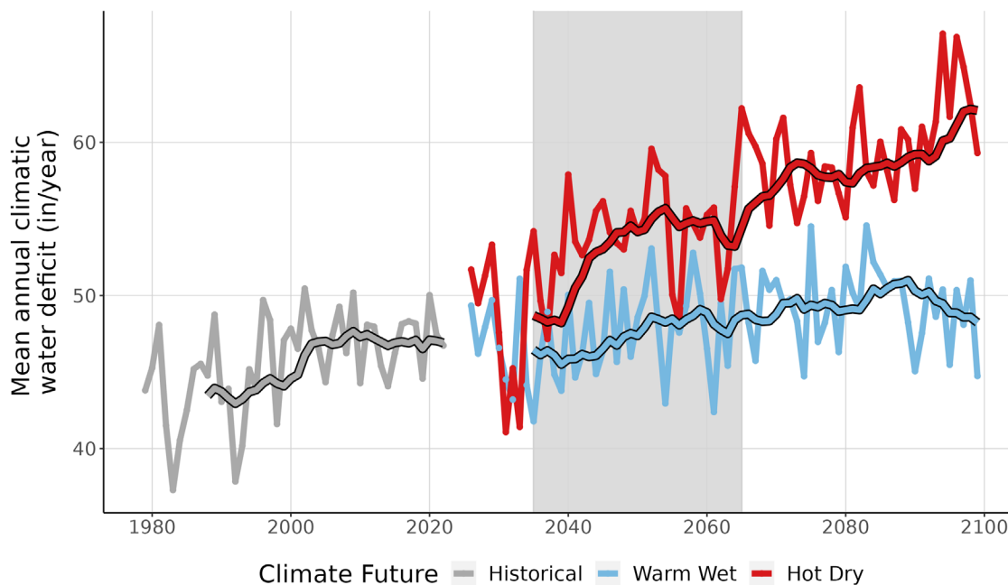
Figure 9. This line graph compares observed climatic water deficit at PIMA (inches/year) (1979-2022) with projected climatic water deficit for the two climate futures over the period 2023-2099. The historical observation data is shown in gray, the Warm Wet climate future in blue, and the Hot Dry climate future in red. The smooth line running through each projection is the 10-year running average for historical observations and future projections. Gray-shaded area represents the time period that was averaged (2035-2065) to summarize future projections for the year 2050.
