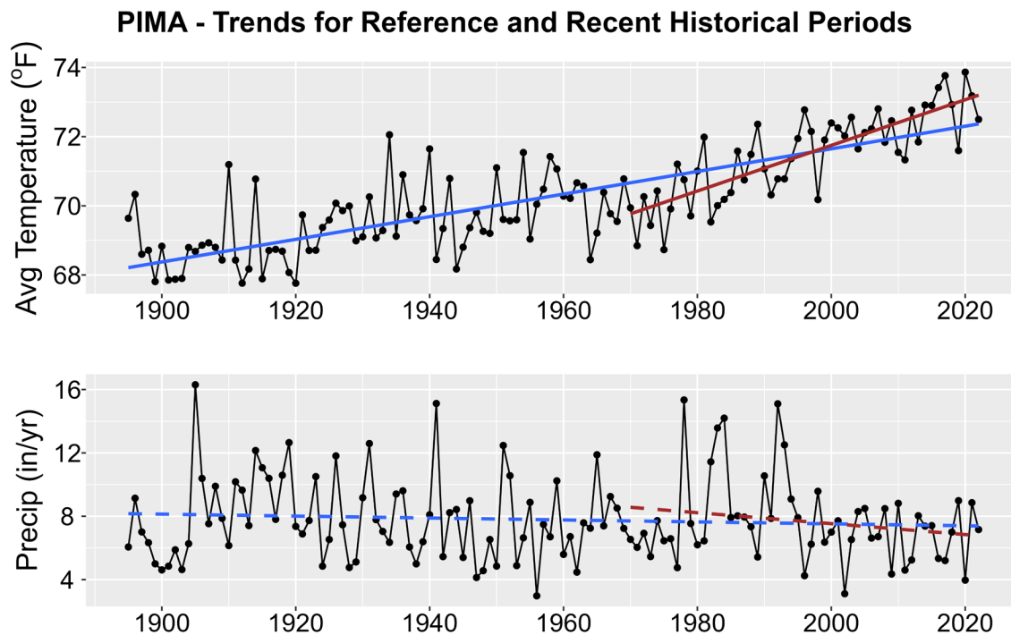
Figure 1. Historical trends in annual average temperature (upper plot) and annual total precipitation (lower plot) for PIMA from 1895-2022. Black points show yearly values while blue lines are linear regressions for the entire period record and red lines for 1970-2022 trends. Solid lines are significant trends (i.e., p < 0.05 ); dashed lines are not statistically significant.
