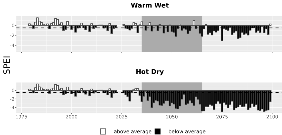
Figure 7. Drought metrics for PIMA. Drought index (SPEI; units = standard deviations from historical) timeseries for each climate future. Below-average SPEI (black bars) indicates dry conditions. The dotted line (SPEI = -0.5) indicates drought conditions.
