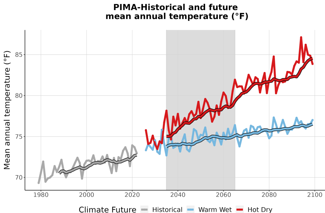
Figure 3. This graph compares observed average annual temperature at PIMA (°F) (1979-2022) with projected average annual temperature for the two climate futures over the period 2023-2099. The historically observed data
