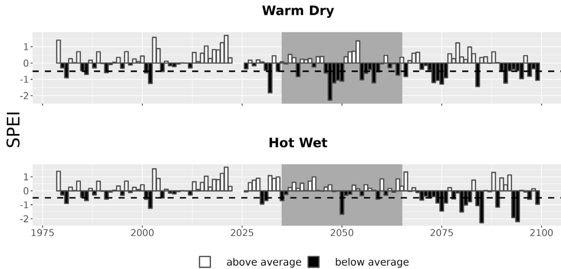
Figure 7. Drought metrics for PETE. Drought index (SPEI; units = standard deviations from historical) timeseries for each climate future. Below-average SPEI (black bars) indicates dry conditions. The dotted line (SPEI = -0.5) indicates drought conditions.
