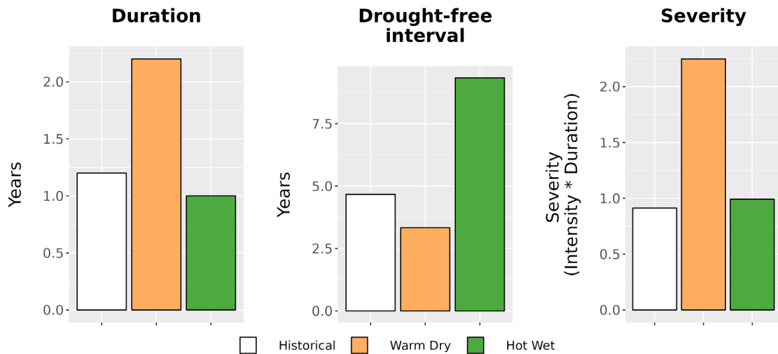
Figure 8. Drought metrics for PETE. (Left) Average drought duration (years) historically (1979-2012) and under each climate future. (Middle) Average drought return interval (years), indicating the expected amount of time between periods of drought, historically and under each climate future. (Right) Average drought severity, a measure of drought intensity multiplied by duration, historically and under each climate future.
