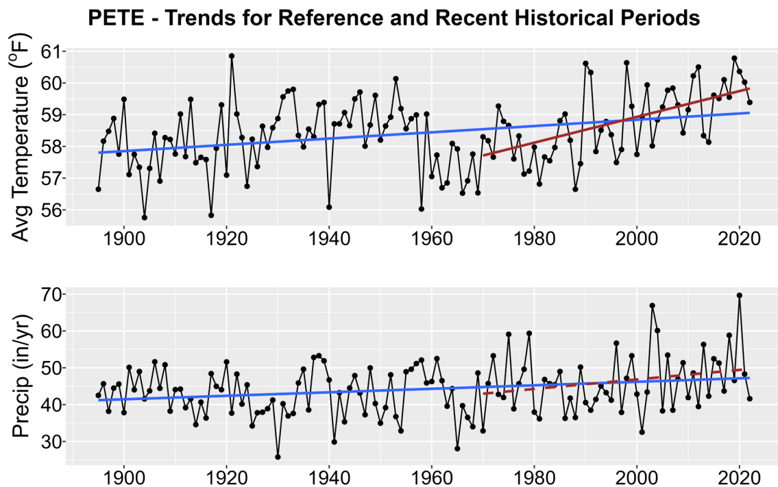
Figure 1. Historical trends in annual average temperature (upper plot) and annual total precipitation (lower plot) for PETE from 1895-2022. Black points show yearly values while blue lines are linear regressions for the entire period record and red lines for 1970-2022 trends. Solid lines are significant trends (i.e., p < 0.05 ); dashed lines are not statistically significant.
