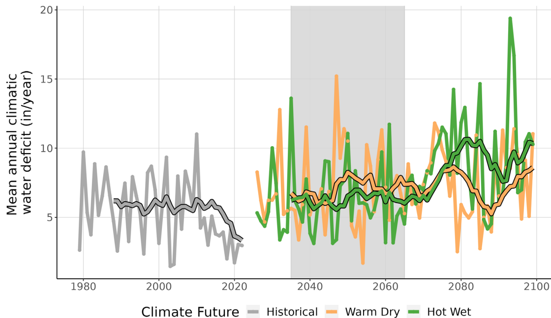
Figure 9. This line graph compares observed climatic water deficit at PETE (inches/year) (1979-2022) with projected climatic water deficit for the two climate futures over the period 2023-2099. The historical observation data is shown in gray, the Warm Dry climate future in orange, and the Hot Wet climate future in green. The smooth line running through each projection is the 10-year running average for historical observations and future projections. Gray-shaded area represents the time period that was averaged (2035-2065) to summarize future projections for the year 2050.
