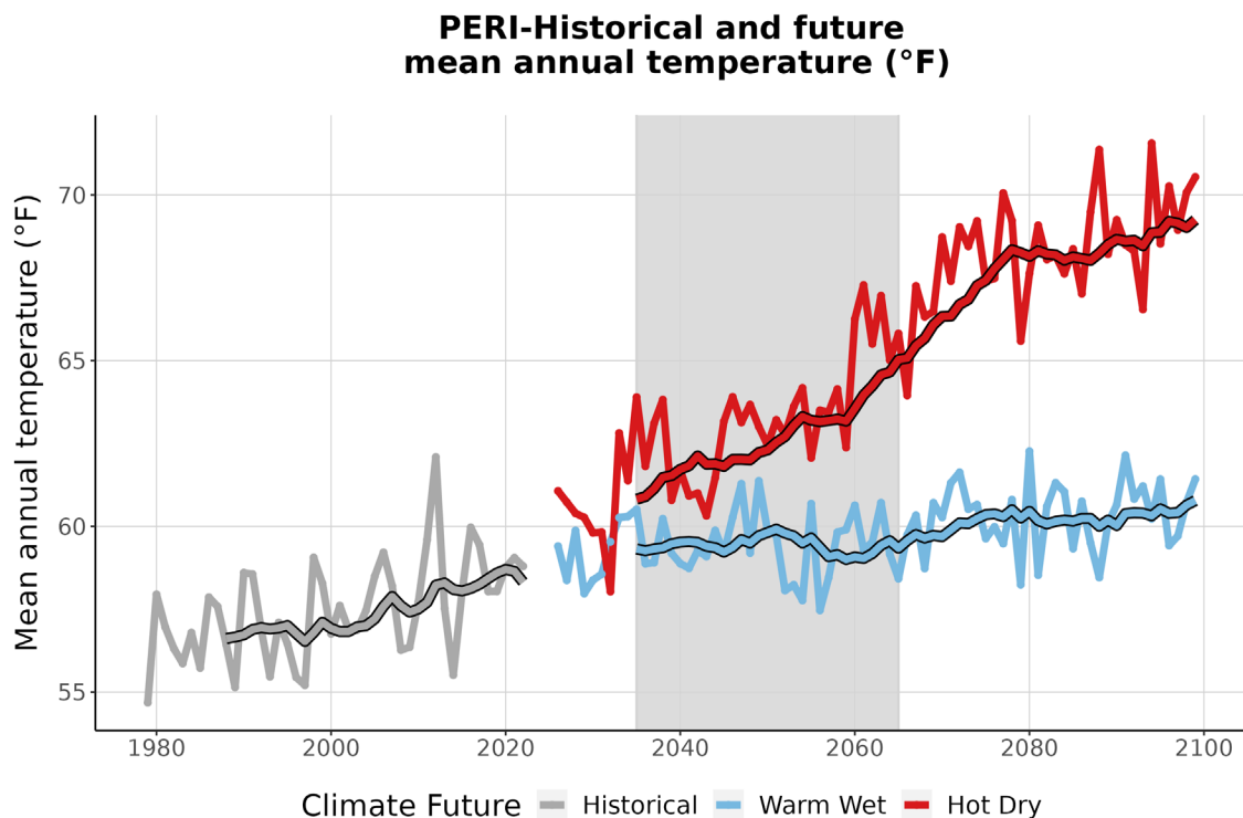
Figure 3. This graph compares observed average annual temperature at PERI (°F) (1979-2022) with projected average annual temperature for the two climate futures over the period 2023-2099. The historically observed data
