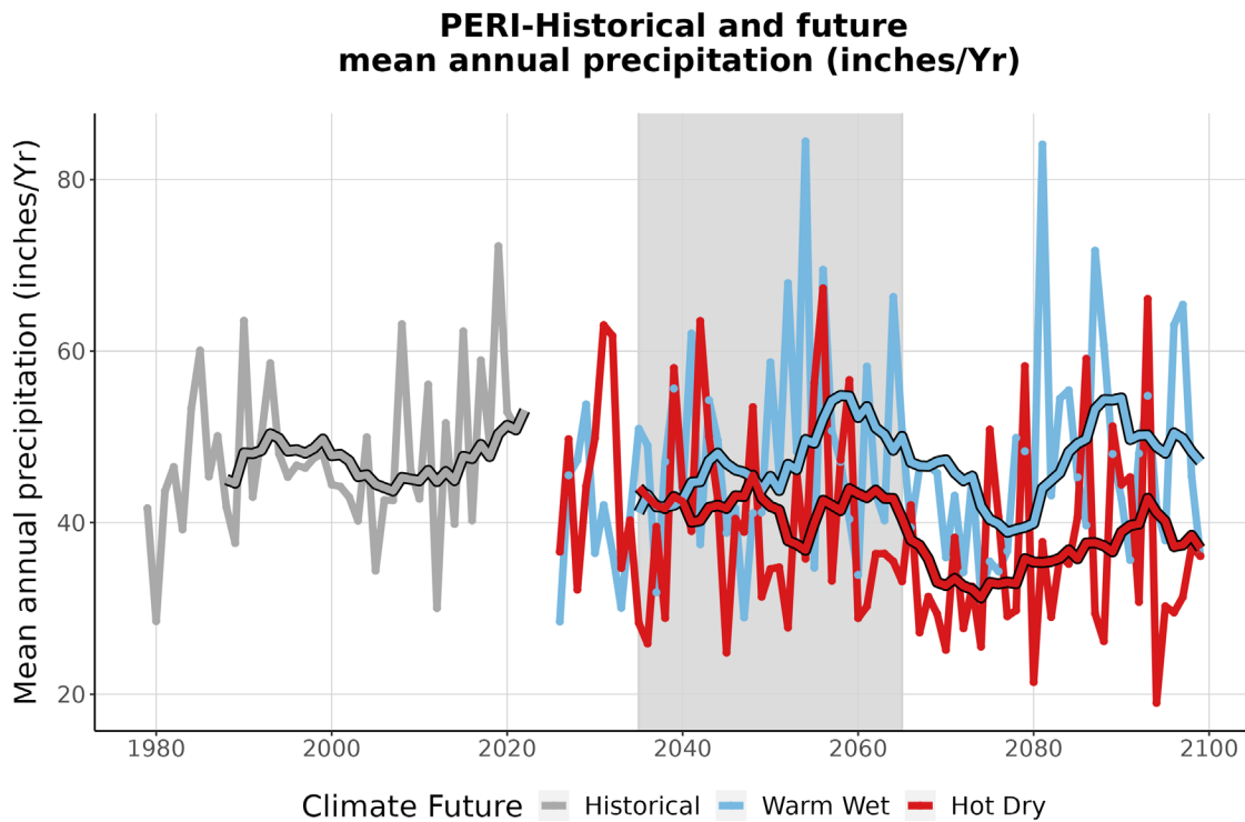
Figure 4. This graph compares observed average annual precipitation at PERI (inches/year) (1979-2022) with projected average annual precipitation for the two climate futures over the period 2023-2099. The historically observed data is shown in gray, the Warm Wet climate future in blue, and the Hot Dry climate future in red. The smooth line running through each projection is the 10-year running average for historical observations and future projections. The gray-shaded area represents the time period that was averaged (2035-2065) to summarize future projections for the year 2050 (Appendix 1).
