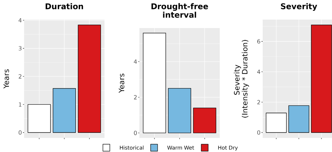
Figure 8. Drought metrics for PERI. (Left) Average drought duration (years) historically (1979-2012) and under each climate future. (Middle) Average drought return interval (years), indicating the expected amount of time between periods of drought, historically and under each climate future. (Right) Average drought severity, a measure of drought intensity multiplied by duration, historically and under each climate future.
