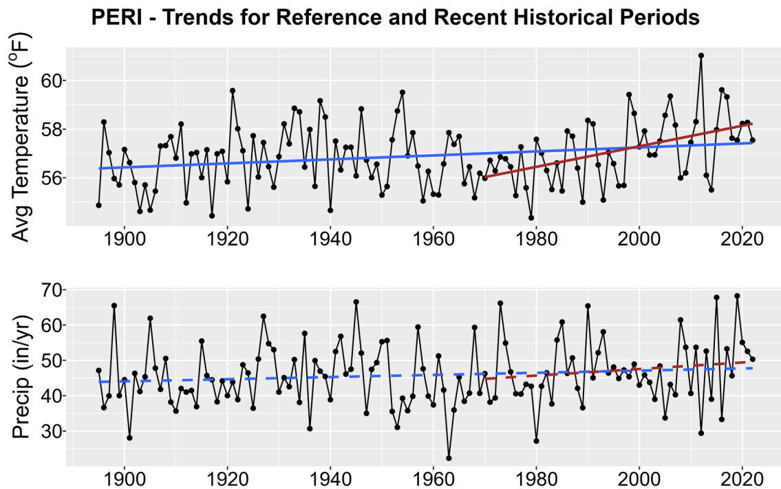
Figure 1. Historical trends in annual average temperature (upper plot) and annual total precipitation (lower plot) for PERI from 1895-2022. Black points show yearly values while blue lines are linear regressions for the entire period record and red lines for 1970-2022 trends. Solid lines are significant trends (i.e., p < 0.05 ); dashed lines are not statistically significant.
