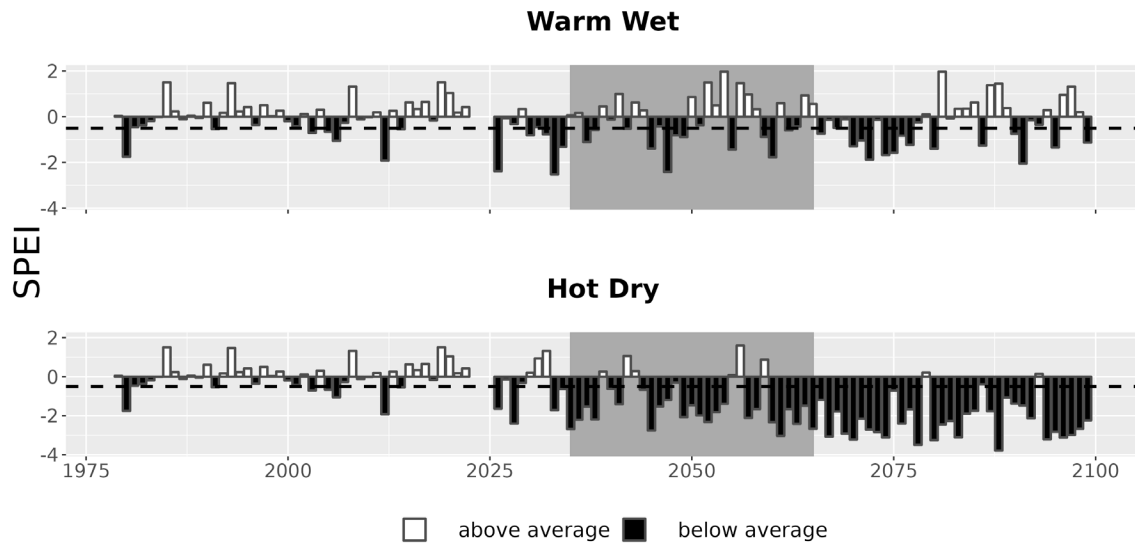
Figure 7. Drought metrics for PERI. Drought index (SPEI; units = standard deviations from historical) timeseries for each climate future. Below-average SPEI (black bars) indicates dry conditions. The dotted line (SPEI = -0.5) indicates drought conditions.
