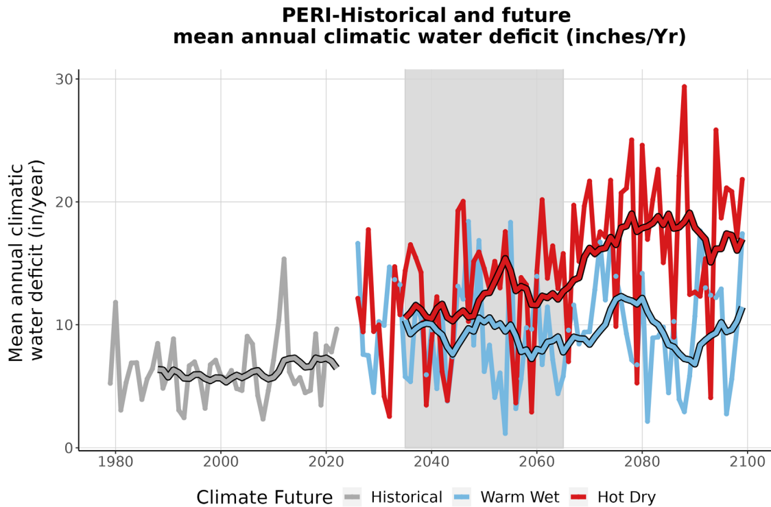
Figure 9. This line graph compares observed climatic water deficit at PERI (inches/year) (1979-2022) with projected climatic water deficit for the two climate futures over the period 2023-2099. The historical observation data is shown in gray, the Warm Wet climate future in blue, and the Hot Dry climate future in red. The smooth line running through each projection is the 10-year running average for historical observations and future projections. Gray-shaded area represents the time period that was averaged (2035-2065) to summarize future projections for the year 2050.
