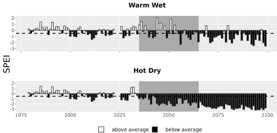
Figure 7. Drought metrics for PECO. Drought index (SPEI; units = standard deviations from historical) timeseries for each climate future. Below-average SPEI (black bars) indicates dry conditions. The dotted line (SPEI = -0.5) indicates drought conditions.
