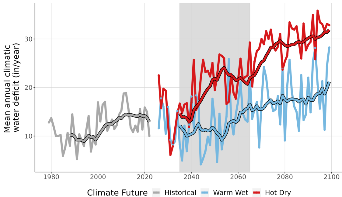
Figure 9. This line graph compares observed climatic water deficit at PECO (inches/year) (1979-2022) with projected climatic water deficit for the two climate futures over the period 2023-2099. The historical observation data is shown in gray, the Warm Wet climate future in blue, and the Hot Dry climate future in red. The smooth line running through each projection is the 10-year running average for historical observations and future projections. Gray-shaded area represents the time period that was averaged (2035-2065) to summarize future projections for the year 2050.
