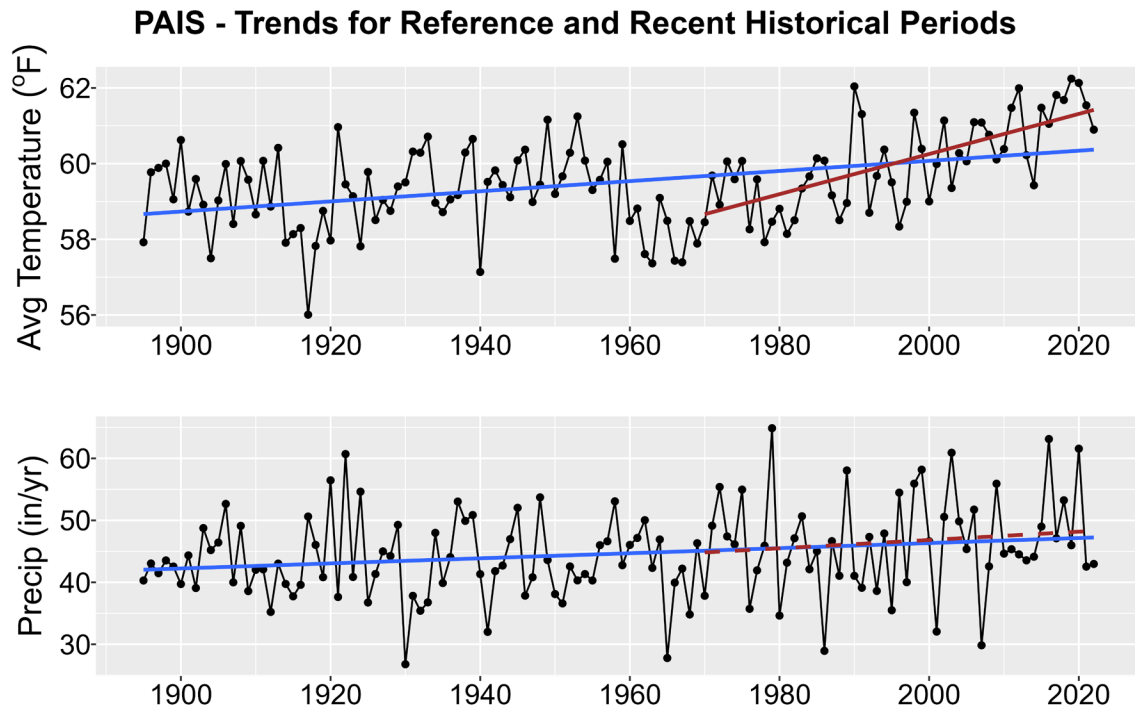
Figure 1. Historical trends in annual average temperature (upper plot) and annual total precipitation (lower plot) for PAIS from 1895-2022. Black points show yearly values while blue lines are linear regressions for the entire period record and red lines for 1970-2022 trends. Solid lines are significant trends (i.e., p < 0.05 ); dashed lines are not statistically significant.
