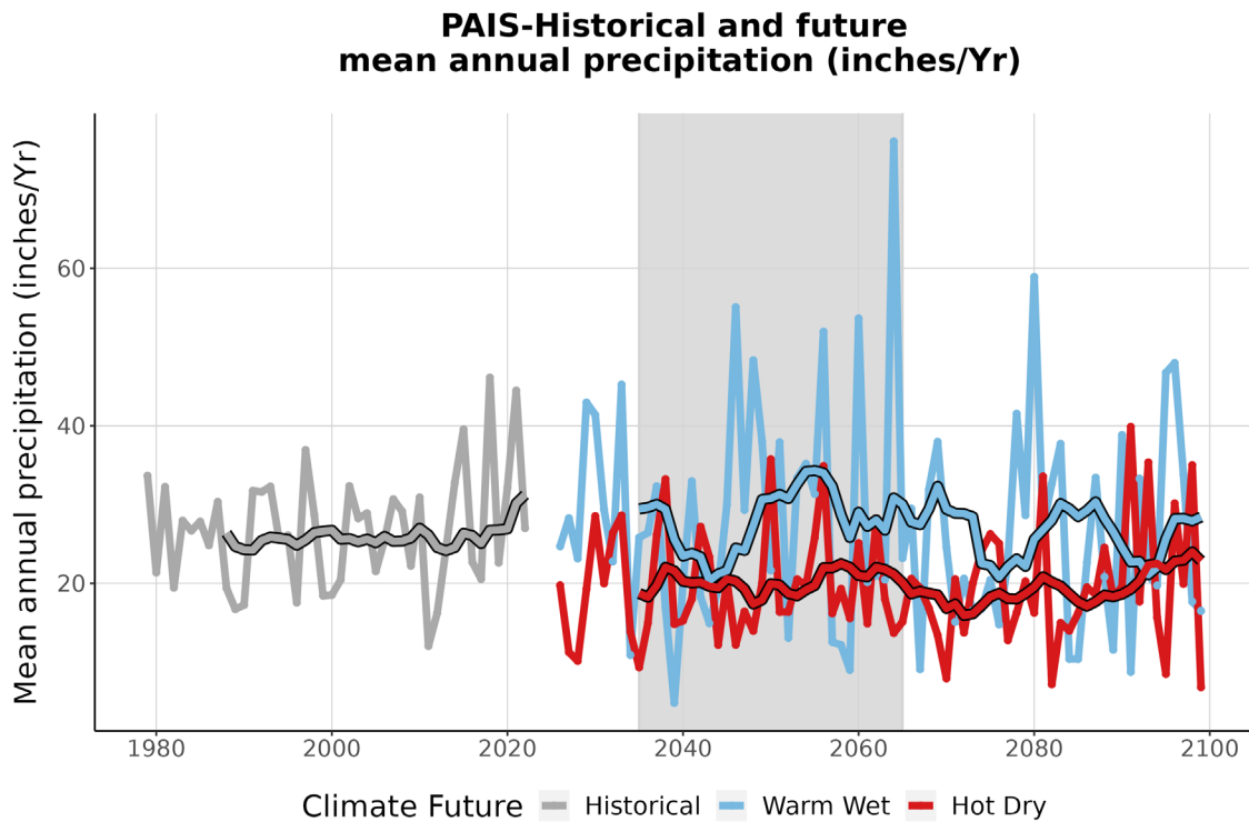
Figure 4. This graph compares observed average annual precipitation at PAIS (inches/year) (1979-2022) with projected average annual precipitation for the two climate futures over the period 2023-2099. The historically observed data is shown in gray, the Warm Wet climate future in blue, and the Hot Dry climate future in red. The smooth line running through each projection is the 10-year running average for historical observations and future projections. The gray-shaded area represents the time period that was averaged (2035-2065) to summarize future projections for the year 2050 (Appendix 1).
