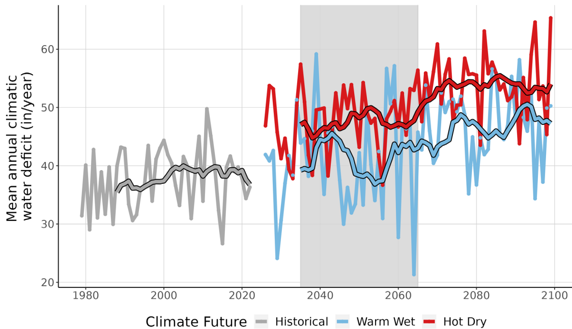
Figure 9. This line graph compares observed climatic water deficit at PAIS (inches/year) (1979-2022) with projected climatic water deficit for the two climate futures over the period 2023-2099. The historical observation data is shown in gray, the Warm Wet climate future in blue, and the Hot Dry climate future in red. The smooth line running through each projection is the 10-year running average for historical observations and future projections. Gray-shaded area represents the time period that was averaged (2035-2065) to summarize future projections for the year 2050.
