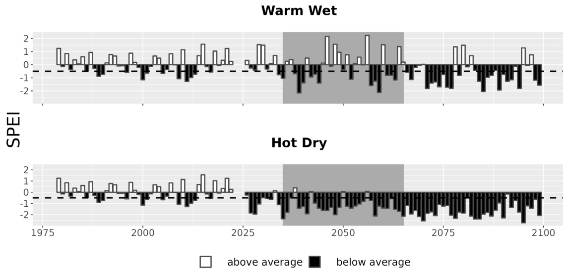
Figure 7. Drought metrics for PAIS. Drought index (SPEI; units = standard deviations from historical) timeseries for each climate future. Below-average SPEI (black bars) indicates dry conditions. The dotted line (SPEI = -0.5) indicates drought conditions.
