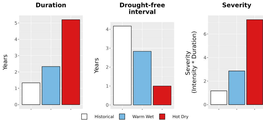
Figure 8. Drought metrics for PAIS. (Left) Average drought duration (years) historically (1979-2012) and under each climate future. (Middle) Average drought return interval (years), indicating the expected amount of time between periods of drought, historically and under each climate future. (Right) Average drought severity, a measure of drought intensity multiplied by duration, historically and under each climate future.
