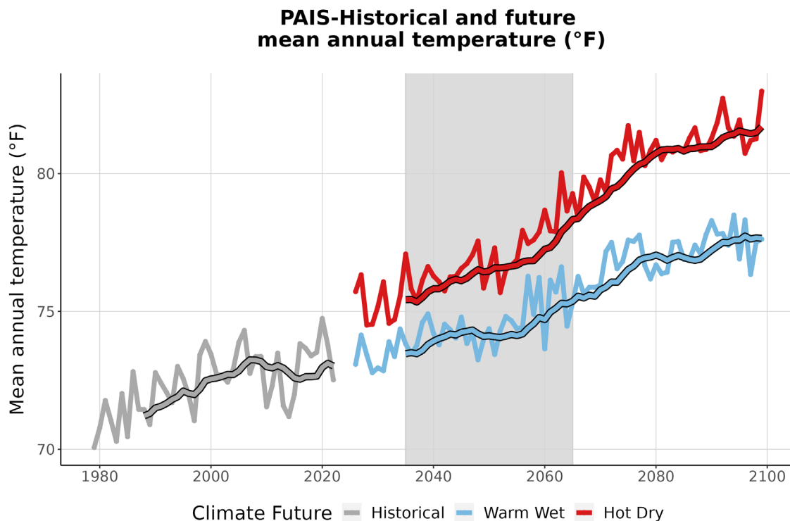
Figure 3. This graph compares observed average annual temperature at PAIS (°F) (1979-2022) with projected average annual temperature for the two climate futures over the period 2023-2099. The historically observed data
