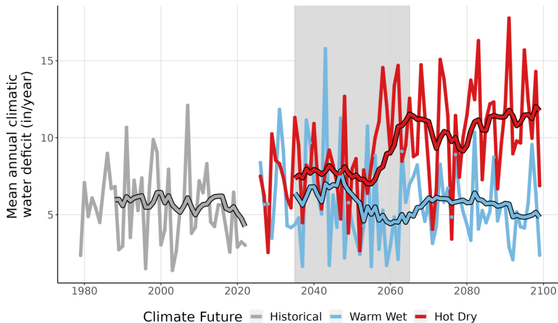
Figure 9. This line graph compares observed climatic water deficit at PAAV (inches/year) (1979-2022) with projected climatic water deficit for the two climate futures over the period 2023-2099. The historical observation data is shown in gray, the Warm Wet climate future in blue, and the Hot Dry climate future in red. The smooth line running through each projection is the 10-year running average for historical observations and future projections. Gray-shaded area represents the time period that was averaged (2035-2065) to summarize future projections for the year 2050.
