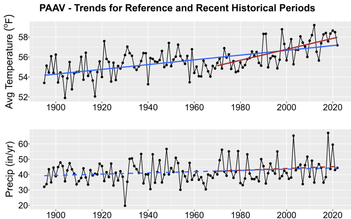
Figure 1. Historical trends in annual average temperature (upper plot) and annual total precipitation (lower plot) for PAAV from 1895-2022. Black points show yearly values while blue lines are linear regressions for the entire period record and red lines for 1970-2022 trends. Solid lines are significant trends (i.e., p < 0.05 ); dashed lines are not statistically significant.
