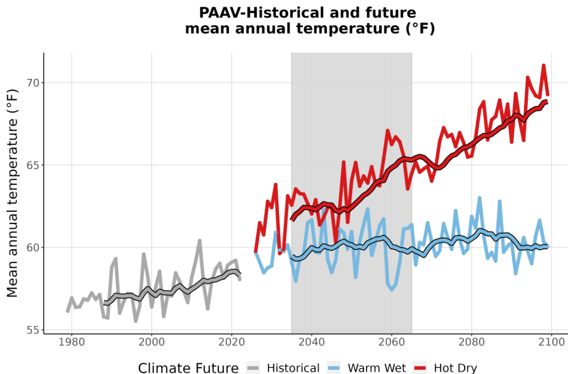
Figure 3. This graph compares observed average annual temperature at PAAV (°F) (1979-2022) with projected average annual temperature for the two climate futures over the period 2023-2099. The historically observed data
