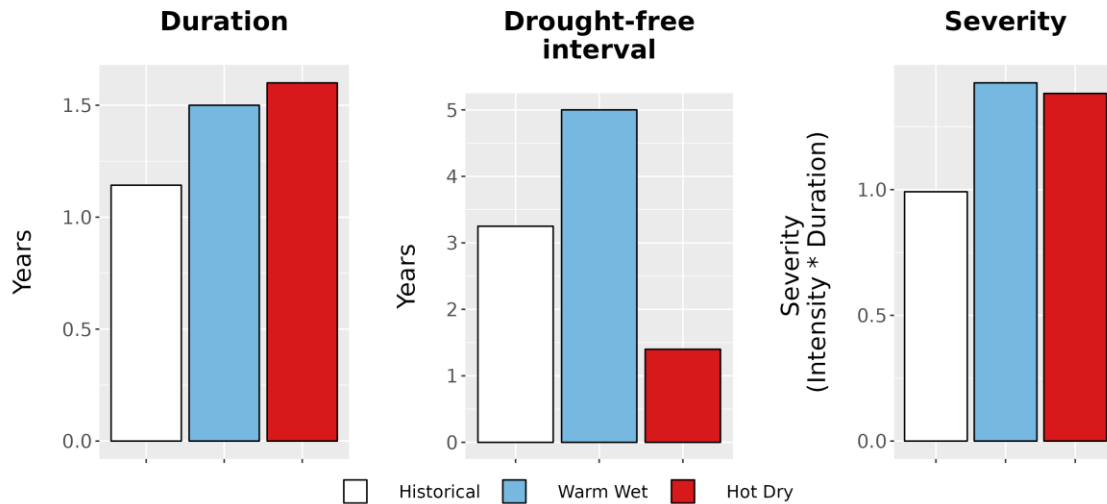
Figure 8. Drought metrics for PAAV. (Left) Average drought duration (years) historically (1979-2012) and under each climate future. (Middle) Average drought return interval (years), indicating the expected amount of time between periods of drought, historically and under each climate future. (Right) Average drought severity, a measure of drought intensity multiplied by duration, historically and under each climate future.
