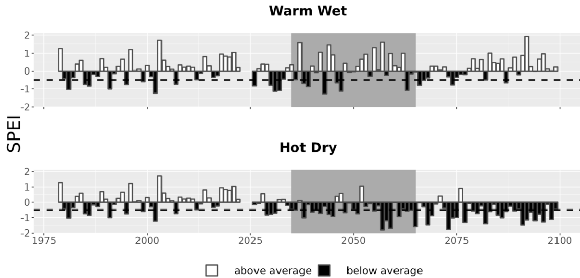
Figure 7. Drought metrics for PAAV. Drought index (SPEI; units = standard deviations from historical) timeseries for each climate future. Below-average SPEI (black bars) indicates dry conditions. The dotted line (SPEI = -0.5) indicates drought conditions.
