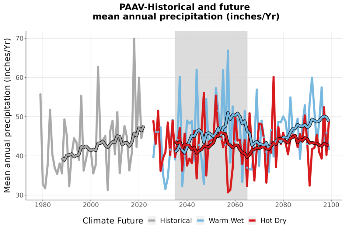
Figure 4. This graph compares observed average annual precipitation at PAAV (inches/year) (1979-2022) with projected average annual precipitation for the two climate futures over the period 2023-2099. The historically observed data is shown in gray, the Warm Wet climate future in blue, and the Hot Dry climate future in red. The smooth line running through each projection is the 10-year running average for historical observations and future projections. The gray-shaded area represents the time period that was averaged (2035-2065) to summarize future projections for the year 2050 (Appendix 1).
