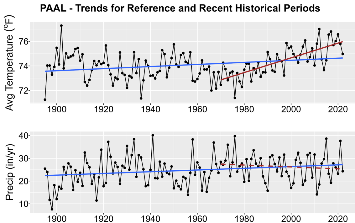
Figure 1. Historical trends in annual average temperature (upper plot) and annual total precipitation (lower plot) for PAAL from 1895-2022. Black points show yearly values while blue lines are linear regressions for the entire period record and red lines for 1970-2022 trends. Solid lines are significant trends (i.e., p < 0.05 ); dashed lines are not statistically significant.
