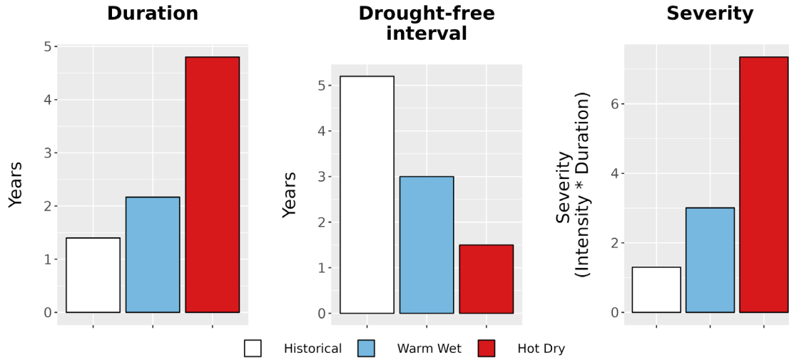
Figure 8. Drought metrics for PAAL. (Left) Average drought duration (years) historically (1979-2012) and under each climate future. (Middle) Average drought return interval (years), indicating the expected amount of time between periods of drought, historically and under each climate future. (Right) Average drought severity, a measure of drought intensity multiplied by duration, historically and under each climate future.
