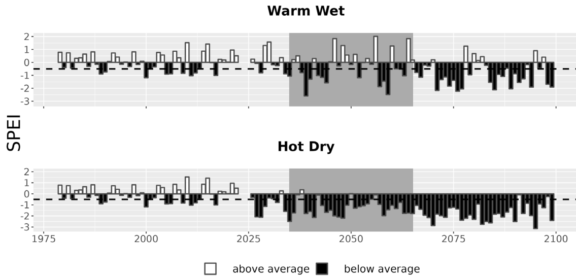
Figure 7. Drought metrics for PAAL. Drought index (SPEI; units = standard deviations from historical) timeseries for each climate future. Below-average SPEI (black bars) indicates dry conditions. The dotted line (SPEI = -0.5) indicates drought conditions.
