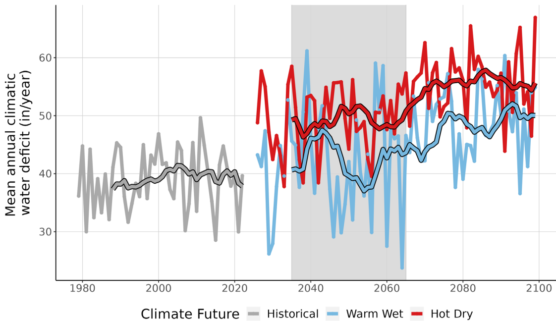
Figure 9. This line graph compares observed climatic water deficit at PAAL (inches/year) (1979-2022) with projected climatic water deficit for the two climate futures over the period 2023-2099. The historical observation data is shown in gray, the Warm Wet climate future in blue, and the Hot Dry climate future in red. The smooth line running through each projection is the 10-year running average for historical observations and future projections. Gray-shaded area represents the time period that was averaged (2035-2065) to summarize future projections for the year 2050.
