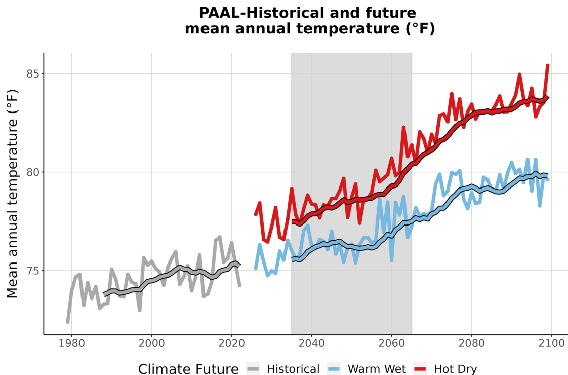
Figure 3. This graph compares observed average annual temperature at PAAL (°F) (1979-2022) with projected average annual temperature for the two climate futures over the period 2023-2099. The historically observed data
