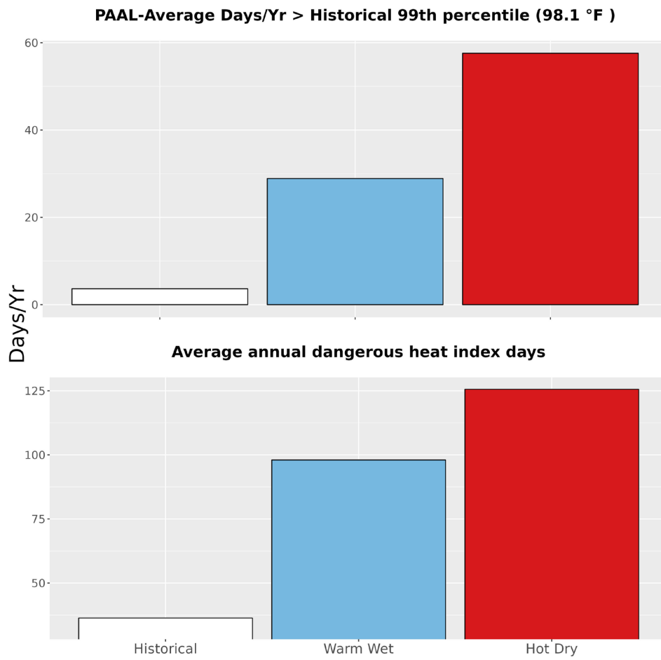
Figure 5. The upper bar graph represents the average number of days annually with temperatures greater than the historical 99th percentile (98.1 °F) historically (1979-2012) and for the two climate futures (2050). The bottom bar graph represents the average annual number of dangerous heat index days historically and for the two climate futures. Dangerous heat index days are days that exceed 105 °F.
