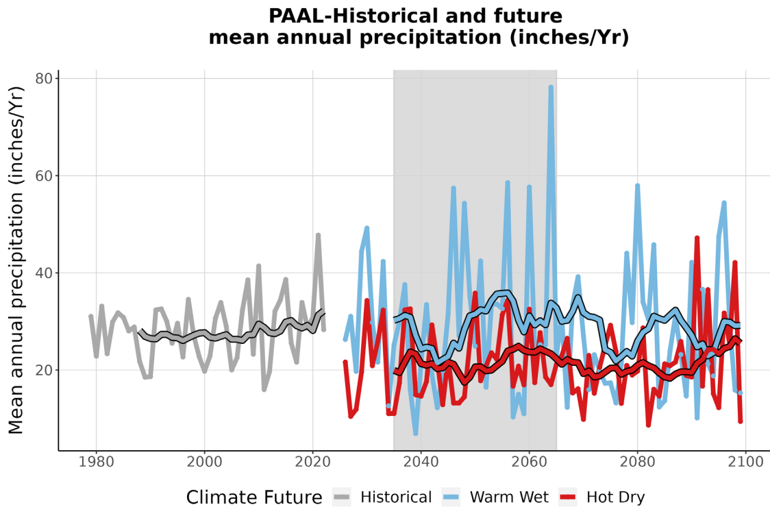
Figure 4. This graph compares observed average annual precipitation at PAAL (inches/year) (1979-2022) with projected average annual precipitation for the two climate futures over the period 2023-2099. The historically observed data is shown in gray, the Warm Wet climate future in blue, and the Hot Dry climate future in red. The smooth line running through each projection is the 10-year running average for historical observations and future projections. The gray-shaded area represents the time period that was averaged (2035-2065) to summarize future projections for the year 2050 (Appendix 1).
