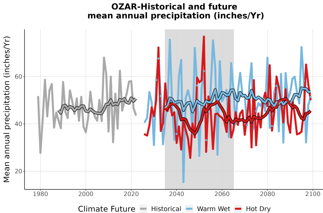
Figure 4. This graph compares observed average annual precipitation at OZAR (inches/year) (1979-2022) with projected average annual precipitation for the two climate futures over the period 2023-2099. The historically observed data is shown in gray, the Warm Wet climate future in blue, and the Hot Dry climate future in red. The smooth line running through each projection is the 10-year running average for historical observations and future projections. The gray-shaded area represents the time period that was averaged (2035-2065) to summarize future projections for the year 2050 (Appendix 1).
