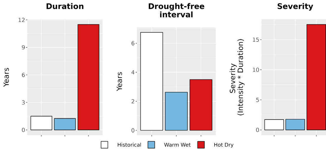
Figure 8. Drought metrics for OZAR. (Left) Average drought duration (years) historically (1979-2012) and under each climate future. (Middle) Average drought return interval (years), indicating the expected amount of time between periods of drought, historically and under each climate future. (Right) Average drought severity, a measure of drought intensity multiplied by duration, historically and under each climate future.
