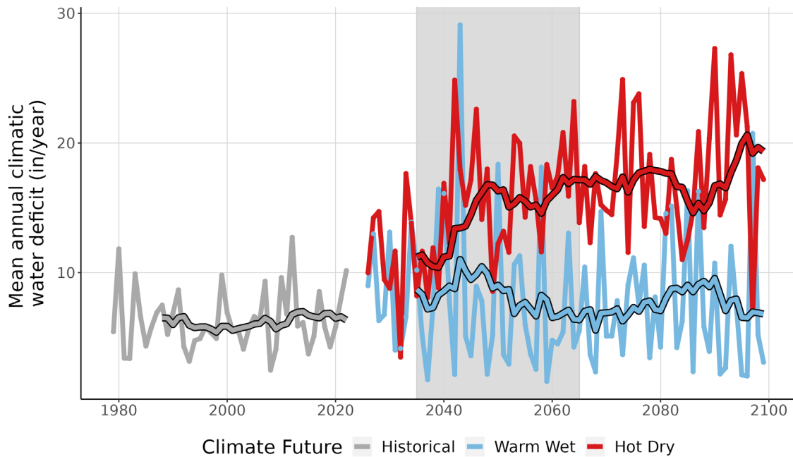
Figure 9. This line graph compares observed climatic water deficit at OZAR (inches/year) (1979-2022) with projected climatic water deficit for the two climate futures over the period 2023-2099. The historical observation data is shown in gray, the Warm Wet climate future in blue, and the Hot Dry climate future in red. The smooth line running through each projection is the 10-year running average for historical observations and future projections. Gray-shaded area represents the time period that was averaged (2035-2065) to summarize future projections for the year 2050.
