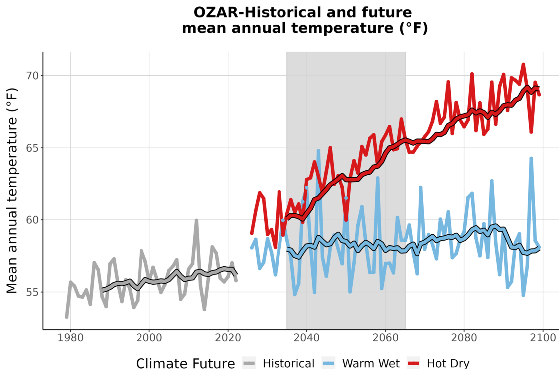
Figure 3. This graph compares observed average annual temperature at OZAR (°F) (1979-2022) with projected average annual temperature for the two climate futures over the period 2023-2099. The historically observed data
