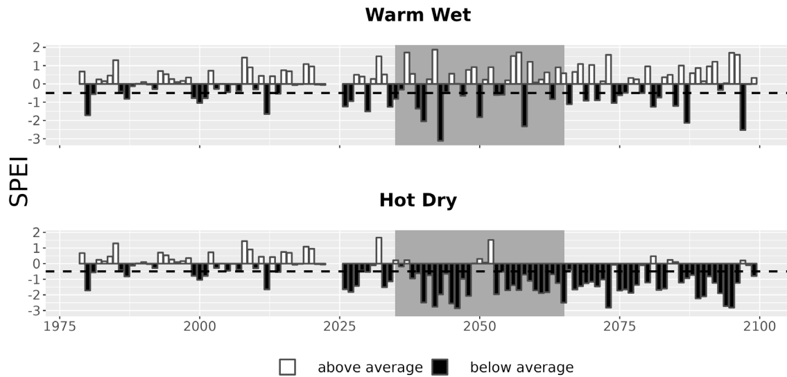
Figure 7. Drought metrics for OZAR. Drought index (SPEI; units = standard deviations from historical) timeseries for each climate future. Below-average SPEI (black bars) indicates dry conditions. The dotted line (SPEI = -0.5) indicates drought conditions.
