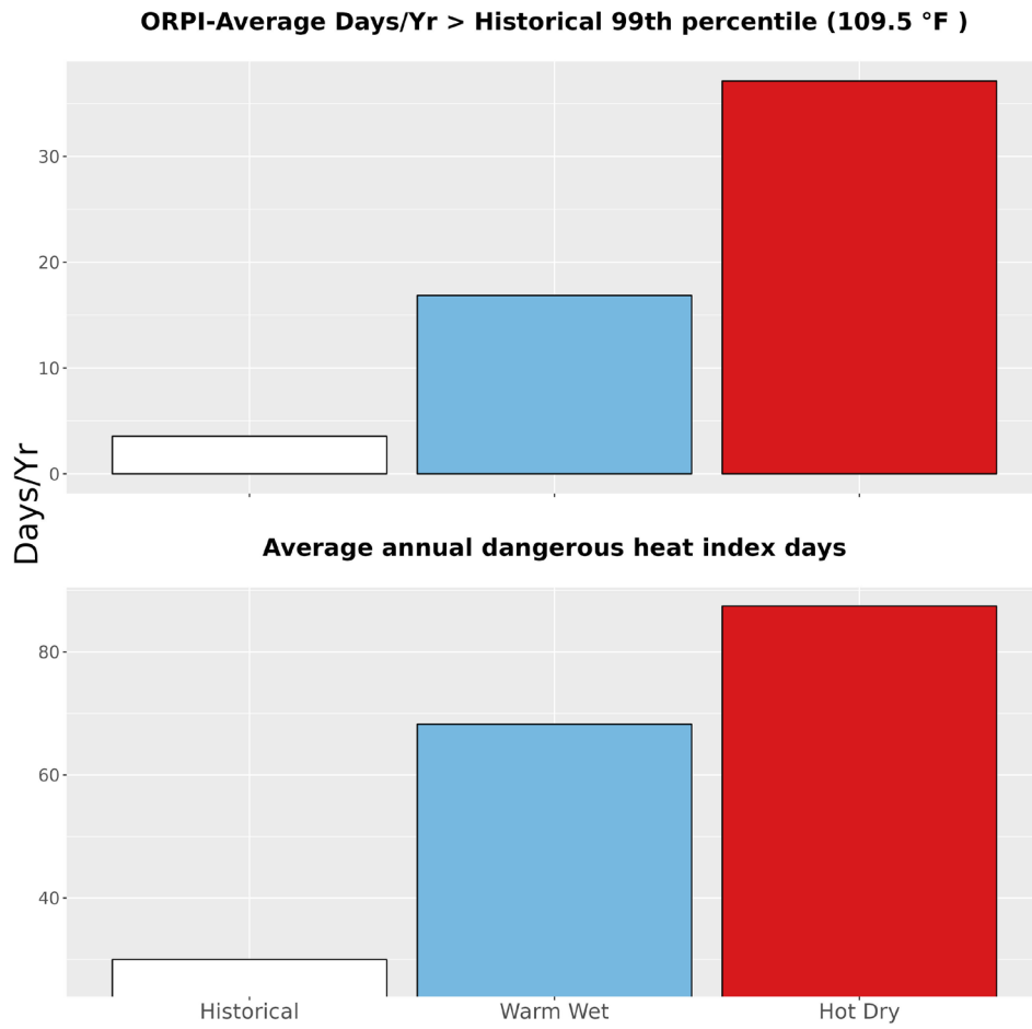
Figure 5. The upper bar graph represents the average number of days annually with temperatures greater than the historical 99th percentile (109.5 °F) historically (1979-2012) and for the two climate futures (2050). The bottom bar graph represents the average annual number of dangerous heat index days historically and for the two climate futures. Dangerous heat index days are days that exceed 105 °F.
