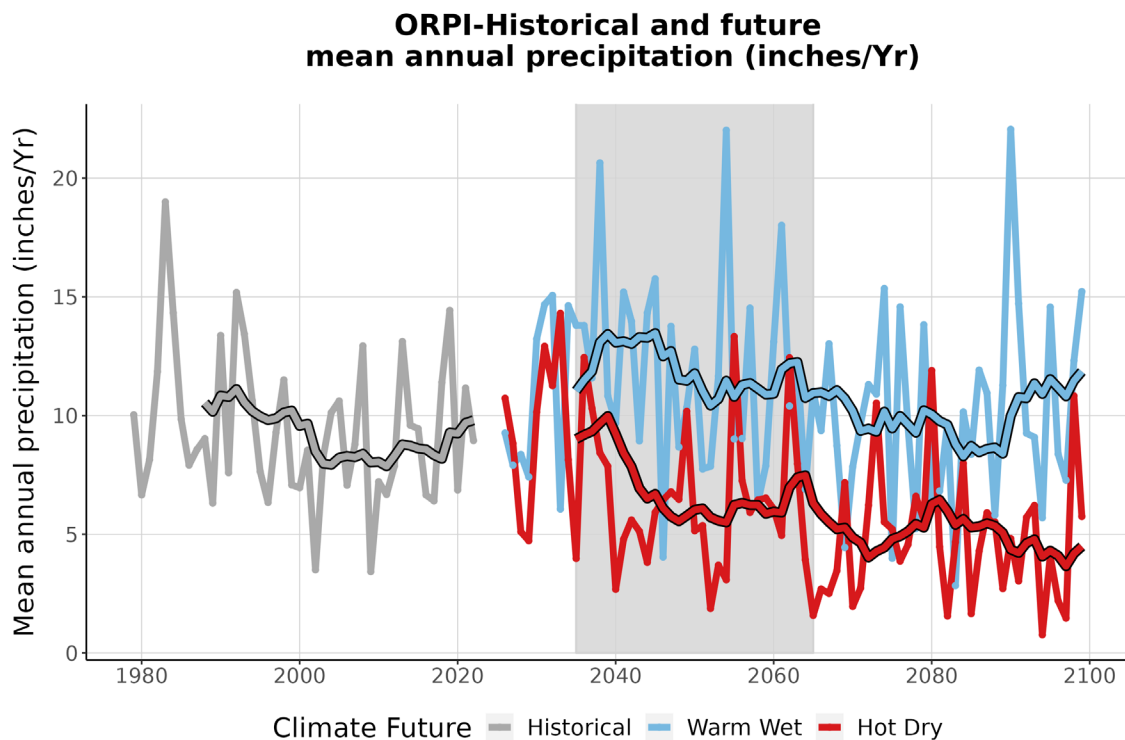
Figure 4. This graph compares observed average annual precipitation at ORPI (inches/year) (1979-2022) with projected average annual precipitation for the two climate futures over the period 2023-2099. The historically observed data is shown in gray, the Warm Wet climate future in blue, and the Hot Dry climate future in red. The smooth line running through each projection is the 10-year running average for historical observations and future projections. The gray-shaded area represents the time period that was averaged (2035-2065) to summarize future projections for the year 2050 (Appendix 1).
