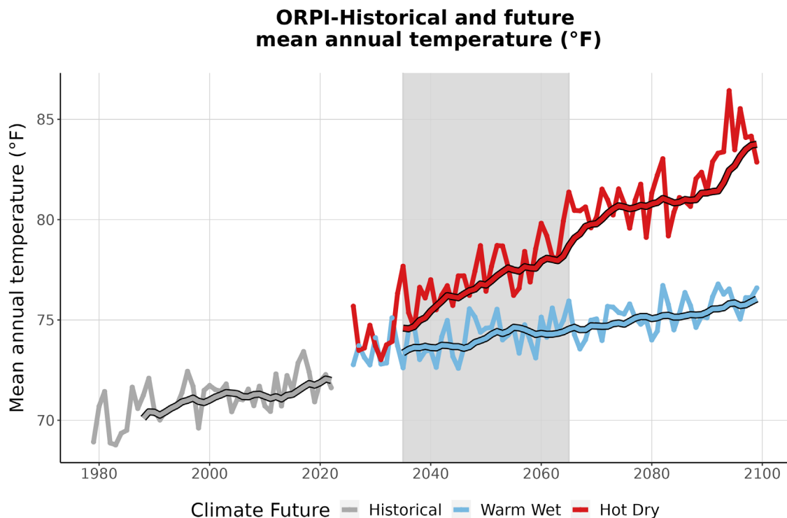
Figure 3. This graph compares observed average annual temperature at ORPI (°F) (1979-2022) with projected average annual temperature for the two climate futures over the period 2023-2099. The historically observed data
