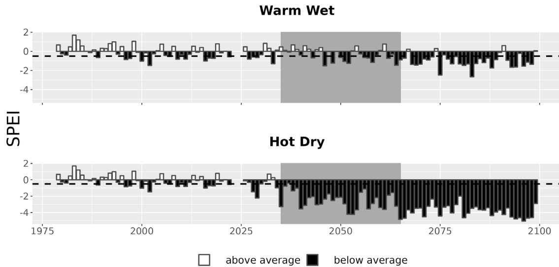
Figure 7. Drought metrics for ORPI. Drought index (SPEI; units = standard deviations from historical) timeseries for each climate future. Below-average SPEI (black bars) indicates dry conditions. The dotted line (SPEI = -0.5) indicates drought conditions.
