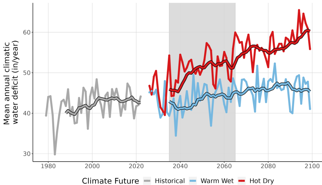
Figure 9. This line graph compares observed climatic water deficit at ORPI (inches/year) (1979-2022) with projected climatic water deficit for the two climate futures over the period 2023-2099. The historical observation data is shown in gray, the Warm Wet climate future in blue, and the Hot Dry climate future in red. The smooth line running through each projection is the 10-year running average for historical observations and future projections. Gray-shaded area represents the time period that was averaged (2035-2065) to summarize future projections for the year 2050.
