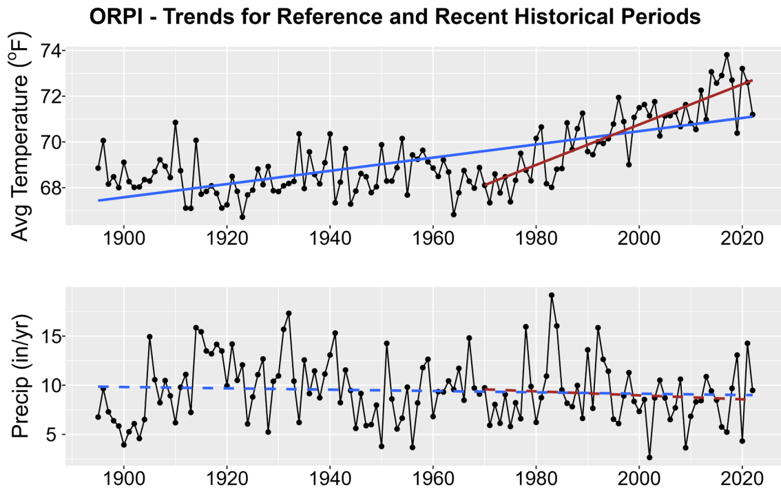
Figure 1. Historical trends in annual average temperature (upper plot) and annual total precipitation (lower plot) for ORPI from 1895-2022. Black points show yearly values while blue lines are linear regressions for the entire period record and red lines for 1970-2022 trends. Solid lines are significant trends (i.e., p < 0.05 ); dashed lines are not statistically significant.
