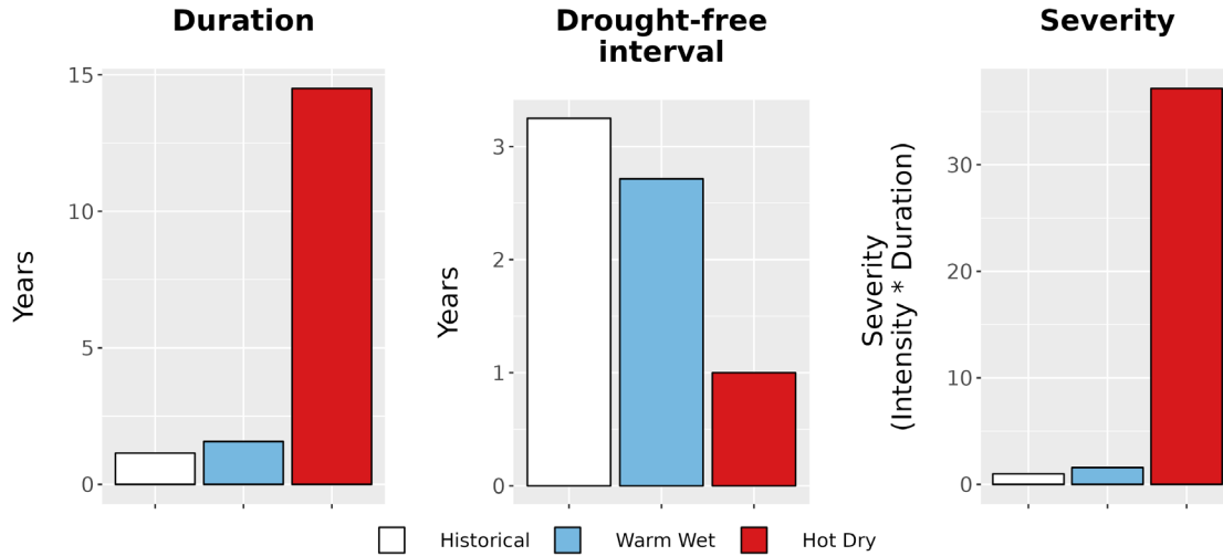
Figure 8. Drought metrics for ORPI. (Left) Average drought duration (years) historically (1979-2012) and under each climate future. (Middle) Average drought return interval (years), indicating the expected amount of time between periods of drought, historically and under each climate future. (Right) Average drought severity, a measure of drought intensity multiplied by duration, historically and under each climate future.
