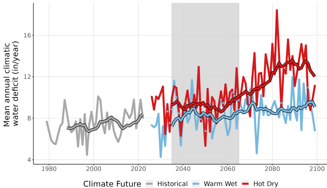
Figure 9. This line graph compares observed climatic water deficit at ORCA (inches/year) (1979-2022) with projected climatic water deficit for the two climate futures over the period 2023-2099. The historical observation data is shown in gray, the Warm Wet climate future in blue, and the Hot Dry climate future in red. The smooth line running through each projection is the 10-year running average for historical observations and future projections. Gray-shaded area represents the time period that was averaged (2035-2065) to summarize future projections for the year 2050.
