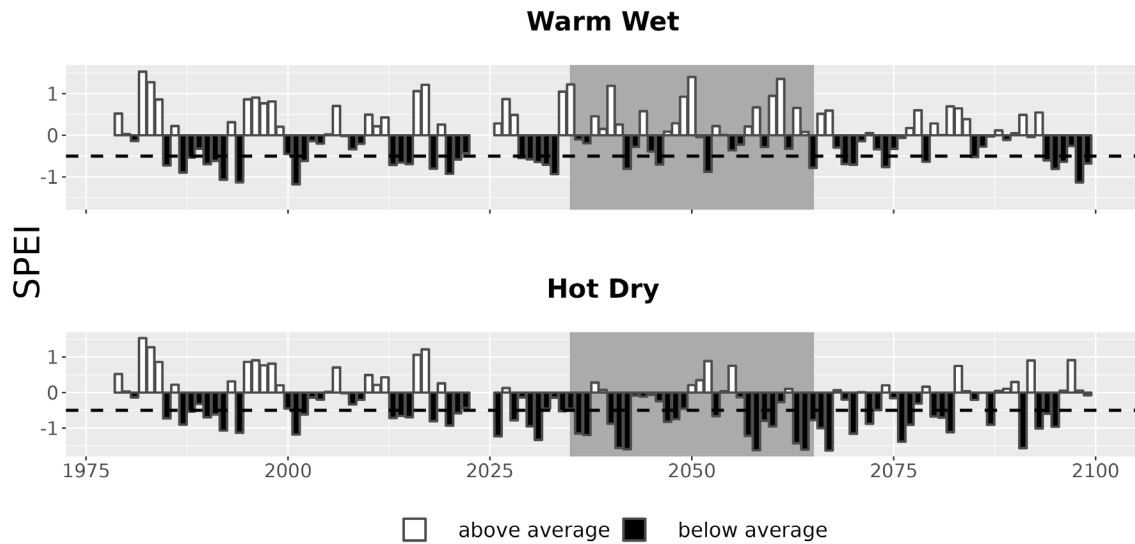
Figure 7. Drought metrics for ORCA. Drought index (SPEI; units = standard deviations from historical) timeseries for each climate future. Below-average SPEI (black bars) indicates dry conditions. The dotted line (SPEI = -0.5) indicates drought conditions.
