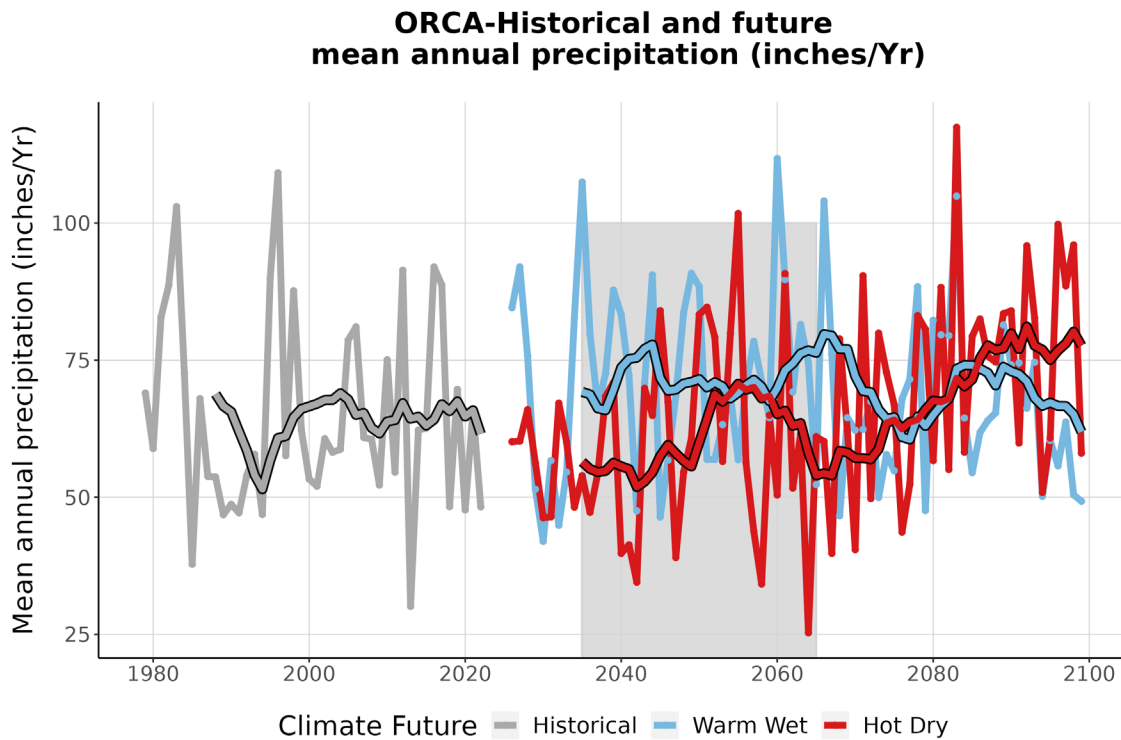
Figure 4. This graph compares observed average annual precipitation at ORCA (inches/year) (1979-2022) with projected average annual precipitation for the two climate futures over the period 2023-2099. The historically observed data is shown in gray, the Warm Wet climate future in blue, and the Hot Dry climate future in red. The smooth line running through each projection is the 10-year running average for historical observations and future projections. The gray-shaded area represents the time period that was averaged (2035-2065) to summarize future projections for the year 2050 (Appendix 1).
