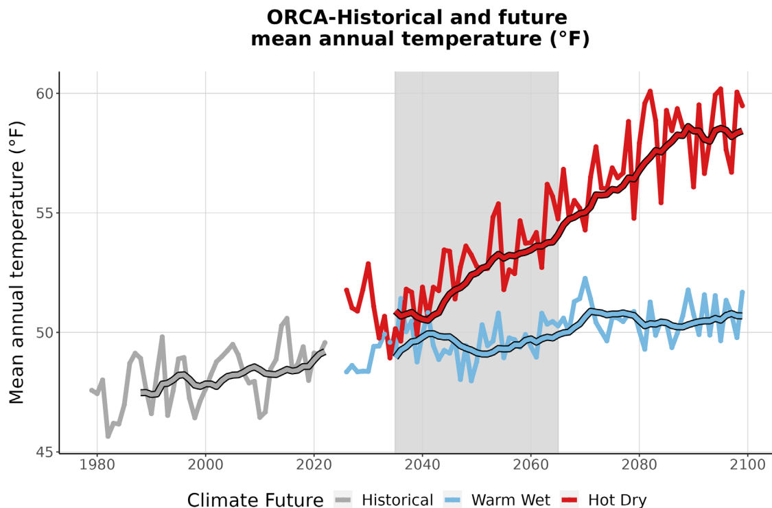
Figure 3. This graph compares observed average annual temperature at ORCA (°F) (1979-2022) with projected average annual temperature for the two climate futures over the period 2023-2099. The historically observed data
