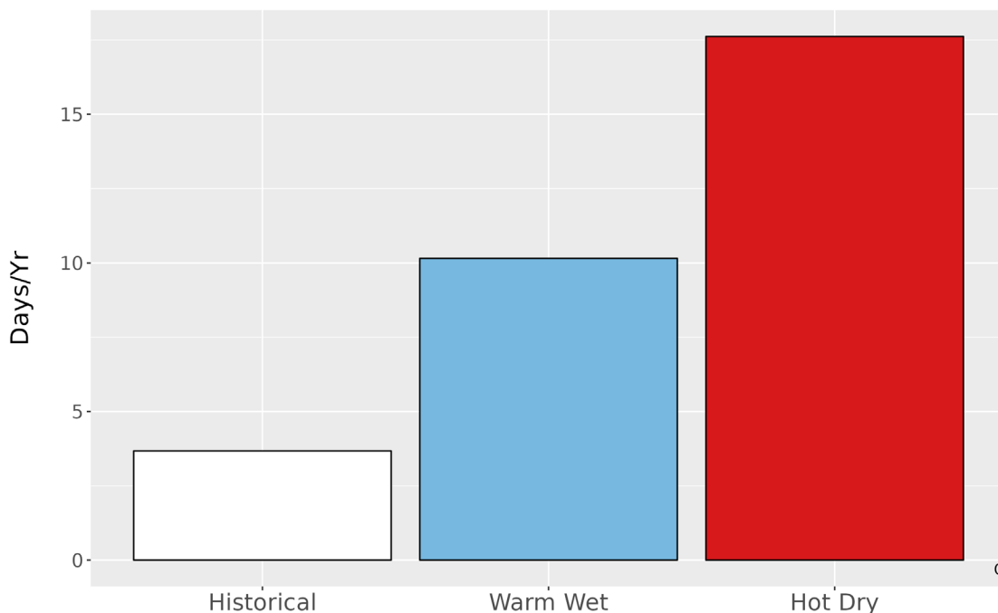
Figure 5. Metrics of extreme temperature at ORCA. The bar graph represents the average number of days annually with temperatures greater than the historical 99th percentile (88.8 °F) historically (1979-2012) and for the two climate futures (2050).
