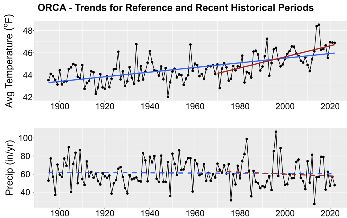
Figure 1. Historical trends in annual average temperature (upper plot) and annual total precipitation (lower plot) for ORCA from 1895-2022. Black points show yearly values while blue lines are linear regressions for the entire period record and red lines for 1970-2022 trends. Solid lines are significant trends (i.e., p < 0.05 ); dashed lines are not statistically significant.
