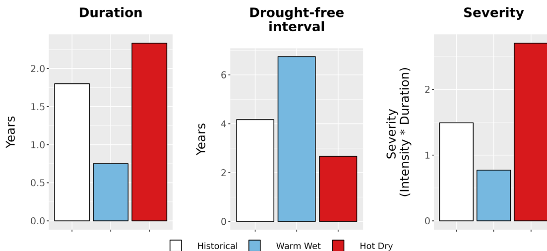
Figure 8. Drought metrics for ORCA. (Left) Average drought duration (years) historically (1979-2012) and under each climate future. (Middle) Average drought return interval (years), indicating the expected amount of time between periods of drought, historically and under each climate future. (Right) Average drought severity, a measure of drought intensity multiplied by duration, historically and under each climate future.
