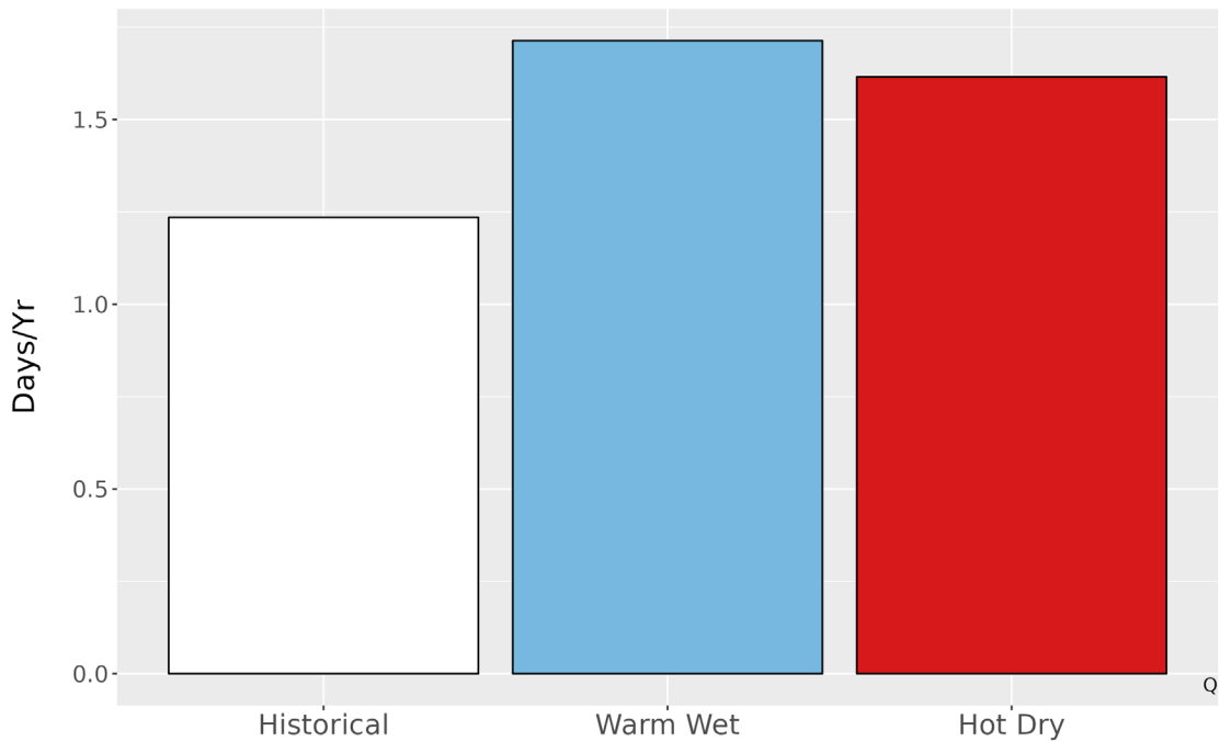
Figure 6. Average number of days annually with precipitation exceeding the 99th percentile (3.1 in.) of precipitation from the historical period 1979-2012 and for each climate future.
