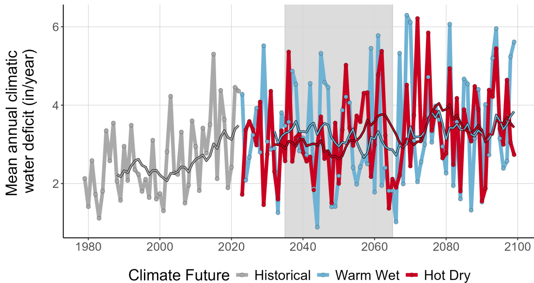
Figure 9. This line graph compares observed climatic water deficit at OLYM (inches/year) (1979-2022) with projected climatic water deficit for the two climate futures over the period 2023-2099. The historical observation data is shown in gray, the Warm Wet climate future in blue, and the Hot Dry climate future in red. The smooth line running through each projection is the 10-year running average for historical observations and future projections. Gray-shaded area represents the time period that was averaged (2035-2065) to summarize future projections for the year 2050.
