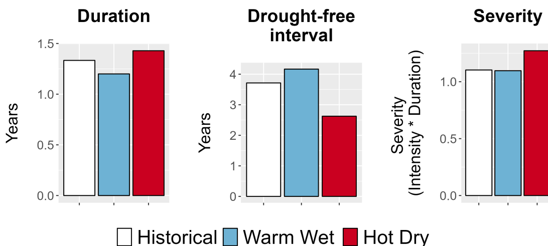
Figure 8. Drought metrics for OLYM. (Left) Average drought duration (years) historically (1979-2012) and under each climate future. (Middle) Average drought return interval (years), indicating the expected amount of time between periods of drought, historically and under each climate future. (Right) Average drought severity, a measure of drought intensity multiplied by duration, historically and under each climate future.
