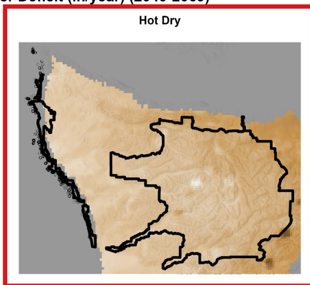
Figure A3. (Top) Map showing average annual climatic water deficit for the historical period (inches/year) and (bottom) change in average annual climatic water deficit for the two climate futures. Legends are located below each set of maps as a continuous color gradient. Gridded data is extracted from 30-year summary GIS layers for CONUS water balance model (Tercek et al 2021, 2023). ( http://screenedcleanedsummaries.s3-website-us-west-2.amazonaws.com/ ) accessed on 6/3/2024.
