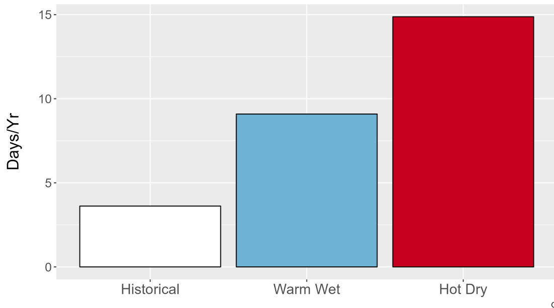
Figure 5. Metrics of extreme temperature at OLYM. The bar graph represents the average number of days annually with temperatures greater than the historical 99th percentile (86.3 °F) historically (1979-2012) and for the two climate futures (2050).
