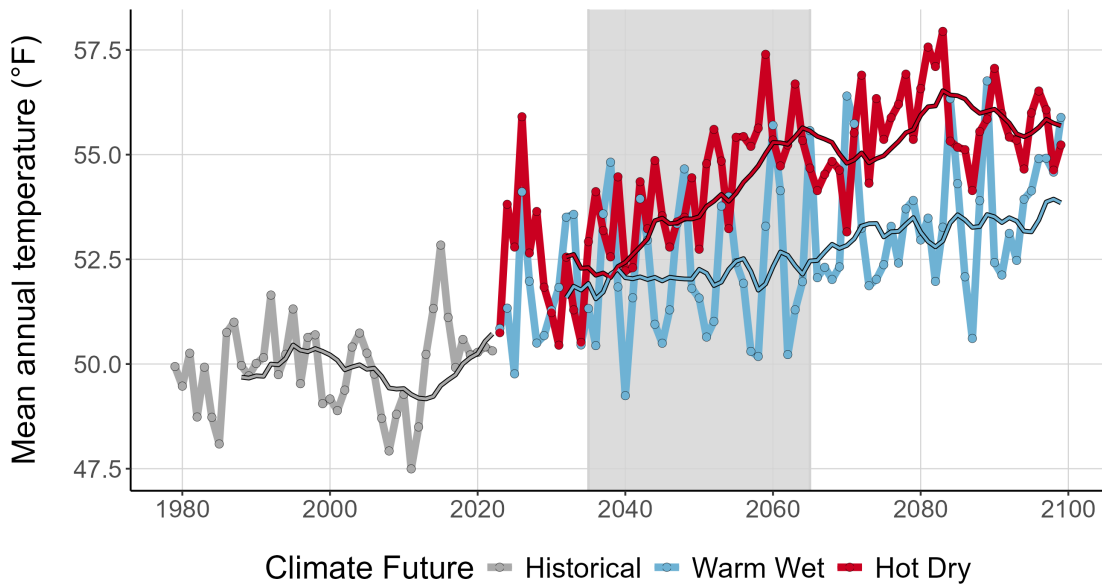
Figure 3. This graph compares observed average annual temperature at OLYM (°F) (1979-2022) with projected average annual temperature for the two climate futures over the period 2023-2099. The historically observed data is shown in gray, the Warm Wet climate future in blue, and the Hot Dry climate future in red. The smooth line running through each projection is the 10-year running average for historical observations and future projections. Gray-shaded area represents the time period that was averaged (2035-2065) to summarize future projections for the year 2050 (Appendix 1).
