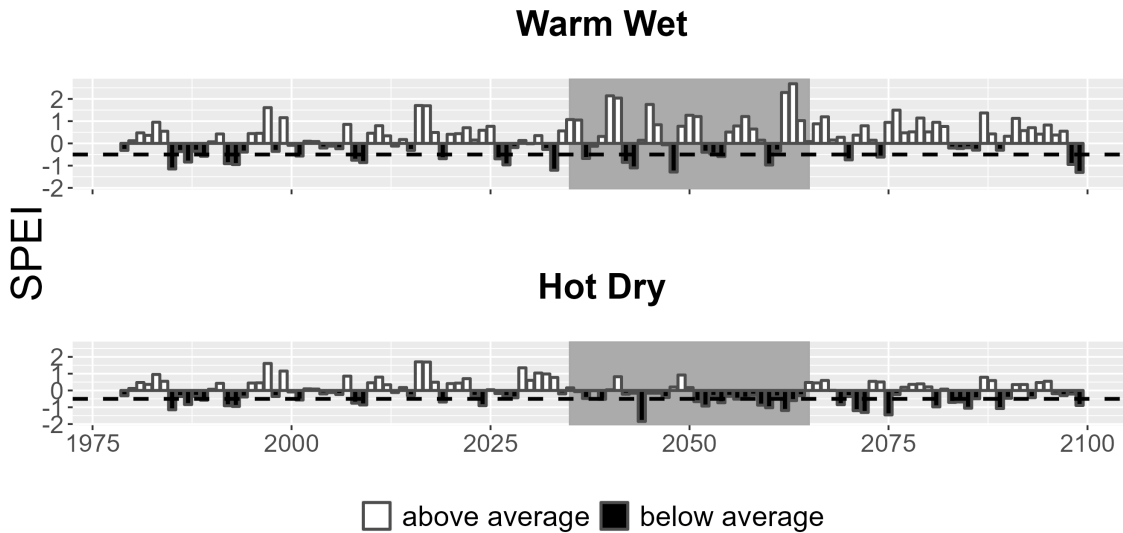
Figure 7. Drought metrics for OLYM. Drought index (SPEI; units = standard deviations from historical) timeseries for each climate future. Below-average SPEI (black bars) indicates dry conditions. The dotted line (SPEI = -0.5) indicates drought conditions.
