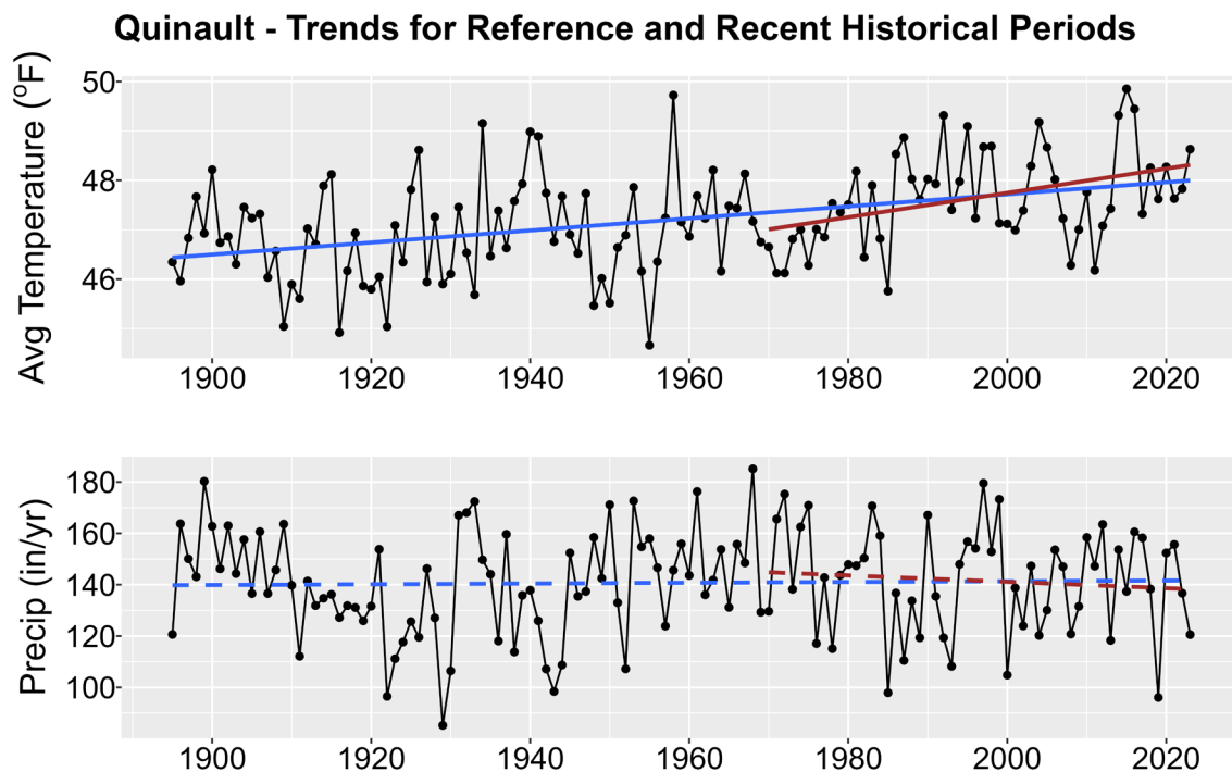
Figure 1. Historical trends in annual average temperature (upper plot) and annual total precipitation (lower plot) for OLYM from 1895-2022. Black points show yearly values while blue lines are linear regressions for the entire period record and red lines for 1970-2022 trends. Solid lines are significant trends (i.e., p < 0.05 ); dashed lines are not statistically significant.
