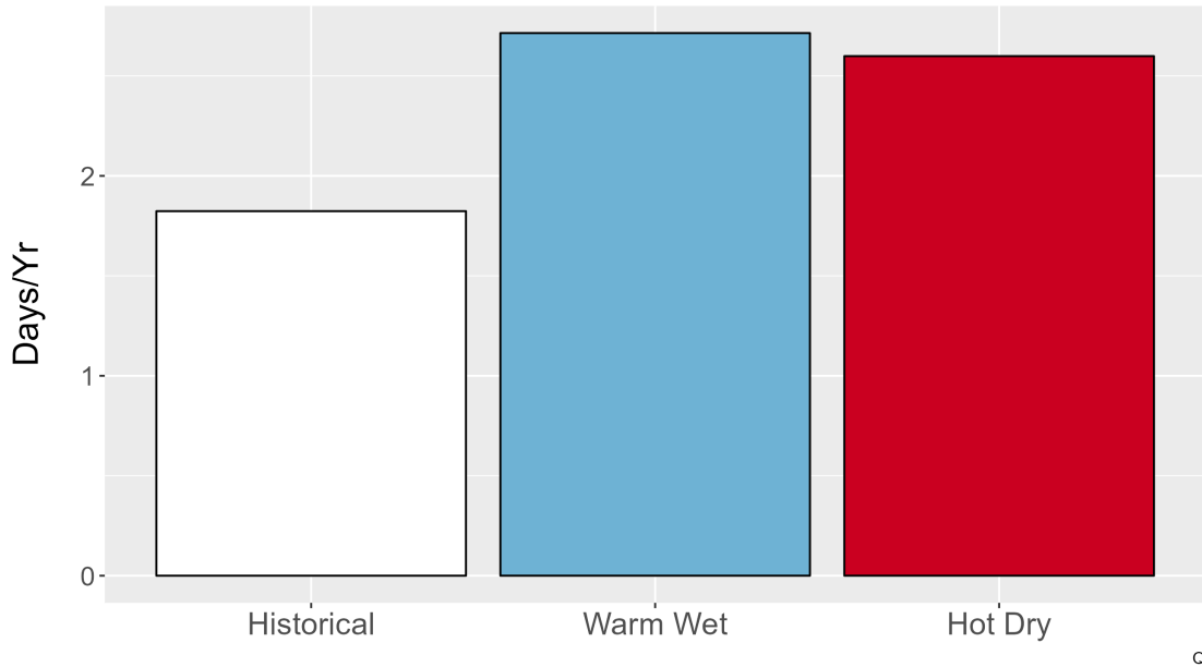
Figure 6. Average number of days annually with precipitation exceeding the 99th percentile (3.6 in.) of precipitation from the historical period 1979-2012 and for each climate future.
