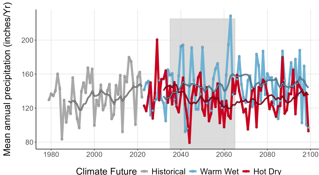
Figure 4. This graph compares observed average annual precipitation at OLYM (inches/year) (1979-2022) with projected average annual precipitation for the two climate futures over the period 2023-2099. The historically observed data is shown in gray, the Warm Wet climate future in blue, and the Hot Dry climate future in red. The smooth line running through each projection is the 10-year running average for historical observations and future projections. The gray-shaded area represents the time period that was averaged (2035-2065) to summarize future projections for the year 2050 (Appendix 1).
