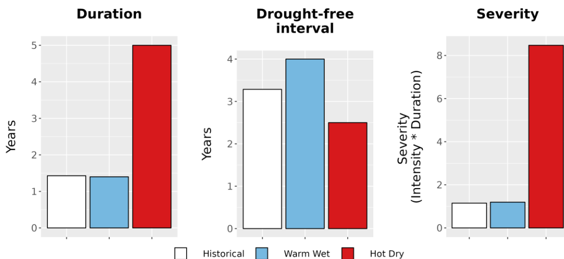
Figure 8. Drought metrics for OCMU. (Left) Average drought duration (years) historically (1979-2012) and under each climate future. (Middle) Average drought return interval (years), indicating the expected amount of time between periods of drought, historically and under each climate future. (Right) Average drought severity, a measure of drought intensity multiplied by duration, historically and under each climate future.
