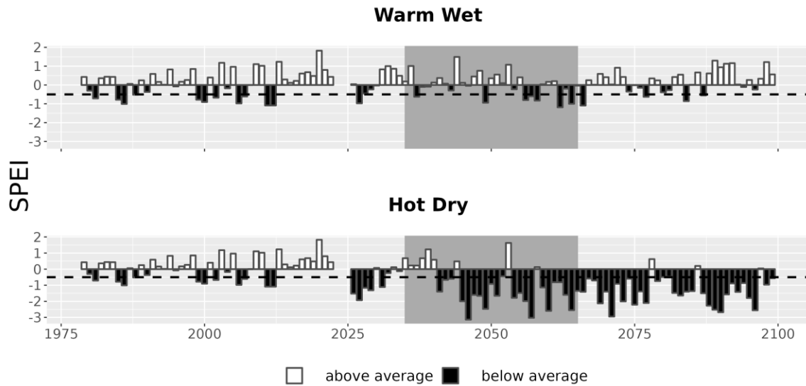
Figure 7. Drought metrics for OCMU. Drought index (SPEI; units = standard deviations from historical) timeseries for each climate future. Below-average SPEI (black bars) indicates dry conditions. The dotted line (SPEI = -0.5) indicates drought conditions.
