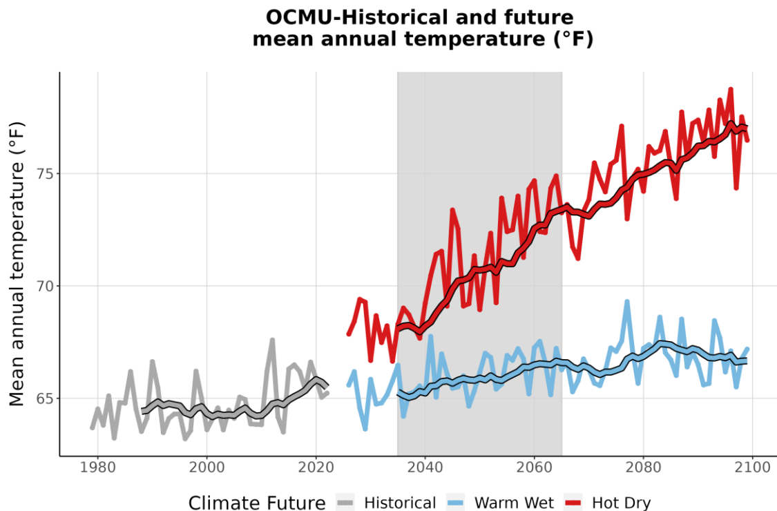
Figure 3. This graph compares observed average annual temperature at OCMU (°F) (1979-2022) with projected average annual temperature for the two climate futures over the period 2023-2099. The historically observed data
