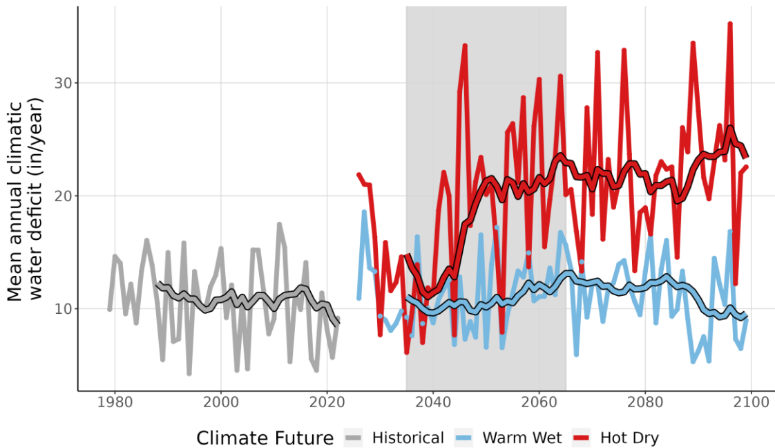
Figure 9. This line graph compares observed climatic water deficit at OCMU (inches/year) (1979-2022) with projected climatic water deficit for the two climate futures over the period 2023-2099. The historical observation data is shown in gray, the Warm Wet climate future in blue, and the Hot Dry climate future in red. The smooth line running through each projection is the 10-year running average for historical observations and future projections. Gray-shaded area represents the time period that was averaged (2035-2065) to summarize future projections for the year 2050.
