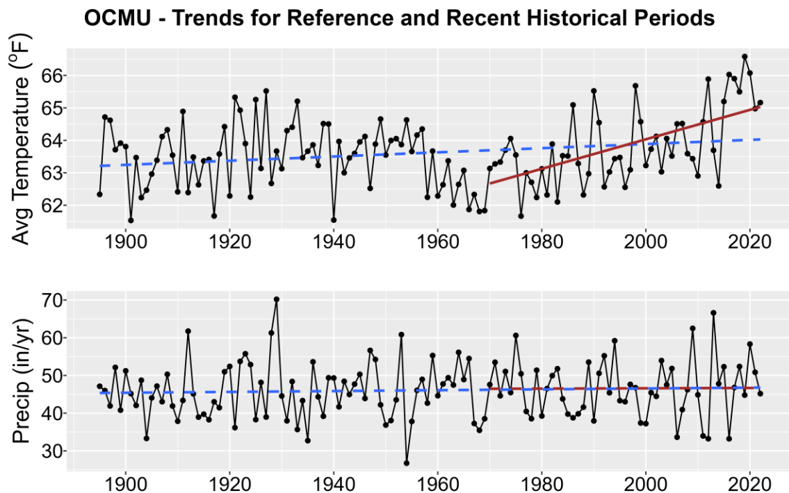
Figure 1. Historical trends in annual average temperature (upper plot) and annual total precipitation (lower plot) for OCMU from 1895-2022. Black points show yearly values while blue lines are linear regressions for the entire period record and red lines for 1970-2022 trends. Solid lines are significant trends (i.e., p < 0.05 ); dashed lines are not statistically significant.
