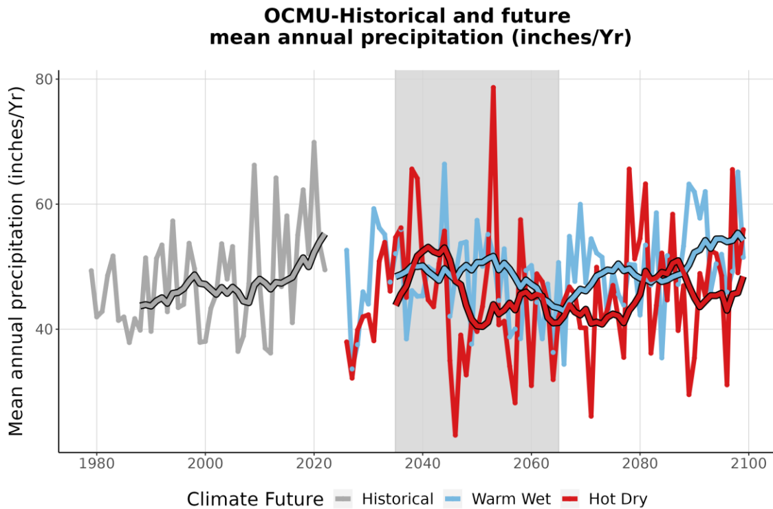
Figure 4. This graph compares observed average annual precipitation at OCMU (inches/year) (1979-2022) with projected average annual precipitation for the two climate futures over the period 2023-2099. The historically observed data is shown in gray, the Warm Wet climate future in blue, and the Hot Dry climate future in red. The smooth line running through each projection is the 10-year running average for historical observations and future projections. The gray-shaded area represents the time period that was averaged (2035-2065) to summarize future projections for the year 2050 (Appendix 1).
