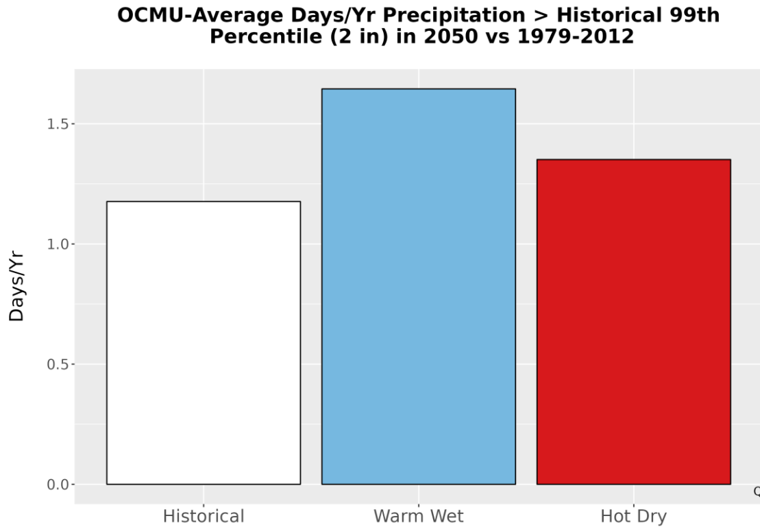
Figure 6. Average number of days annually with precipitation exceeding the 99th percentile (2 in.) of precipitation from the historical period 1979-2012 and for each climate future.
