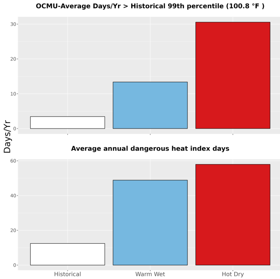
Figure 5. The upper bar graph represents the average number of days annually with temperatures greater than the historical 99th percentile (100.8 °F) historically (1979-2012) and for the two climate futures (2050). The bottom bar graph represents the average annual number of dangerous heat index days historically and for the two climate futures. Dangerous heat index days are days that exceed 105 °F.
