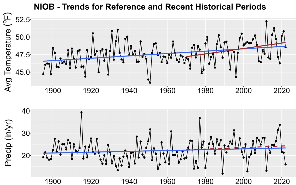
Figure 1. Historical trends in annual average temperature (upper plot) and annual total precipitation (lower plot) for NIOB from 1895-2022. Black points show yearly values while blue lines are linear regressions for the entire period record and red lines for 1970-2022 trends. Solid lines are significant trends (i.e., p < 0.05 ); dashed lines are not statistically significant.
