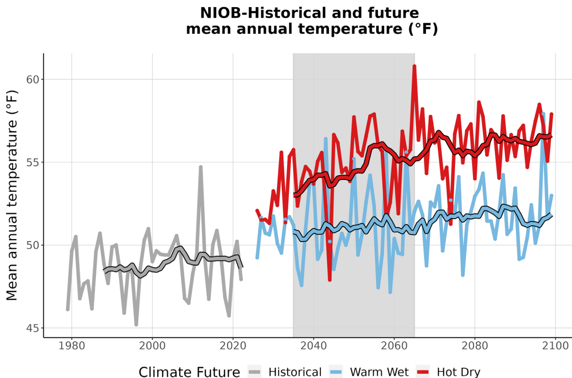
Figure 3. This graph compares observed average annual temperature at NIOB (°F) (1979-2022) with projected average annual temperature for the two climate futures over the period 2023-2099. The historically observed data
