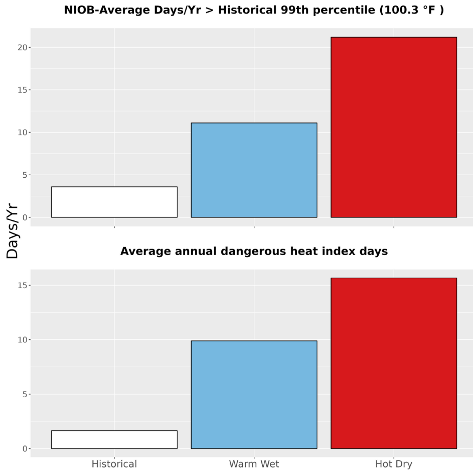
Figure 5. The upper bar graph represents the average number of days annually with temperatures greater than the historical 99th percentile (100.3 °F) historically (1979-2012) and for the two climate futures (2050). The bottom bar graph represents the average annual number of dangerous heat index days historically and for the two climate futures. Dangerous heat index days are days that exceed 105 °F.
