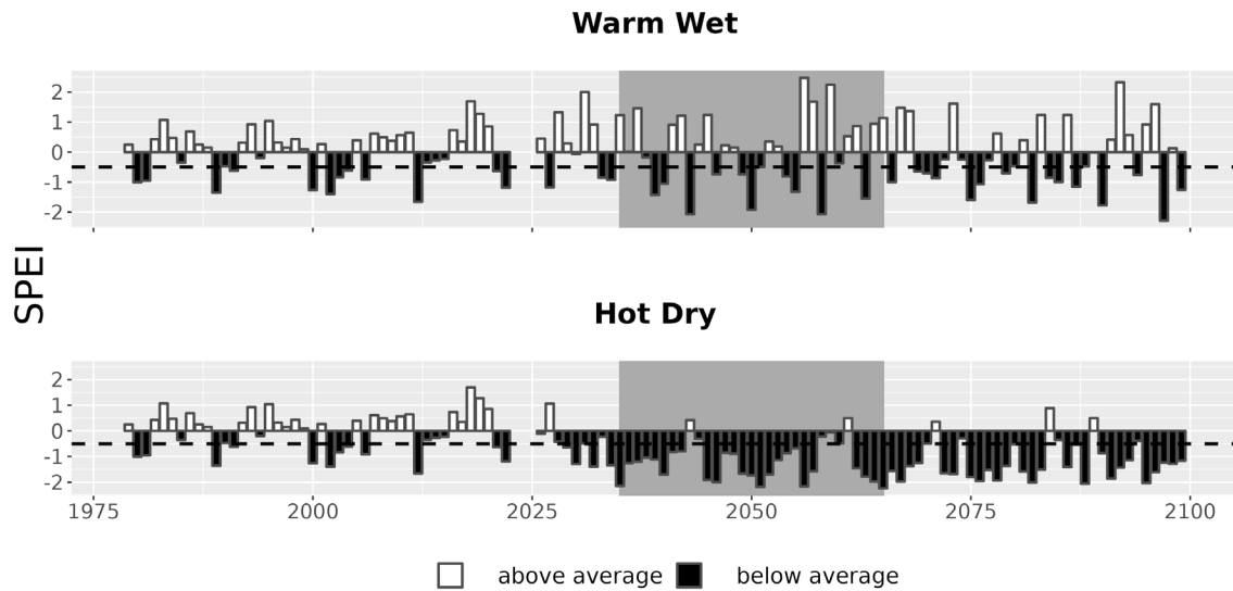
Figure 7. Drought metrics for NIOB. Drought index (SPEI; units = standard deviations from historical) timeseries for each climate future. Below-average SPEI (black bars) indicates dry conditions. The dotted line (SPEI = -0.5) indicates drought conditions.
