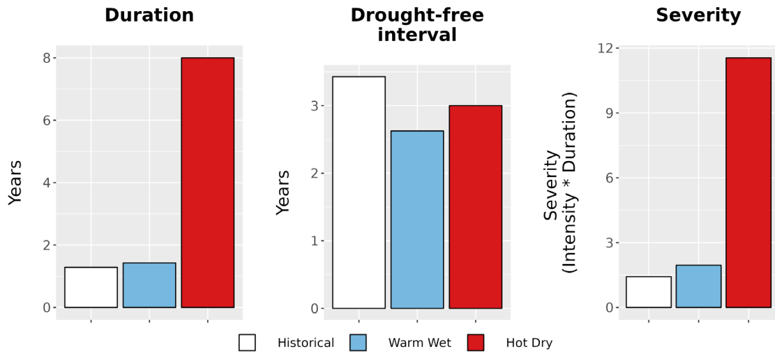
Figure 8. Drought metrics for NIOB. (Left) Average drought duration (years) historically (1979-2012) and under each climate future. (Middle) Average drought return interval (years), indicating the expected amount of time between periods of drought, historically and under each climate future. (Right) Average drought severity, a measure of drought intensity multiplied by duration, historically and under each climate future.
