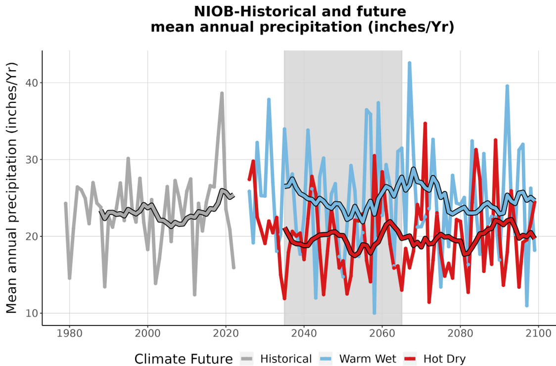
Figure 4. This graph compares observed average annual precipitation at NIOB (inches/year) (1979-2022) with projected average annual precipitation for the two climate futures over the period 2023-2099. The historically observed data is shown in gray, the Warm Wet climate future in blue, and the Hot Dry climate future in red. The smooth line running through each projection is the 10-year running average for historical observations and future projections. The gray-shaded area represents the time period that was averaged (2035-2065) to summarize future projections for the year 2050 (Appendix 1).
