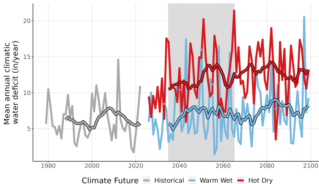
Figure 9. This line graph compares observed climatic water deficit at NIOB (inches/year) (1979-2022) with projected climatic water deficit for the two climate futures over the period 2023-2099. The historical observation data is shown in gray, the Warm Wet climate future in blue, and the Hot Dry climate future in red. The smooth line running through each projection is the 10-year running average for historical observations and future projections. Gray-shaded area represents the time period that was averaged (2035-2065) to summarize future projections for the year 2050.
