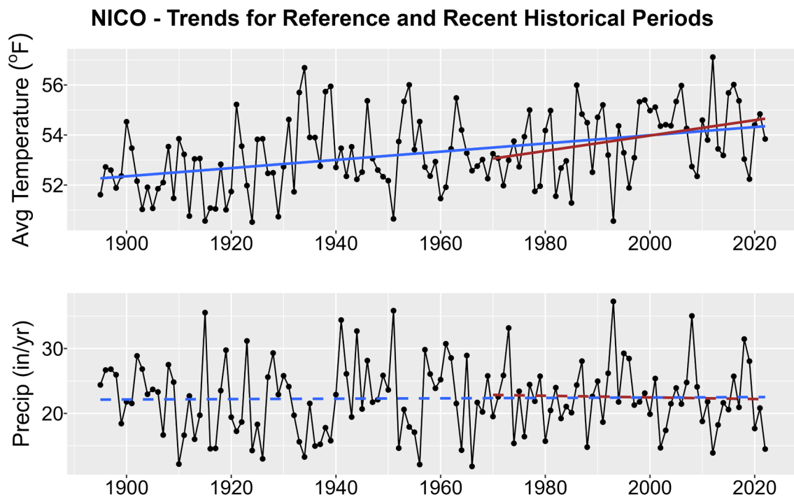
Figure 1. Historical trends in annual average temperature (upper plot) and annual total precipitation (lower plot) for NICO from 1895-2022. Black points show yearly values while blue lines are linear regressions for the entire period record and red lines for 1970-2022 trends. Solid lines are significant trends (i.e., p < 0.05 ); dashed lines are not statistically significant.
