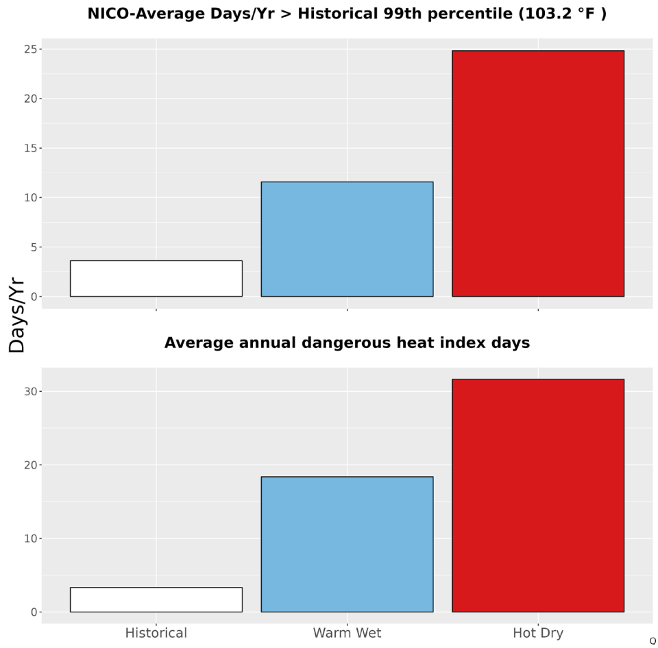
Figure 5. The upper bar graph represents the average number of days annually with temperatures greater than the historical 99th percentile (103.2 °F) historically (1979-2012) and for the two climate futures (2050). The bottom bar graph represents the average annual number of dangerous heat index days historically and for the two climate futures. Dangerous heat index days are days that exceed 105 °F.
