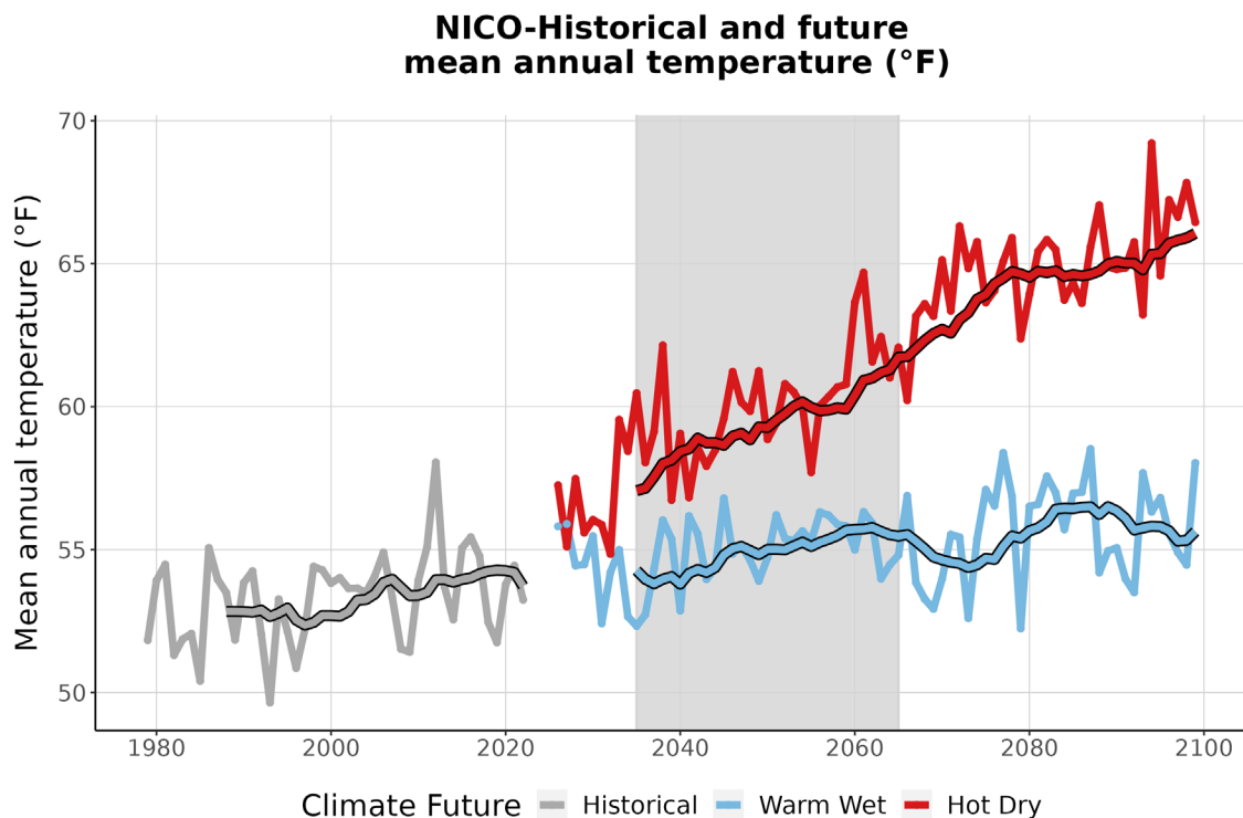
Figure 3. This graph compares observed average annual temperature at NICO (°F) (1979-2022) with projected average annual temperature for the two climate futures over the period 2023-2099. The historically observed data
