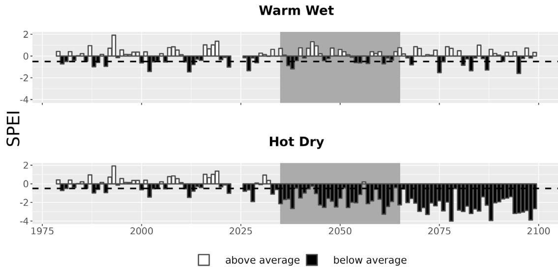
Figure 7. Drought metrics for NICO. Drought index (SPEI; units = standard deviations from historical) timeseries for each climate future. Below-average SPEI (black bars) indicates dry conditions. The dotted line (SPEI = -0.5) indicates drought conditions.
