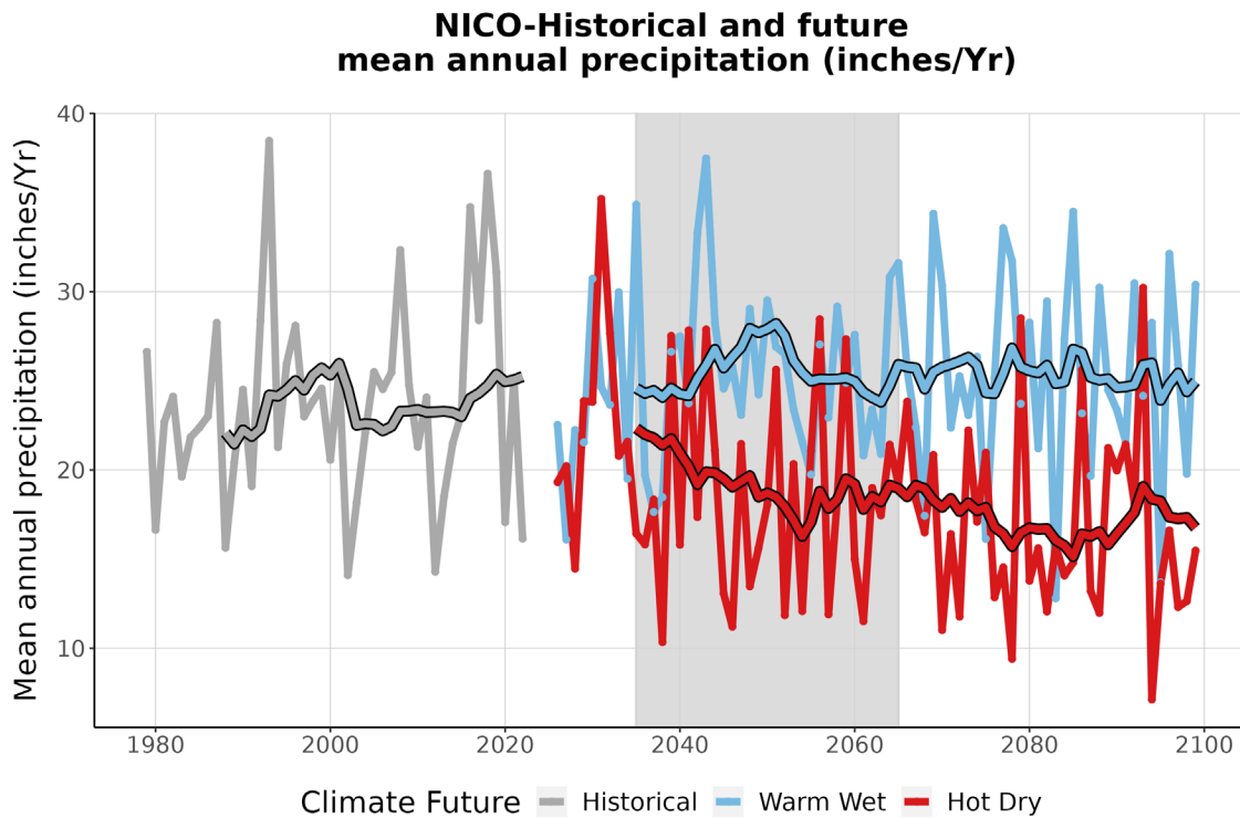
Figure 4. This graph compares observed average annual precipitation at NICO (inches/year) (1979-2022) with projected average annual precipitation for the two climate futures over the period 2023-2099. The historically observed data is shown in gray, the Warm Wet climate future in blue, and the Hot Dry climate future in red. The smooth line running through each projection is the 10-year running average for historical observations and future projections. The gray-shaded area represents the time period that was averaged (2035-2065) to summarize future projections for the year 2050 (Appendix 1).
