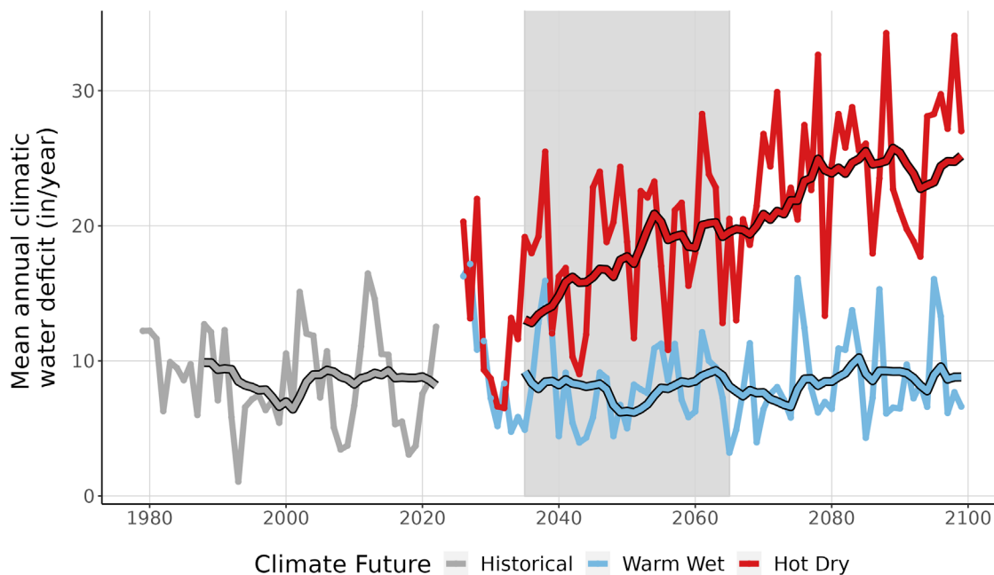
Figure 9. This line graph compares observed climatic water deficit at NICO (inches/year) (1979-2022) with projected climatic water deficit for the two climate futures over the period 2023-2099. The historical observation data is shown in gray, the Warm Wet climate future in blue, and the Hot Dry climate future in red. The smooth line running through each projection is the 10-year running average for historical observations and future projections. Gray-shaded area represents the time period that was averaged (2035-2065) to summarize future projections for the year 2050.
