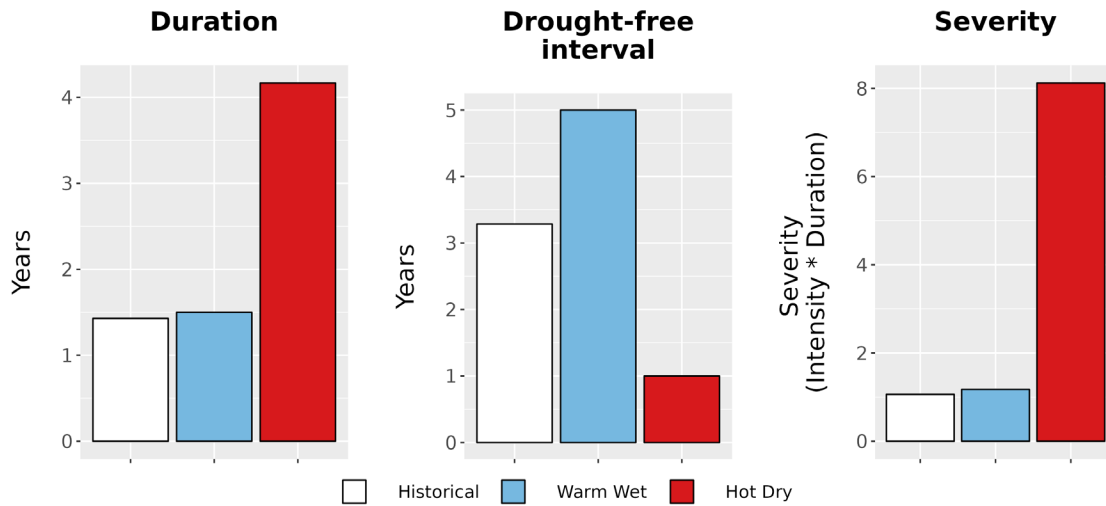
Figure 8. Drought metrics for NICO. (Left) Average drought duration (years) historically (1979-2012) and under each climate future. (Middle) Average drought return interval (years), indicating the expected amount of time between periods of drought, historically and under each climate future. (Right) Average drought severity, a measure of drought intensity multiplied by duration, historically and under each climate future.
