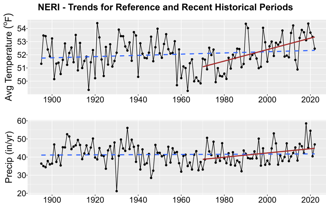
Figure 1. Historical trends in annual average temperature (upper plot) and annual total precipitation (lower plot) for NERI from 1895-2022. Black points show yearly values while blue lines are linear regressions for the entire period record and red lines for 1970-2022 trends. Solid lines are significant trends (i.e., p < 0.05 ); dashed lines are not statistically significant.
