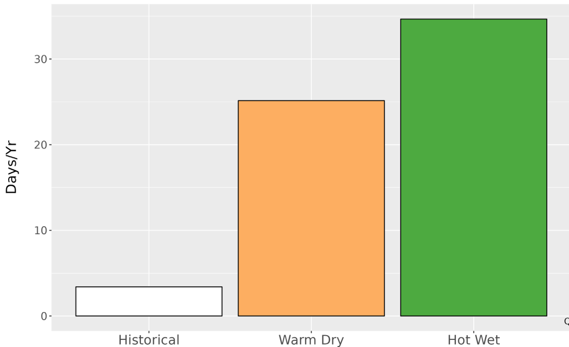
Figure 5. Metrics of extreme temperature at NERI. The bar graph represents the average number of days annually with temperatures greater than the historical 99th percentile (88.4 °F) historically (1979-2012) and for the two climate futures (2050).
