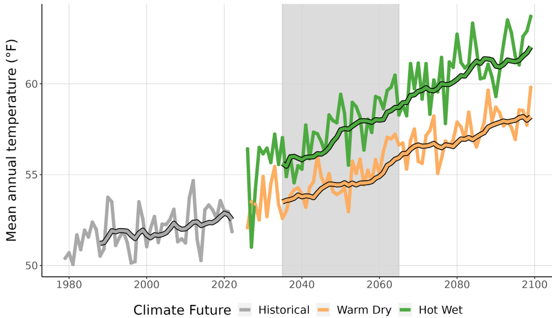
Figure 3. This graph compares observed average annual temperature at NERI (°F) (1979-2022) with projected average annual temperature for the two climate futures over the period 2023-2099. The historically observed data is shown in gray, the Warm Dry climate future in orange, and the Hot Wet climate future in green. The smooth line running through each projection is the 10-year running average for historical observations and future projections. Gray-shaded area represents the time period that was averaged (2035-2065) to summarize future projections for the year 2050 (Appendix 1).
