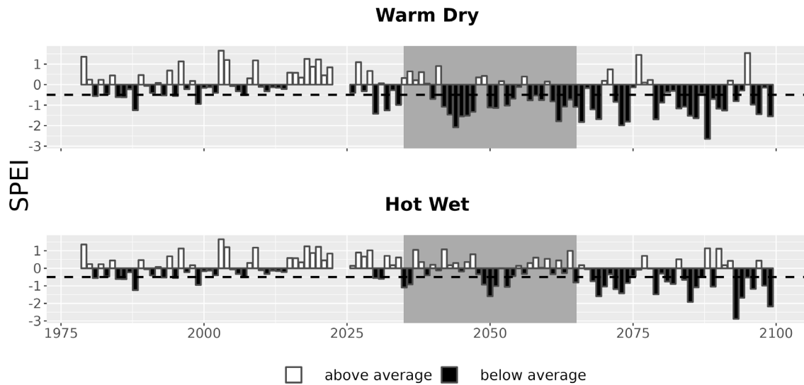
Figure 7. Drought metrics for NERI. Drought index (SPEI; units = standard deviations from historical) timeseries for each climate future. Below-average SPEI (black bars) indicates dry conditions. The dotted line (SPEI = -0.5) indicates drought conditions.
