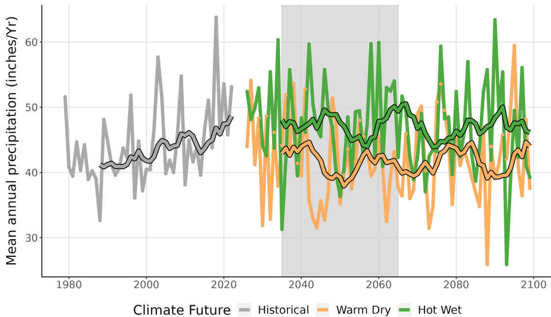
Figure 4. This graph compares observed average annual precipitation at NERI (inches/year) (1979-2022) with projected average annual precipitation for the two climate futures over the period 2023-2099. The historically observed data is shown in gray, the Warm Dry climate future in orange, and the Hot Wet climate future in green. The smooth line running through each projection is the 10-year running average for historical observations and future projections. The gray-shaded area represents the time period that was averaged (2035-2065) to summarize future projections for the year 2050 (Appendix 1).
