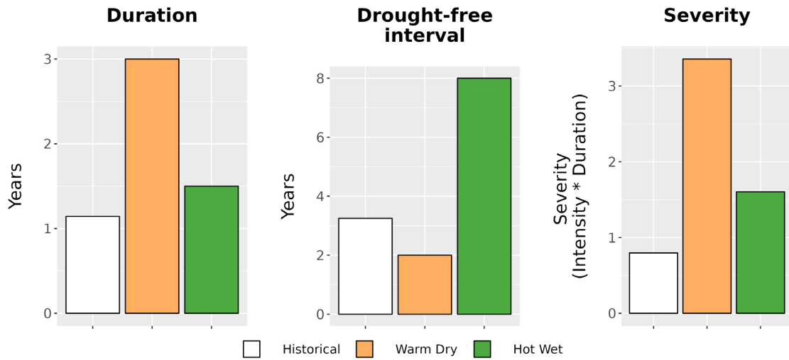
Figure 8. Drought metrics for NERI. (Left) Average drought duration (years) historically (1979-2012) and under each climate future. (Middle) Average drought return interval (years), indicating the expected amount of time between periods of drought, historically and under each climate future. (Right) Average drought severity, a measure of drought intensity multiplied by duration, historically and under each climate future.
