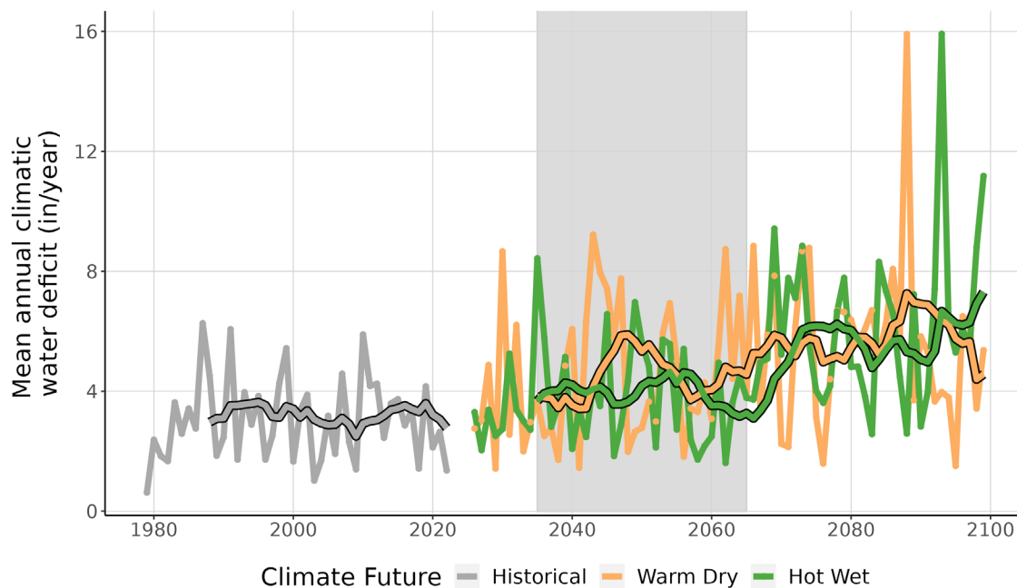
Figure 9. This line graph compares observed climatic water deficit at NERI (inches/year) (1979-2022) with projected climatic water deficit for the two climate futures over the period 2023-2099. The historical observation data is shown in gray, the Warm Dry climate future in orange, and the Hot Wet climate future in green. The smooth line running through each projection is the 10-year running average for historical observations and future projections. Gray-shaded area represents the time period that was averaged (2035-2065) to summarize future projections for the year 2050.
