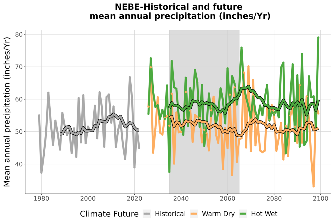
Figure 4. This graph compares observed average annual precipitation at NEBE (inches/year) (1979-2022) with projected average annual precipitation for the two climate futures over the period 2023-2099. The historically observed data is shown in gray, the Warm Dry climate future in orange, and the Hot Wet climate future in green. The smooth line running through each projection is the 10-year running average for historical observations and future projections. The gray-shaded area represents the time period that was averaged (2035-2065) to summarize future projections for the year 2050 (Appendix 1).
