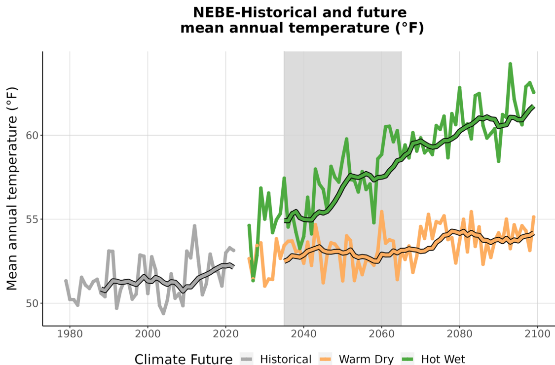
Figure 3. This graph compares observed average annual temperature at NEBE (°F) (1979-2022) with projected average annual temperature for the two climate futures over the period 2023-2099. The historically observed data
