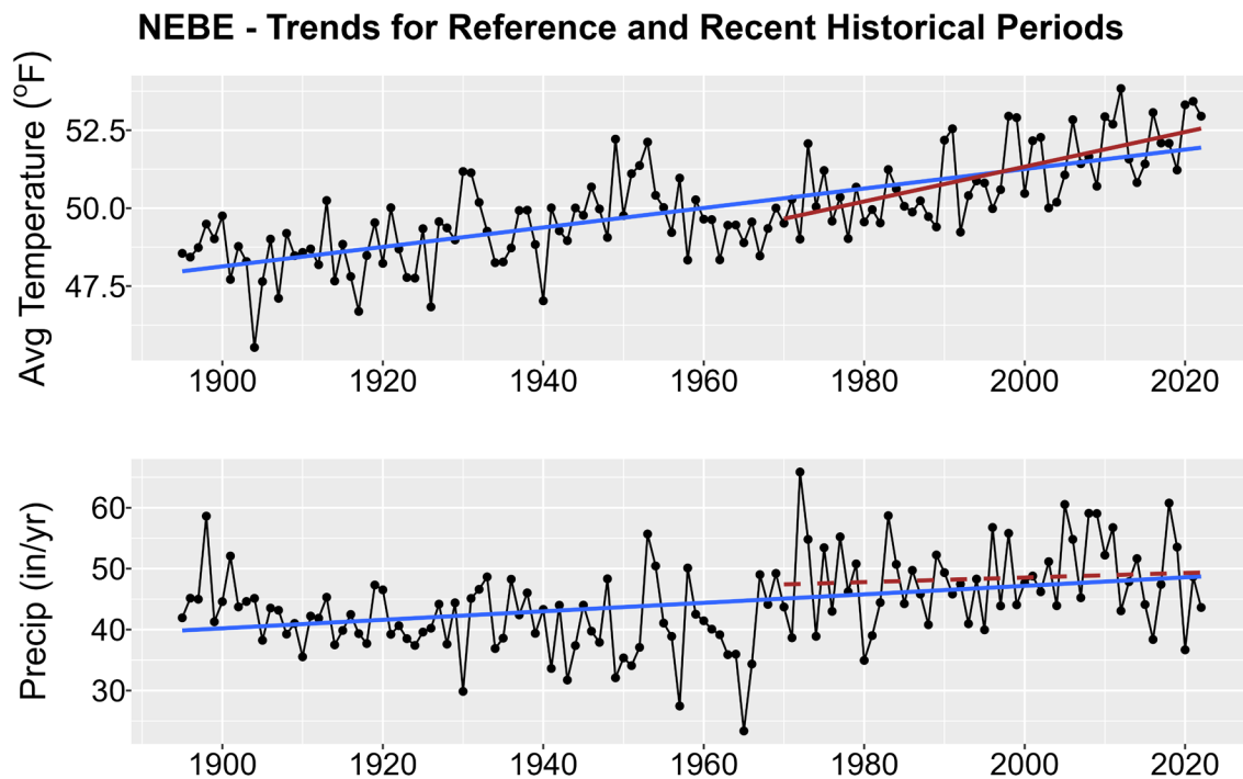
Figure 1. Historical trends in annual average temperature (upper plot) and annual total precipitation (lower plot) for NEBE from 1895-2022. Black points show yearly values while blue lines are linear regressions for the entire period record and red lines for 1970-2022 trends. Solid lines are significant trends (i.e., p < 0.05 ); dashed lines are not statistically significant.
