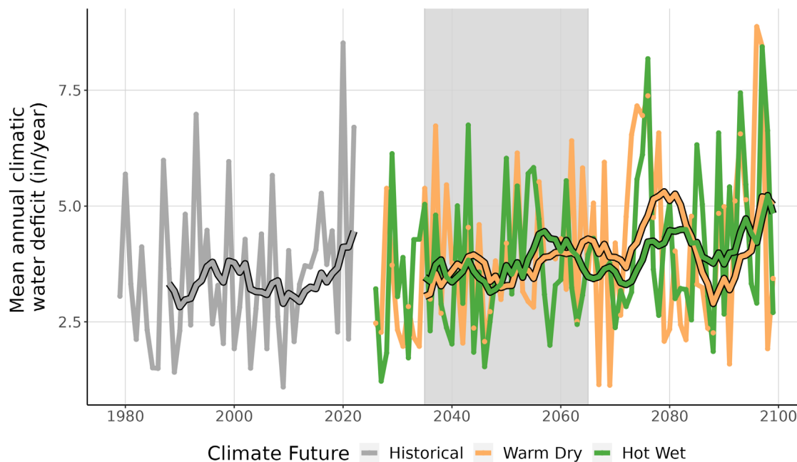
Figure 9. This line graph compares observed climatic water deficit at NEBE (inches/year) (1979-2022) with projected climatic water deficit for the two climate futures over the period 2023-2099. The historical observation data is shown in gray, the Warm Dry climate future in orange, and the Hot Wet climate future in green. The smooth line running through each projection is the 10-year running average for historical observations and future projections. Gray-shaded area represents the time period that was averaged (2035-2065) to summarize future projections for the year 2050.
