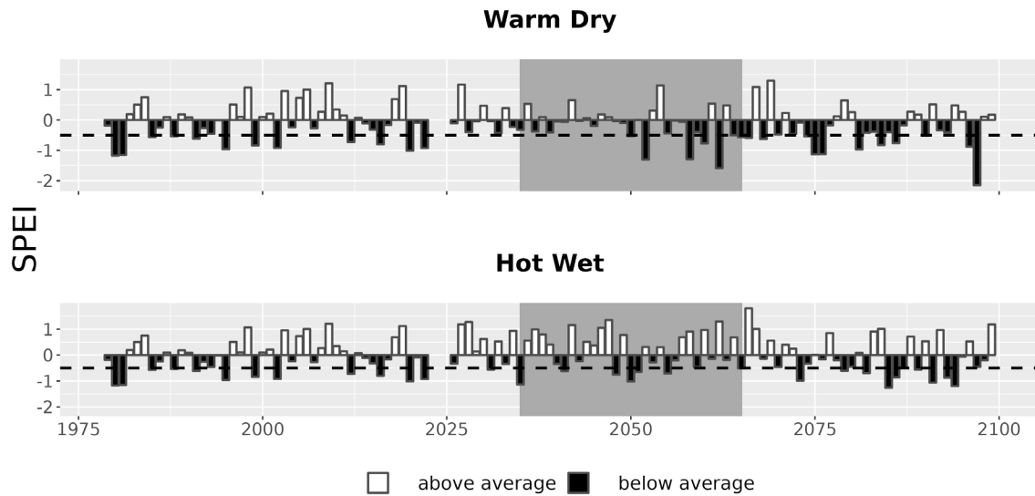
Figure 7. Drought metrics for NEBE. Drought index (SPEI; units = standard deviations from historical) timeseries for each climate future. Below-average SPEI (black bars) indicates dry conditions. The dotted line (SPEI = -0.5) indicates drought conditions.
