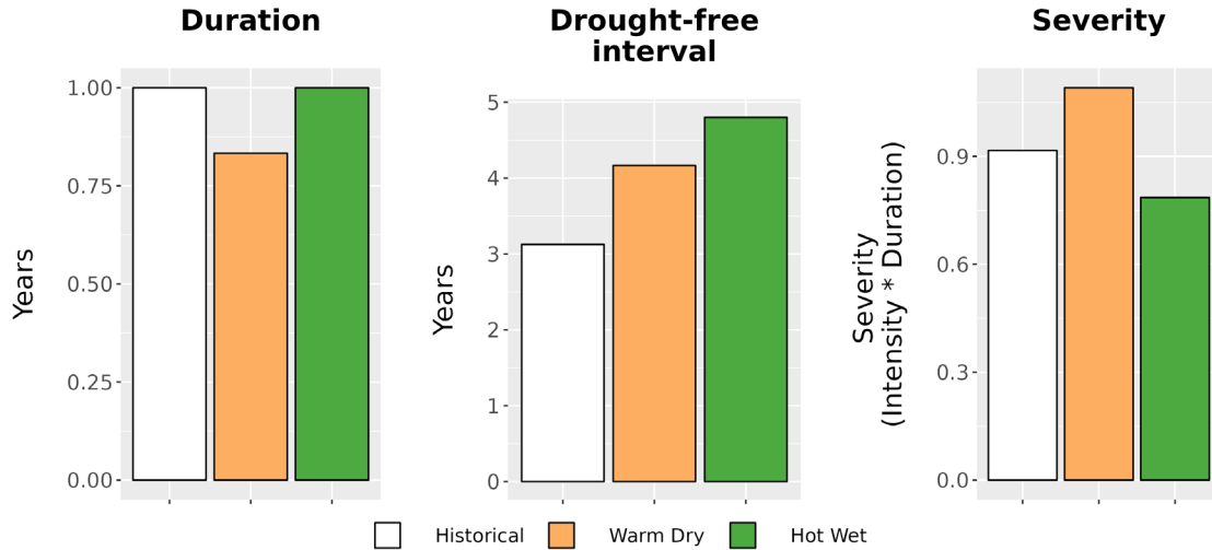
Figure 8. Drought metrics for NEBE. (Left) Average drought duration (years) historically (1979-2012) and under each climate future. (Middle) Average drought return interval (years), indicating the expected amount of time between periods of drought, historically and under each climate future. (Right) Average drought severity, a measure of drought intensity multiplied by duration, historically and under each climate future.
