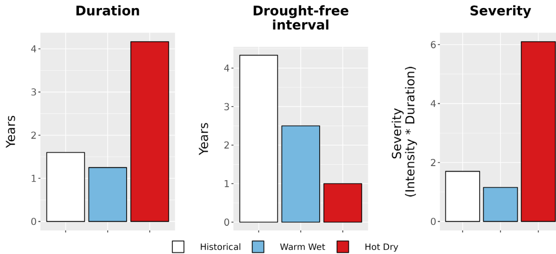
Figure 8. Drought metrics for NAVA. (Left) Average drought duration (years) historically (1979-2012) and under each climate future. (Middle) Average drought return interval (years), indicating the expected amount of time between periods of drought, historically and under each climate future. (Right) Average drought severity, a measure of drought intensity multiplied by duration, historically and under each climate future.
