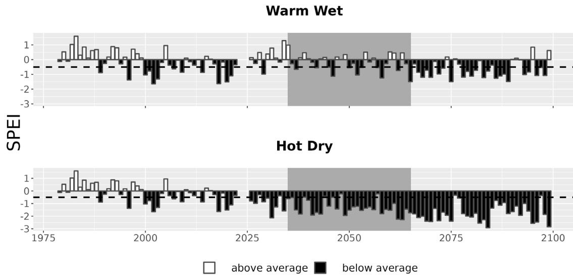
Figure 7. Drought metrics for NAVA. Drought index (SPEI; units = standard deviations from historical) timeseries for each climate future. Below-average SPEI (black bars) indicates dry conditions. The dotted line (SPEI = -0.5) indicates drought conditions.
