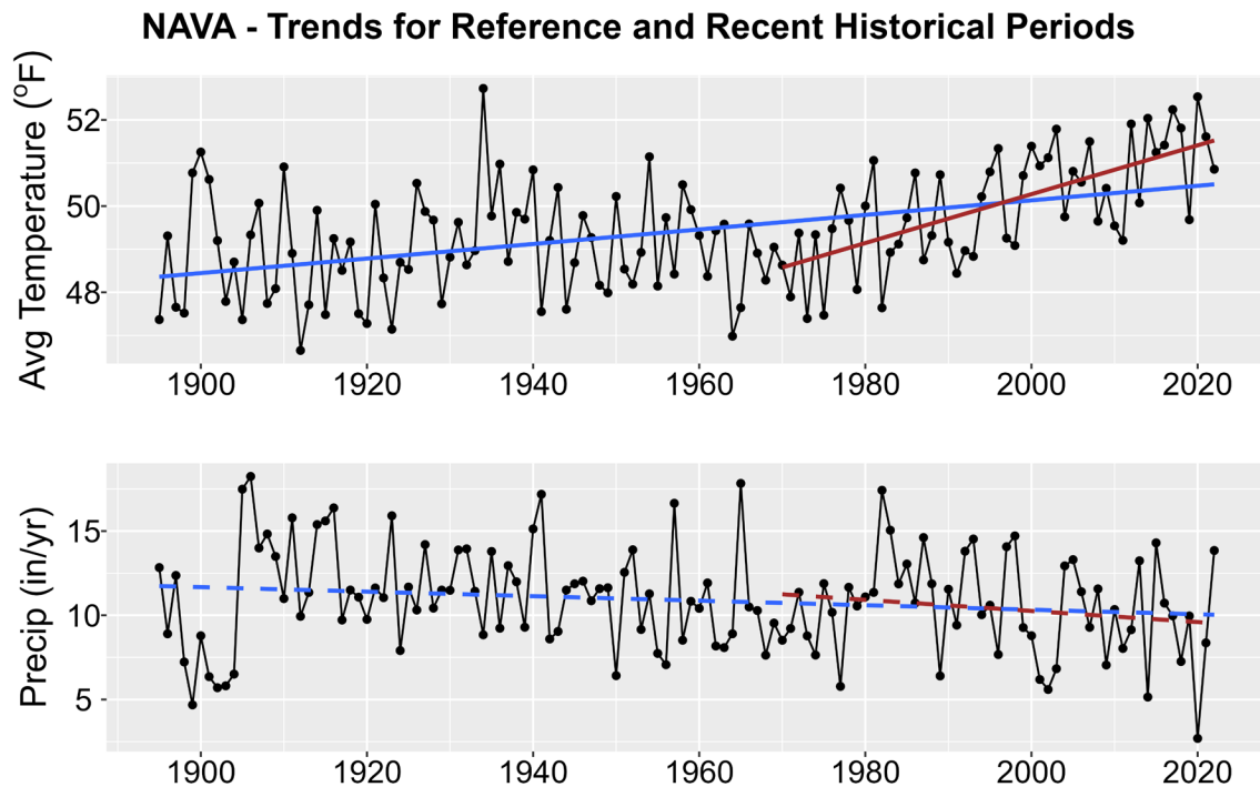
Figure 1. Historical trends in annual average temperature (upper plot) and annual total precipitation (lower plot) for NAVA from 1895-2022. Black points show yearly values while blue lines are linear regressions for the entire period record and red lines for 1970-2022 trends. Solid lines are significant trends (i.e., p < 0.05 ); dashed lines are not statistically significant.
