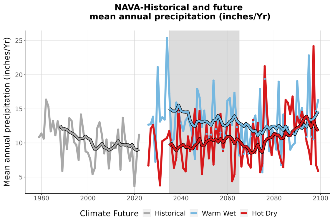
Figure 4. This graph compares observed average annual precipitation at NAVA (inches/year) (1979-2022) with projected average annual precipitation for the two climate futures over the period 2023-2099. The historically observed data is shown in gray, the Warm Wet climate future in blue, and the Hot Dry climate future in red. The smooth line running through each projection is the 10-year running average for historical observations and future projections. The gray-shaded area represents the time period that was averaged (2035-2065) to summarize future projections for the year 2050 (Appendix 1).
