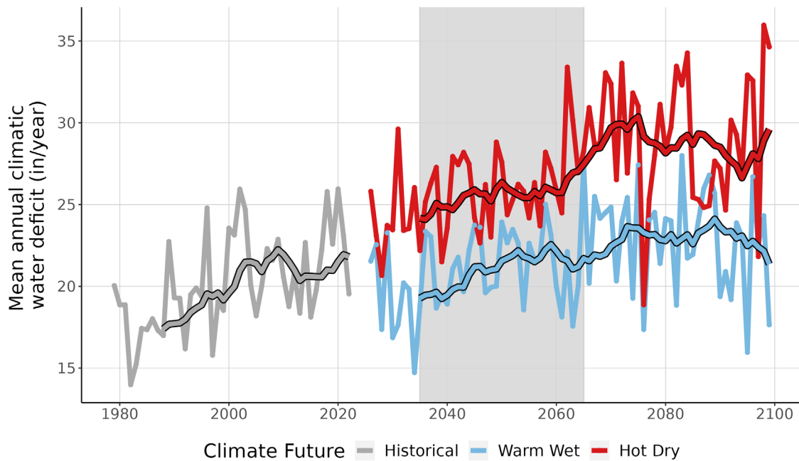
Figure 9. This line graph compares observed climatic water deficit at NAVA (inches/year) (1979-2022) with projected climatic water deficit for the two climate futures over the period 2023-2099. The historical observation data is shown in gray, the Warm Wet climate future in blue, and the Hot Dry climate future in red. The smooth line running through each projection is the 10-year running average for historical observations and future projections. Gray-shaded area represents the time period that was averaged (2035-2065) to summarize future projections for the year 2050.
