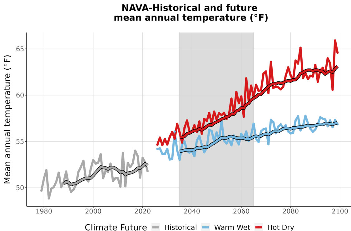
Figure 3. This graph compares observed average annual temperature at NAVA (°F) (1979-2022) with projected average annual temperature for the two climate futures over the period 2023-2099. The historically observed data
