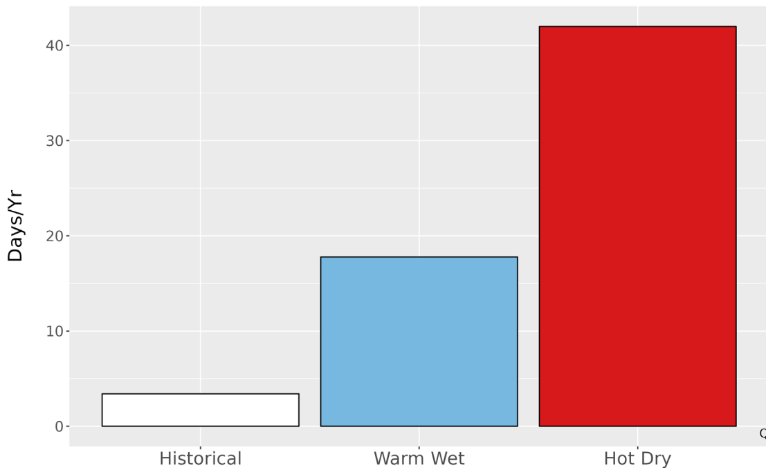
Figure 5. Metrics of extreme temperature at NAVA. The bar graph represents the average number of days annually with temperatures greater than the historical 99th percentile (94.5 °F) historically (1979-2012) and for the two climate futures (2050).
