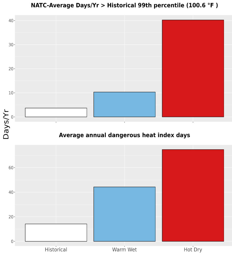
Figure 5. The upper bar graph represents the average number of days annually with temperatures greater than the historical 99th percentile (100.6 °F) historically (1979-2012) and for the two climate futures (2050). The bottom bar graph represents the average annual number of dangerous heat index days historically and for the two climate futures. Dangerous heat index days are days that exceed 105 °F.
