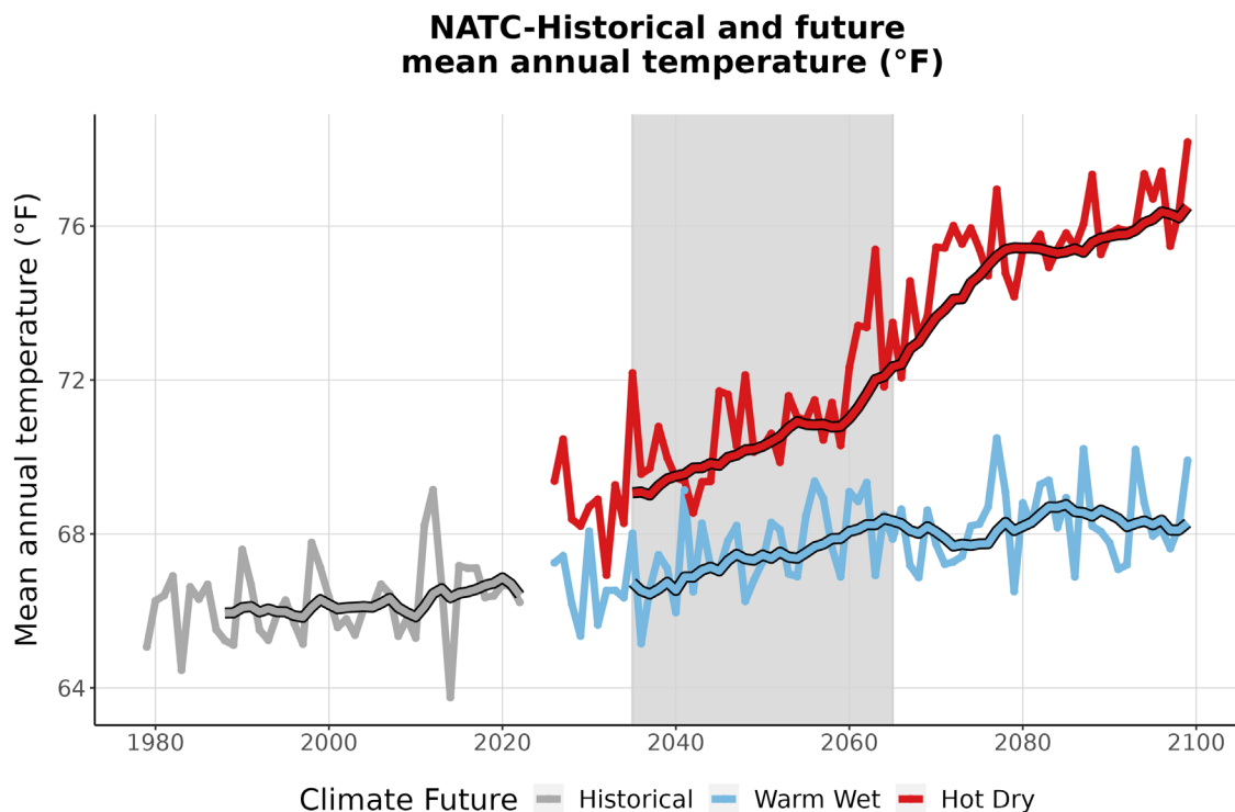
Figure 3. This graph compares observed average annual temperature at NATC (°F) (1979-2022) with projected average annual temperature for the two climate futures over the period 2023-2099. The historically observed data
