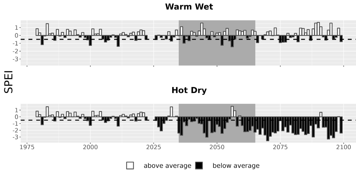
Figure 7. Drought metrics for NATC. Drought index (SPEI; units = standard deviations from historical) timeseries for each climate future. Below-average SPEI (black bars) indicates dry conditions. The dotted line (SPEI = -0.5) indicates drought conditions.
