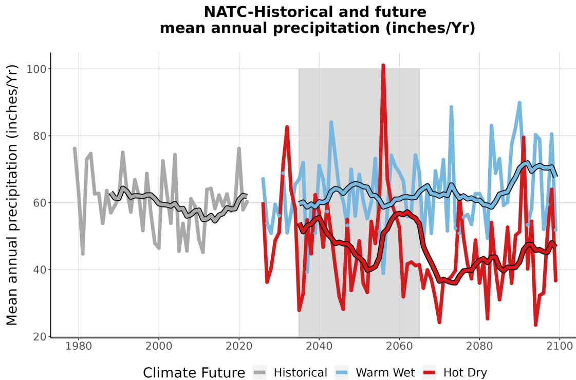
Figure 4. This graph compares observed average annual precipitation at NATC (inches/year) (1979-2020) with projected average annual precipitation for the two climate futures over the period 2023-2099. The historically observed data is shown in gray, the Warm Wet climate future in blue, and the Hot Dry climate future in red. The smooth line running through each projection is the 10-year running average for historical observations and future projections. The gray-shaded area represents the time period that was averaged (2035-2065) to summarize future projections for the year 2050 (Appendix 1).
