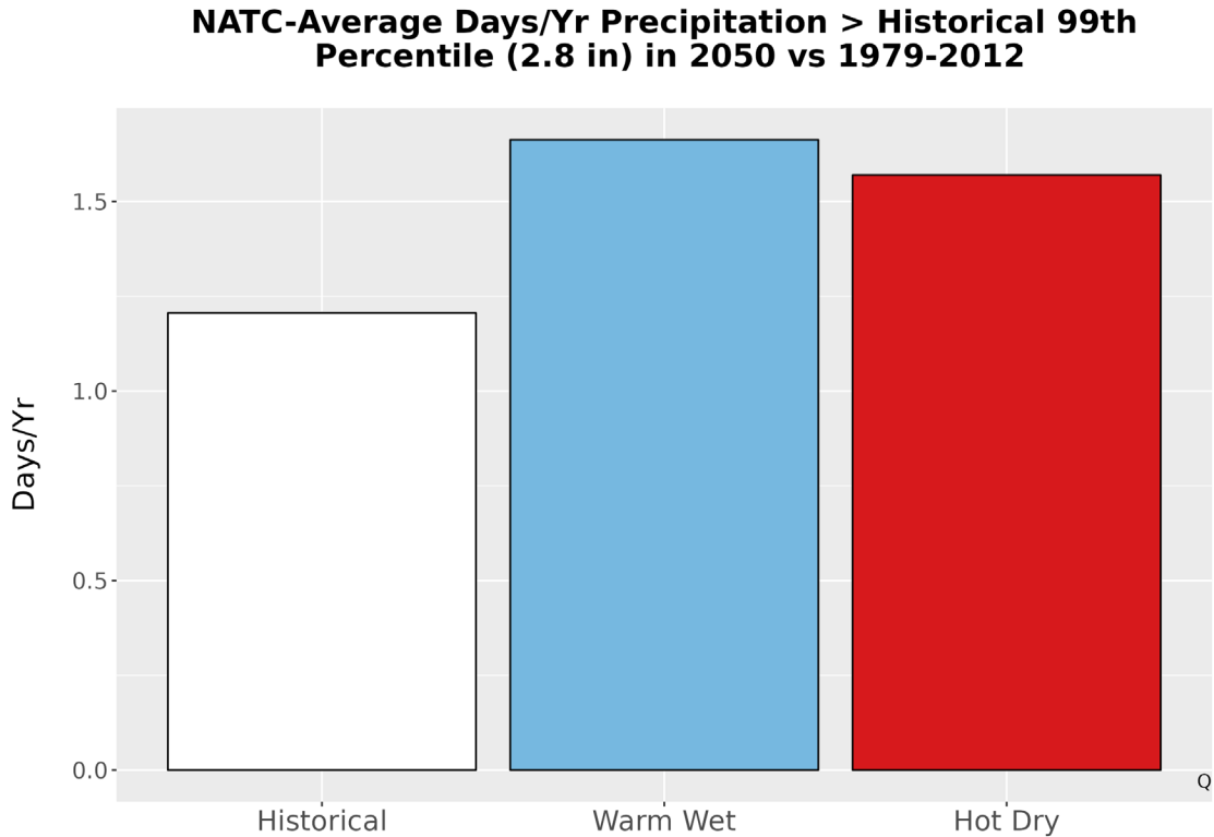
Figure 6. Average number of days annually with precipitation exceeding the 99th percentile (2.8 in.) of precipitation from the historical period 1979-2012 and for each climate future.
