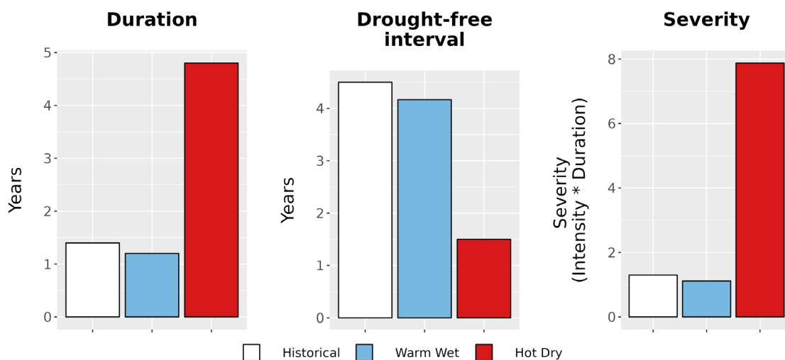
Figure 8. Drought metrics for NATC. (Left) Average drought duration (years) historically (1979-2012) and under each climate future. (Middle) Average drought return interval (years), indicating the expected amount of time between periods of drought, historically and under each climate future. (Right) Average drought severity, a measure of drought intensity multiplied by duration, historically and under each climate future.
