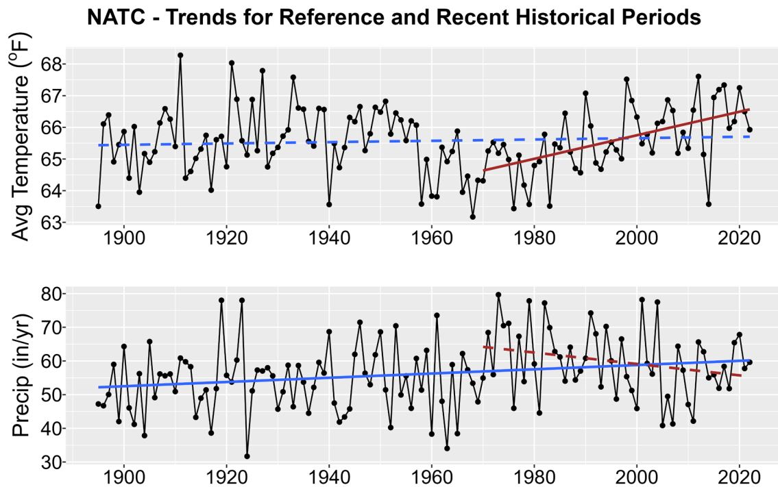
Figure 1. Historical trends in annual average temperature (upper plot) and annual total precipitation (lower plot) for NATC from 1895-2022. Black points show yearly values while blue lines are linear regressions for the entire period record and red lines for 1970-2022 trends. Solid lines are significant trends (i.e., p < 0.05 ); dashed lines are not statistically significant.
