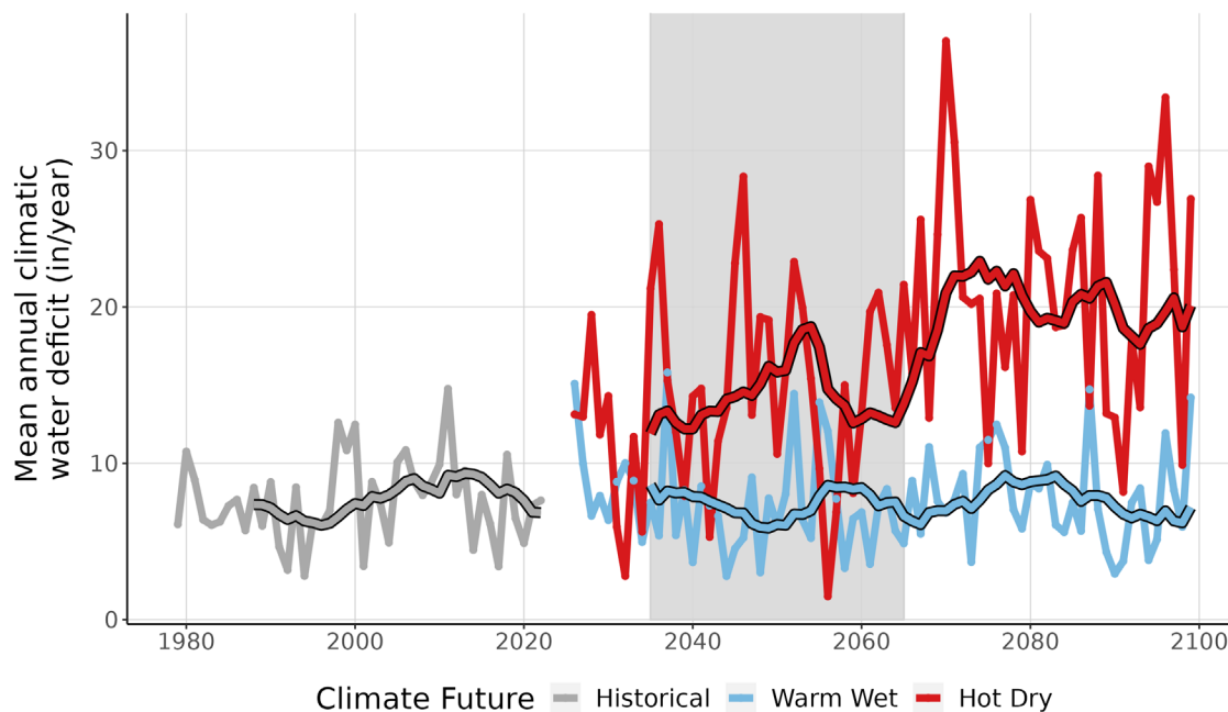
Figure 9. This line graph compares observed climatic water deficit at NATC (inches/year) (1979-2022) with projected climatic water deficit for the two climate futures over the period 2023-2099. The historical observation data is shown in gray, the Warm Wet climate future in blue, and the Hot Dry climate future in red. The smooth line running through each projection is the 10-year running average for historical observations and future projections. Gray-shaded area represents the time period that was averaged (2035-2065) to summarize future projections for the year 2050.
