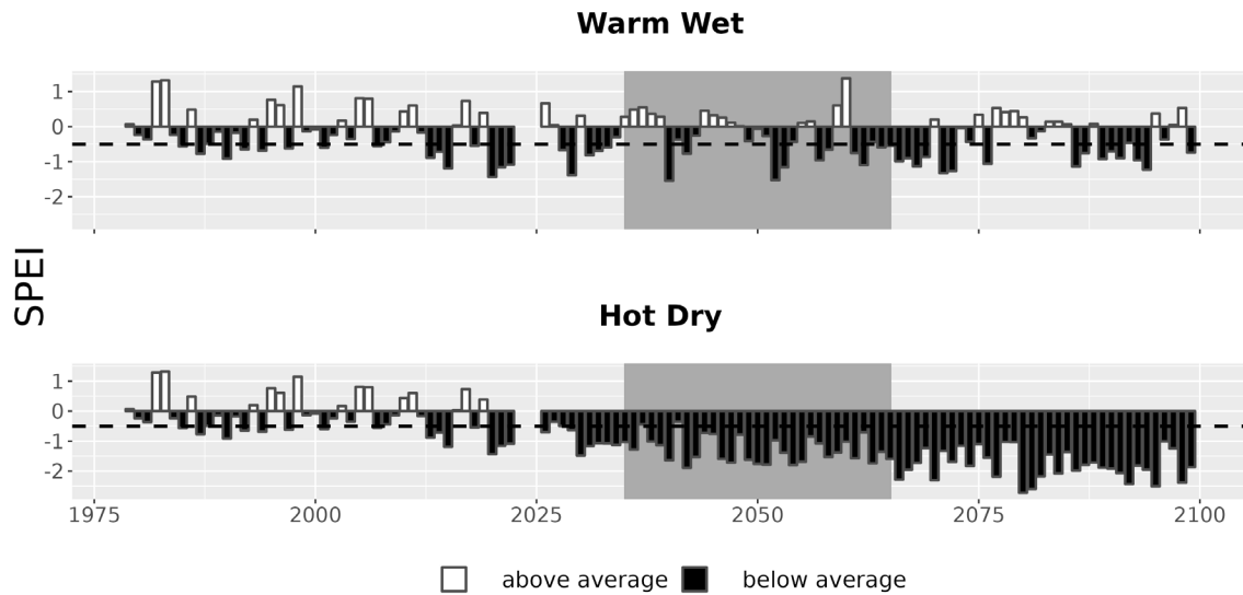
Figure 7. Drought metrics for MUWO. Drought index (SPEI; units = standard deviations from historical) timeseries for each climate future. Below-average SPEI (black bars) indicates dry conditions. The dotted line (SPEI = -0.5) indicates drought conditions.
