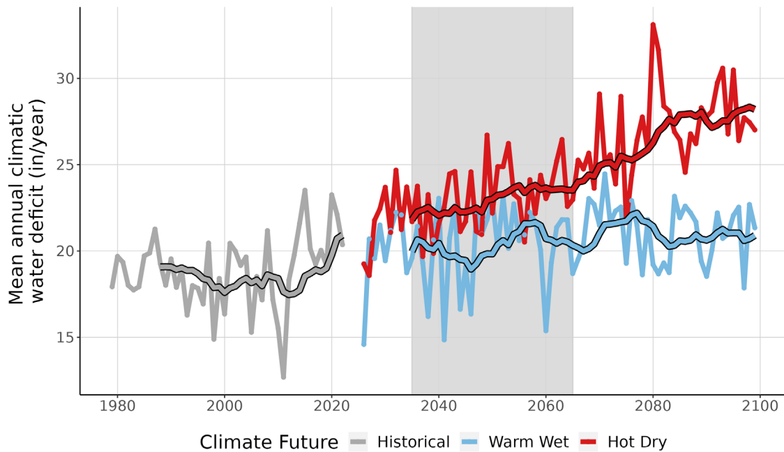
Figure 9. This line graph compares observed climatic water deficit at MUWO (inches/year) (1979-2022) with projected climatic water deficit for the two climate futures over the period 2023-2099. The historical observation data is shown in gray, the Warm Wet climate future in blue, and the Hot Dry climate future in red. The smooth line running through each projection is the 10-year running average for historical observations and future projections. Gray-shaded area represents the time period that was averaged (2035-2065) to summarize future projections for the year 2050.
