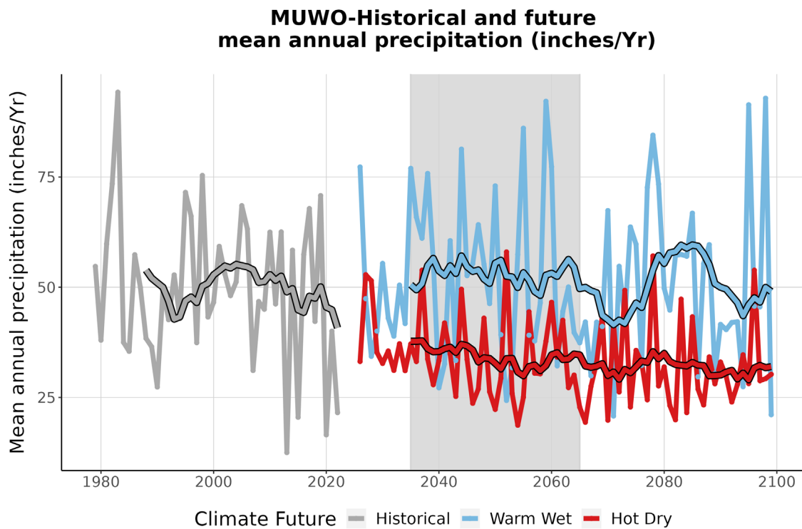
Figure 4. This graph compares observed average annual precipitation at MUWO (inches/year) (1979-2022) with projected average annual precipitation for the two climate futures over the period 2023-2099. The historically observed data is shown in gray, the Warm Wet climate future in blue, and the Hot Dry climate future in red. The smooth line running through each projection is the 10-year running average for historical observations and future projections. The gray-shaded area represents the time period that was averaged (2035-2065) to summarize future projections for the year 2050 (Appendix 1).
