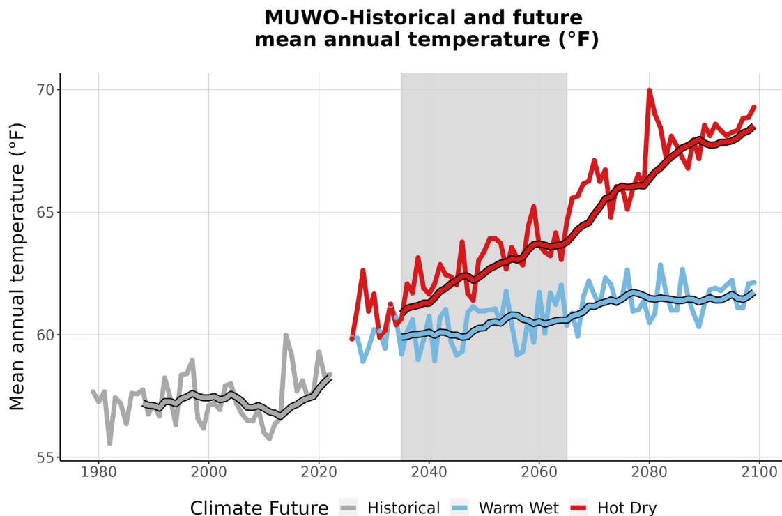
Figure 3. This graph compares observed average annual temperature at MUWO (°F) (1979-2022) with projected average annual temperature for the two climate futures over the period 2023-2099. The historically observed data
