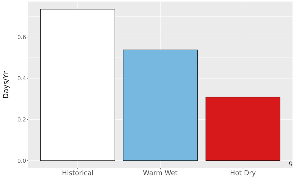
Figure 6. Average number of days annually with precipitation exceeding the 99th percentile (3.8 in.) of precipitation from the historical period 1979-2012 and for each climate future.
