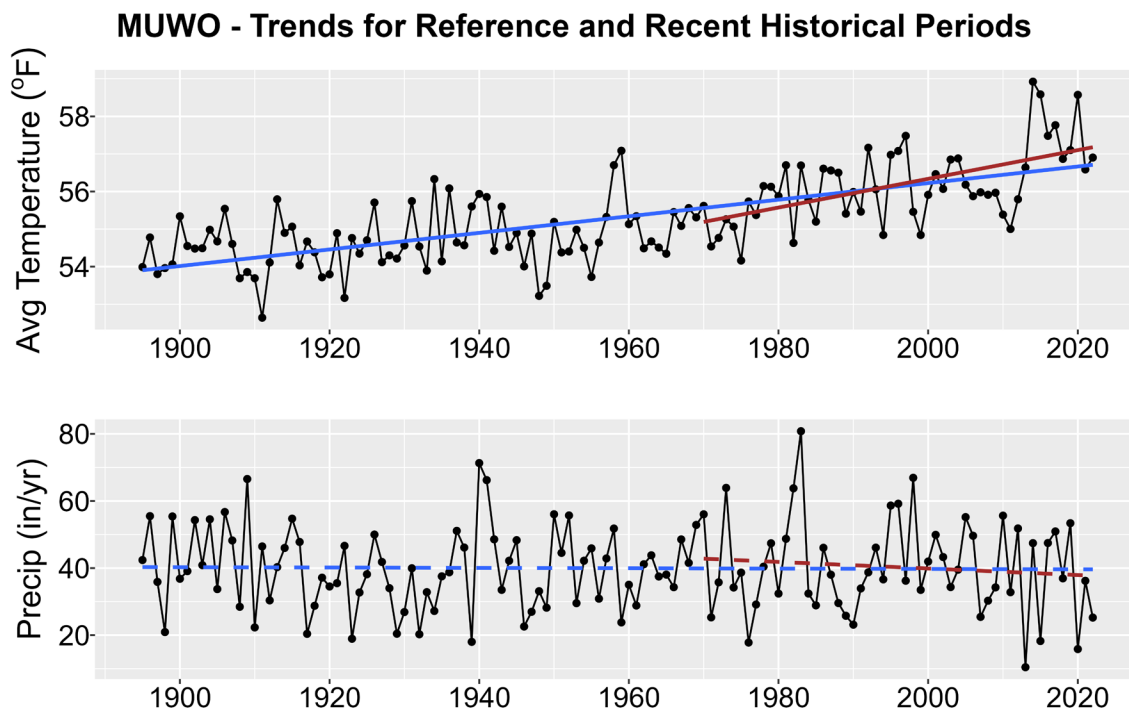
Figure 1. Historical trends in annual average temperature (upper plot) and annual total precipitation (lower plot) for MUWO from 1895-2022. Black points show yearly values while blue lines are linear regressions for the entire period record and red lines for 1970-2022 trends. Solid lines are significant trends (i.e., p < 0.05 ); dashed lines are not statistically significant.
