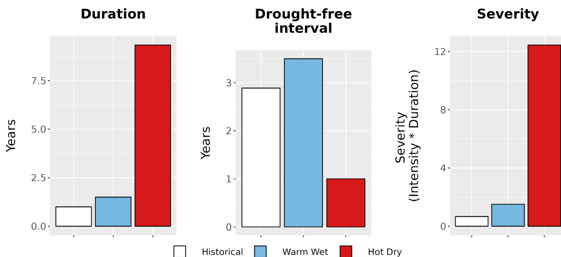
Figure 8. Drought metrics for MUWO. (Left) Average drought duration (years) historically (1979-2012) and under each climate future. (Middle) Average drought return interval (years), indicating the expected amount of time between periods of drought, historically and under each climate future. (Right) Average drought severity, a measure of drought intensity multiplied by duration, historically and under each climate future.
