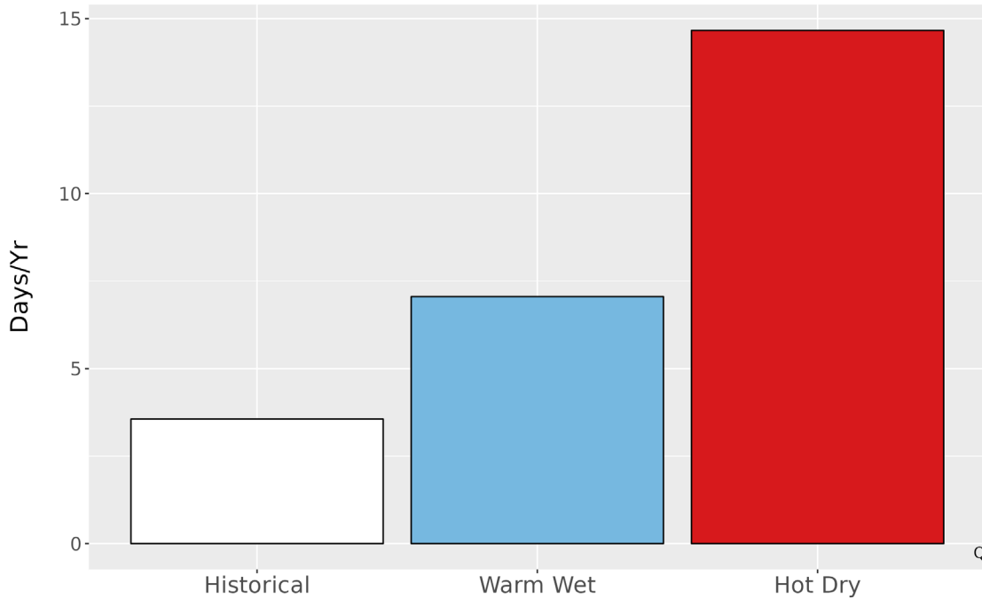
Figure 5. Metrics of extreme temperature at MUWO. The bar graph represents the average number of days annually with temperatures greater than the historical 99th percentile (85.5 °F) historically (1979-2012) and for the two climate futures (2050).
