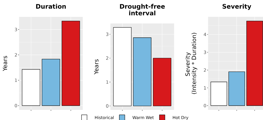
Figure 8. Drought metrics for MORU. (Left) Average drought duration (years) historically (1979-2012) and under each climate future. (Middle) Average drought return interval (years), indicating the expected amount of time between periods of drought, historically and under each climate future. (Right) Average drought severity, a measure of drought intensity multiplied by duration, historically and under each climate future.
