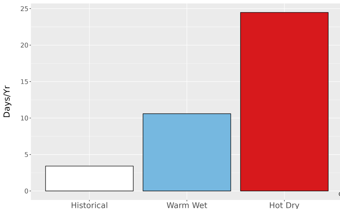
Figure 5. Metrics of extreme temperature at MORU. The bar graph represents the average number of days annually with temperatures greater than the historical 99th percentile (92.6 °F) historically (1979-2012) and for the two climate futures (2050).
