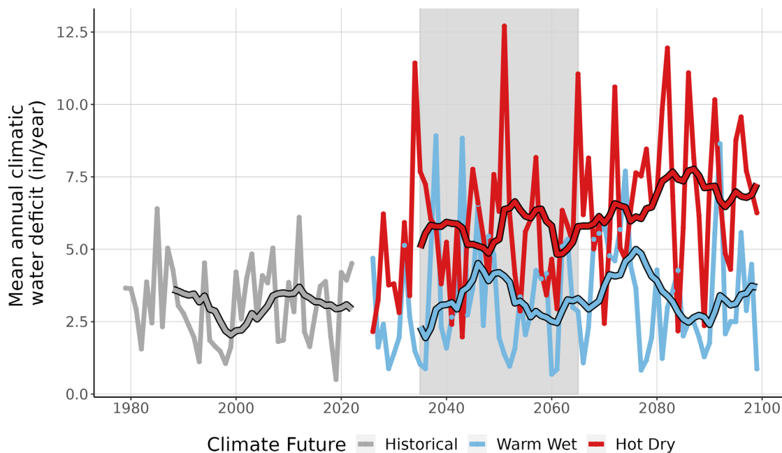
Figure 9. This line graph compares observed climatic water deficit at MORU (inches/year) (1979-2022) with projected climatic water deficit for the two climate futures over the period 2023-2099. The historical observation data is shown in gray, the Warm Wet climate future in blue, and the Hot Dry climate future in red. The smooth line running through each projection is the 10-year running average for historical observations and future projections. Gray-shaded area represents the time period that was averaged (2035-2065) to summarize future projections for the year 2050.
