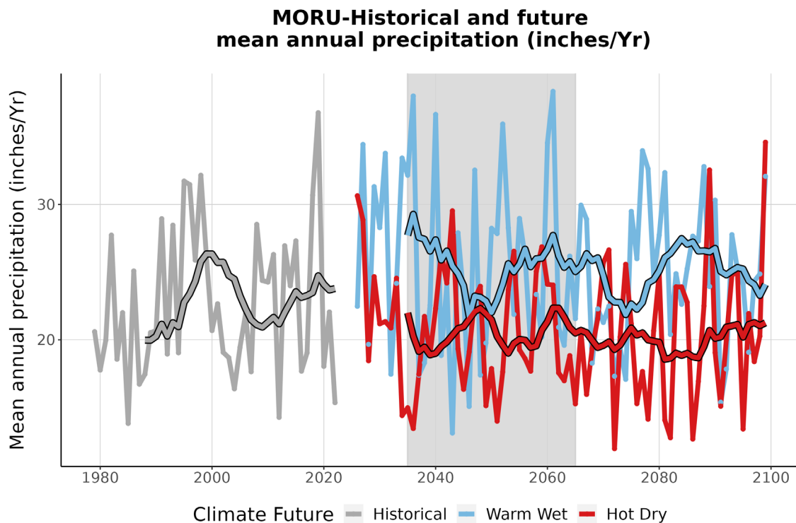
Figure 4. This graph compares observed average annual precipitation at MORU (inches/year) (1979-2022) with projected average annual precipitation for the two climate futures over the period 2023-2099. The historically observed data is shown in gray, the Warm Wet climate future in blue, and the Hot Dry climate future in red. The smooth line running through each projection is the 10-year running average for historical observations and future projections. The gray-shaded area represents the time period that was averaged (2035-2065) to summarize future projections for the year 2050 (Appendix 1).
