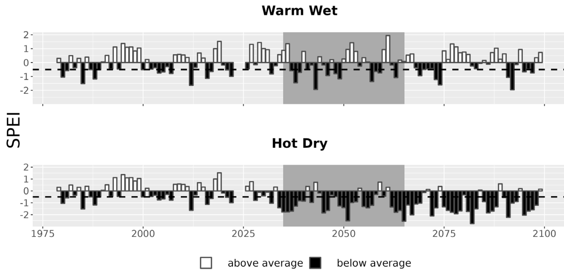
Figure 7. Drought metrics for MORU. Drought index (SPEI; units = standard deviations from historical) timeseries for each climate future. Below-average SPEI (black bars) indicates dry conditions. The dotted line (SPEI = -0.5) indicates drought conditions.
