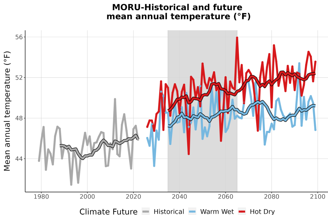
Figure 3. This graph compares observed average annual temperature at MORU (°F) (1979-2022) with projected average annual temperature for the two climate futures over the period 2023-2099. The historically observed data
