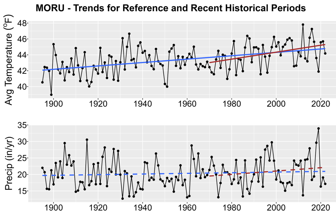
Figure 1. Historical trends in annual average temperature (upper plot) and annual total precipitation (lower plot) for MORU from 1895-2022. Black points show yearly values while blue lines are linear regressions for the entire period record and red lines for 1970-2022 trends. Solid lines are significant trends (i.e., p < 0.05 ); dashed lines are not statistically significant.
