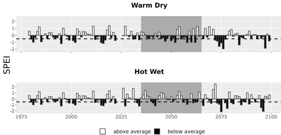
Figure 7. Drought metrics for MORR. Drought index (SPEI; units = standard deviations from historical) timeseries for each climate future. Below-average SPEI (black bars) indicates dry conditions. The dotted line (SPEI = -0.5) indicates drought conditions.
