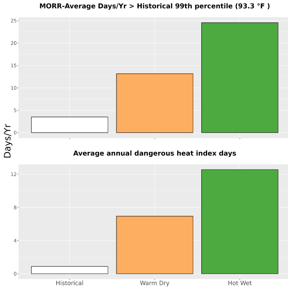
Figure 5. The upper bar graph represents the average number of days annually with temperatures greater than the historical 99th percentile (93.3 °F) historically (1979-2012) and for the two climate futures (2050). The bottom bar graph represents the average annual number of dangerous heat index days historically and for the two climate futures. Dangerous heat index days are days that exceed 105 °F.
