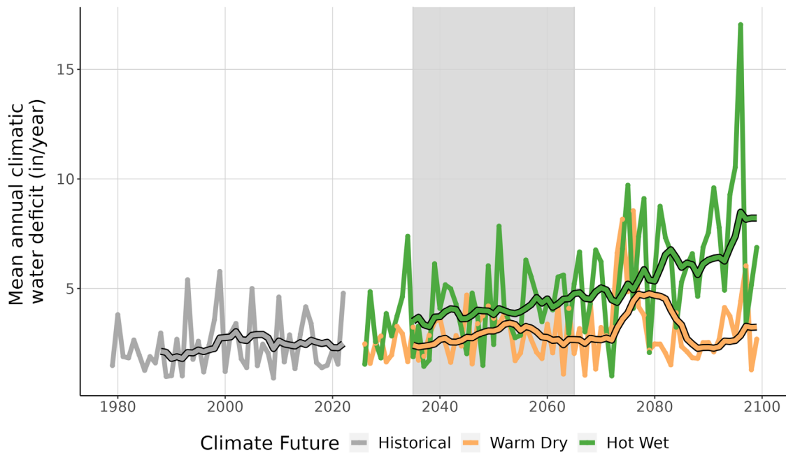
Figure 9. This line graph compares observed climatic water deficit at MORR (inches/year) (1979-2022) with projected climatic water deficit for the two climate futures over the period 2023-2099. The historical observation data is shown in gray, the Warm Dry climate future in orange, and the Hot Wet climate future in green. The smooth line running through each projection is the 10-year running average for historical observations and future projections. Gray-shaded area represents the time period that was averaged (2035-2065) to summarize future projections for the year 2050.
