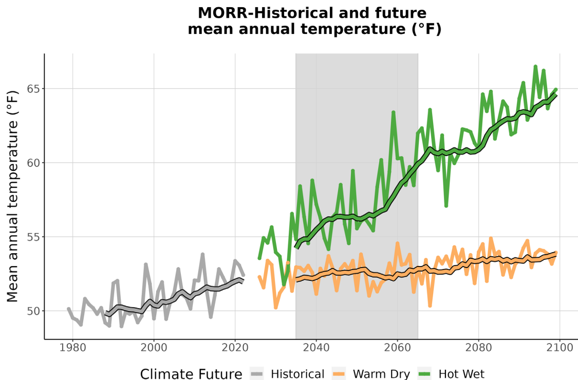
Figure 3. This graph compares observed average annual temperature at MORR (°F) (1979-2022) with projected average annual temperature for the two climate futures over the period 2023-2099. The historically observed data
