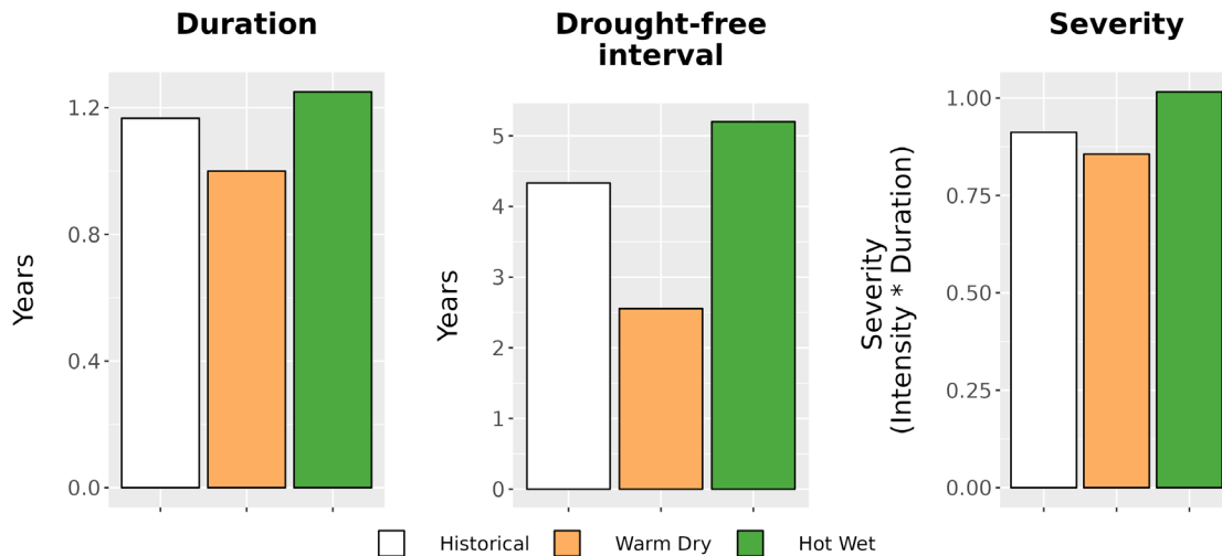
Figure 8. Drought metrics for MORR. (Left) Average drought duration (years) historically (1979-2012) and under each climate future. (Middle) Average drought return interval (years), indicating the expected amount of time between periods of drought, historically and under each climate future. (Right) Average drought severity, a measure of drought intensity multiplied by duration, historically and under each climate future.
