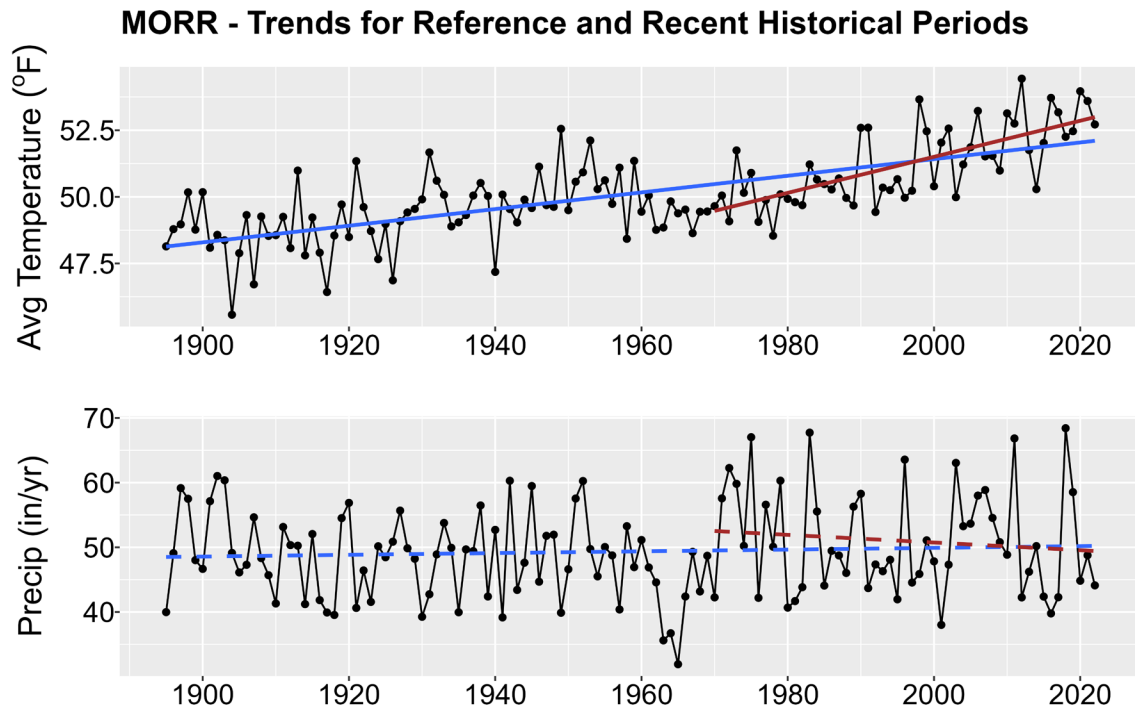
Figure 1. Historical trends in annual average temperature (upper plot) and annual total precipitation (lower plot) for MORR from 1895-2022. Black points show yearly values while blue lines are linear regressions for the entire period record and red lines for 1970-2022 trends. Solid lines are significant trends (i.e., p < 0.05 ); dashed lines are not statistically significant.
