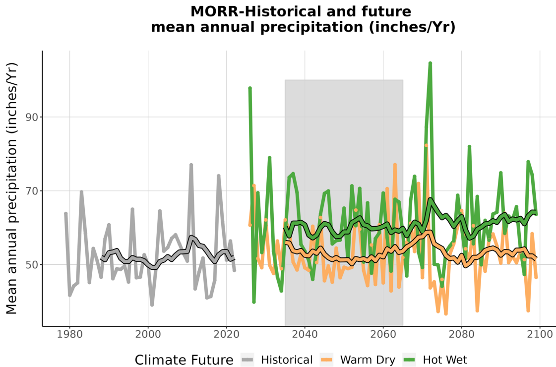
Figure 4. This graph compares observed average annual precipitation at MORR (inches/year) (1979-2022) with projected average annual precipitation for the two climate futures over the period 2023-2099. The historically observed data is shown in gray, the Warm Dry climate future in orange, and the Hot Wet climate future in green. The smooth line running through each projection is the 10-year running average for historical observations and future projections. The gray-shaded area represents the time period that was averaged (2035-2065) to summarize future projections for the year 2050 (Appendix 1).
