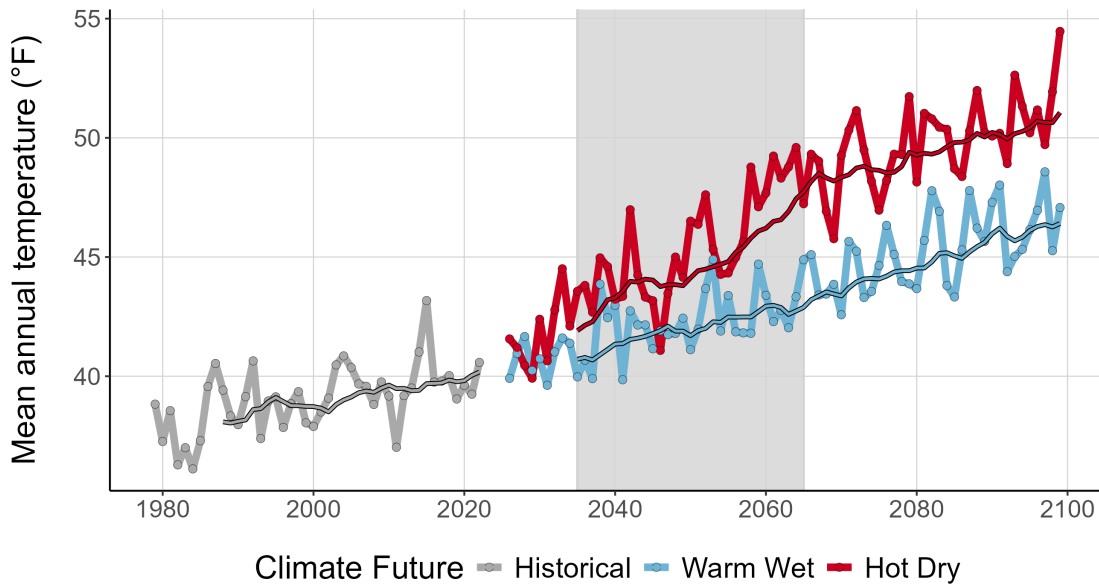
Figure 3. This graph compares observed average annual temperature at MORA (°F) (1979-2022) with projected average annual temperature for the two climate futures over the period 2023-2099. The historically observed data is shown in gray, the Warm Wet climate future in blue, and the Hot Dry climate future in red. The smooth line running through each projection is the 10-year running average for historical observations and future projections. Gray-shaded area represents the time period that was averaged (2035-2065) to summarize future projections for the year 2050 (Appendix 1).
