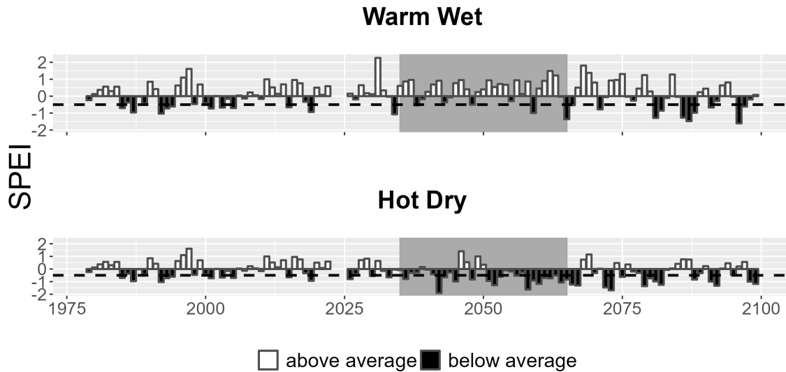
Figure 7. Drought metrics for MORA. Drought index (SPEI; units = standard deviations from historical) timeseries for each climate future. Below-average SPEI (black bars) indicates dry conditions. The dotted line (SPEI = -0.5) indicates drought conditions.
