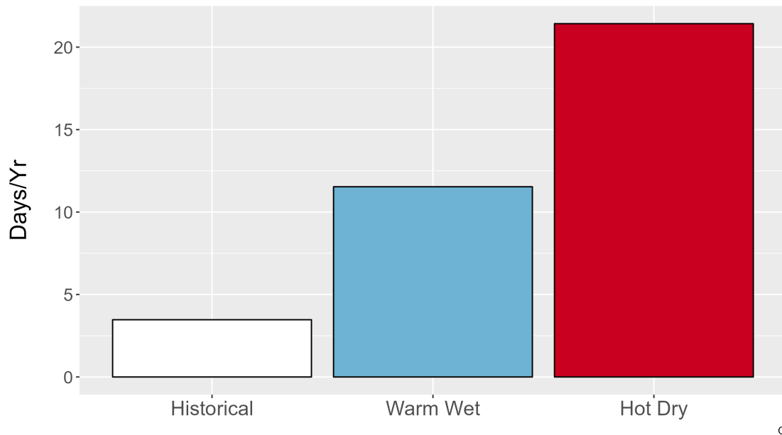
Figure 5. Metrics of extreme temperature at MORA. The bar graph represents the average number of days annually with temperatures greater than the historical 99th percentile (76.4 °F) historically (1979-2012) and for the two climate futures (2050).
