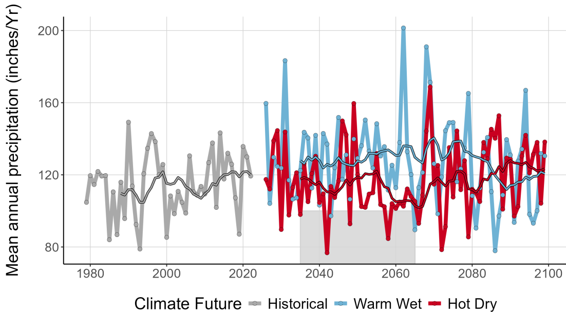
Figure 4. This graph compares observed average annual precipitation at MORA (inches/year) (1979-2022) with projected average annual precipitation for the two climate futures over the period 2023-2099. The historically observed data is shown in gray, the Warm Wet climate future in blue, and the Hot Dry climate future in red. The smooth line running through each projection is the 10-year running average for historical observations and future projections. The gray-shaded area represents the time period that was averaged (2035-2065) to summarize future projections for the year 2050 (Appendix 1).
