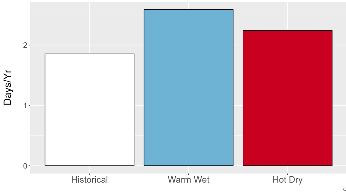
Figure 6. Average number of days annually with precipitation exceeding the 99th percentile (3.3 in.) of precipitation from the historical period 1979-2012 and for each climate future.
