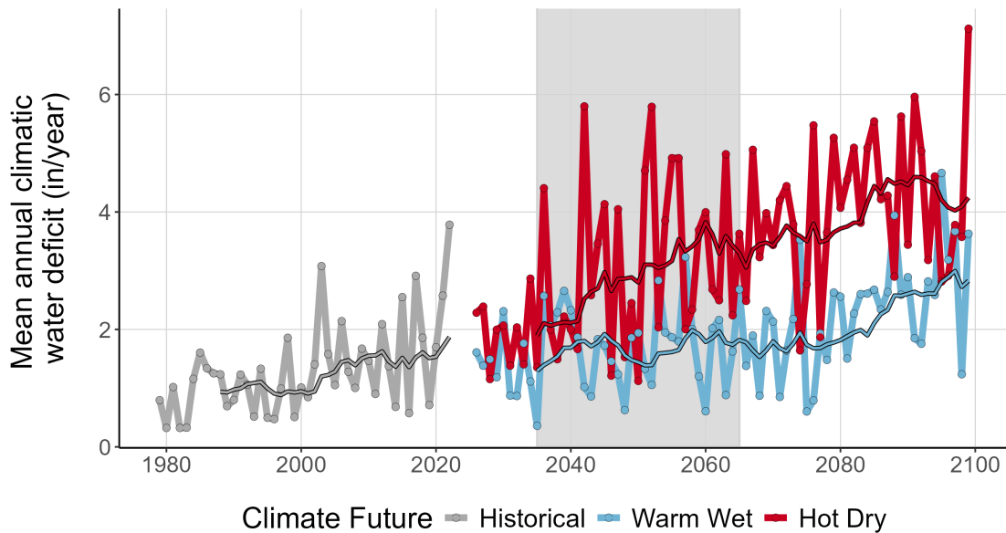
Figure 9. This line graph compares observed climatic water deficit at MORA (inches/year) (1979-2022) with projected climatic water deficit for the two climate futures over the period 2023-2099. The historical observation data is shown in gray, the Warm Wet climate future in blue, and the Hot Dry climate future in red. The smooth line running through each projection is the 10-year running average for historical observations and future projections. Gray-shaded area represents the time period that was averaged (2035-2065) to summarize future projections for the year 2050.
