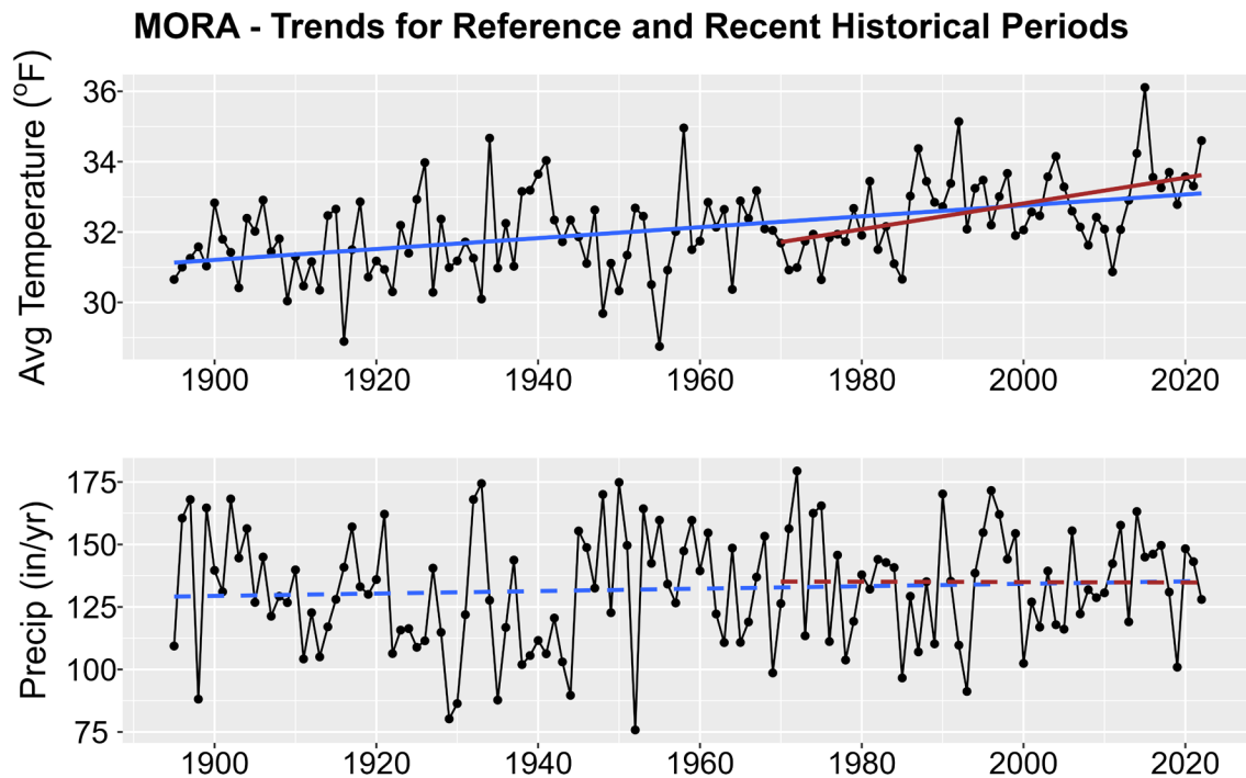
Figure 1. Historical trends in annual average temperature (upper plot) and annual total precipitation (lower plot) for MORA from 1895-2022. Black points show yearly values while blue lines are linear regressions for the entire period record and red lines for 1970-2022 trends. Solid lines are significant trends (i.e., p < 0.05 ); dashed lines are not statistically significant.
