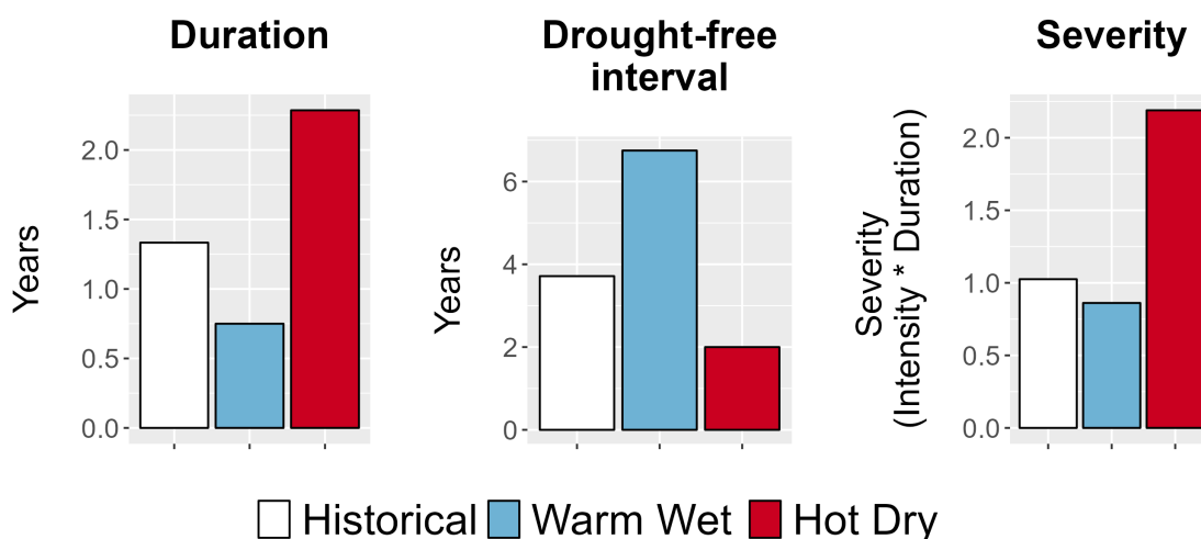
Figure 8. Drought metrics for MORA. (Left) Average drought duration (years) historically (1979-2012) and under each climate future. (Middle) Average drought return interval (years), indicating the expected amount of time between periods of drought, historically and under each climate future. (Right) Average drought severity, a measure of drought intensity multiplied by duration, historically and under each climate future.
