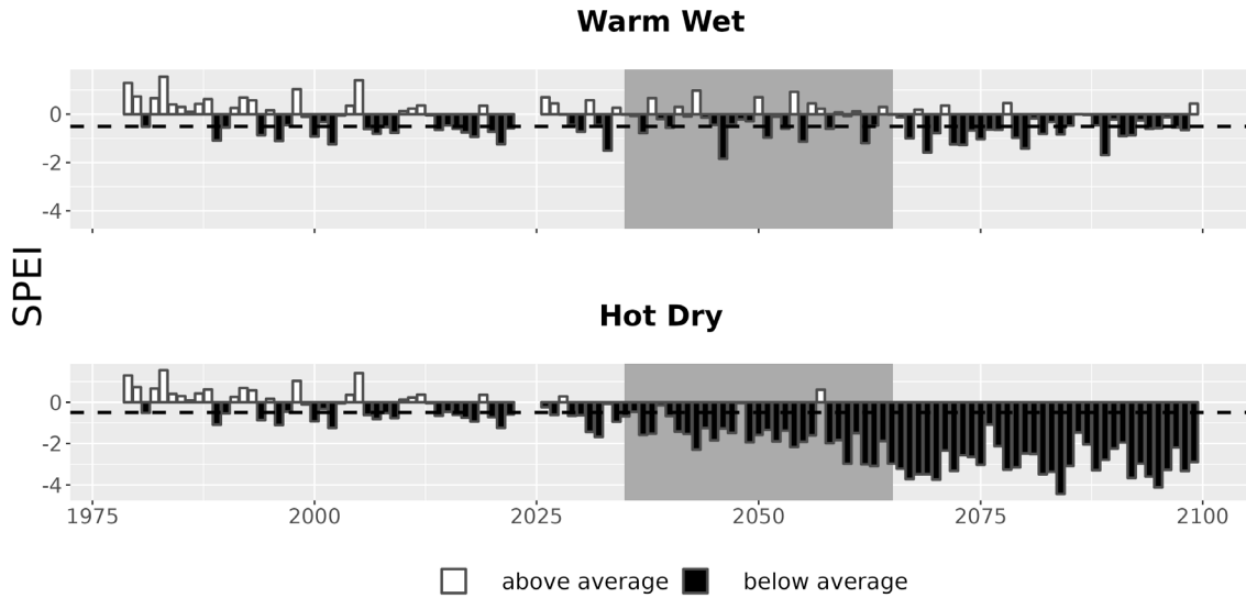
Figure 7. Drought metrics for MOJA. Drought index (SPEI; units = standard deviations from historical) timeseries for each climate future. Below-average SPEI (black bars) indicates dry conditions. The dotted line (SPEI = -0.5) indicates drought conditions.
