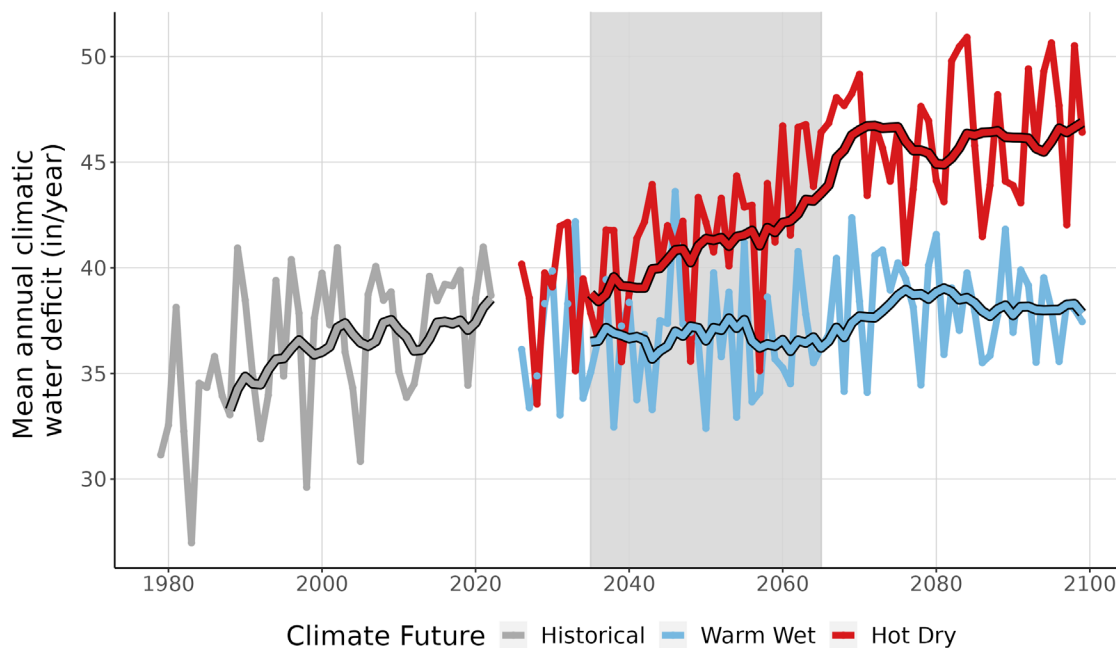
Figure 9. This line graph compares observed climatic water deficit at MOJA (inches/year) (1979-2022) with projected climatic water deficit for the two climate futures over the period 2023-2099. The historical observation data is shown in gray, the Warm Wet climate future in blue, and the Hot Dry climate future in red. The smooth line running through each projection is the 10-year running average for historical observations and future projections. Gray-shaded area represents the time period that was averaged (2035-2065) to summarize future projections for the year 2050.
