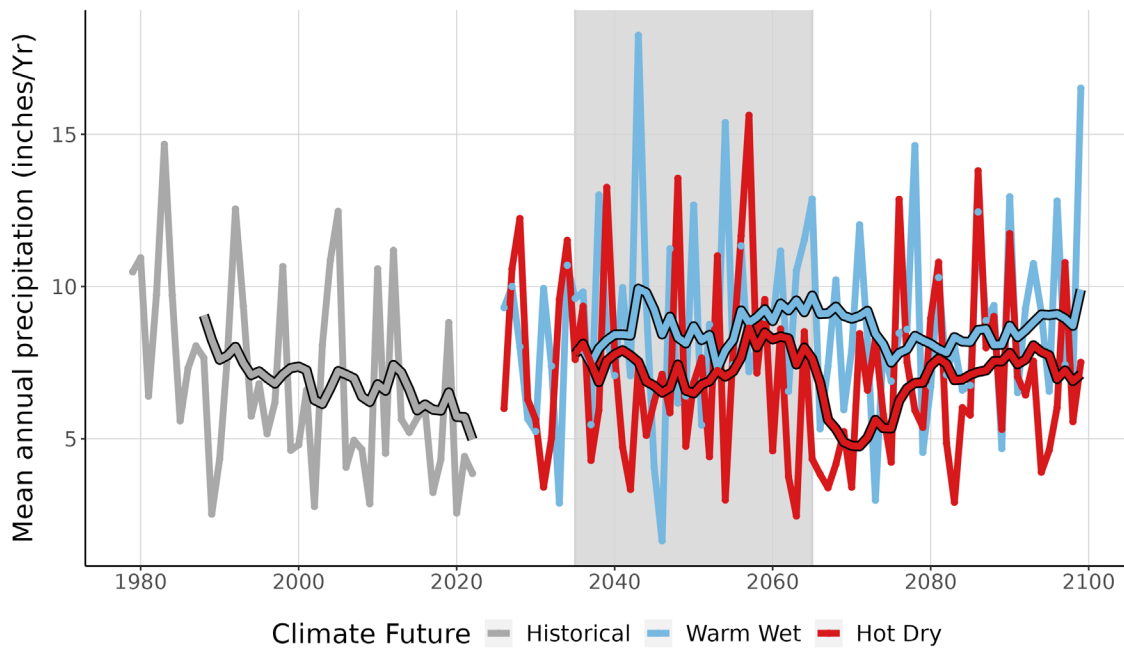
Figure 4. This graph compares observed average annual precipitation at MOJA (inches/year) (1979-2022) with projected average annual precipitation for the two climate futures over the period 2023-2099. The historically observed data is shown in gray, the Warm Wet climate future in blue, and the Hot Dry climate future in red. The smooth line running through each projection is the 10-year running average for historical observations and future projections. The gray-shaded area represents the time period that was averaged (2035-2065) to summarize future projections for the year 2050 (Appendix 1).
