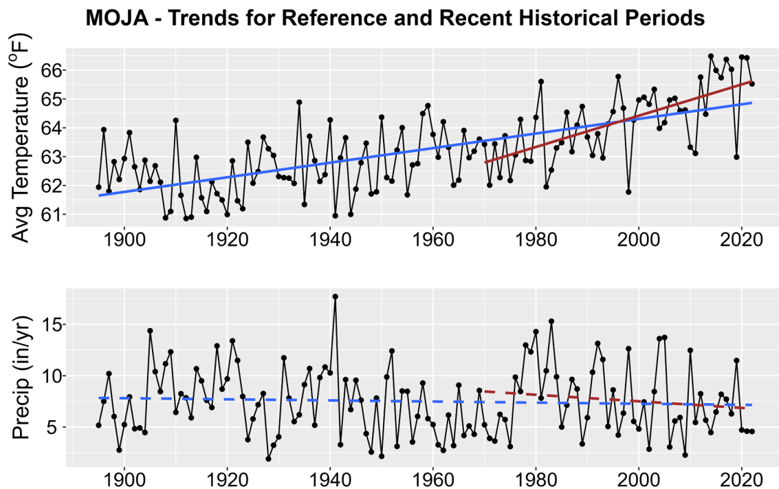
Figure 1. Historical trends in annual average temperature (upper plot) and annual total precipitation (lower plot) for MOJA from 1895-2022. Black points show yearly values while blue lines are linear regressions for the entire period record and red lines for 1970-2022 trends. Solid lines are significant trends (i.e., p < 0.05 ); dashed lines are not statistically significant.
