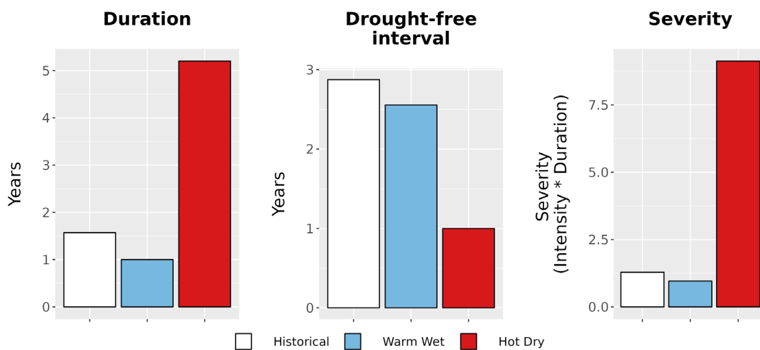
Figure 8. Drought metrics for MOJA. (Left) Average drought duration (years) historically (1979-2012) and under each climate future. (Middle) Average drought return interval (years), indicating the expected amount of time between periods of drought, historically and under each climate future. (Right) Average drought severity, a measure of drought intensity multiplied by duration, historically and under each climate future.
