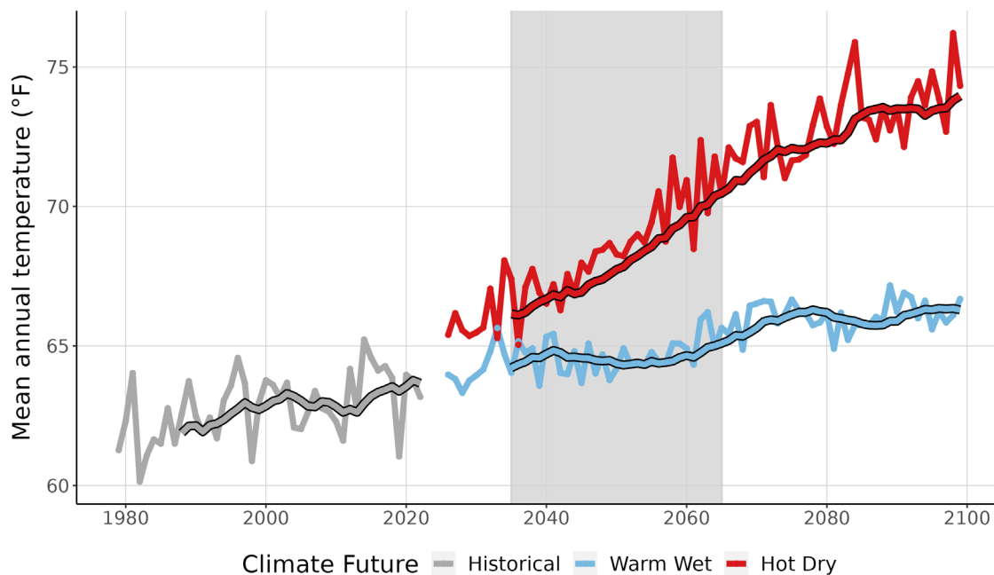
Figure 3. This graph compares observed average annual temperature at MOJA (°F) (1979-2022) with projected average annual temperature for the two climate futures over the period 2023-2099. The historically observed data is shown in gray, the Warm Wet climate future in blue, and the Hot Dry climate future in red. The smooth line running through each projection is the 10-year running average for historical observations and future projections. Gray-shaded area represents the time period that was averaged (2035-2065) to summarize future projections for the year 2050 (Appendix 1).
