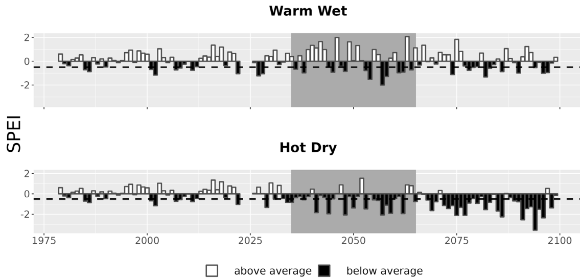
Figure 7. Drought metrics for MOCR. Drought index (SPEI; units = standard deviations from historical) timeseries for each climate future. Below-average SPEI (black bars) indicates dry conditions. The dotted line (SPEI = -0.5) indicates drought conditions.
