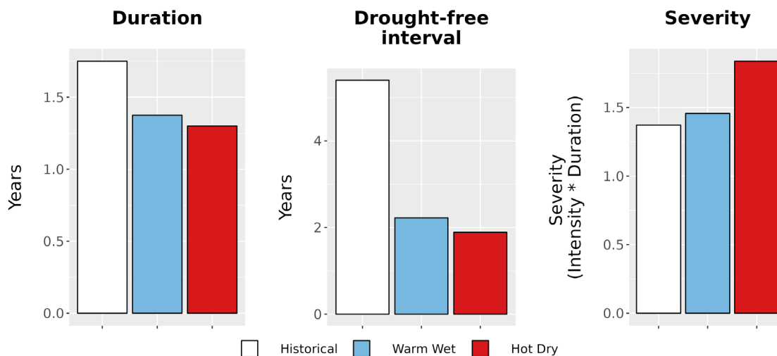
Figure 8. Drought metrics for MOCR. (Left) Average drought duration (years) historically (1979-2012) and under each climate future. (Middle) Average drought return interval (years), indicating the expected amount of time between periods of drought, historically and under each climate future. (Right) Average drought severity, a measure of drought intensity multiplied by duration, historically and under each climate future.
