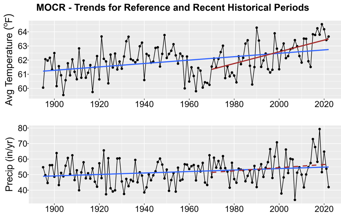
Figure 1. Historical trends in annual average temperature (upper plot) and annual total precipitation (lower plot) for MOCR from 1895-2022. Black points show yearly values while blue lines are linear regressions for the entire period record and red lines for 1970-2022 trends. Solid lines are significant trends (i.e., p < 0.05 ); dashed lines are not statistically significant.
