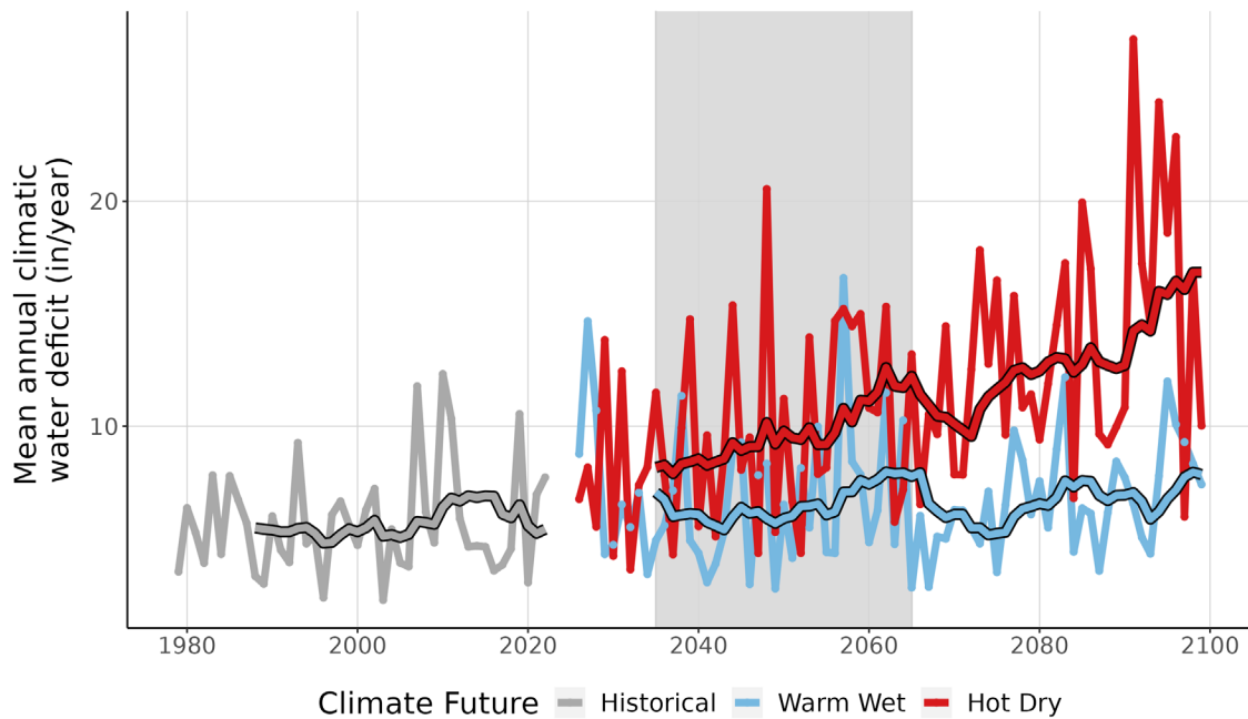
Figure 9. This line graph compares observed climatic water deficit at MOCR (inches/year) (1979-2022) with projected climatic water deficit for the two climate futures over the period 2023-2099. The historical observation data is shown in gray, the Warm Wet climate future in blue, and the Hot Dry climate future in red. The smooth line running through each projection is the 10-year running average for historical observations and future projections. Gray-shaded area represents the time period that was averaged (2035-2065) to summarize future projections for the year 2050.
