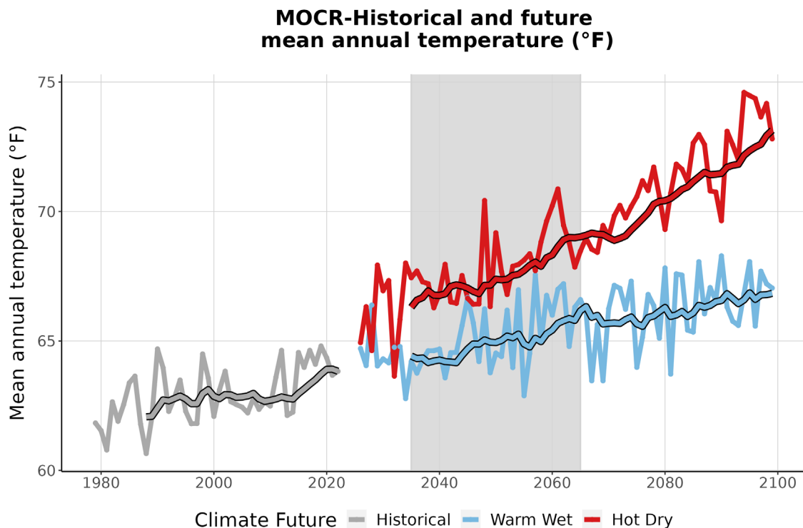
Figure 3. This graph compares observed average annual temperature at MOCR (°F) (1979-2022) with projected average annual temperature for the two climate futures over the period 2023-2099. The historically observed data
