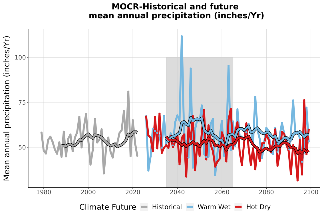
Figure 4. This graph compares observed average annual precipitation at MOCR (inches/year) (1979-2022) with projected average annual precipitation for the two climate futures over the period 2023-2099. The historically observed data is shown in gray, the Warm Wet climate future in blue, and the Hot Dry climate future in red. The smooth line running through each projection is the 10-year running average for historical observations and future projections. The gray-shaded area represents the time period that was averaged (2035-2065) to summarize future projections for the year 2050 (Appendix 1).
