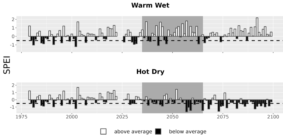
Figure 7. Drought metrics for MLKM. Drought index (SPEI; units = standard deviations from historical) timeseries for each climate future. Below-average SPEI (black bars) indicates dry conditions. The dotted line (SPEI = -0.5) indicates drought conditions.
