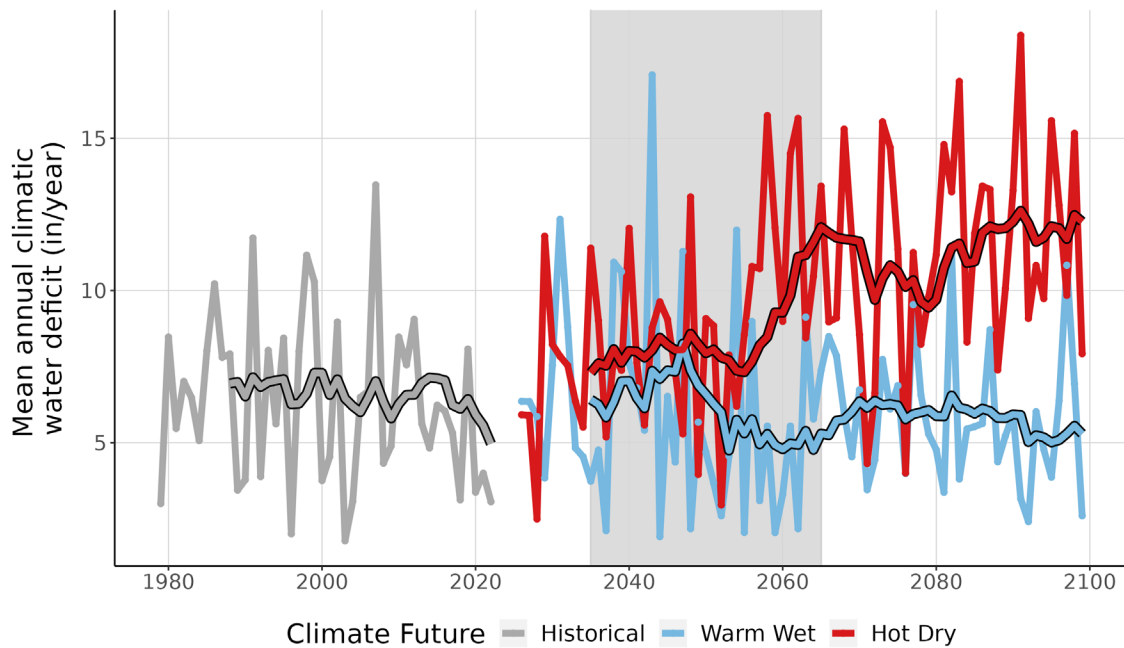
Figure 9. This line graph compares observed climatic water deficit at MLKM (inches/year) (1979-2022) with projected climatic water deficit for the two climate futures over the period 2023-2099. The historical observation data is shown in gray, the Warm Wet climate future in blue, and the Hot Dry climate future in red. The smooth line running through each projection is the 10-year running average for historical observations and future projections. Gray-shaded area represents the time period that was averaged (2035-2065) to summarize future projections for the year 2050.
