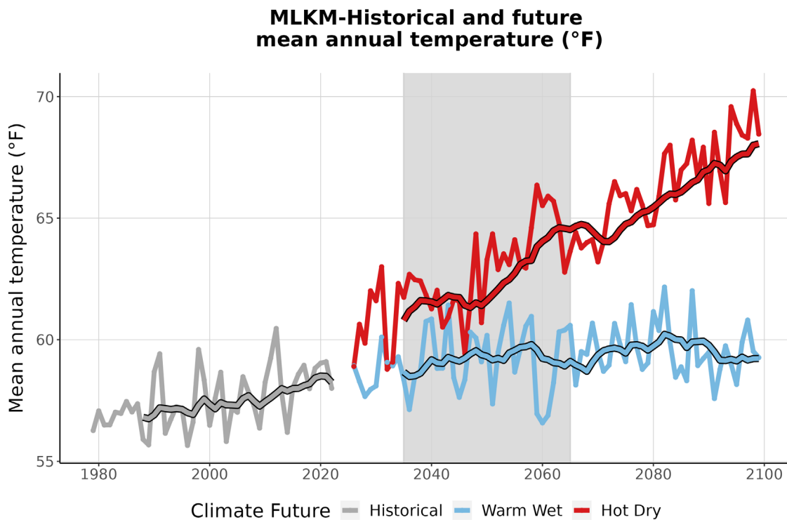
Figure 3. This graph compares observed average annual temperature at MLKM (°F) (1979-2022) with projected average annual temperature for the two climate futures over the period 2023-2099. The historically observed data is shown in gray, the Warm Wet climate future in blue, and the Hot Dry climate future in red. The smooth line
