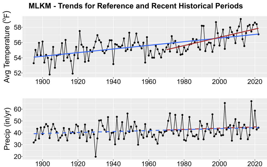
Figure 1. Historical trends in annual average temperature (upper plot) and annual total precipitation (lower plot) for MLKM from 1895-2022. Black points show yearly values while blue lines are linear regressions for the entire period record and red lines for 1970-2022 trends. Solid lines are significant trends (i.e., p < 0.05 ); dashed lines are not statistically significant.
