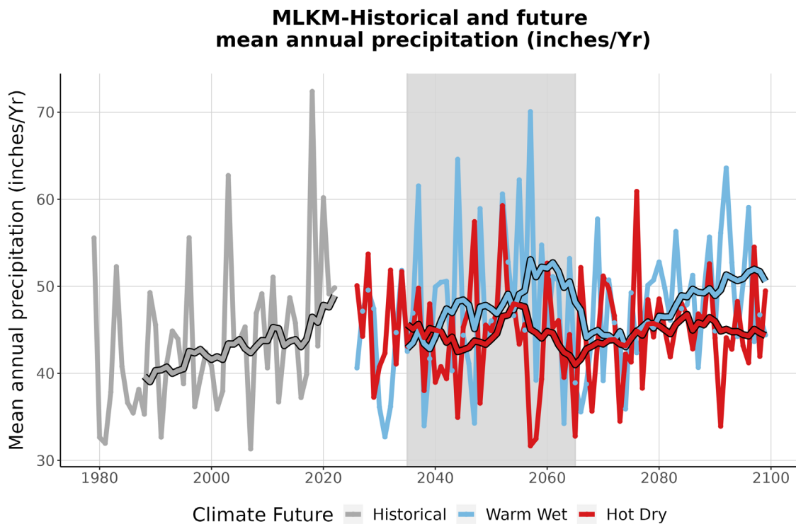
Figure 4. This graph compares observed average annual precipitation at MLMK (inches/year) (1979-2022) with projected average annual precipitation for the two climate futures over the period 2023-2099. The historically observed data is shown in gray, the Warm Wet climate future in blue, and the Hot Dry climate future in red. The smooth line running through each projection is the 10-year running average for historical observations and future projections. The gray-shaded area represents the time period that was averaged (2035-2065) to summarize future projections for the year 2050 (Appendix 1).
