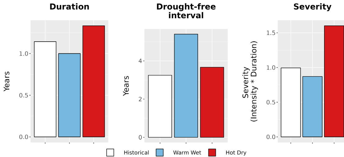
Figure 8. Drought metrics for MLKM. (Left) Average drought duration (years) historically (1979-2012) and under each climate future. (Middle) Average drought return interval (years), indicating the expected amount of time between periods of drought, historically and under each climate future. (Right) Average drought severity, a measure of drought intensity multiplied by duration, historically and under each climate future.
