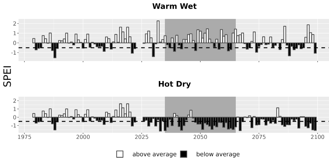
Figure 7. Drought metrics for MISS. Drought index (SPEI; units = standard deviations from historical) timeseries for each climate future. Below-average SPEI (black bars) indicates dry conditions. The dotted line (SPEI = -0.5) indicates drought conditions.
