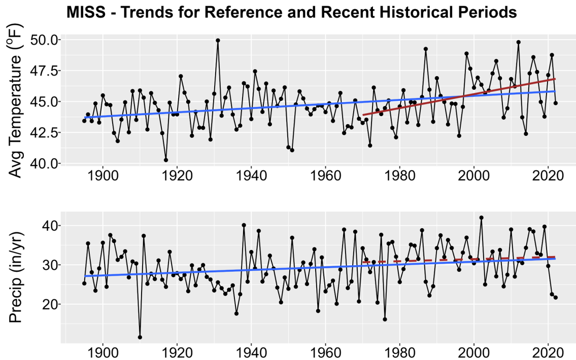
Figure 1. Historical trends in annual average temperature (upper plot) and annual total precipitation (lower plot) for MISS from 1895-2022. Black points show yearly values while blue lines are linear regressions for the entire period record and red lines for 1970-2022 trends. Solid lines are significant trends (i.e., p < 0.05 ); dashed lines are not statistically significant.
