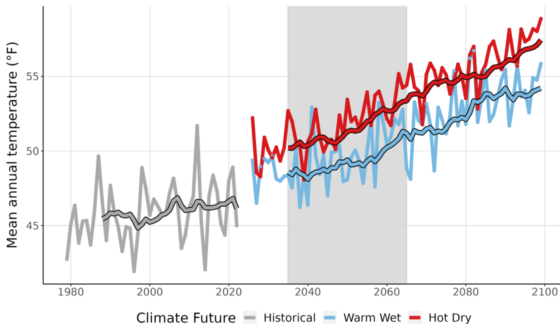
Figure 3. This graph compares observed average annual temperature at MISS (°F) (1979-2022) with projected average annual temperature for the two climate futures over the period 2023-2099. The historically observed data is shown in gray, the Warm Wet climate future in blue, and the Hot Dry climate future in red. The smooth line running through each projection is the 10-year running average for historical observations and future projections. Gray-shaded area represents the time period that was averaged (2035-2065) to summarize future projections for the year 2050 (Appendix 1).
