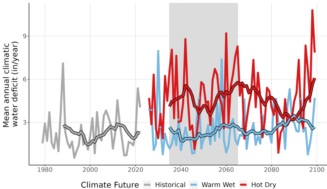
Figure 9. This line graph compares observed climatic water deficit at MISS (inches/year) (1979-2022) with projected climatic water deficit for the two climate futures over the period 2023-2099. The historical observation data is shown in gray, the Warm Wet climate future in blue, and the Hot Dry climate future in red. The smooth line running through each projection is the 10-year running average for historical observations and future projections. Gray-shaded area represents the time period that was averaged (2035-2065) to summarize future projections for the year 2050.
