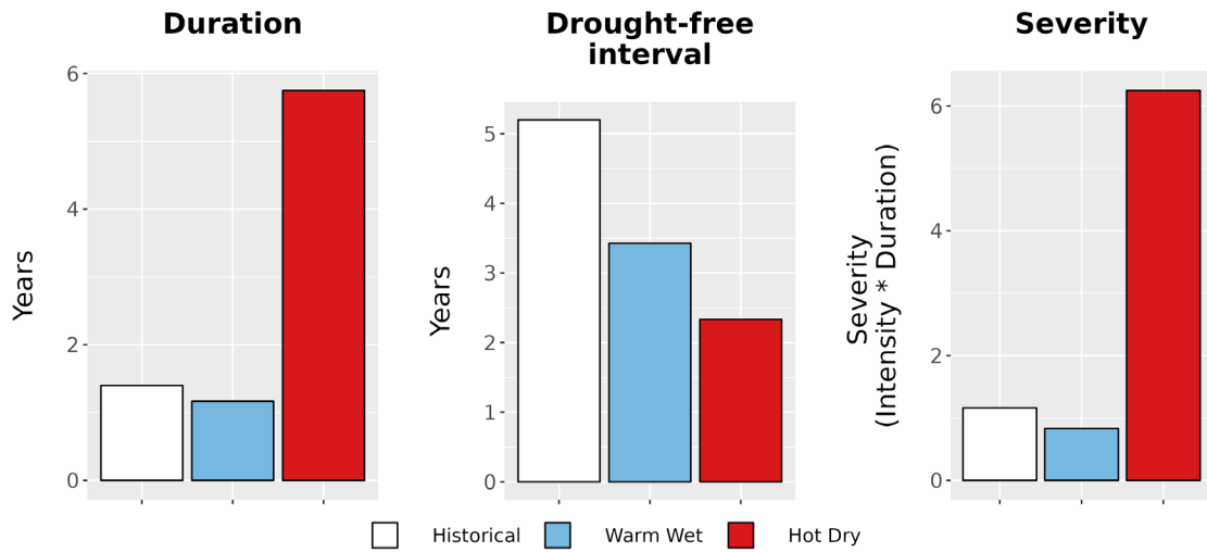
Figure 8. Drought metrics for MISS. (Left) Average drought duration (years) historically (1979-2012) and under each climate future. (Middle) Average drought return interval (years), indicating the expected amount of time between periods of drought, historically and under each climate future. (Right) Average drought severity, a measure of drought intensity multiplied by duration, historically and under each climate future.
