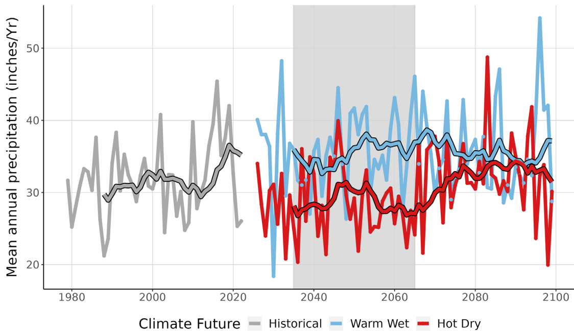
Figure 4. This graph compares observed average annual precipitation at MISS (inches/year) (1979-2022) with projected average annual precipitation for the two climate futures over the period 2023-2099. The historically observed data is shown in gray, the Warm Wet climate future in blue, and the Hot Dry climate future in red. The smooth line running through each projection is the 10-year running average for historical observations and future projections. The gray-shaded area represents the time period that was averaged (2035-2065) to summarize future projections for the year 2050 (Appendix 1).
