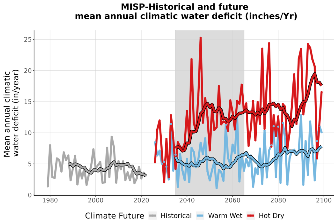
Figure 9. This line graph compares observed climatic water deficit at MISP (inches/year) (1979-2022) with projected climatic water deficit for the two climate futures over the period 2023-2099. The historical observation data is shown in gray, the Warm Wet climate future in blue, and the Hot Dry climate future in red. The smooth line running through each projection is the 10-year running average for historical observations and future projections. Gray-shaded area represents the time period that was averaged (2035-2065) to summarize future projections for the year 2050.
