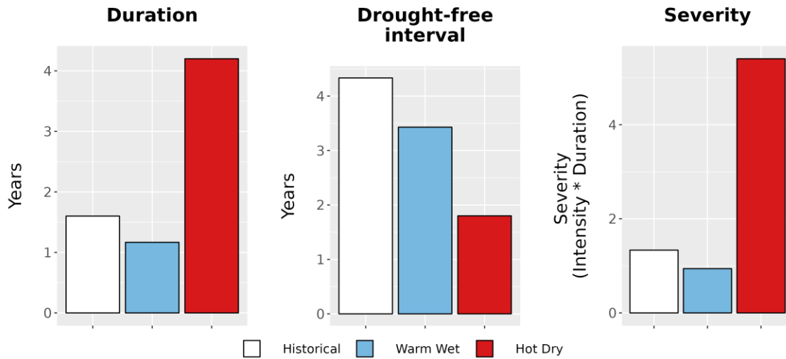
Figure 8. Drought metrics for MISP. (Left) Average drought duration (years) historically (1979-2012) and under each climate future. (Middle) Average drought return interval (years), indicating the expected amount of time between periods of drought, historically and under each climate future. (Right) Average drought severity, a measure of drought intensity multiplied by duration, historically and under each climate future.
