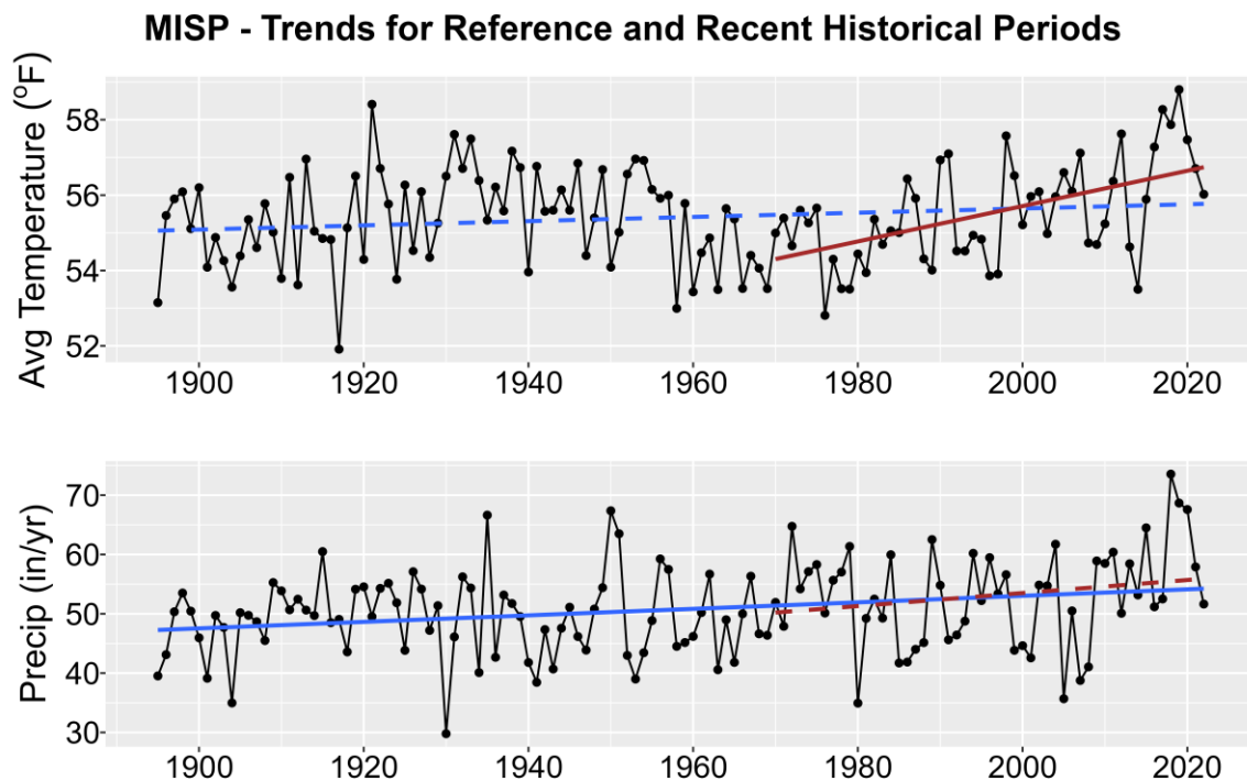
Figure 1. Historical trends in annual average temperature (upper plot) and annual total precipitation (lower plot) for MISP from 1895-2022. Black points show yearly values while blue lines are linear regressions for the entire period record and red lines for 1970-2022 trends. Solid lines are significant trends (i.e., p < 0.05 ); dashed lines are not statistically significant.
