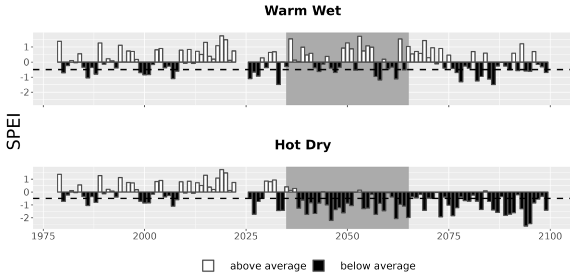
Figure 7. Drought metrics for MISP. Drought index (SPEI; units = standard deviations from historical) timeseries for each climate future. Below-average SPEI (black bars) indicates dry conditions. The dotted line (SPEI = -0.5) indicates drought conditions.
