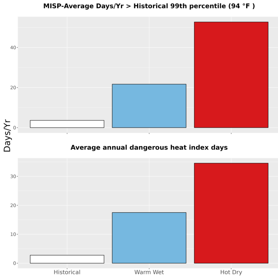
Figure 5. The upper bar graph represents the average number of days annually with temperatures greater than the historical 99th percentile (94 °F) historically (1979-2012) and for the two climate futures (2050). The bottom bar graph represents the average annual number of dangerous heat index days historically and for the two climate futures. Dangerous heat index days are days that exceed 105 °F.
