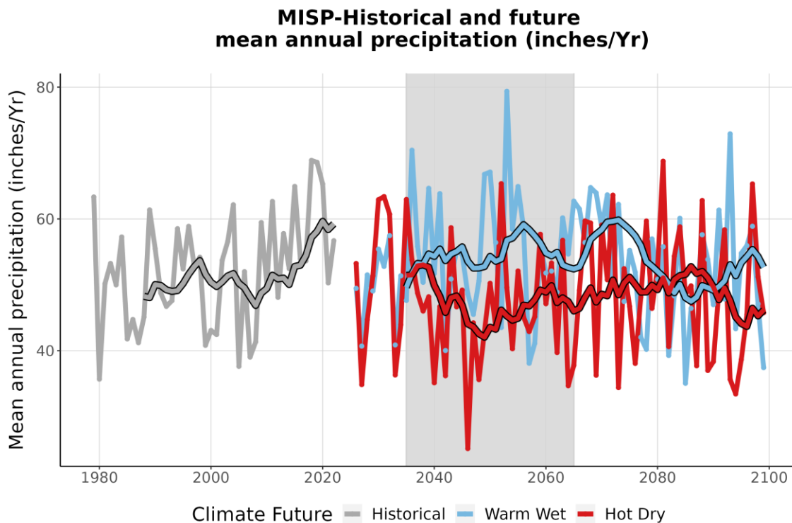
Figure 4. This graph compares observed average annual precipitation at MISP (inches/year) (1979-2022) with projected average annual precipitation for the two climate futures over the period 2023-2099. The historically observed data is shown in gray, the Warm Wet climate future in blue, and the Hot Dry climate future in red. The smooth line running through each projection is the 10-year running average for historical observations and future projections. The gray-shaded area represents the time period that was averaged (2035-2065) to summarize future projections for the year 2050 (Appendix 1).
