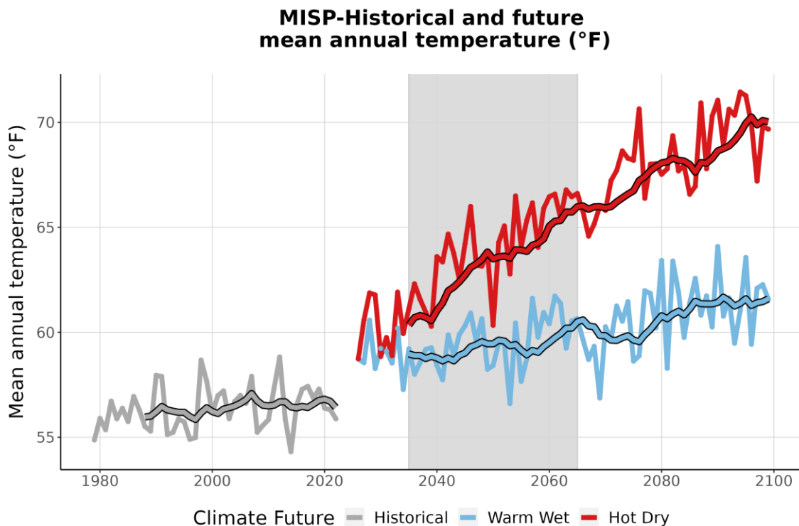
Figure 3. This graph compares observed average annual temperature at MISP (°F) (1979-2022) with projected average annual temperature for the two climate futures over the period 2023-2099. The historically observed data
