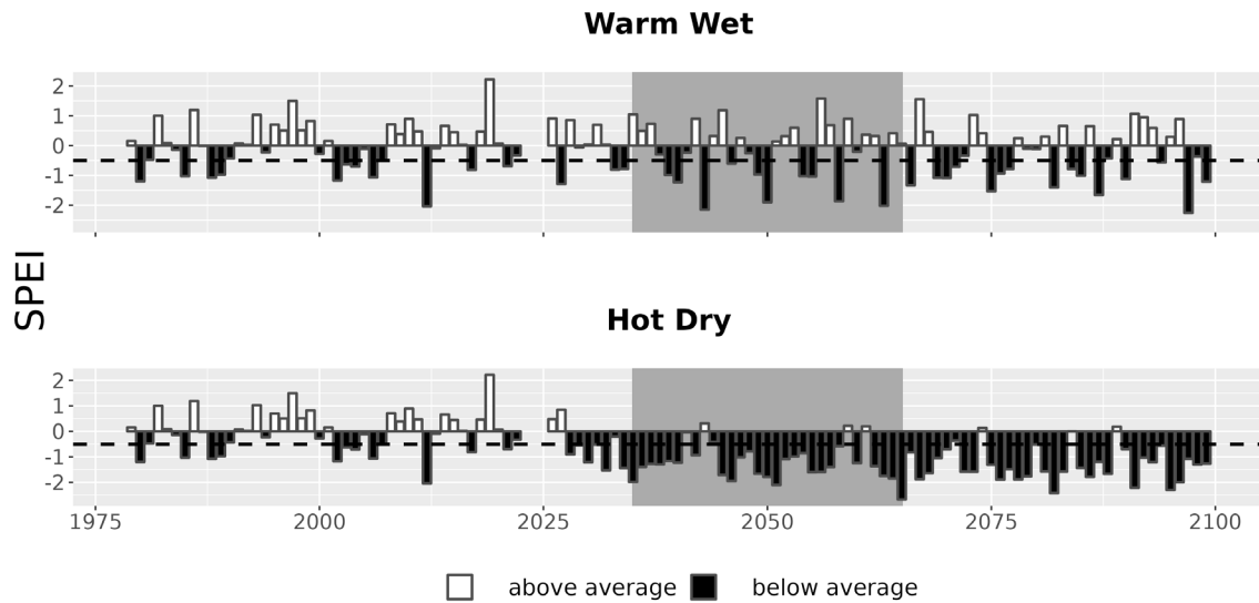
Figure 7. Drought metrics for MIMI. Drought index (SPEI; units = standard deviations from historical) timeseries for each climate future. Below-average SPEI (black bars) indicates dry conditions. The dotted line (SPEI = -0.5) indicates drought conditions.
