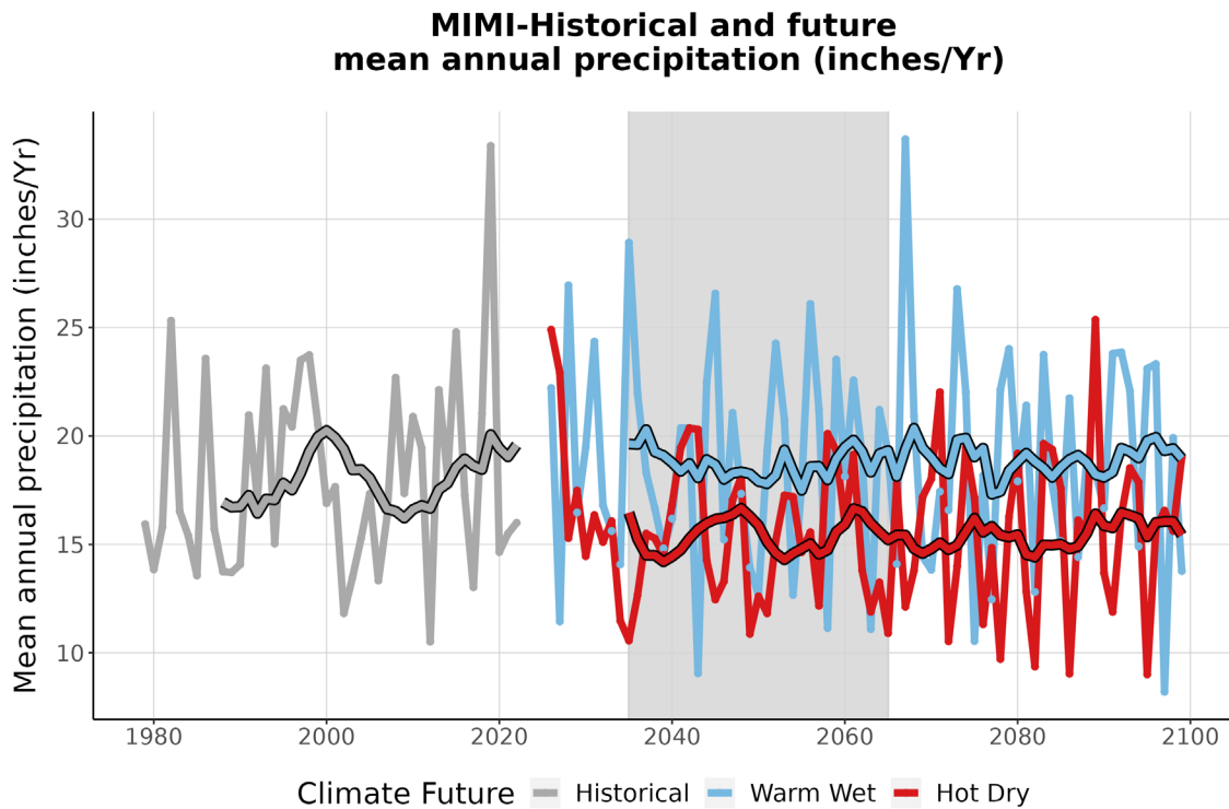
Figure 4. This graph compares observed average annual precipitation at MIMI (inches/year) (1979-2022) with projected average annual precipitation for the two climate futures over the period 2023-2099. The historically observed data is shown in gray, the Warm Wet climate future in blue, and the Hot Dry climate future in red. The smooth line running through each projection is the 10-year running average for historical observations and future projections. The gray-shaded area represents the time period that was averaged (2035-2065) to summarize future projections for the year 2050 (Appendix 1).
