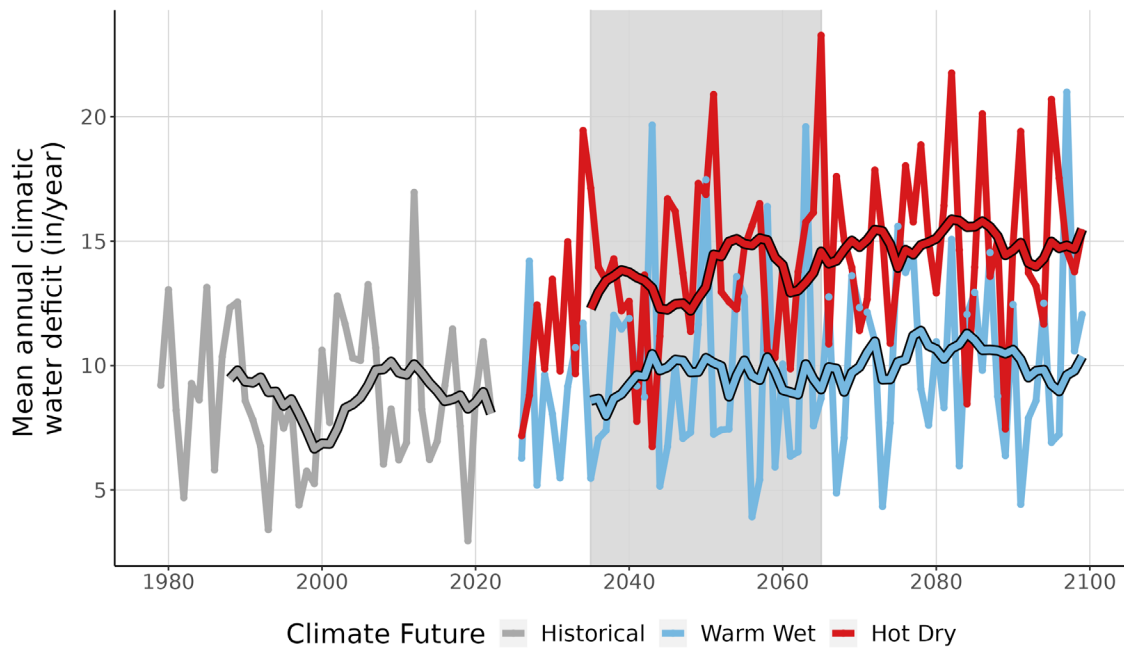
Figure 9. This line graph compares observed climatic water deficit at MIMI (inches/year) (1979-2022) with projected climatic water deficit for the two climate futures over the period 2023-2099. The historical observation data is shown in gray, the Warm Wet climate future in blue, and the Hot Dry climate future in red. The smooth line running through each projection is the 10-year running average for historical observations and future projections. Gray-shaded area represents the time period that was averaged (2035-2065) to summarize future projections for the year 2050.
