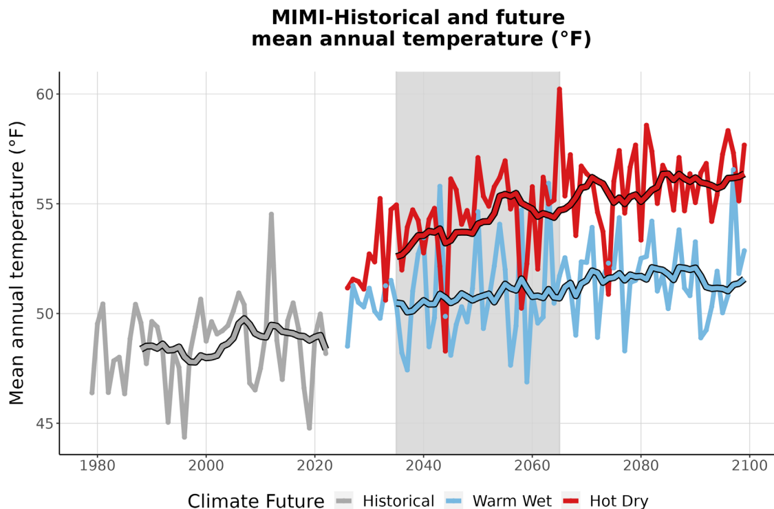
Figure 3. This graph compares observed average annual temperature at MIMI (°F) (1979-2022) with projected average annual temperature for the two climate futures over the period 2023-2099. The historically observed data
