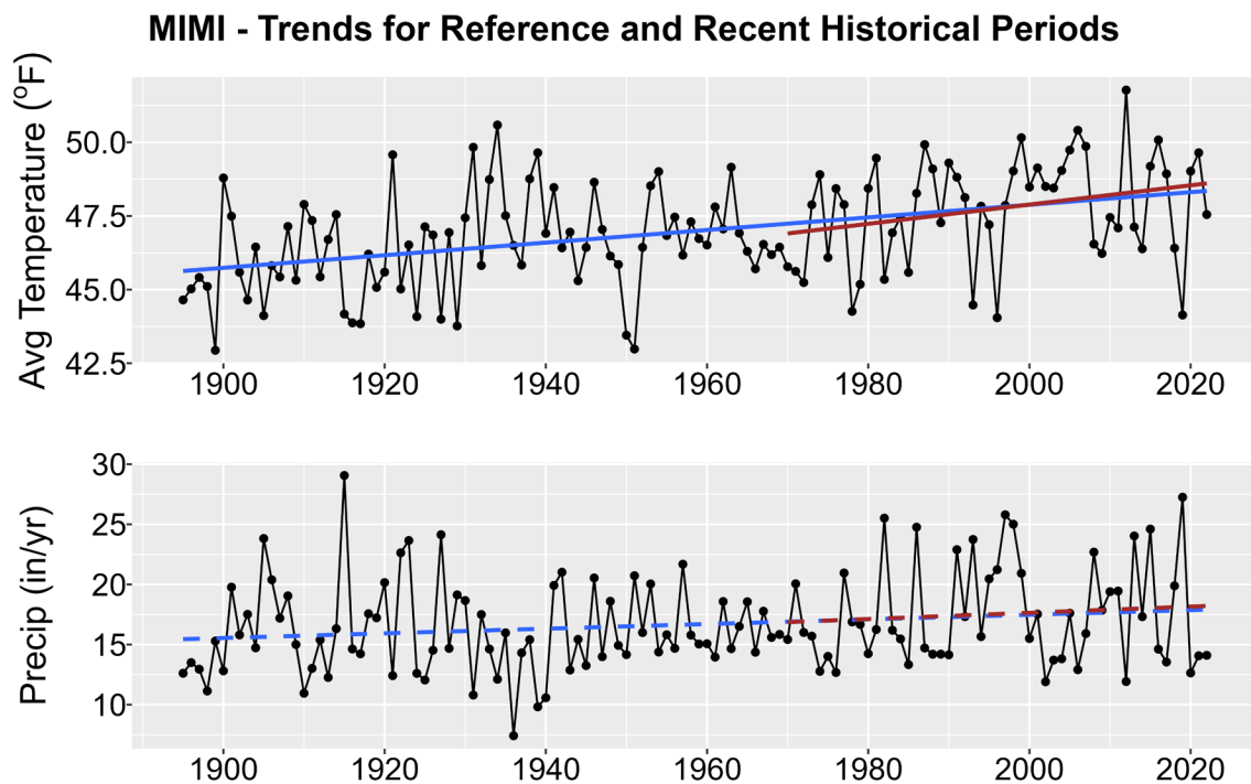
Figure 1. Historical trends in annual average temperature (upper plot) and annual total precipitation (lower plot) for MIMI from 1895-2022. Black points show yearly values while blue lines are linear regressions for the entire period record and red lines for 1970-2022 trends. Solid lines are significant trends (i.e., p < 0.05 ); dashed lines are not statistically significant.
