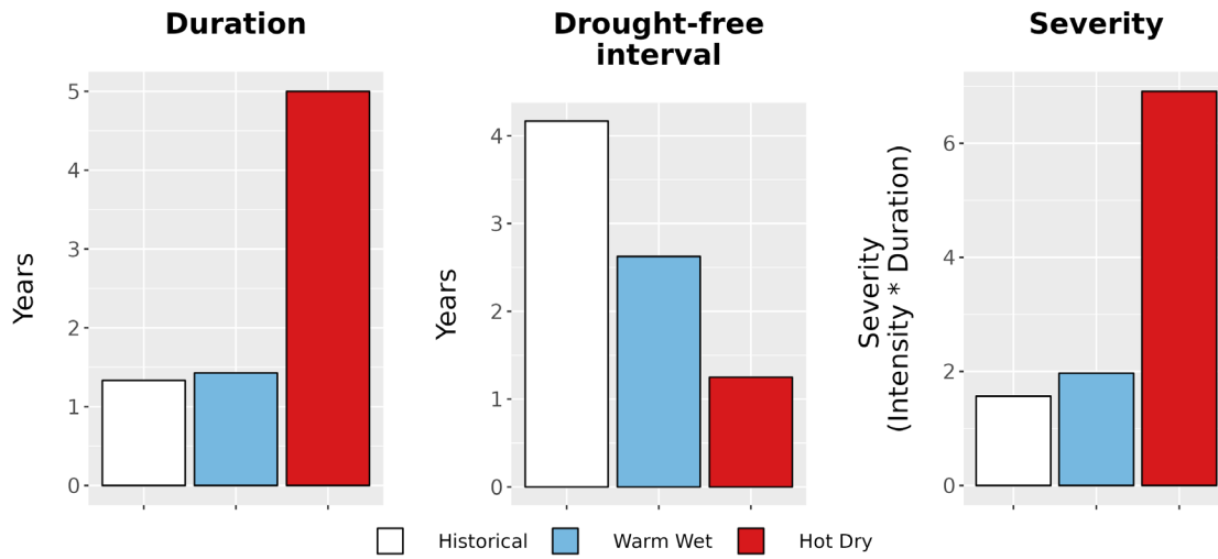
Figure 8. Drought metrics for MIMI. (Left) Average drought duration (years) historically (1979-2012) and under each climate future. (Middle) Average drought return interval (years), indicating the expected amount of time between periods of drought, historically and under each climate future. (Right) Average drought severity, a measure of drought intensity multiplied by duration, historically and under each climate future.
