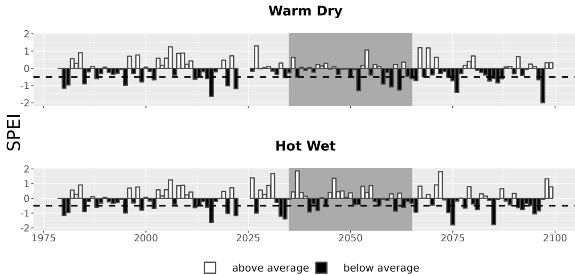
Figure 7. Drought metrics for MIMA. Drought index (SPEI; units = standard deviations from historical) timeseries for each climate future. Below-average SPEI (black bars) indicates dry conditions. The dotted line (SPEI = -0.5) indicates drought conditions.
