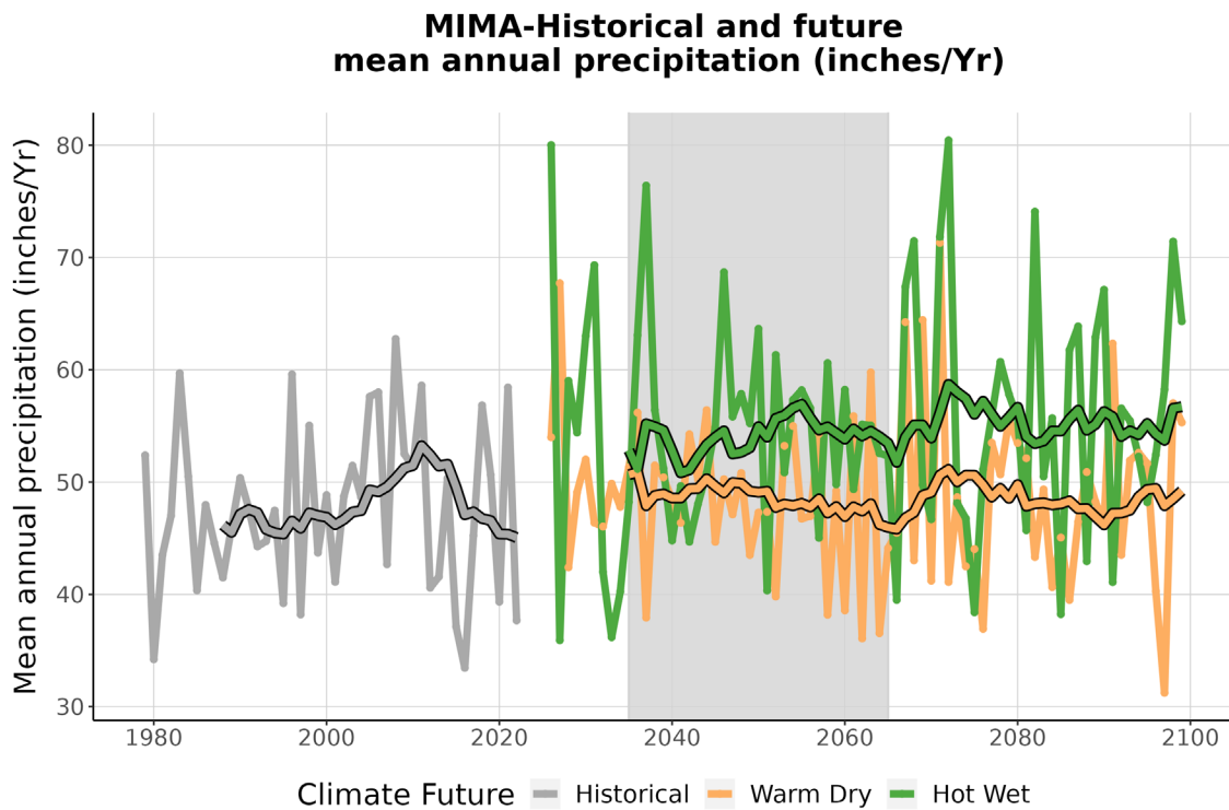
Figure 4. This graph compares observed average annual precipitation at MIMA (inches/year) (1979-2022) with projected average annual precipitation for the two climate futures over the period 2023-2099. The historically observed data is shown in gray, the Warm Dry climate future in orange, and the Hot Wet climate future in green. The smooth line running through each projection is the 10-year running average for historical observations and future projections. The gray-shaded area represents the time period that was averaged (2035-2065) to summarize future projections for the year 2050 (Appendix 1).
