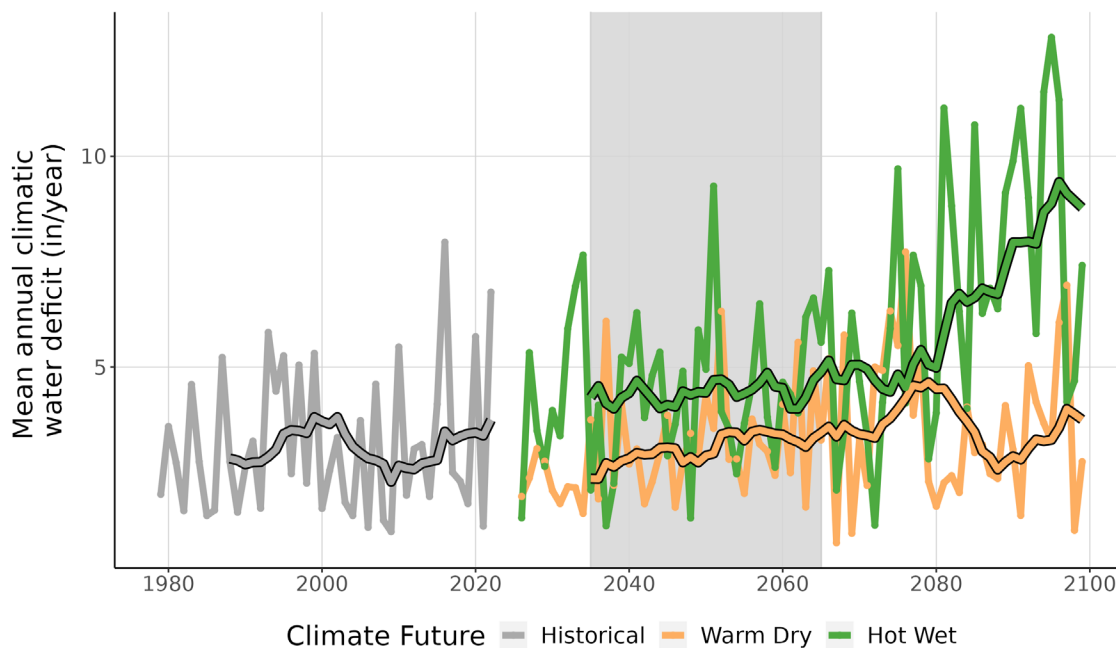
Figure 9. This line graph compares observed climatic water deficit at MIMA (inches/year) (1979-2022) with projected climatic water deficit for the two climate futures over the period 2023-2099. The historical observation data is shown in gray, the Warm Dry climate future in orange, and the Hot Wet climate future in green. The smooth line running through each projection is the 10-year running average for historical observations and future projections. Gray-shaded area represents the time period that was averaged (2035-2065) to summarize future projections for the year 2050.
