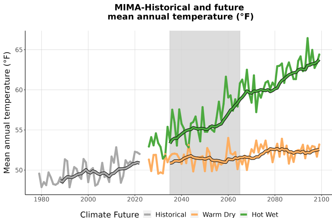
Figure 3. This graph compares observed average annual temperature at MIMA (°F) (1979-2022) with projected average annual temperature for the two climate futures over the period 2023-2099. The historically observed data
