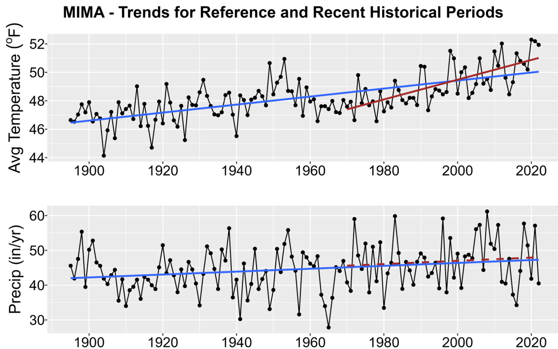
Figure 1. Historical trends in annual average temperature (upper plot) and annual total precipitation (lower plot) for MIMA from 1895-2022. Black points show yearly values while blue lines are linear regressions for the entire period record and red lines for 1970-2022 trends. Solid lines are significant trends (i.e., p < 0.05 ); dashed lines are not statistically significant.
