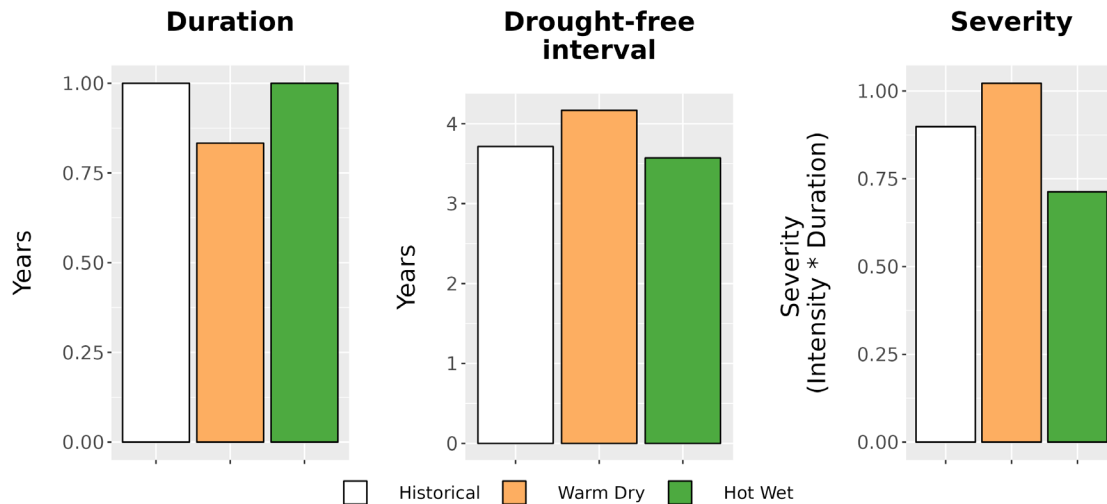
Figure 8. Drought metrics for MIMA. (Left) Average drought duration (years) historically (1979-2012) and under each climate future. (Middle) Average drought return interval (years), indicating the expected amount of time between periods of drought, historically and under each climate future. (Right) Average drought severity, a measure of drought intensity multiplied by duration, historically and under each climate future.
