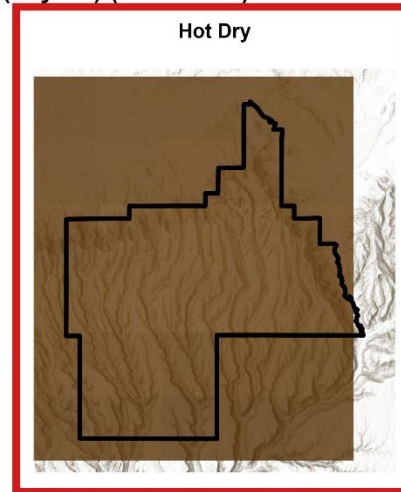
Figure A3. (Top) Map showing average annual climatic water deficit for the historical period (inches/year) and (bottom) change in average annual climatic water deficit for the two climate futures. Legends are located below each set of maps as a continuous color gradient. Gridded data is extracted from 30-year summary GIS layers for CONUS water balance model (Tercek et al 2021, 2023). ( http://screenedcleanedsummaries.s3-website-us-west-2.amazonaws.com/ ) accessed on 6/3/2024.
