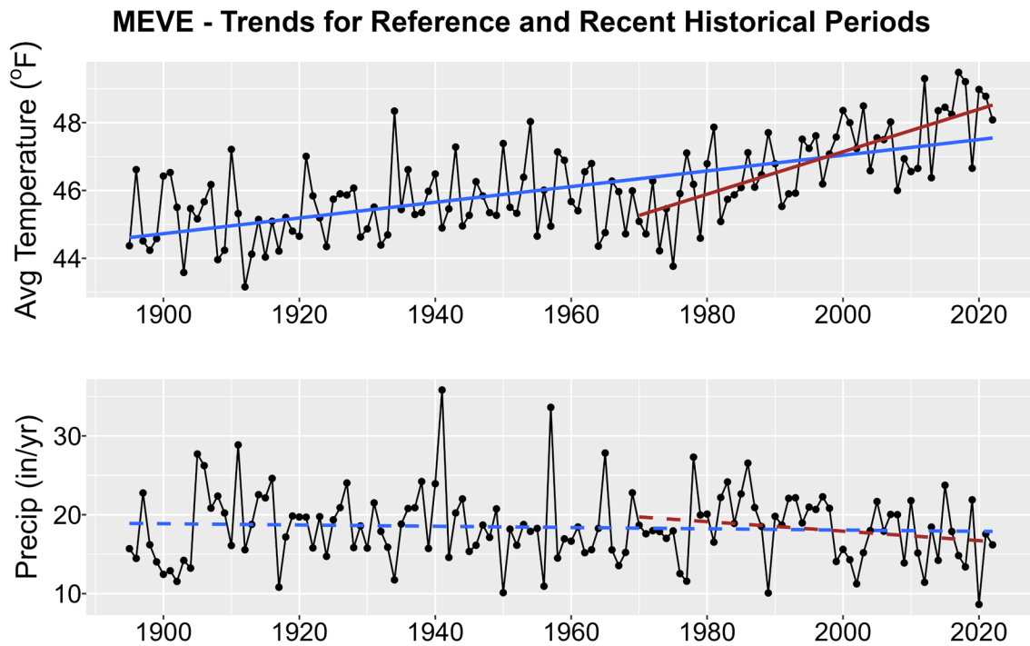
Figure 1. Historical trends in annual average temperature (upper plot) and annual total precipitation (lower plot) for MEVE from 1895-2022. Black points show yearly values while blue lines are linear regressions for the entire period record and red lines for 1970-2022 trends. Solid lines are significant trends (i.e., p < 0.05 ); dashed lines are not statistically significant.
