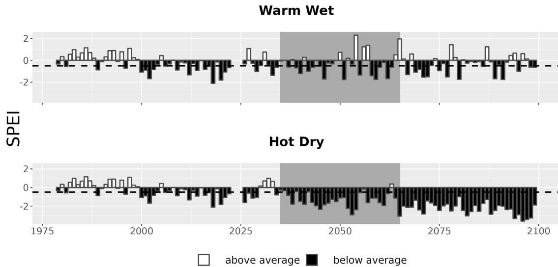
Figure 7. Drought metrics for MEVE. Drought index (SPEI; units = standard deviations from historical) timeseries for each climate future. Below-average SPEI (black bars) indicates dry conditions. The dotted line (SPEI = -0.5) indicates drought conditions.
