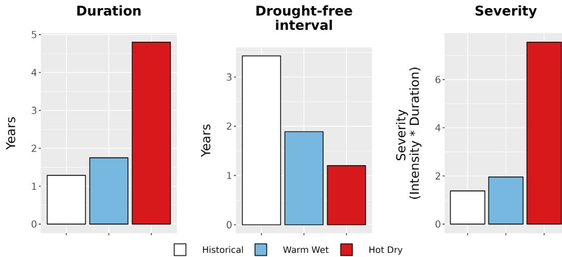
Figure 8. Drought metrics for MEVE. (Left) Average drought duration (years) historically (1979-2012) and under each climate future. (Middle) Average drought return interval (years), indicating the expected amount of time between periods of drought, historically and under each climate future. (Right) Average drought severity, a measure of drought intensity multiplied by duration, historically and under each climate future.
