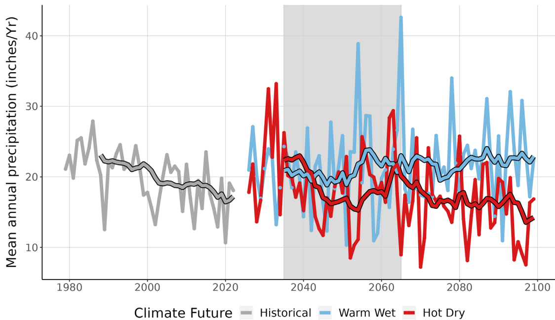
Figure 4. This graph compares observed average annual precipitation at MEVE (inches/year) (1979-2022) with projected average annual precipitation for the two climate futures over the period 2023-2099. The historically observed data is shown in gray, the Warm Wet climate future in blue, and the Hot Dry climate future in red. The smooth line running through each projection is the 10-year running average for historical observations and future projections. The gray-shaded area represents the time period that was averaged (2035-2065) to summarize future projections for the year 2050 (Appendix 1).
