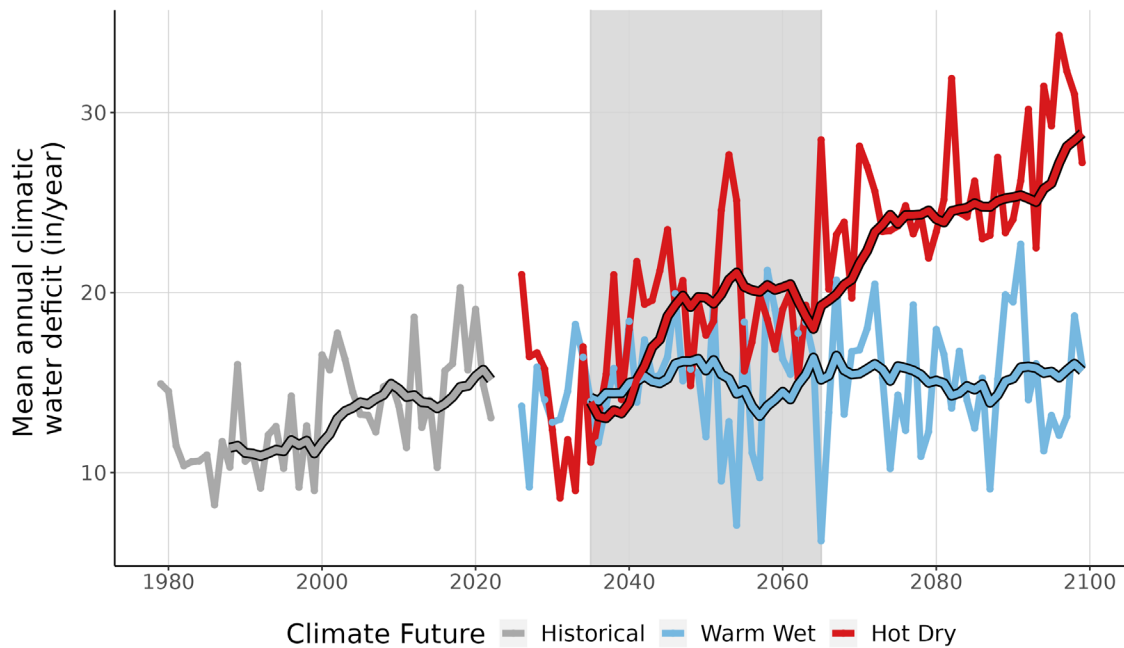
Figure 9. This line graph compares observed climatic water deficit at MEVE (inches/year) (1979-2022) with projected climatic water deficit for the two climate futures over the period 2023-2099. The historical observation data is shown in gray, the Warm Wet climate future in blue, and the Hot Dry climate future in red. The smooth line running through each projection is the 10-year running average for historical observations and future projections. Gray-shaded area represents the time period that was averaged (2035-2065) to summarize future projections for the year 2050.
