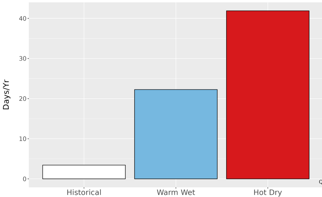
Figure 5. Metrics of extreme temperature at MEVE. The bar graph represents the average number of days annually with temperatures greater than the historical 99th percentile (89.5 °F) historically (1979-2012) and for the two climate futures (2050).
