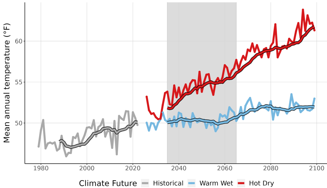
Figure 3. This graph compares observed average annual temperature at MEVE (°F) (1979-2022) with projected average annual temperature for the two climate futures over the period 2023-2099. The historically observed data is shown in gray, the Warm Wet climate future in blue, and the Hot Dry climate future in red. The smooth line running through each projection is the 10-year running average for historical observations and future projections. Gray-shaded area represents the time period that was averaged (2035-2065) to summarize future projections for the year 2050 (Appendix 1).
