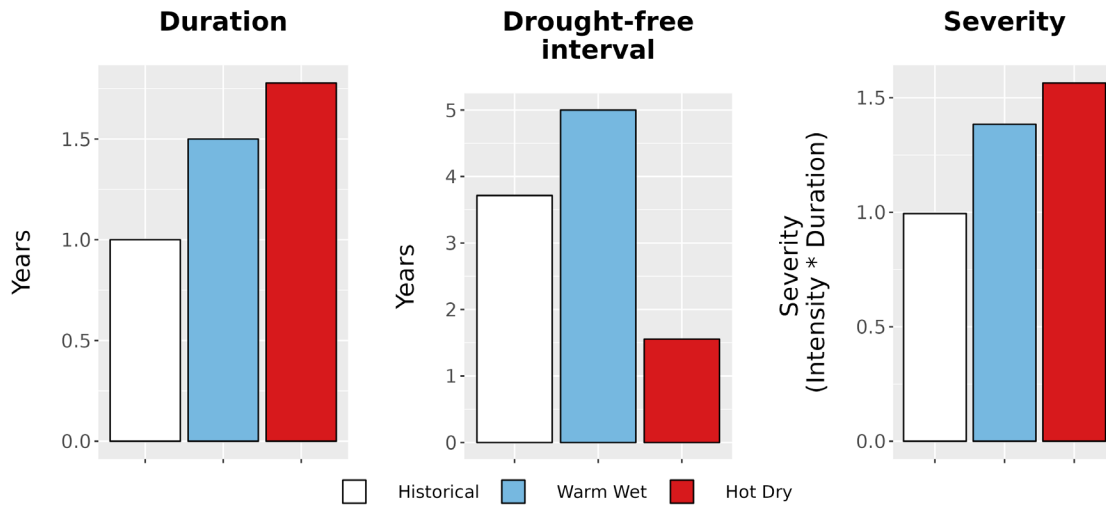
Figure 8. Drought metrics for MANA. (Left) Average drought duration (years) historically (1979-2012) and under each climate future. (Middle) Average drought return interval (years), indicating the expected amount of time between periods of drought, historically and under each climate future. (Right) Average drought severity, a measure of drought intensity multiplied by duration, historically and under each climate future.
