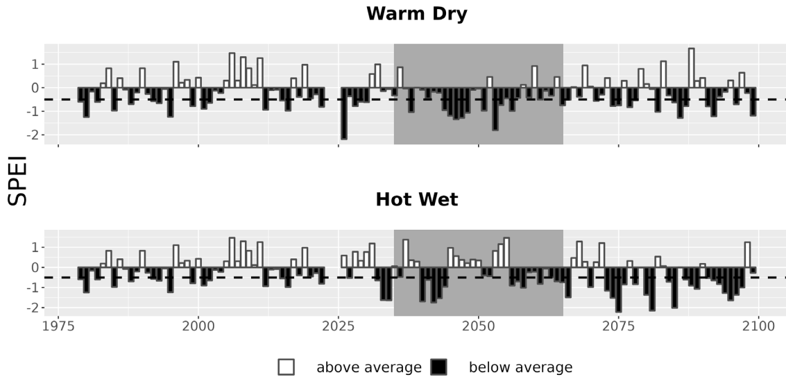
Figure 7. Drought metrics for MABI. Drought index (SPEI; units = standard deviations from historical) timeseries for each climate future. Below-average SPEI (black bars) indicates dry conditions. The dotted line (SPEI = -0.5) indicates drought conditions.
