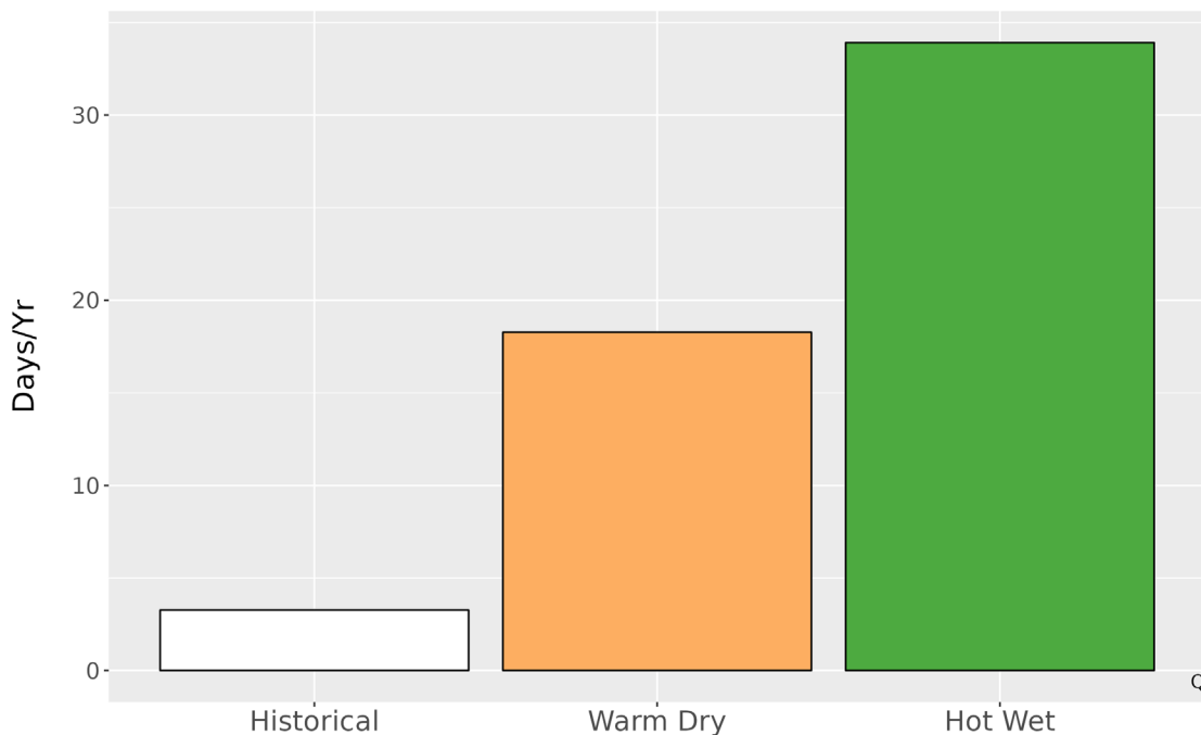
Figure 5. Metrics of extreme temperature at MABI. The bar graph represents the average number of days annually with temperatures greater than the historical 99th percentile (87.5 °F) historically (1979-2012) and for the two climate futures (2050).
