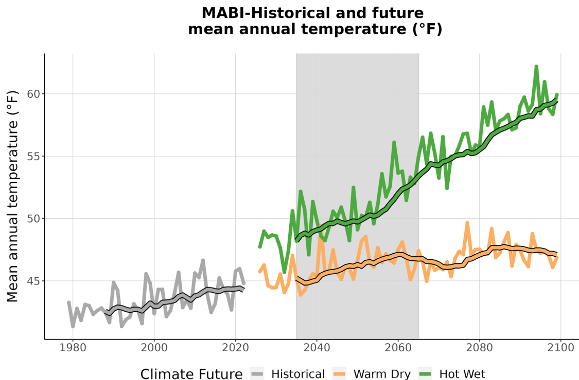
Figure 3. This graph compares observed average annual temperature at MABI (°F) (1979-2022) with projected average annual temperature for the two climate futures over the period 2023-2099. The historically observed data
