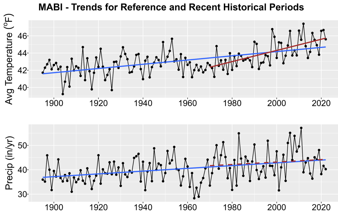
Figure 1. Historical trends in annual average temperature (upper plot) and annual total precipitation (lower plot) for MABI from 1895-2022. Black points show yearly values while blue lines are linear regressions for the entire period record and red lines for 1970-2022 trends. Solid lines are significant trends (i.e., p < 0.05 ); dashed lines are not statistically significant.
