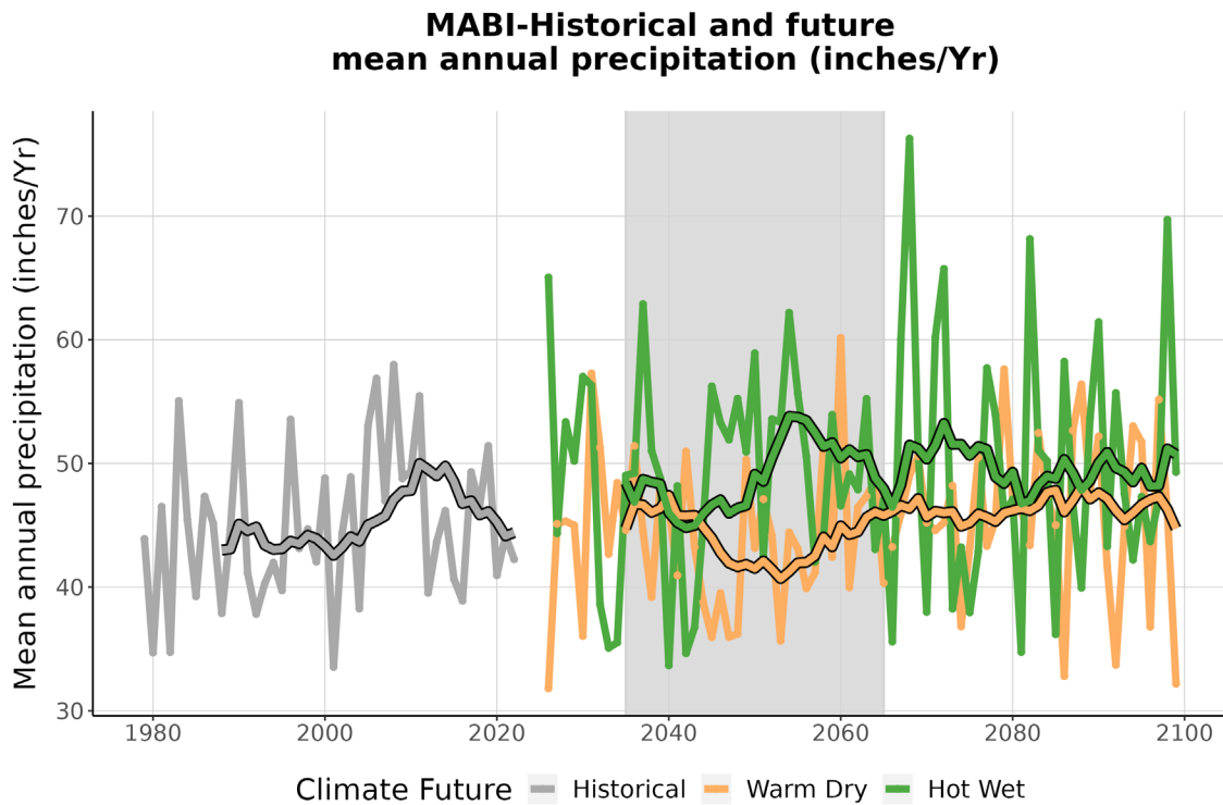
Figure 4. This graph compares observed average annual precipitation at MABI (inches/year) (1979-2022) with projected average annual precipitation for the two climate futures over the period 2023-2099. The historically observed data is shown in gray, the Warm Dry climate future in orange, and the Hot Wet climate future in green. The smooth line running through each projection is the 10-year running average for historical observations and future projections. The gray-shaded area represents the time period that was averaged (2035-2065) to summarize future projections for the year 2050 (Appendix 1).
