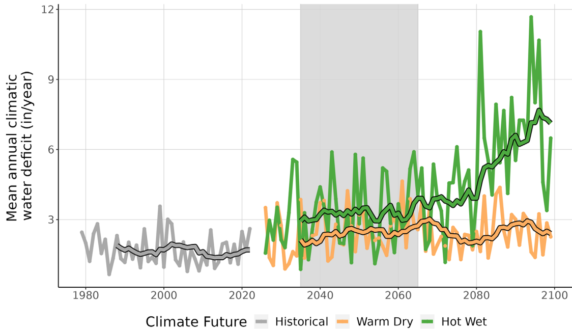
Figure 9. This line graph compares observed climatic water deficit at MABI (inches/year) (1979-2022) with projected climatic water deficit for the two climate futures over the period 2023-2099. The historical observation data is shown in gray, the Warm Dry climate future in orange, and the Hot Wet climate future in green. The smooth line running through each projection is the 10-year running average for historical observations and future projections. Gray-shaded area represents the time period that was averaged (2035-2065) to summarize future projections for the year 2050.
