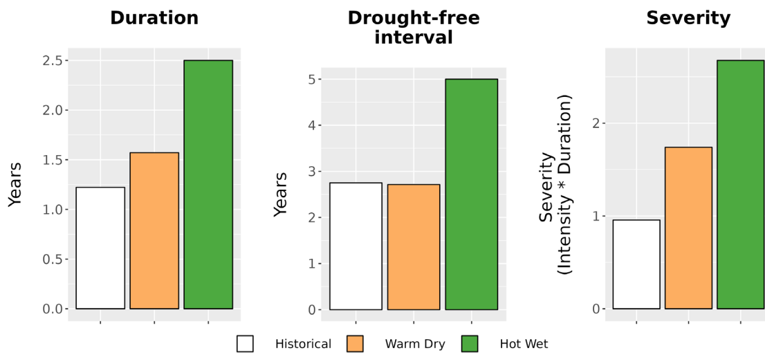
Figure 8. Drought metrics for MABI. (Left) Average drought duration (years) historically (1979-2012) and under each climate future. (Middle) Average drought return interval (years), indicating the expected amount of time between periods of drought, historically and under each climate future. (Right) Average drought severity, a measure of drought intensity multiplied by duration, historically and under each climate future.
