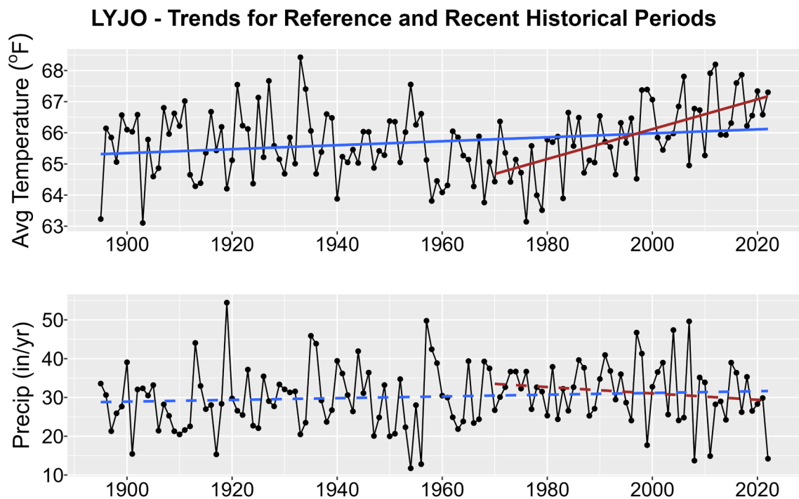
Figure 1. Historical trends in annual average temperature (upper plot) and annual total precipitation (lower plot) for LYJO from 1895-2022. Black points show yearly values while blue lines are linear regressions for the entire period record and red lines for 1970-2022 trends. Solid lines are significant trends (i.e., p < 0.05 ); dashed lines are not statistically significant.
