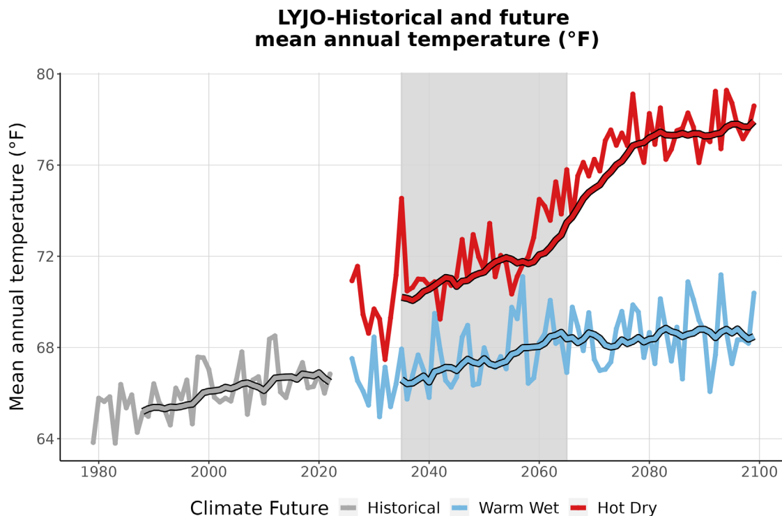
Figure 3. This graph compares observed average annual temperature at LYJO (°F) (1979-2022) with projected average annual temperature for the two climate futures over the period 2023-2099. The historically observed data
