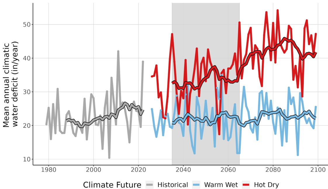
Figure 9. This line graph compares observed climatic water deficit at LYJO (inches/year) (1979-2022) with projected climatic water deficit for the two climate futures over the period 2023-2099. The historical observation data is shown in gray, the Warm Wet climate future in blue, and the Hot Dry climate future in red. The smooth line running through each projection is the 10-year running average for historical observations and future projections. Gray-shaded area represents the time period that was averaged (2035-2065) to summarize future projections for the year 2050.
