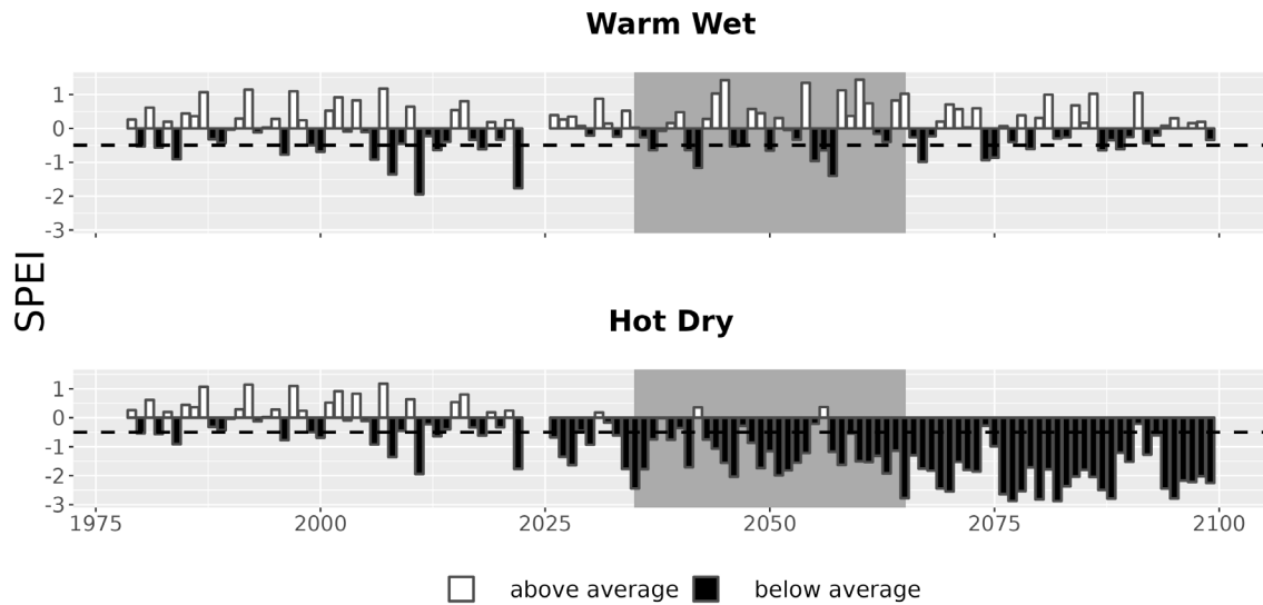
Figure 7. Drought metrics for LYJO. Drought index (SPEI; units = standard deviations from historical) timeseries for each climate future. Below-average SPEI (black bars) indicates dry conditions. The dotted line (SPEI = -0.5) indicates drought conditions.
