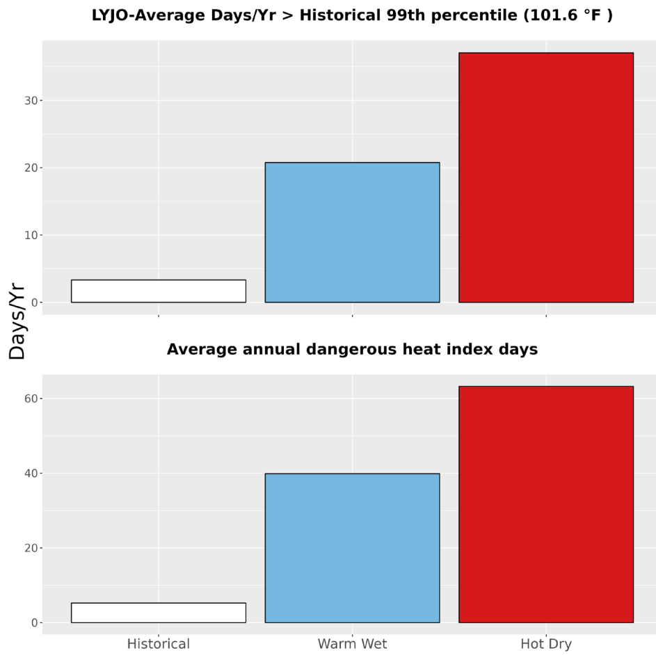
Figure 5. The upper bar graph represents the average number of days annually with temperatures greater than the historical 99th percentile (101.6 °F) historically (1979-2012) and for the two climate futures (2050). The bottom bar graph represents the average annual number of dangerous heat index days historically and for the two climate futures. Dangerous heat index days are days that exceed 105 °F.
