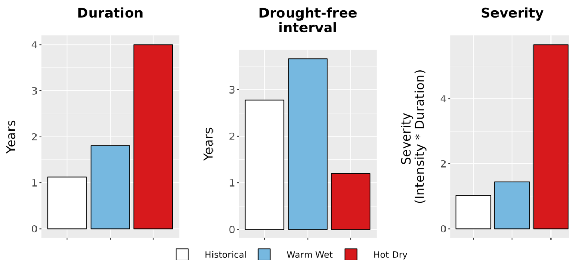
Figure 8. Drought metrics for LYJO. (Left) Average drought duration (years) historically (1979-2012) and under each climate future. (Middle) Average drought return interval (years), indicating the expected amount of time between periods of drought, historically and under each climate future. (Right) Average drought severity, a measure of drought intensity multiplied by duration, historically and under each climate future.
