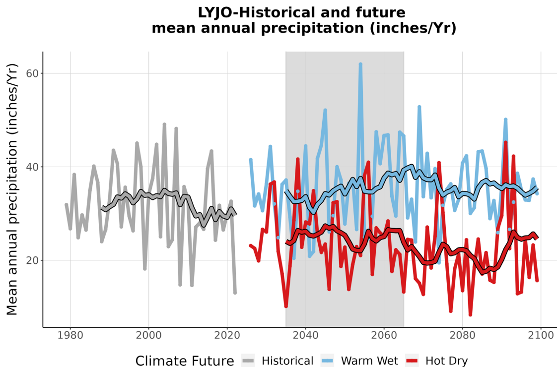
Figure 4. This graph compares observed average annual precipitation at LYJO (inches/year) (1979-2022) with projected average annual precipitation for the two climate futures over the period 2023-2099. The historically observed data is shown in gray, the Warm Wet climate future in blue, and the Hot Dry climate future in red. The smooth line running through each projection is the 10-year running average for historical observations and future projections. The gray-shaded area represents the time period that was averaged (2035-2065) to summarize future projections for the year 2050 (Appendix 1).
