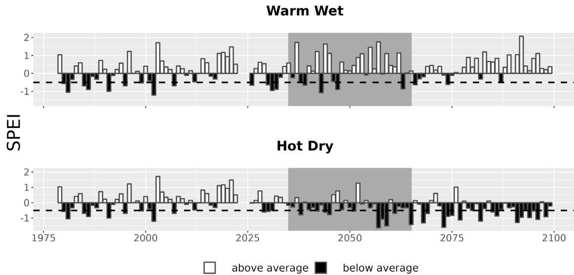
Figure 7. Drought metrics for LYBA. Drought index (SPEI; units = standard deviations from historical) timeseries for each climate future. Below-average SPEI (black bars) indicates dry conditions. The dotted line (SPEI = -0.5) indicates drought conditions.
