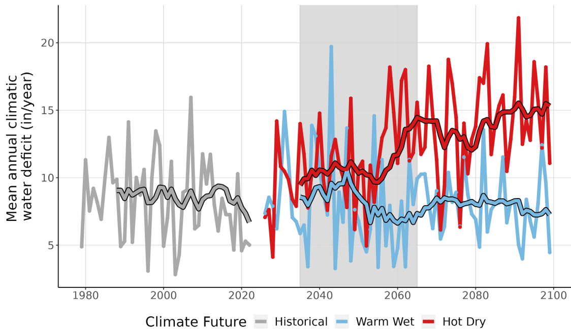
Figure 9. This line graph compares observed climatic water deficit at LYBA (inches/year) (1979-2022) with projected climatic water deficit for the two climate futures over the period 2023-2099. The historical observation data is shown in gray, the Warm Wet climate future in blue, and the Hot Dry climate future in red. The smooth line running through each projection is the 10-year running average for historical observations and future projections. Gray-shaded area represents the time period that was averaged (2035-2065) to summarize future projections for the year 2050.
