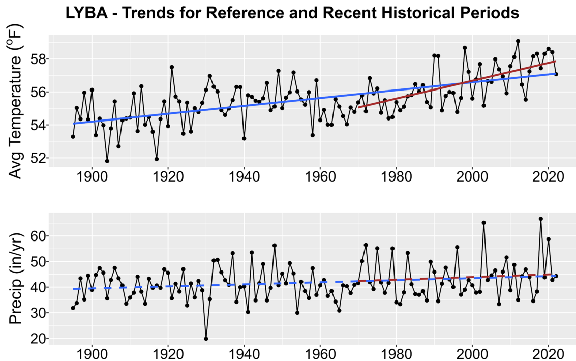
Figure 1. Historical trends in annual average temperature (upper plot) and annual total precipitation (lower plot) for LYBA from 1895-2022. Black points show yearly values while blue lines are linear regressions for the entire period record and red lines for 1970-2022 trends. Solid lines are significant trends (i.e., p < 0.05 ); dashed lines are not statistically significant.
