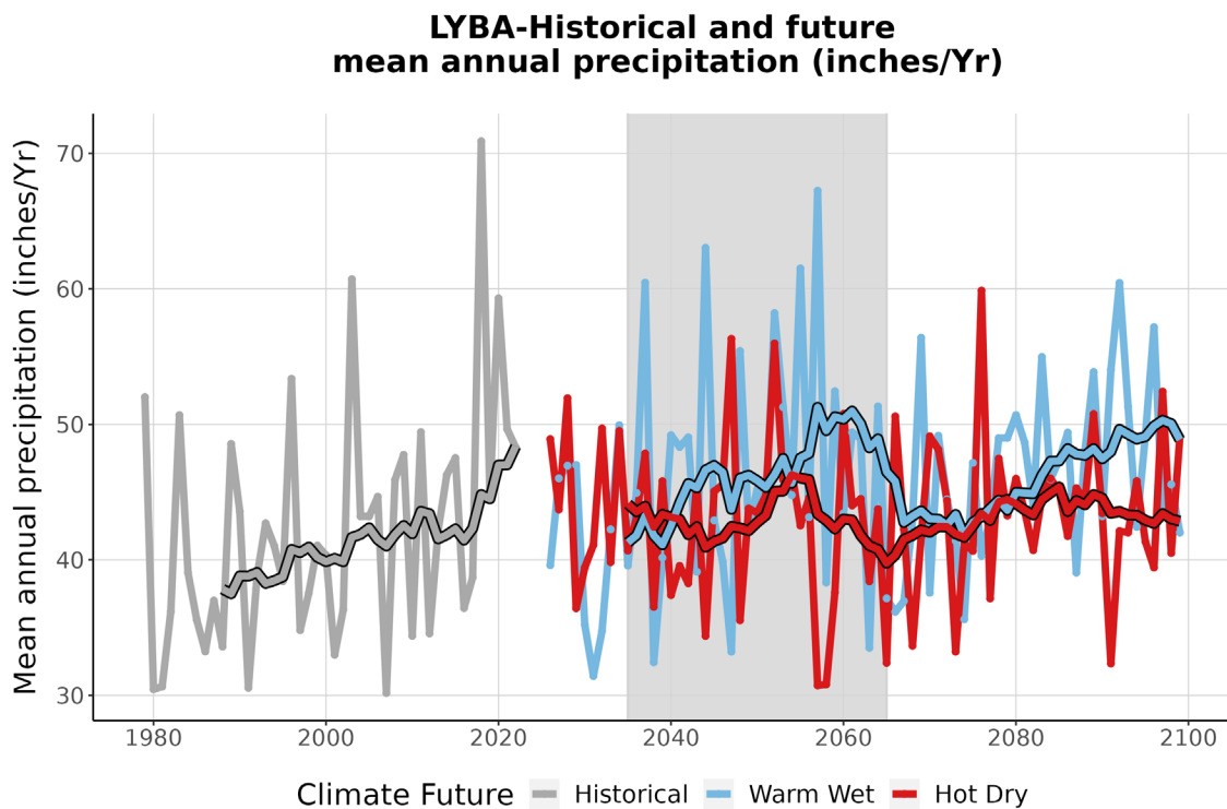
Figure 4. This graph compares observed average annual precipitation at LYBA (inches/year) (1979-2022) with projected average annual precipitation for the two climate futures over the period 2023-2099. The historically observed data is shown in gray, the Warm Wet climate future in blue, and the Hot Dry climate future in red. The smooth line running through each projection is the 10-year running average for historical observations and future projections. The gray-shaded area represents the time period that was averaged (2035-2065) to summarize future projections for the year 2050 (Appendix 1).
