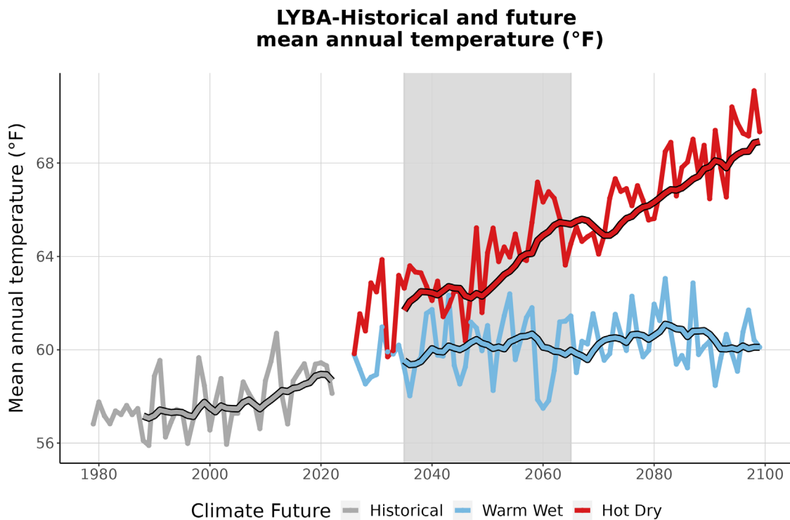
Figure 3. This graph compares observed average annual temperature at LYBA (°F) (1979-2022) with projected average annual temperature for the two climate futures over the period 2023-2099. The historically observed data is shown in gray, the Warm Wet climate future in blue, and the Hot Dry climate future in red. The smooth line
