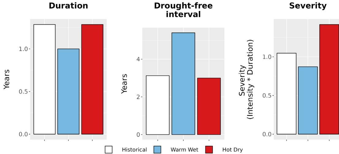
Figure 8. Drought metrics for LYBA. (Left) Average drought duration (years) historically (1979-2012) and under each climate future. (Middle) Average drought return interval (years), indicating the expected amount of time between periods of drought, historically and under each climate future. (Right) Average drought severity, a measure of drought intensity multiplied by duration, historically and under each climate future.
