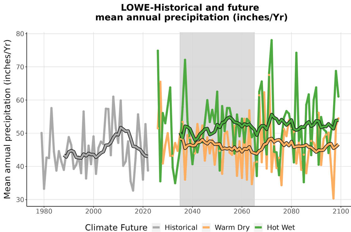
Figure 4. This graph compares observed average annual precipitation at LOWE (inches/year) (1979-2022) with projected average annual precipitation for the two climate futures over the period 2023-2099. The historically observed data is shown in gray, the Warm Dry climate future in orange, and the Hot Wet climate future in green. The smooth line running through each projection is the 10-year running average for historical observations and future projections. The gray-shaded area represents the time period that was averaged (2035-2065) to summarize future projections for the year 2050 (Appendix 1).
