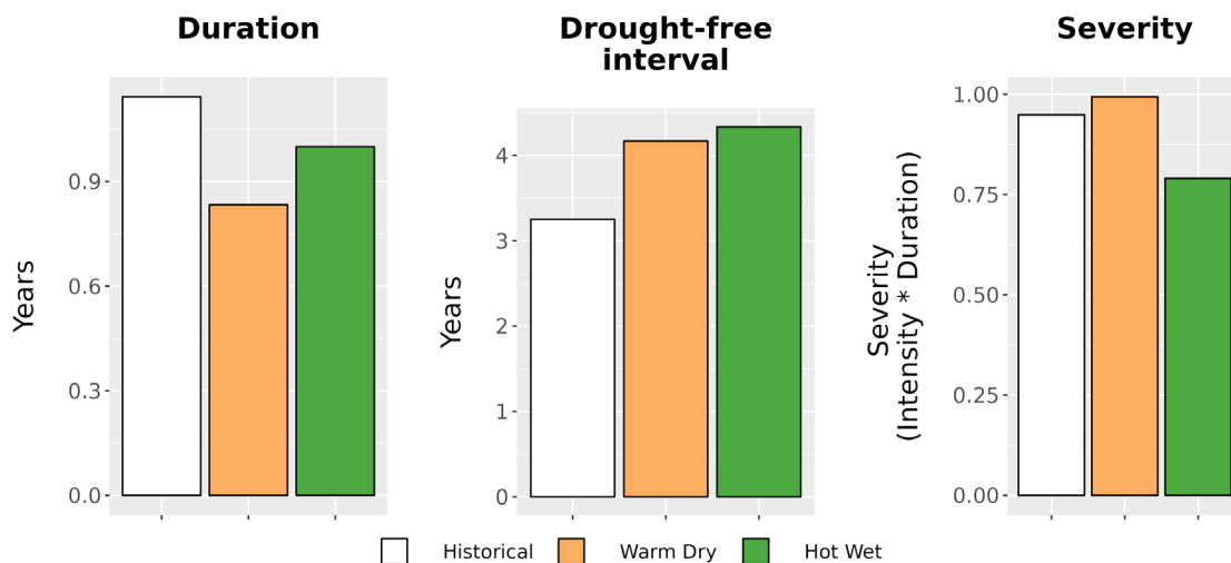
Figure 8. Drought metrics for LOWE. (Left) Average drought duration (years) historically (1979-2012) and under each climate future. (Middle) Average drought return interval (years), indicating the expected amount of time between periods of drought, historically and under each climate future. (Right) Average drought severity, a measure of drought intensity multiplied by duration, historically and under each climate future.
