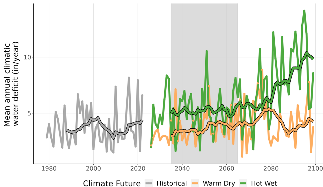
Figure 9. This line graph compares observed climatic water deficit at LOWE (inches/year) (1979-2022) with projected climatic water deficit for the two climate futures over the period 2023-2099. The historical observation data is shown in gray, the Warm Dry climate future in orange, and the Hot Wet climate future in green. The smooth line running through each projection is the 10-year running average for historical observations and future projections. Gray-shaded area represents the time period that was averaged (2035-2065) to summarize future projections for the year 2050.
