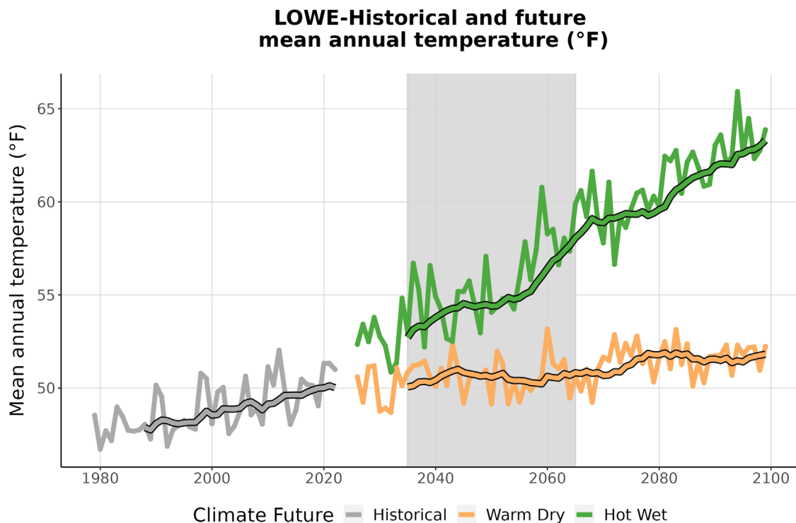
Figure 3. This graph compares observed average annual temperature at LOWE (°F) (1979-2022) with projected average annual temperature for the two climate futures over the period 2023-2099. The historically observed data
