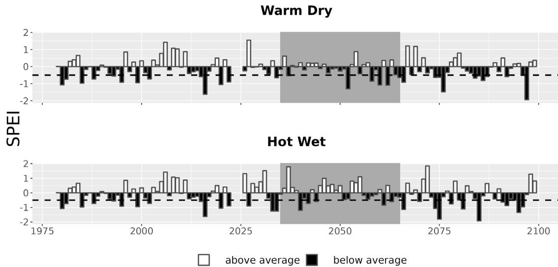
Figure 7. Drought metrics for LOWE. Drought index (SPEI; units = standard deviations from historical) timeseries for each climate future. Below-average SPEI (black bars) indicates dry conditions. The dotted line (SPEI = -0.5) indicates drought conditions.
