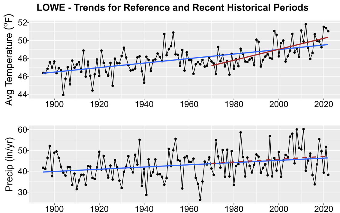
Figure 1. Historical trends in annual average temperature (upper plot) and annual total precipitation (lower plot) for LOWE from 1895-2022. Black points show yearly values while blue lines are linear regressions for the entire period record and red lines for 1970-2022 trends. Solid lines are significant trends (i.e., p < 0.05 ); dashed lines are not statistically significant.
