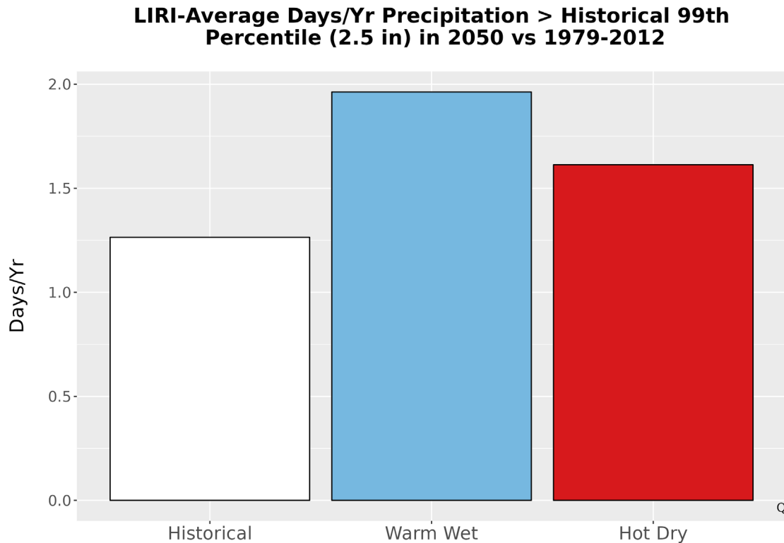
Figure 6. Average number of days annually with precipitation exceeding the 99th percentile (2.5 in.) of precipitation from the historical period 1979-2012 and for each climate future.
