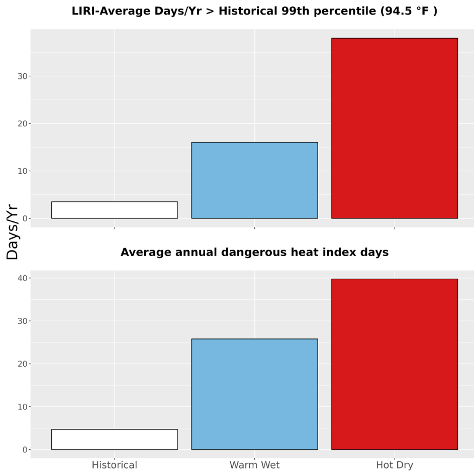
Figure 5. The upper bar graph represents the average number of days annually with temperatures greater than the historical 99th percentile (94.5 °F) historically (1979-2012) and for the two climate futures (2050). The bottom bar graph represents the average annual number of dangerous heat index days historically and for the two climate futures. Dangerous heat index days are days that exceed 105 °F.
