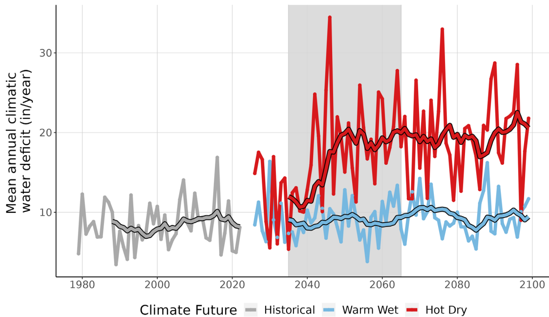
Figure 9. This line graph compares observed climatic water deficit at LIRI (inches/year) (1979-2022) with projected climatic water deficit for the two climate futures over the period 2023-2099. The historical observation data is shown in gray, the Warm Wet climate future in blue, and the Hot Dry climate future in red. The smooth line running through each projection is the 10-year running average for historical observations and future projections. Gray-shaded area represents the time period that was averaged (2035-2065) to summarize future projections for the year 2050.
