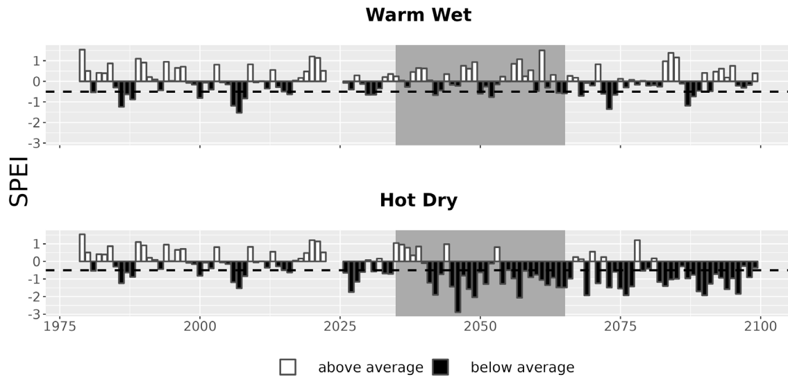
Figure 7. Drought metrics for LIRI. Drought index (SPEI; units = standard deviations from historical) timeseries for each climate future. Below-average SPEI (black bars) indicates dry conditions. The dotted line (SPEI = -0.5) indicates drought conditions.
