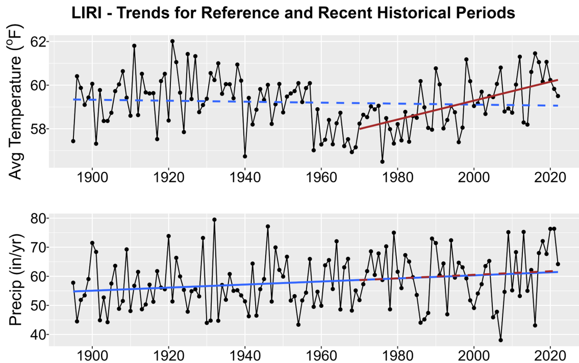
Figure 1. Historical trends in annual average temperature (upper plot) and annual total precipitation (lower plot) for LIRI from 1895-2022. Black points show yearly values while blue lines are linear regressions for the entire period record and red lines for 1970-2022 trends. Solid lines are significant trends (i.e., p < 0.05 ); dashed lines are not statistically significant.
