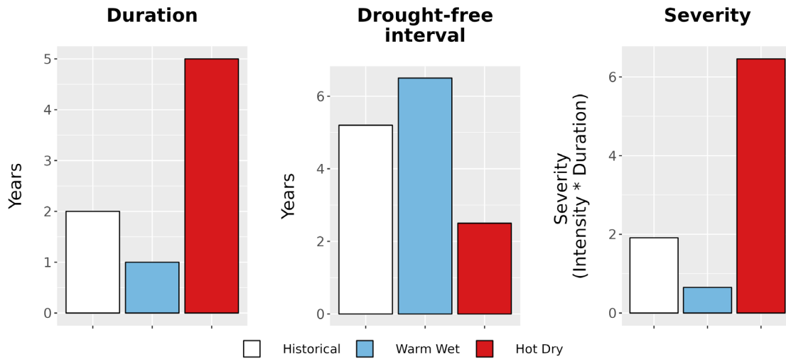
Figure 8. Drought metrics for LIRI. (Left) Average drought duration (years) historically (1979-2012) and under each climate future. (Middle) Average drought return interval (years), indicating the expected amount of time between periods of drought, historically and under each climate future. (Right) Average drought severity, a measure of drought intensity multiplied by duration, historically and under each climate future.
