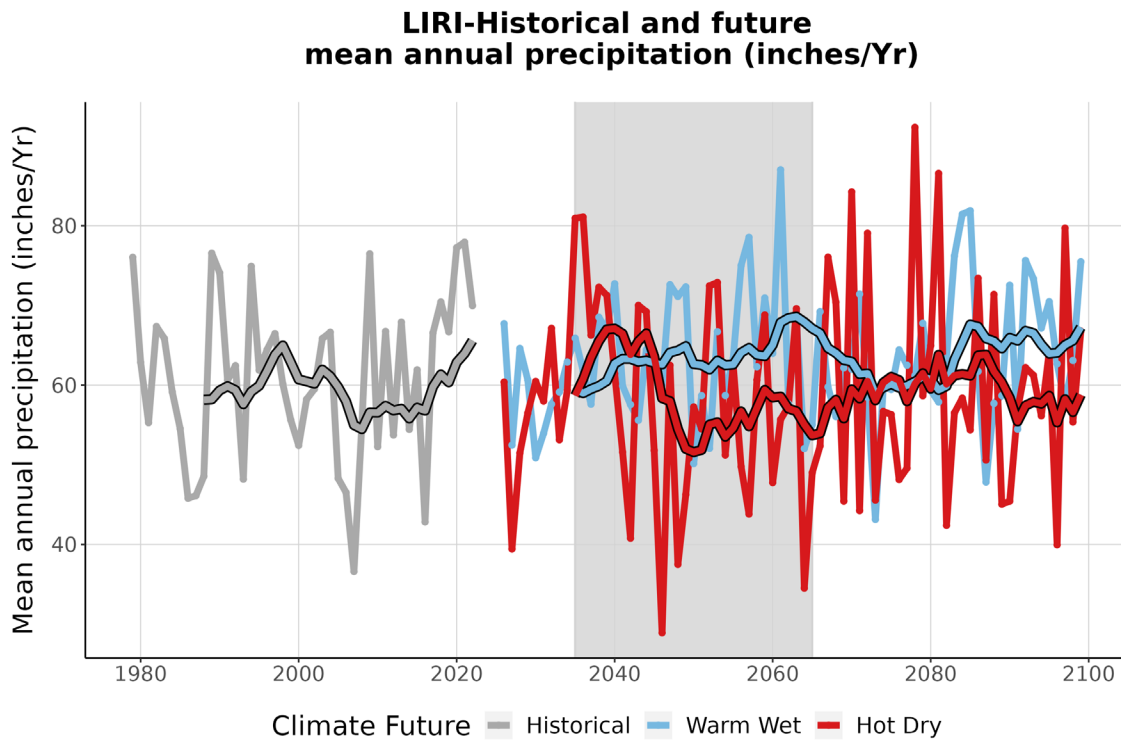
Figure 4. This graph compares observed average annual precipitation at LIRI (inches/year) (1979-2022) with projected average annual precipitation for the two climate futures over the period 2023-2099. The historically observed data is shown in gray, the Warm Wet climate future in blue, and the Hot Dry climate future in red. The smooth line running through each projection is the 10-year running average for historical observations and future projections. The gray-shaded area represents the time period that was averaged (2035-2065) to summarize future projections for the year 2050 (Appendix 1).
