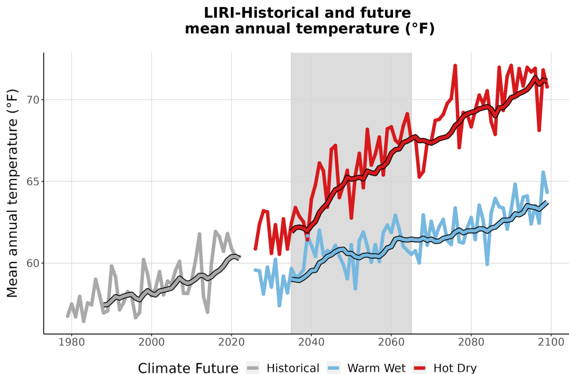
Figure 3. This graph compares observed average annual temperature at LIRI (°F) (1979-2022) with projected average annual temperature for the two climate futures over the period 2023-2099. The historically observed data
