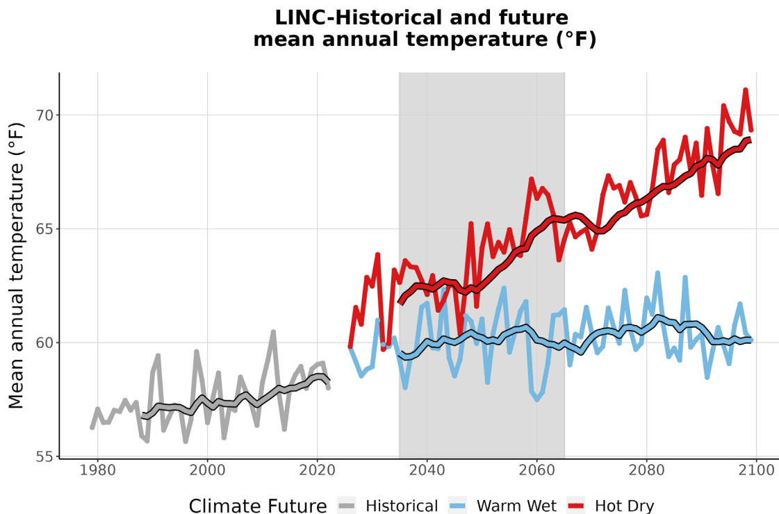
Figure 3. This graph compares observed average annual temperature at LINC (°F) (1979-2022) with projected average annual temperature for the two climate futures over the period 2023-2099. The historically observed data
