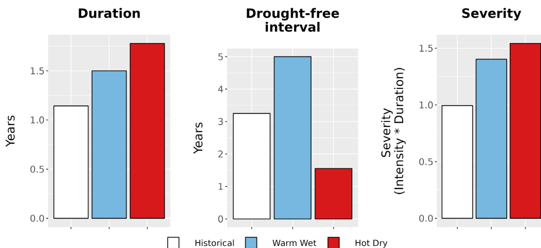
Figure 8. Drought metrics for LINC. (Left) Average drought duration (years) historically (1979-2012) and under each climate future. (Middle) Average drought return interval (years), indicating the expected amount of time between periods of drought, historically and under each climate future. (Right) Average drought severity, a measure of drought intensity multiplied by duration, historically and under each climate future.
