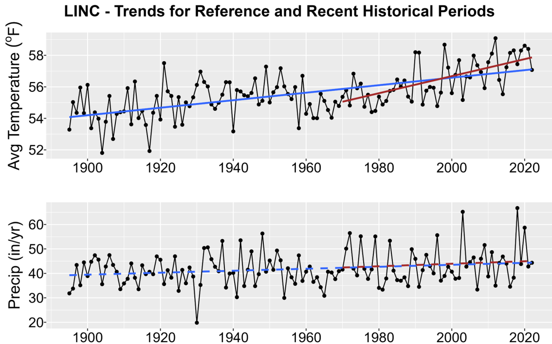
Figure 1. Historical trends in annual average temperature (upper plot) and annual total precipitation (lower plot) for LINC from 1895-2022. Black points show yearly values while blue lines are linear regressions for the entire period record and red lines for 1970-2022 trends. Solid lines are significant trends (i.e., p < 0.05 ); dashed lines are not statistically significant.
