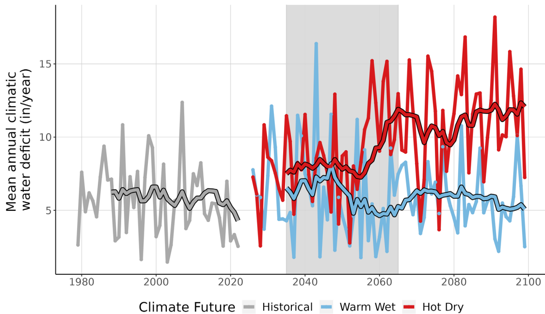
Figure 9. This line graph compares observed climatic water deficit at LINC (inches/year) (1979-2022) with projected climatic water deficit for the two climate futures over the period 2023-2099. The historical observation data is shown in gray, the Warm Wet climate future in blue, and the Hot Dry climate future in red. The smooth line running through each projection is the 10-year running average for historical observations and future projections. Gray-shaded area represents the time period that was averaged (2035-2065) to summarize future projections for the year 2050.
