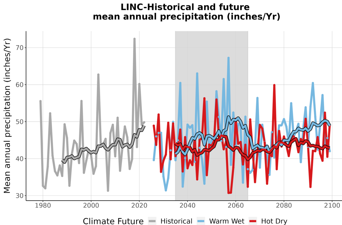
Figure 4. This graph compares observed average annual precipitation at LINC (inches/year) (1979-2022) with projected average annual precipitation for the two climate futures over the period 2023-2099. The historically observed data is shown in gray, the Warm Wet climate future in blue, and the Hot Dry climate future in red. The smooth line running through each projection is the 10-year running average for historical observations and future projections. The gray-shaded area represents the time period that was averaged (2035-2065) to summarize future projections for the year 2050 (Appendix 1).
