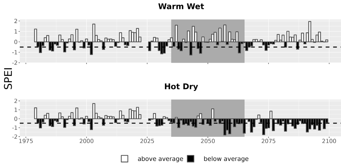
Figure 7. Drought metrics for LINC. Drought index (SPEI; units = standard deviations from historical) timeseries for each climate future. Below-average SPEI (black bars) indicates dry conditions. The dotted line (SPEI = -0.5) indicates drought conditions.
